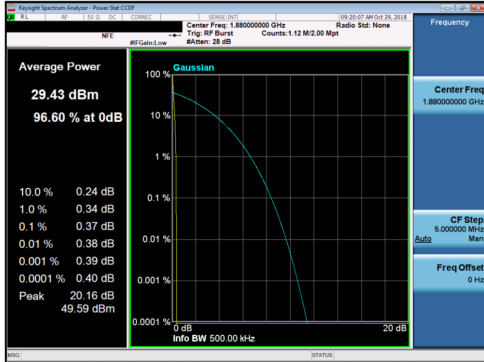
Plot 7-54. Peak-Average Ratio Plot (PCS GPRS Mode)
