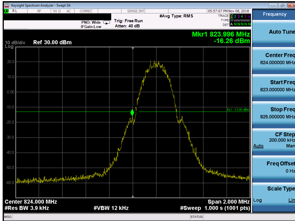
Plot 7-43. Band Edge Plot (Cellular GPRS Mode - Low Channel)
