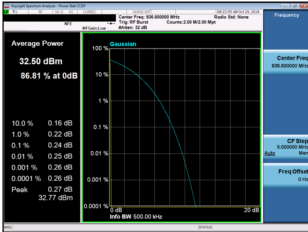
Plot 7-53. Peak-Average Ratio Plot (Cellular GPRS Mode)
