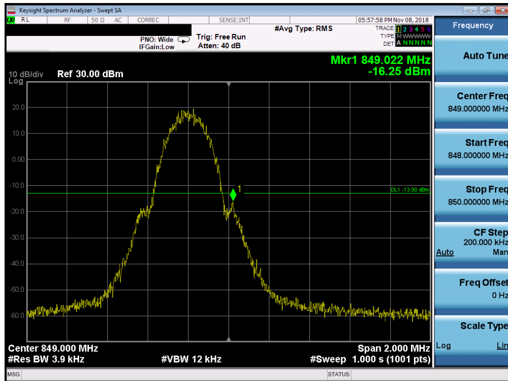
Plot 7-44. Band Edge Plot (Cellular GPRS Mode - High Channel)
