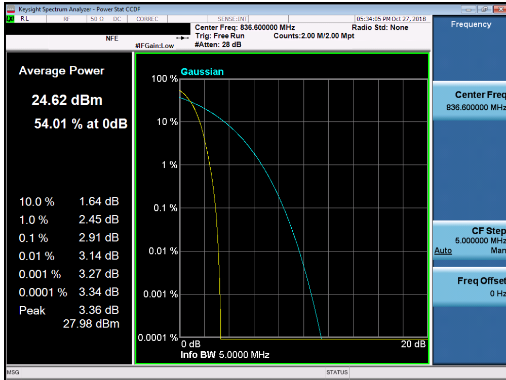
Plot 7-55. Peak-Average Ratio Plot (Cellular WCDMA Mode)
