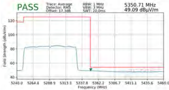
Plot 7-311. Radiated Band Edge Plot SISO ANT1 (Average – WCP)
