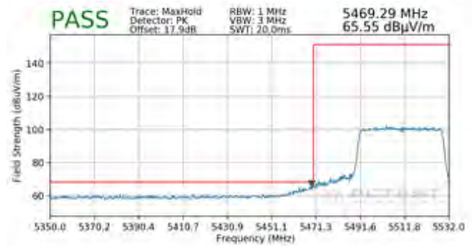
Plot 7-357. Radiated Band Edge Plot MIMO (Peak – WCP)
