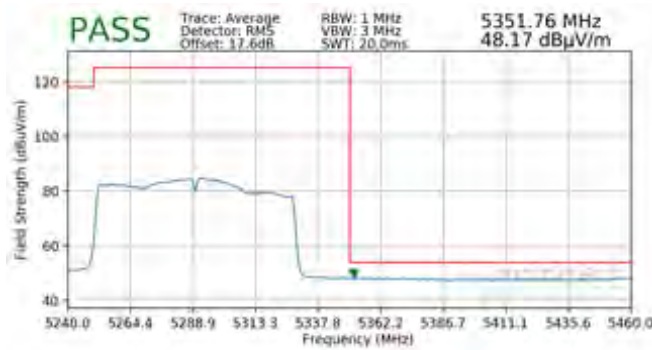
Plot 7-338. Radiated Band Edge Plot SISO ANT2 (Average - WCP)
