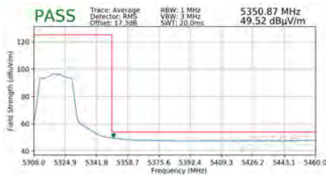
Plot 7-293. Radiated Band Edge Plot SISO ANT1 (Average – WCP)
