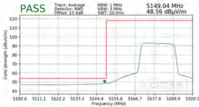
Plot 7-320. Radiated Band Edge Plot SISO ANT2 (Average – WCP)
