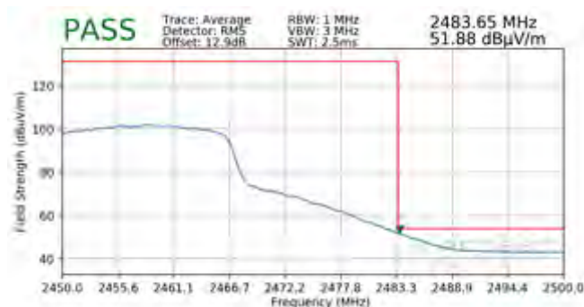
Plot 7-137. Radiated Restricted Upper Band Edge Measurement MIMO (Average)
