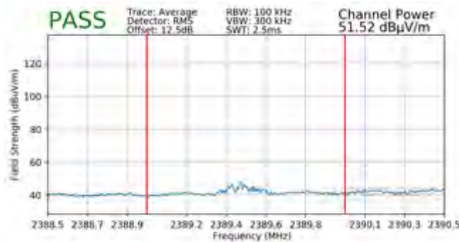
Plot 7-133. Radiated Restricted Lower Band Edge Measurement MIMO (Average)
