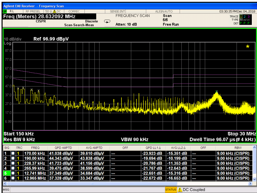
Plot 7-166. Line Conducted Plot with 802.11b (L1) with Wireless Charging Pad
