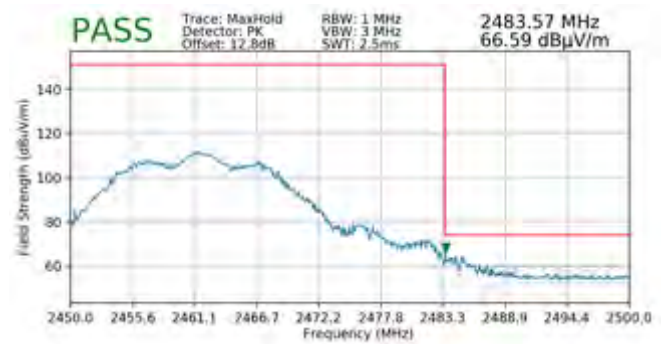
Plot 7-160. Radiated Restricted Band Edge Measurement MIMO with WCP (Peak)
