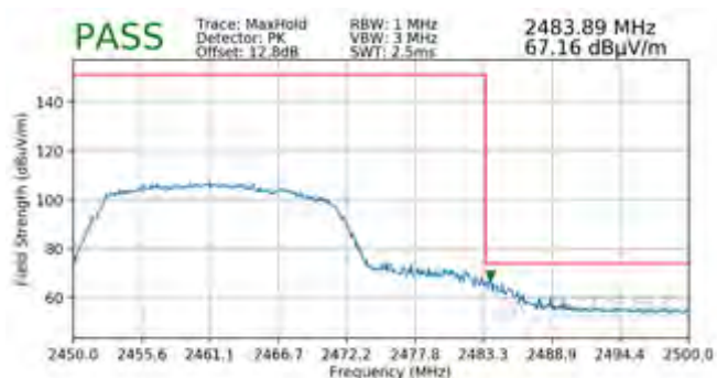
Plot 7-146. Radiated Restricted Band Edge Measurement MIMO with WCP (Peak)
