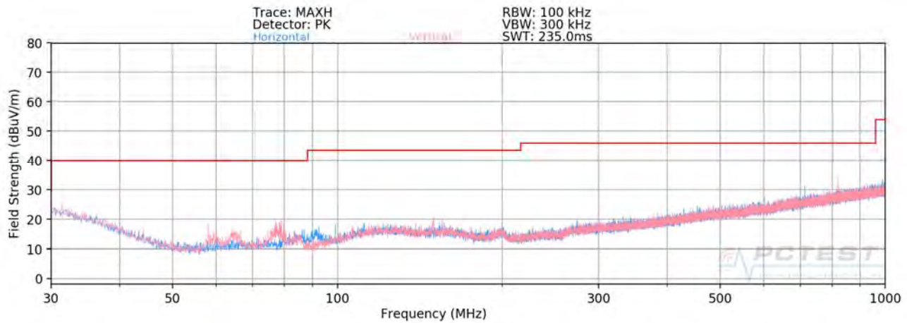
Plot 7-163. Radiated Spurious Plot below 1GHz CDD/MIMO
