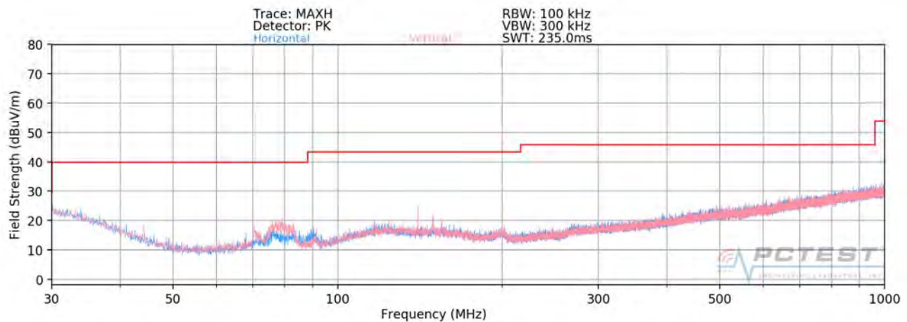
Plot 7-162. Radiated Spurious Plot below 1GHz SISO ANT2
