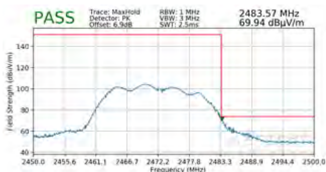
Plot 7-158. Radiated Restricted Upper Band Edge Measurement CDD (Peak)
