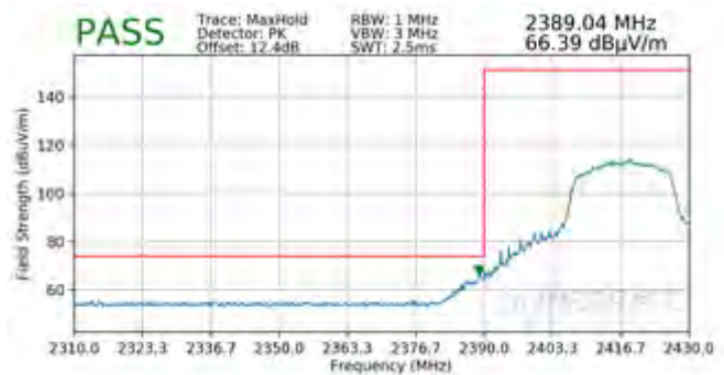
Plot 7-136. Radiated Restricted Lower Band Edge Measurement MIMO (Peak)
