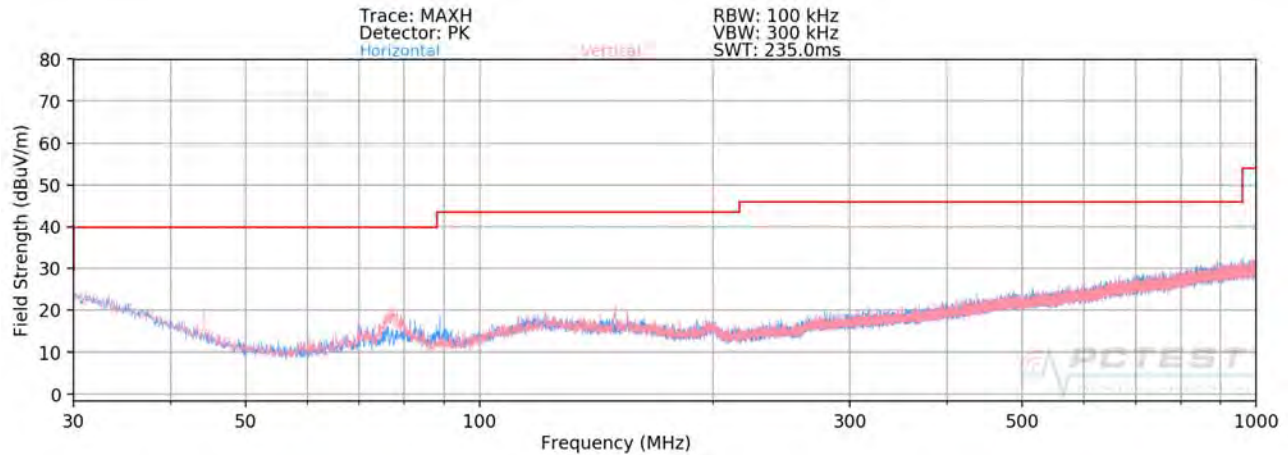
Plot 7-161. Radiated Spurious Plot below 1GHz SISO ANT1
