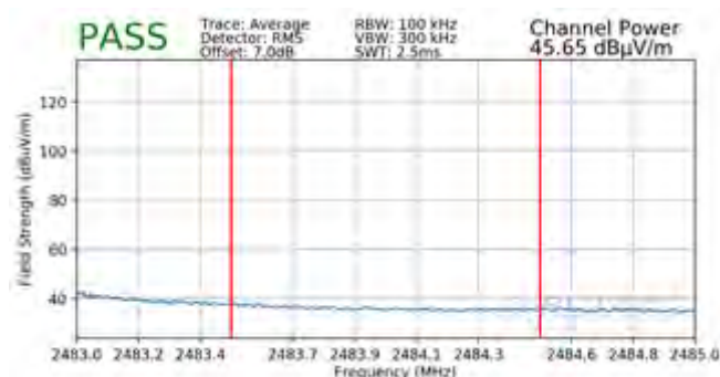
Plot 7-143. Radiated Restricted Upper Band Edge Measurement MIMO (Average)
