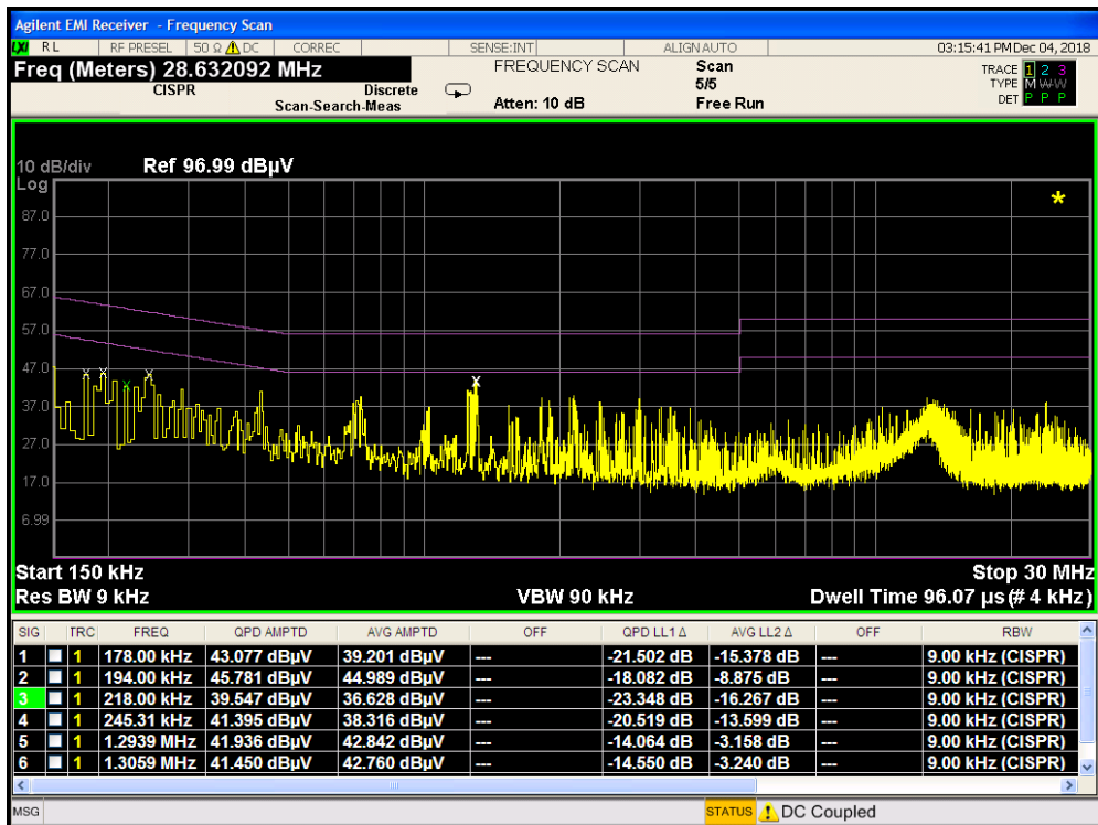
Plot 7-167. Line Conducted Plot with 802.11b (N) with Wireless Charging Pad
