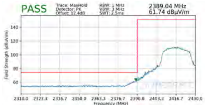
Plot 7-122. Radiated Restricted Lower Band Edge Measurement SISO ANT2 (Peak)
