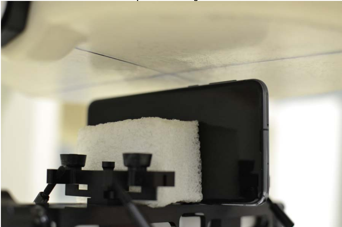
SAR Test Setup Photo 12 – Left Side at 10 mm
