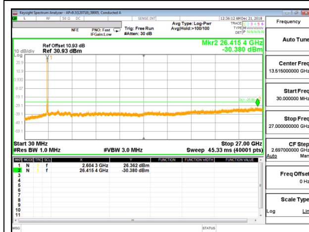
LTE B38 20MHz + 20MHz QPSK High Channel RB1-99 + RB1-0
