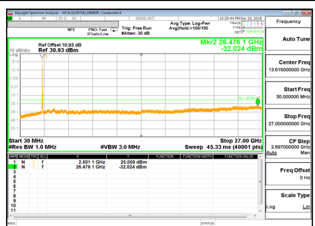
LTE B7 20MHz + 20MHz 16QAM Low Channel RB1-99 + RB1-0
