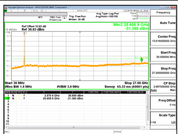
LTE B38 20MHz+20MHz 16QAM Low Channel RB1-99 + RB1-0
