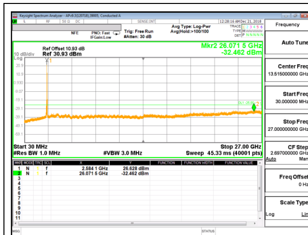
LTE B38 20MHz + 20MHz QPSK Low Channel RB1-99 + RB1-0
