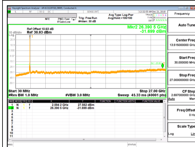
LTE B38 20MHz + 20MHz 16QAM Mid Channel RB1-99 + RB1-0
