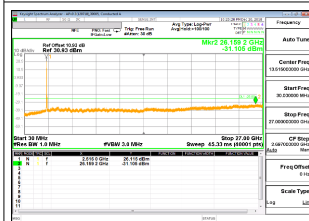
LTE B7 20MHz + 20MHz 16QAM Mid Channel RB1-99 + RB1-0
