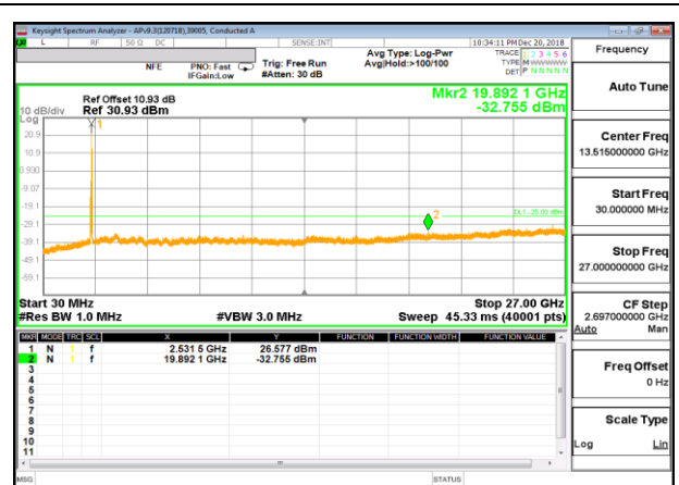
LTE B7 20MHz + 20MHz 16QAM High Channel RB1-99 + RB1-0
