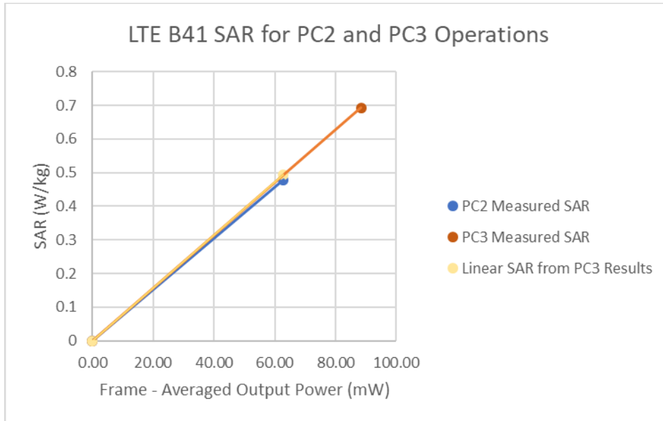
Figure 14-5 LTE Band 41 Single Carrier Hotspot Linearity
