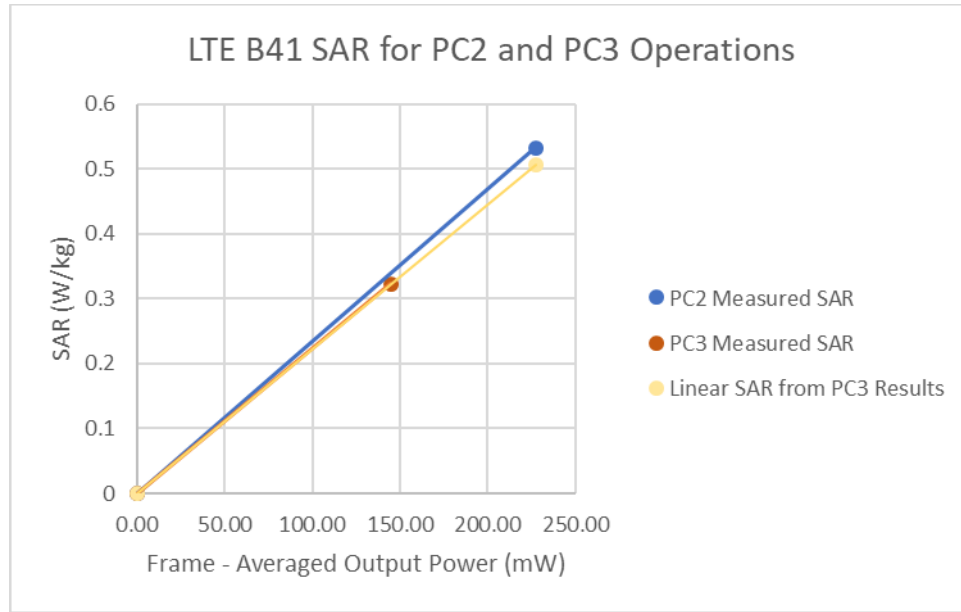
Figure 14-3 LTE Band 41 Single Carrier Body-Worn Linearity
