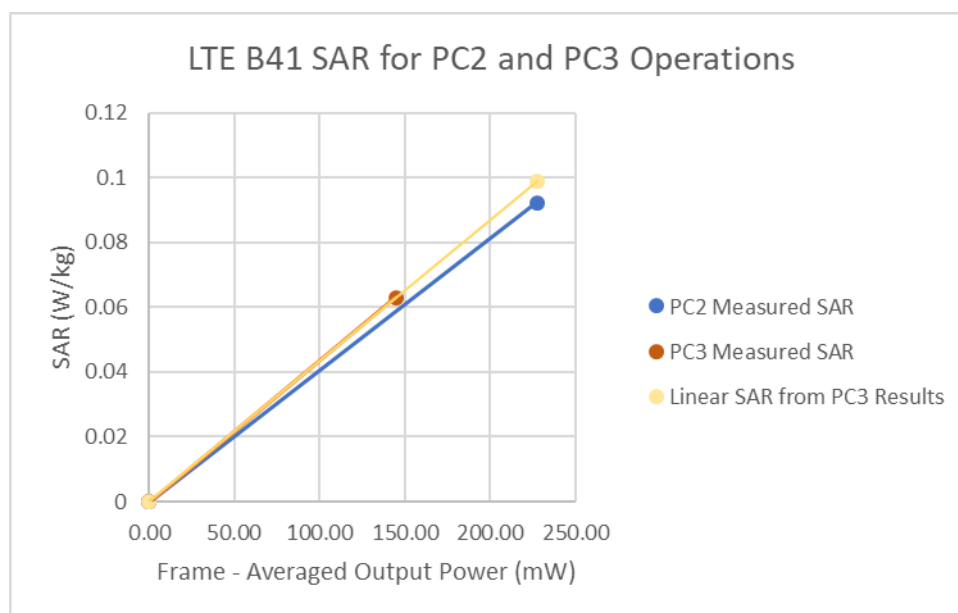
Figure 14-1 LTE Band 41 Single Carrier Head Linearity
