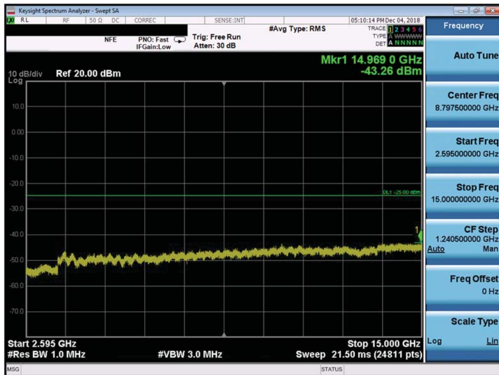
Plot 7-245. Conducted Spurious Plot (Band 7 Ant A - 20.0MHz QPSK - RB Size 1, RB Offset 0 - High Channel)
