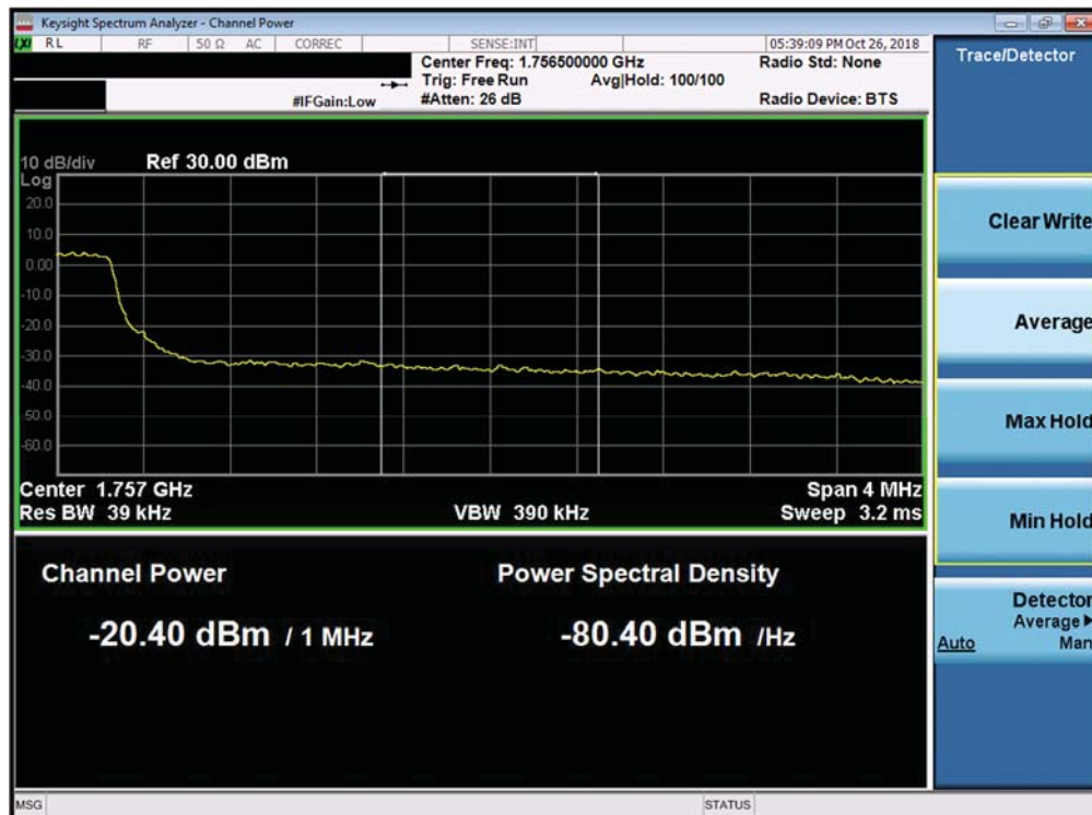
Plot 7-323. Upper Extended Band Edge Plot (Band 4 - 5.0MHz QPSK - Full RB Configuration)
