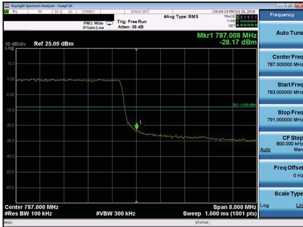
Plot 7-296. Upper Band Edge Plot (Band 13 - 10.0MHz QPSK - Full RB Configuration)
