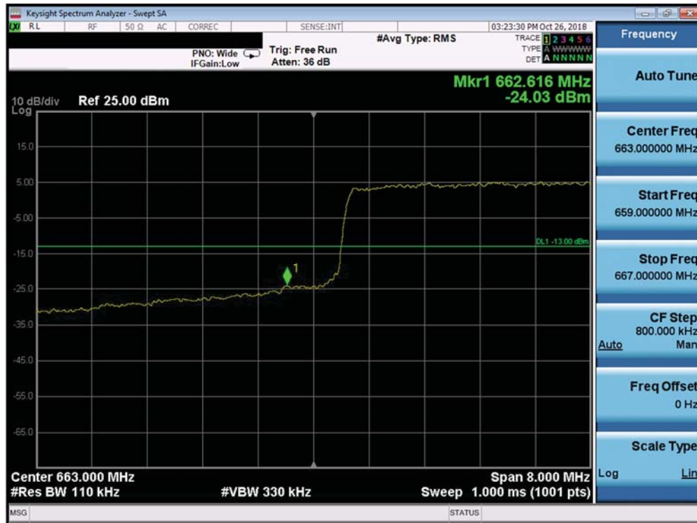
Plot 7-276. Lower Band Edge Plot (Band 71 - 10.0MHz QPSK - Full RB Configuration)
