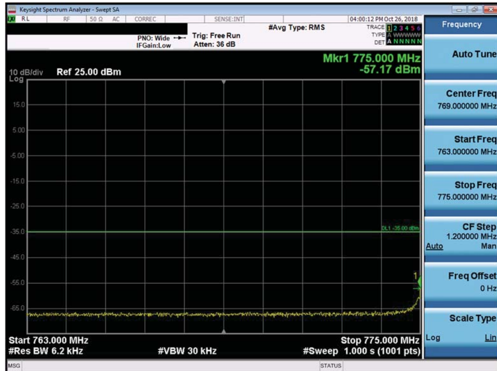
Plot 7-291. Lower Emission Mask Plot (Band 13 - 5.0MHz QPSK - Full RB Configuration)
