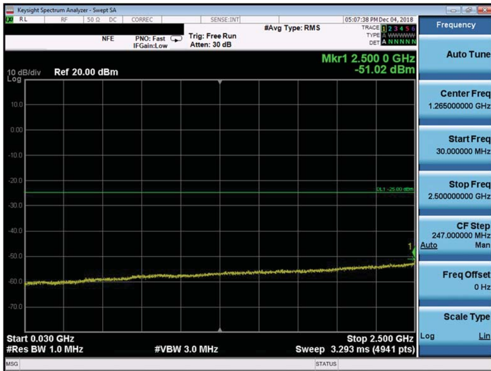
Plot 7-241. Conducted Spurious Plot (Band 7 Ant A - 20.0MHz QPSK - RB Size 1, RB Offset 0 - Mid Channel)
