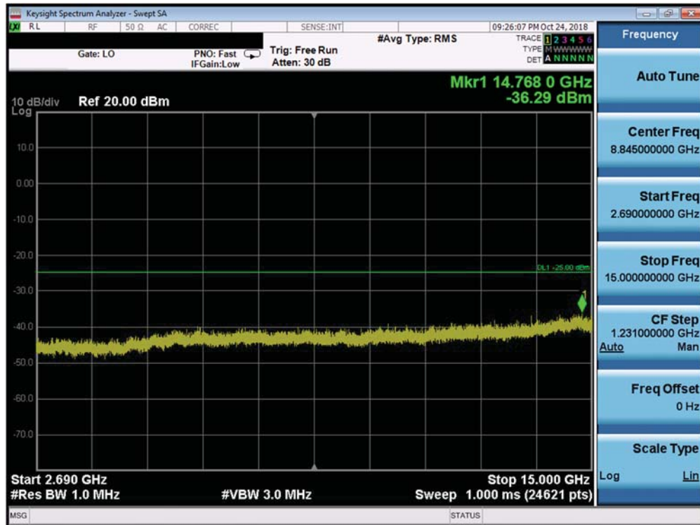
Plot 7-260. Conducted Spurious Plot (Band 41 PC2 - 20.0MHz QPSK - RB Size 1, RB Offset 0 - Mid Channel)
