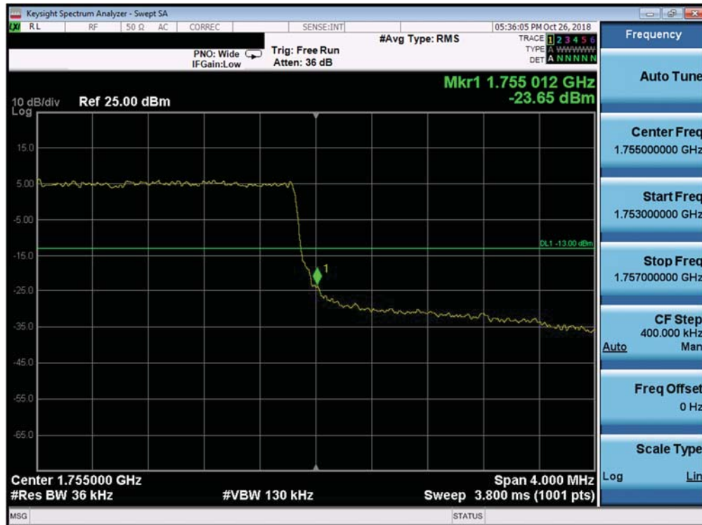
Plot 7-316. Upper Band Edge Plot (Band 4 - 3.0MHz QPSK - Full RB Configuration)
