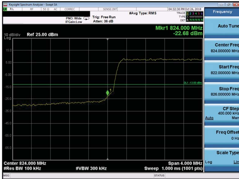
Plot 7-302. Lower Band Edge Plot (Band 26/5 - 5.0MHz QPSK - Full RB Configuration)
