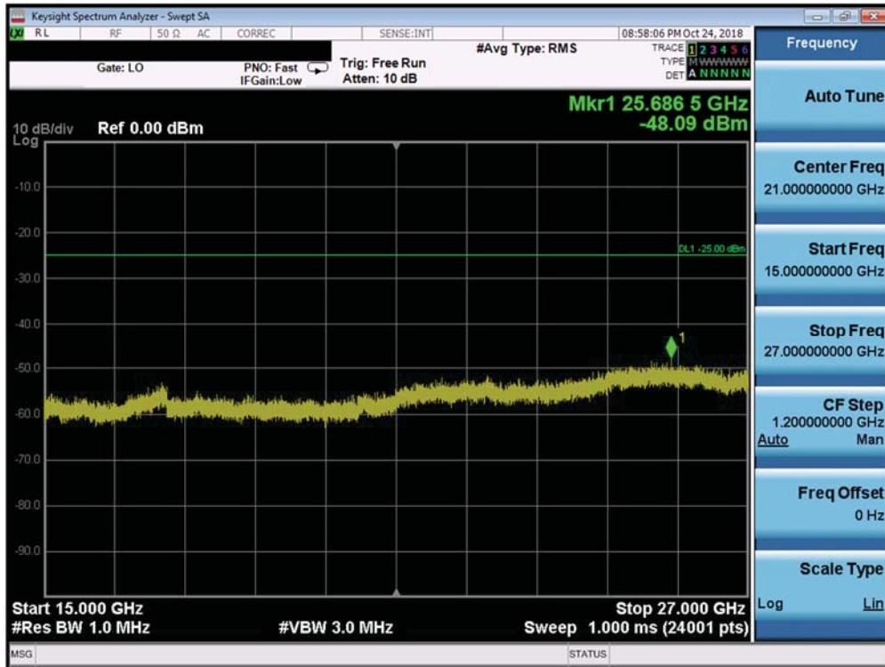
Plot 7-267. Conducted Spurious Plot (Band 41 PC3 / Band 38 - 20.0MHz QPSK - RB Size 1, RB Offset 0 - Low Channel)
