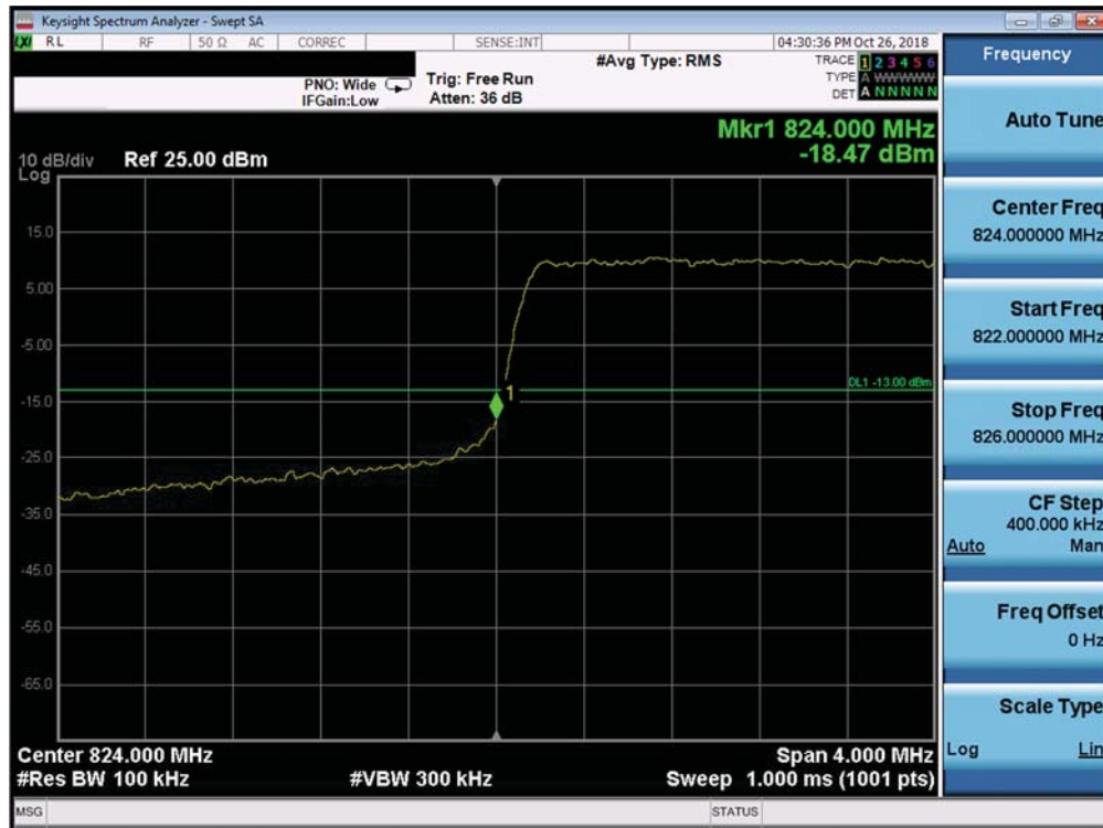
Plot 7-300. Lower Band Edge Plot (Band 26/5 - 3.0MHz QPSK - Full RB Configuration)
