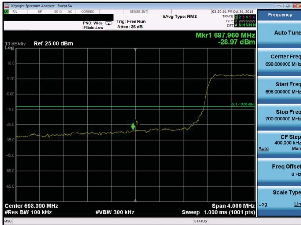
Plot 7-286. Lower Band Edge Plot (Band 12 - 5.0MHz QPSK - Full RB Configuration)
