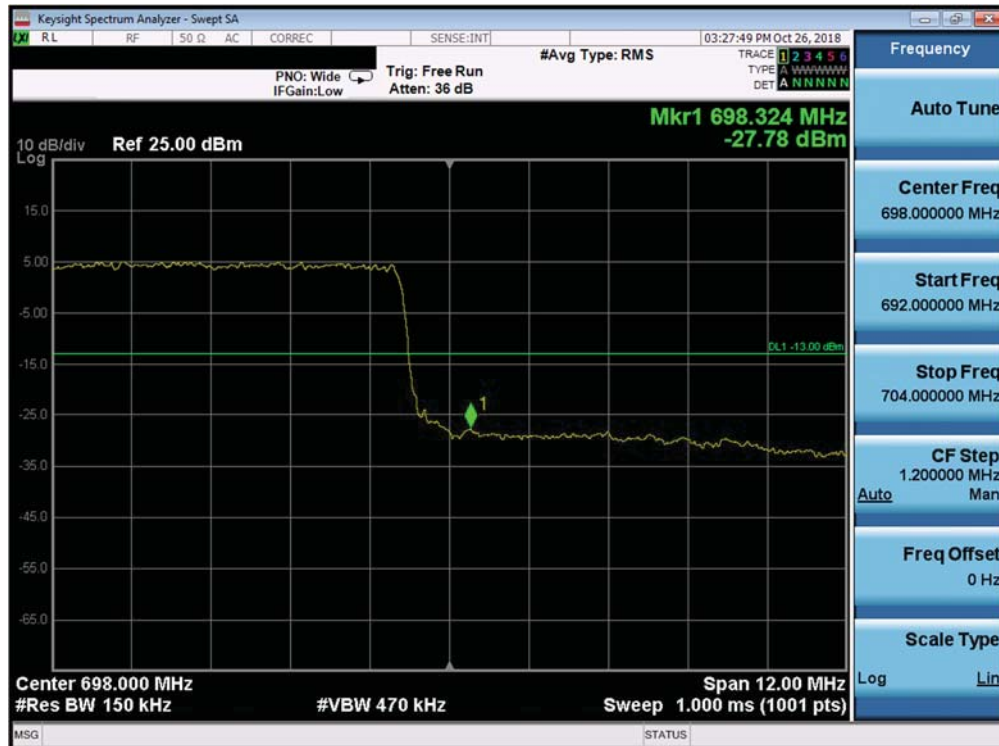
Plot 7-279. Upper Band Edge Plot (Band 71 - 15.0MHz QPSK - Full RB Configuration)
