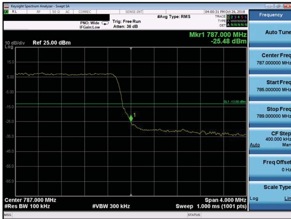
Plot 7-292. Upper Band Edge Plot (Band 13 - 5.0MHz QPSK - Full RB Configuration)
