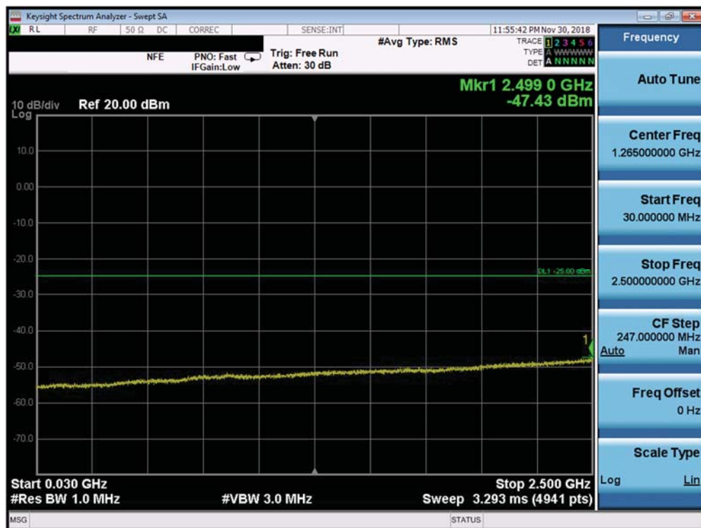
Plot 7-250. Conducted Spurious Plot (Band 7 ANT B - 20.0MHz QPSK - RB Size 1, RB Offset 0 - Mid Channel)
