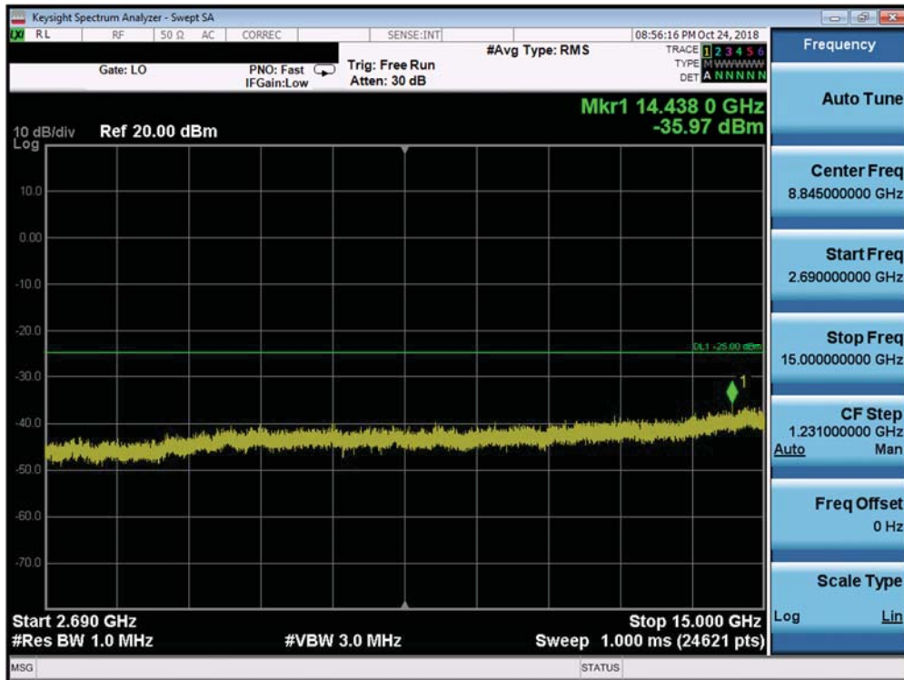
Plot 7-269. Conducted Spurious Plot (Band 41 PC3 / Band 38 - 20.0MHz QPSK - RB Size 1, RB Offset 0 - Mid Channel)
