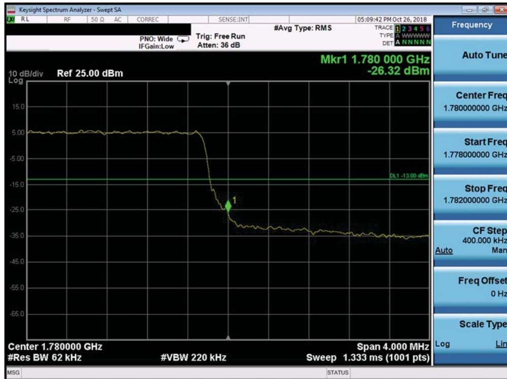
Plot 7-324. Upper Band Edge Plot (Band 66 - 5.0MHz QPSK - Full RB Configuration)
