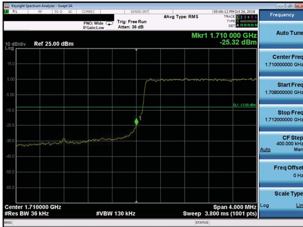
Plot 7-314. Lower Band Edge Plot (Band 66/4 - 3.0MHz QPSK - Full RB Configuration)
