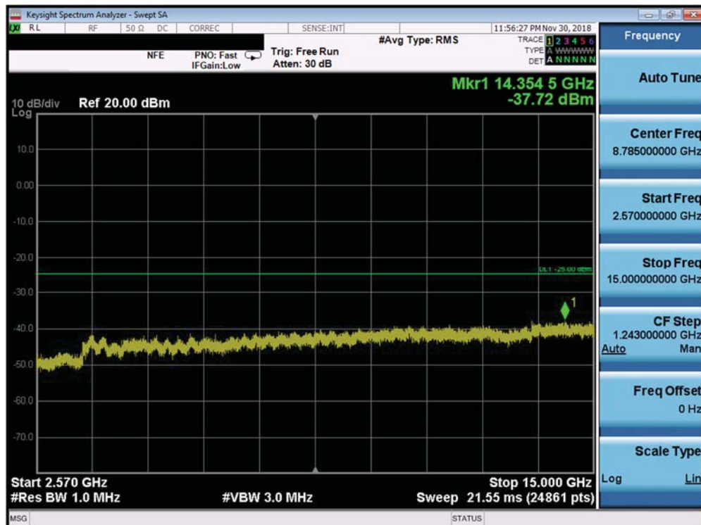
Plot 7-248. Conducted Spurious Plot (Band 7 ANT B - 20.0MHz QPSK - RB Size 1, RB Offset 0 - Low Channel)
