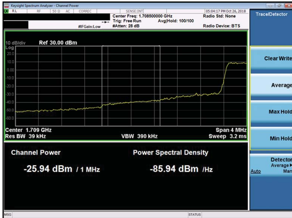
Plot 7-309. Lower Extended Band Edge Plot (Band 66/4 - 1.4MHz QPSK - Full RB Configuration)
