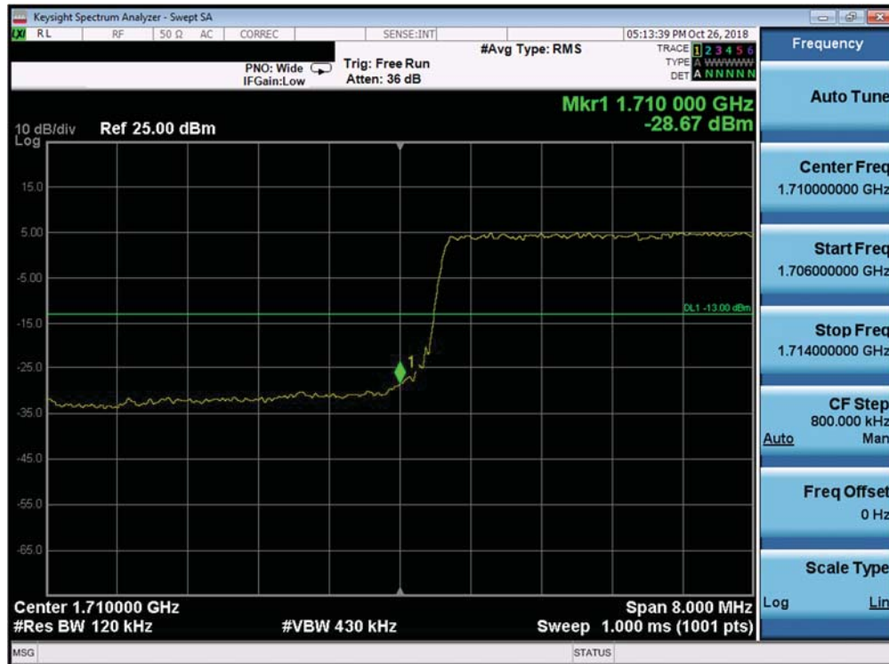
Plot 7-326. Lower Band Edge Plot (Band 66/4 - 10.0MHz QPSK - Full RB Configuration)
