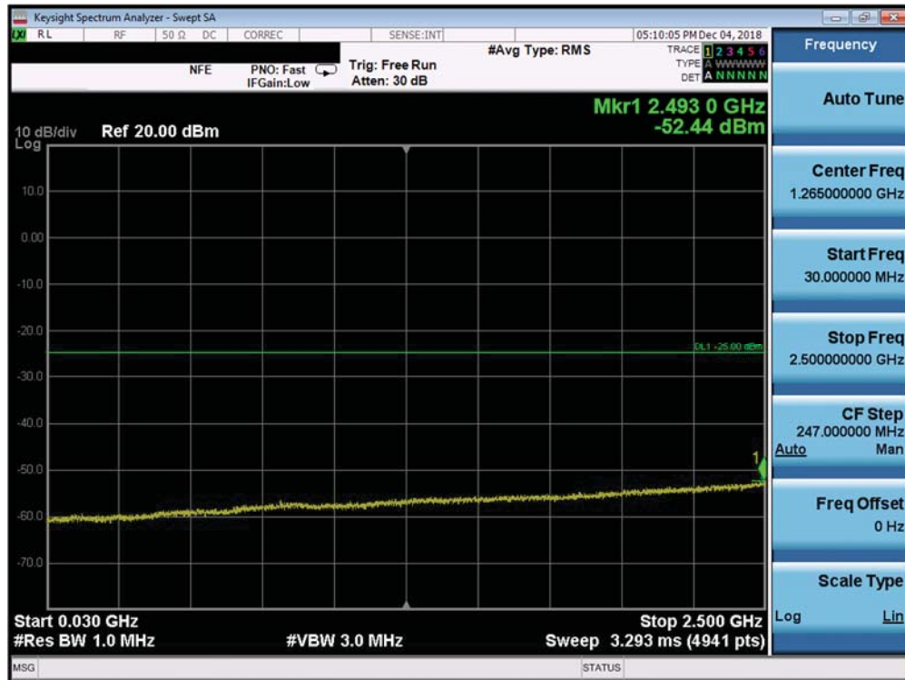
Plot 7-244. Conducted Spurious Plot (Band 7 Ant A - 20.0MHz QPSK - RB Size 1, RB Offset 0 - High Channel)
