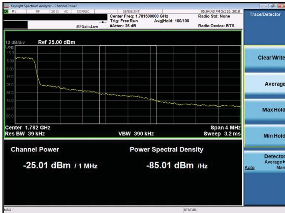
Plot 7-313. Upper Extended Band Edge Plot (Band 66 - 1.4MHz QPSK - Full RB Configuration)
