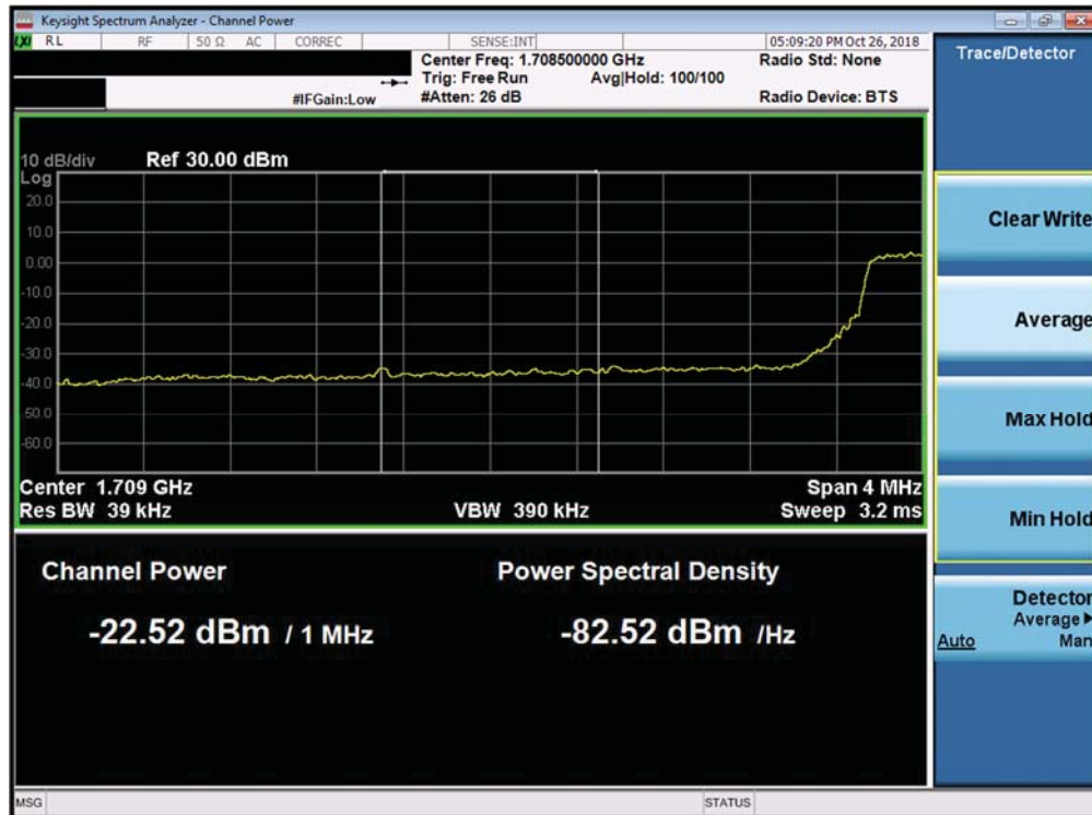
Plot 7-321. Lower Extended Band Edge Plot (Band 66/4 - 5.0MHz QPSK - Full RB Configuration)
