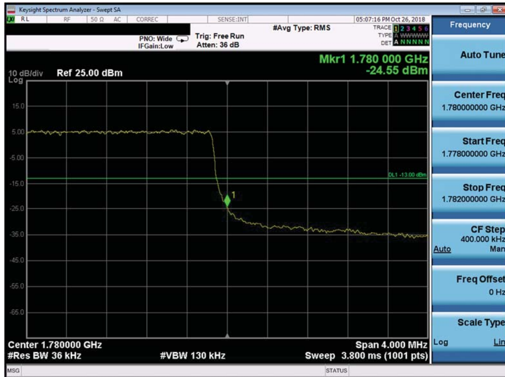
Plot 7-318. Upper Band Edge Plot (Band 66 - 3.0MHz QPSK - Full RB Configuration)
