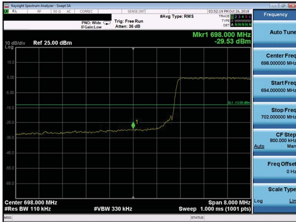
Plot 7-288. Lower Band Edge Plot (Band 12 - 10.0MHz QPSK - Full RB Configuration)
