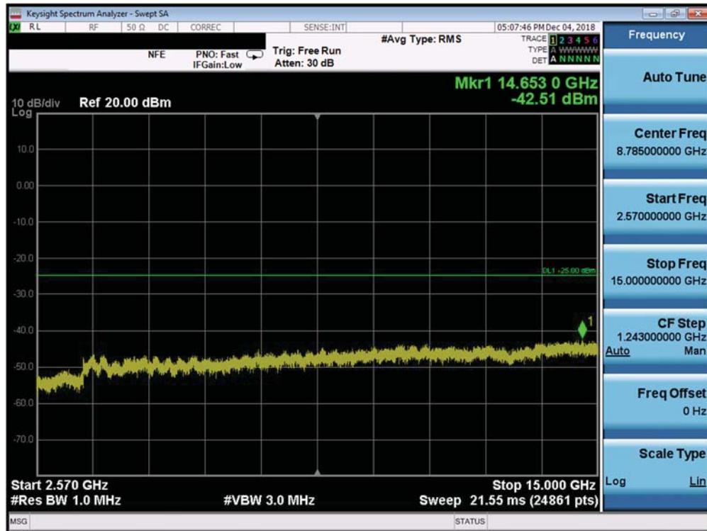
Plot 7-242. Conducted Spurious Plot (Band 7 Ant A - 20.0MHz QPSK - RB Size 1, RB Offset 0 - Mid Channel)
