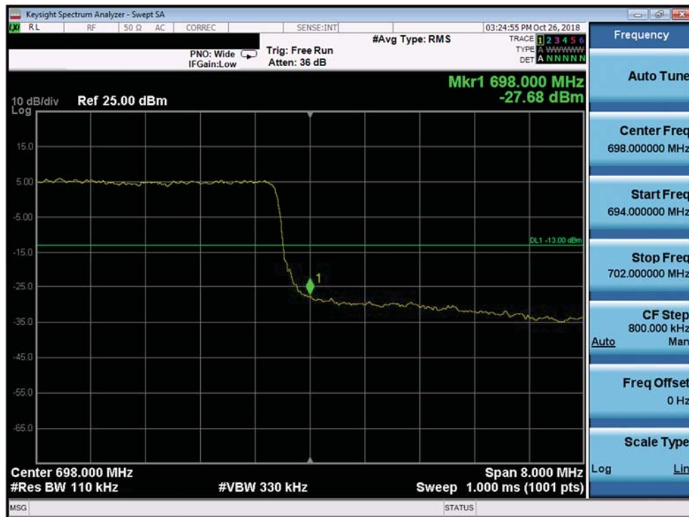
Plot 7-277. Upper Band Edge Plot (Band 71 - 10.0MHz QPSK - Full RB Configuration)
