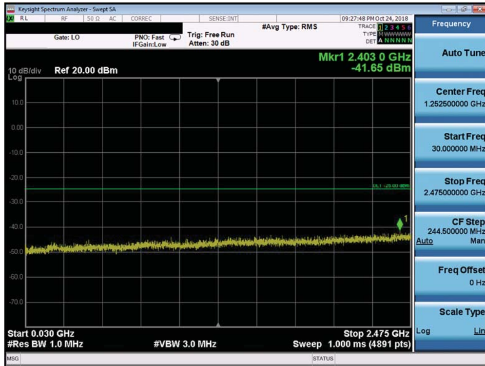
Plot 7-256. Conducted Spurious Plot (Band 41 PC2 - 20.0MHz QPSK - RB Size 1, RB Offset 0 - Low Channel)
