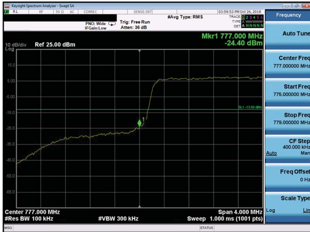
Plot 7-290. Lower Band Edge Plot (Band 13 - 5.0MHz QPSK - Full RB Configuration)
