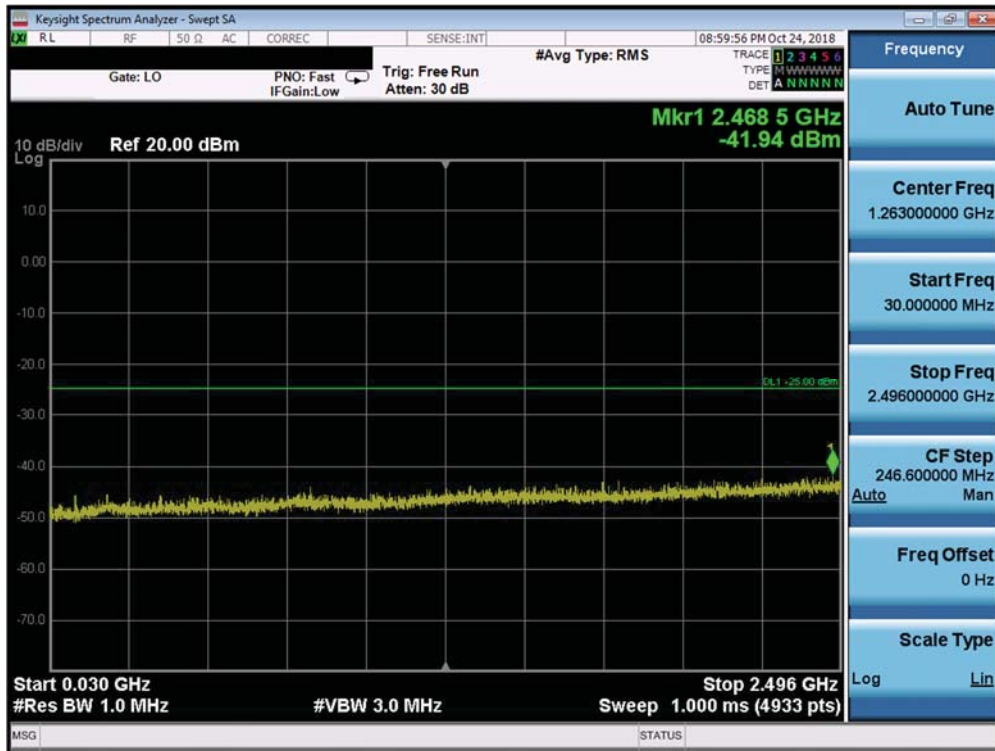
Plot 7-271. Conducted Spurious Plot (Band 41 PC3 / Band 38 - 20.0MHz QPSK - RB Size 1, RB Offset 0 - High Channel)
