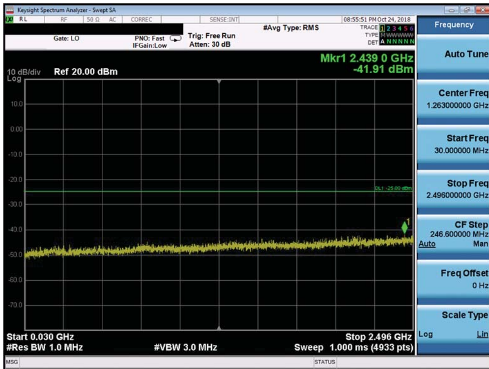
Plot 7-268. Conducted Spurious Plot (Band 41 PC3 / Band 38 - 20.0MHz QPSK - RB Size 1, RB Offset 0 - Mid Channel)
