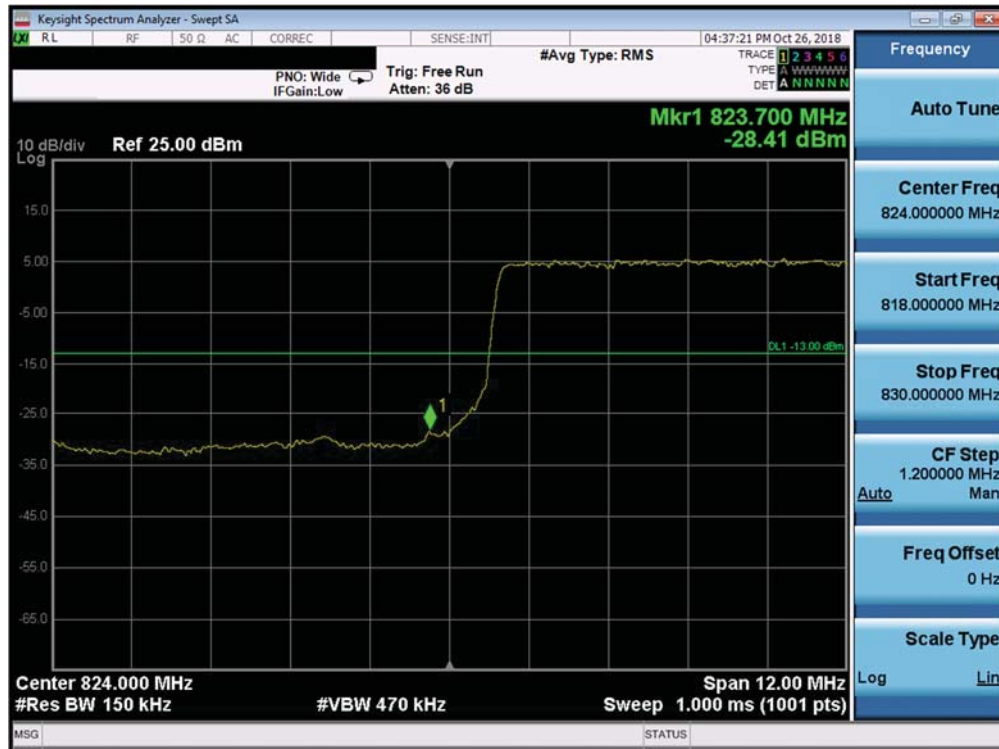
Plot 7-306. Lower Band Edge Plot (Band 26 - 15.0MHz QPSK - Full RB Configuration)
