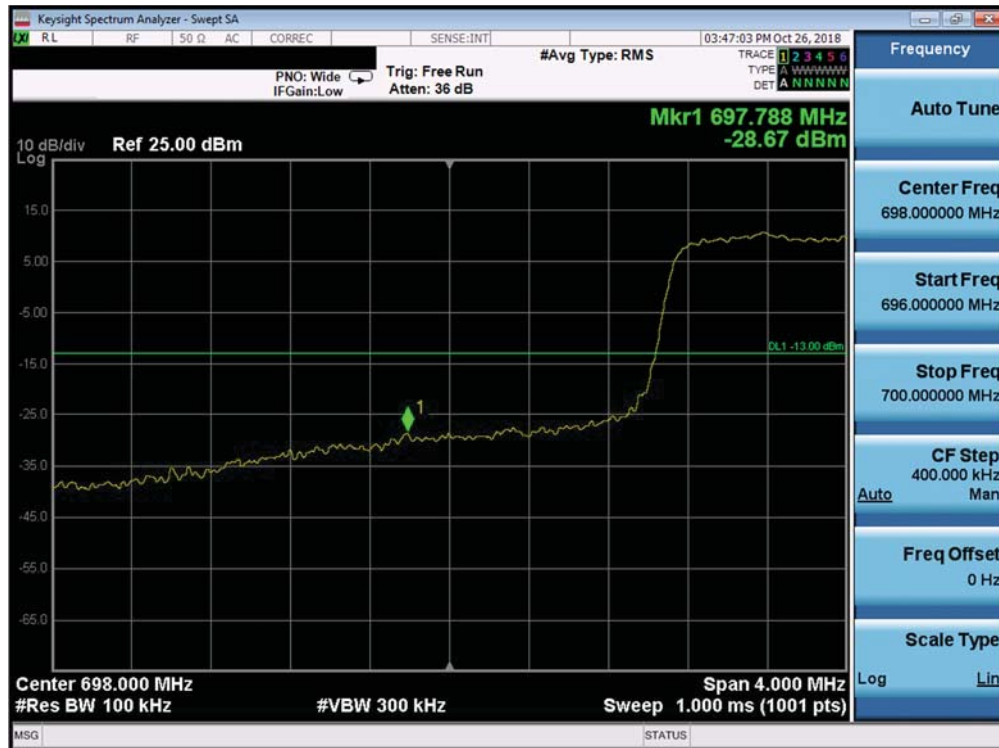
Plot 7-284. Lower Band Edge Plot (Band 12 - 3.0MHz QPSK - Full RB Configuration)
