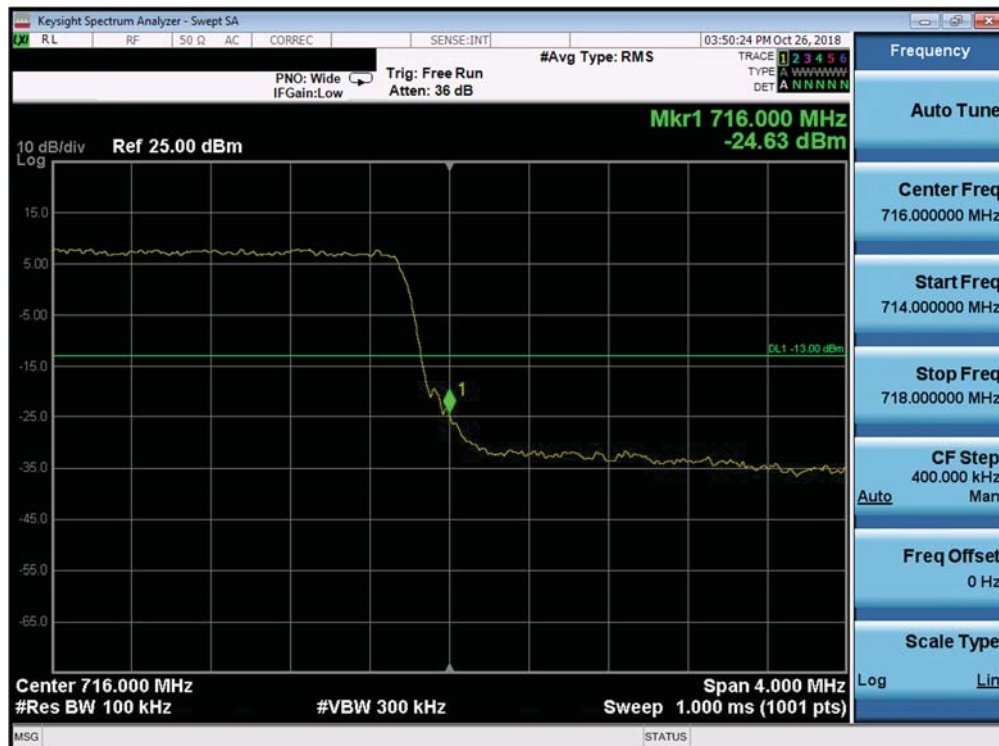
Plot 7-287. Upper Band Edge Plot (Band 12 - 5.0MHz QPSK - Full RB Configuration)
