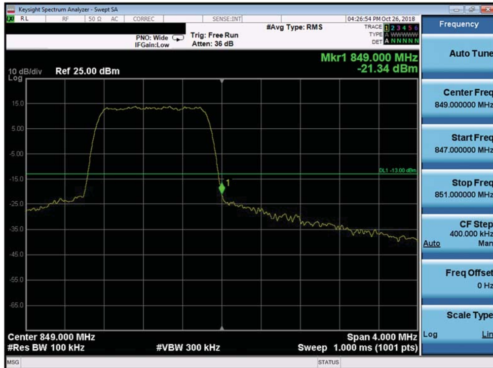
Plot 7-299. Upper Band Edge Plot (Band 26/5 - 1.4MHz QPSK - Full RB Configuration)
