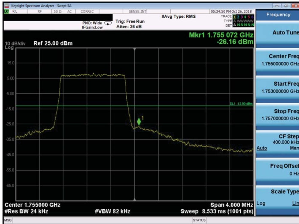
Plot 7-310. Upper Band Edge Plot (Band 4 - 1.4MHz QPSK - Full RB Configuration)
