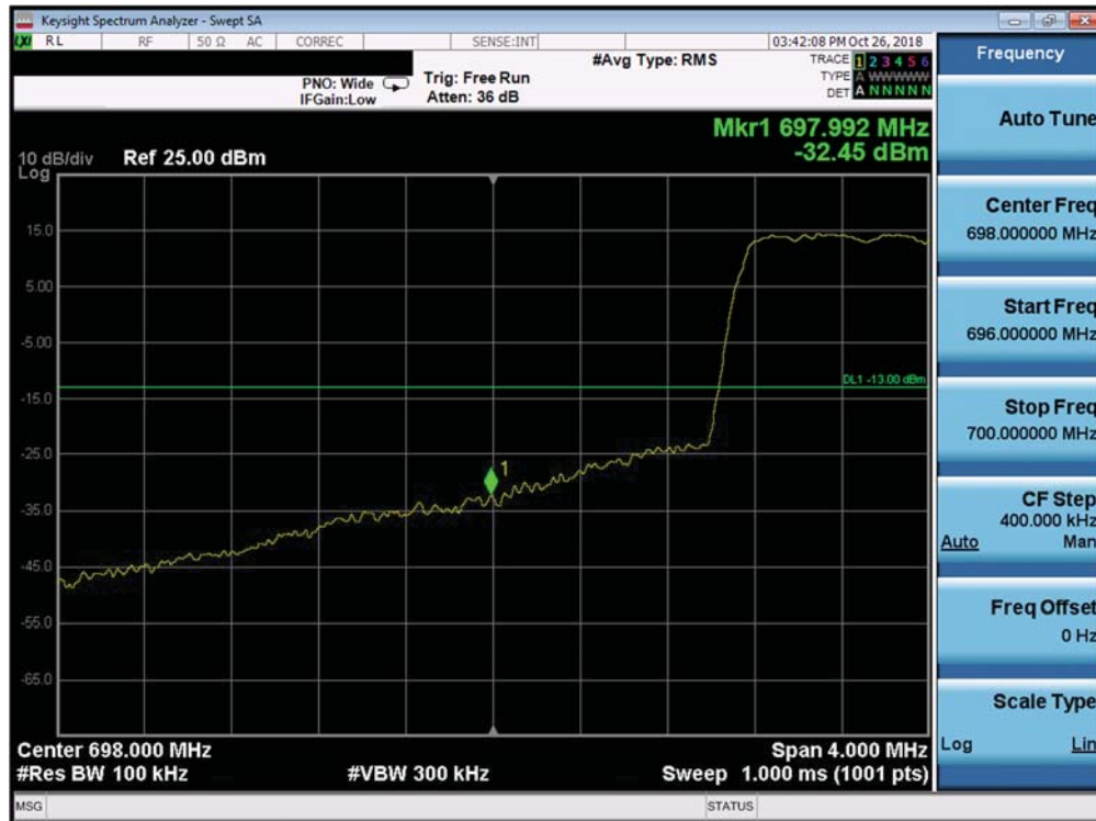
Plot 7-282. Lower Band Edge Plot (Band 12 - 1.4MHz QPSK - Full RB Configuration)
