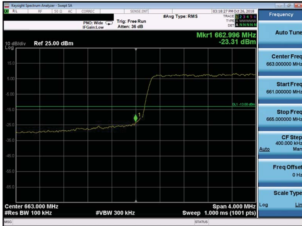
Plot 7-274. Lower Band Edge Plot (Band 71 - 5.0MHz QPSK - Full RB Configuration)
