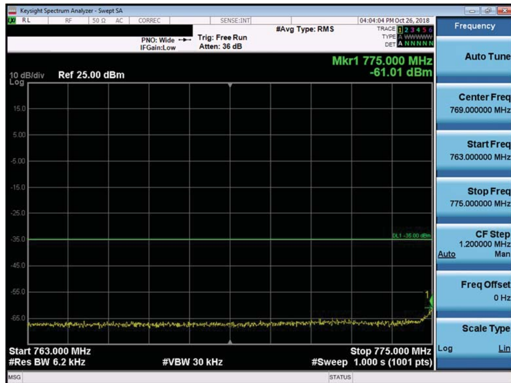
Plot 7-295. Lower Emission Mask Plot (Band 13 - 10.0MHz QPSK - Full RB Configuration)
