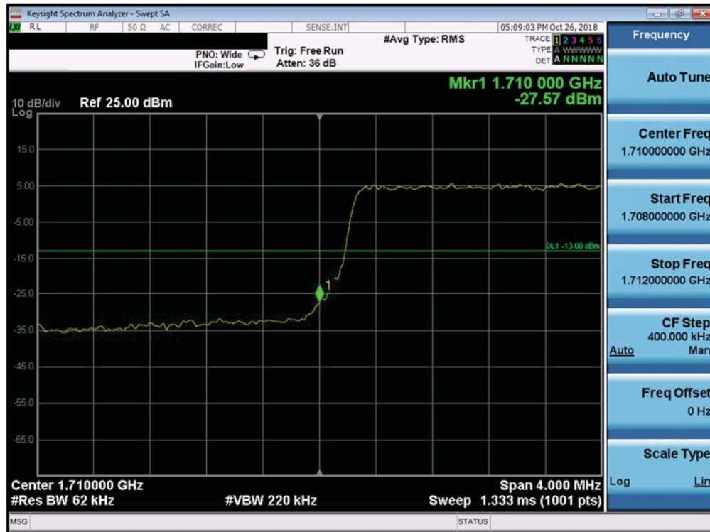
Plot 7-320. Lower Band Edge Plot (Band 66/4 - 5.0MHz QPSK - Full RB Configuration)
