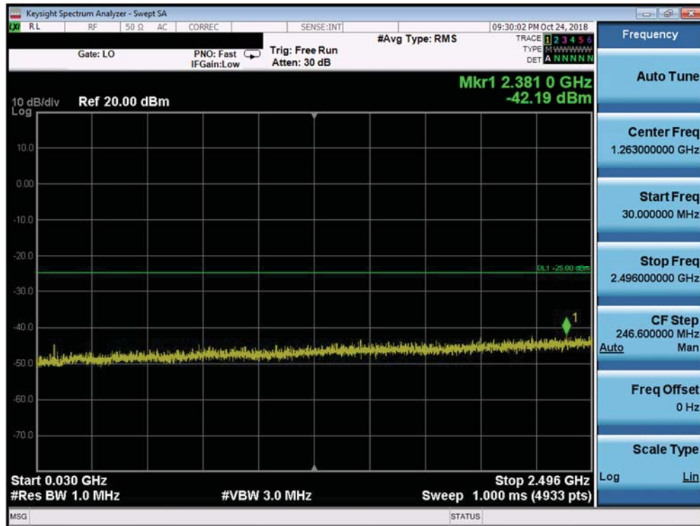
Plot 7-262. Conducted Spurious Plot (Band 41 PC2 - 20.0MHz QPSK - RB Size 1, RB Offset 0 - High Channel)
