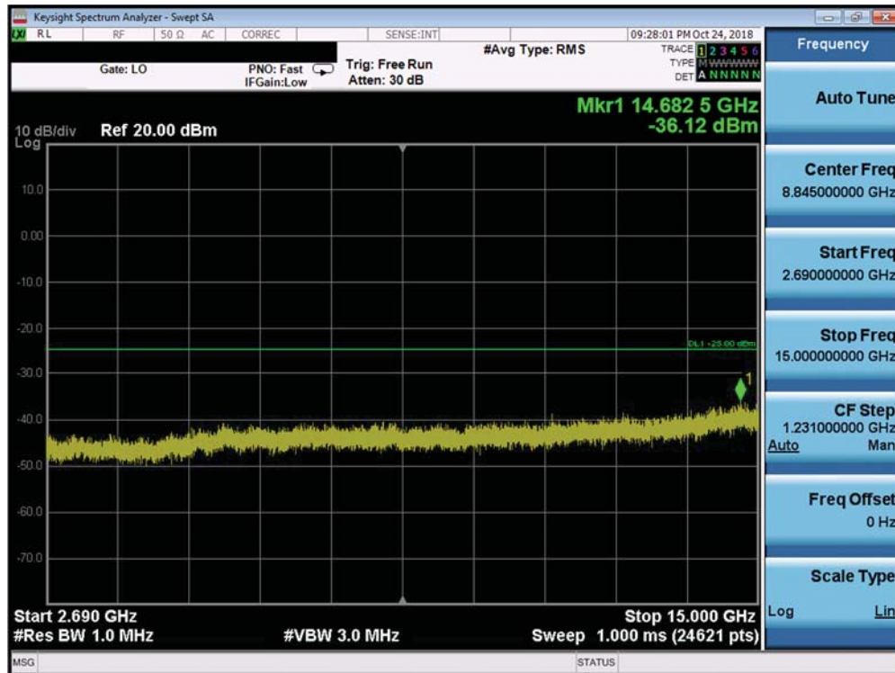
Plot 7-257. Conducted Spurious Plot (Band 41 PC2 - 20.0MHz QPSK - RB Size 1, RB Offset 0 - Low Channel)
