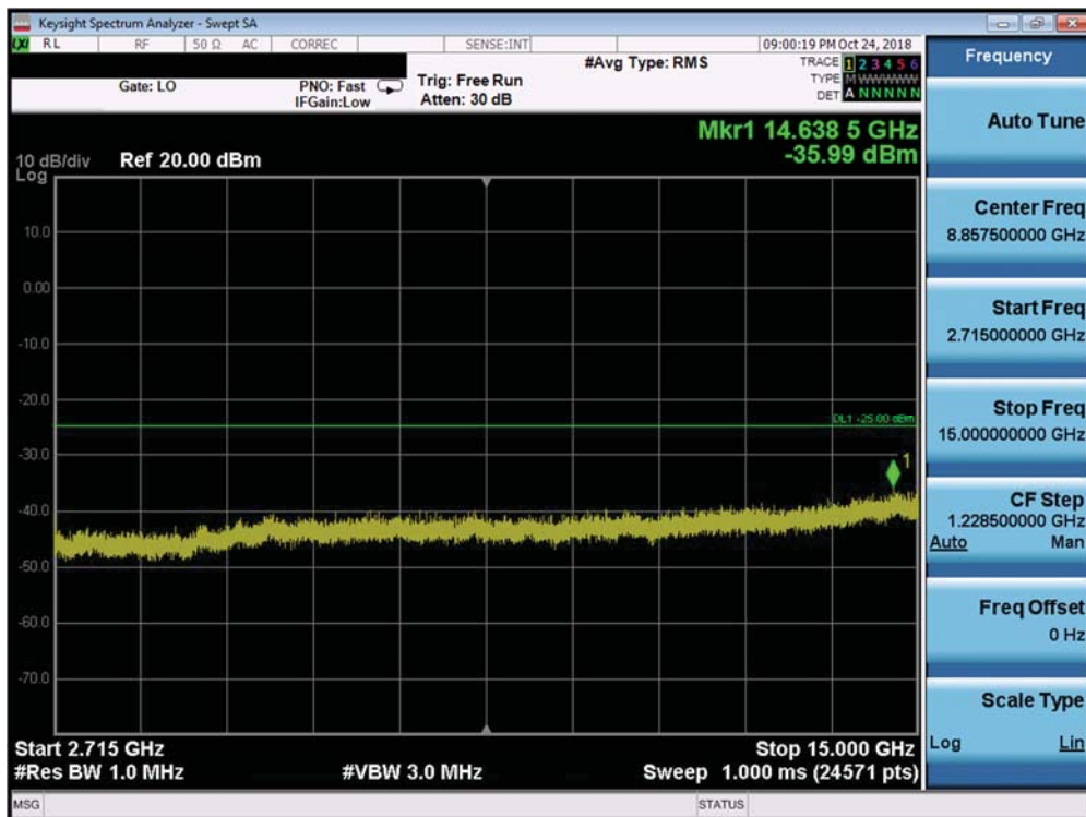
Plot 7-272. Conducted Spurious Plot (Band 41 PC3 / Band 38 - 20.0MHz QPSK - RB Size 1, RB Offset 0 - High Channel)
