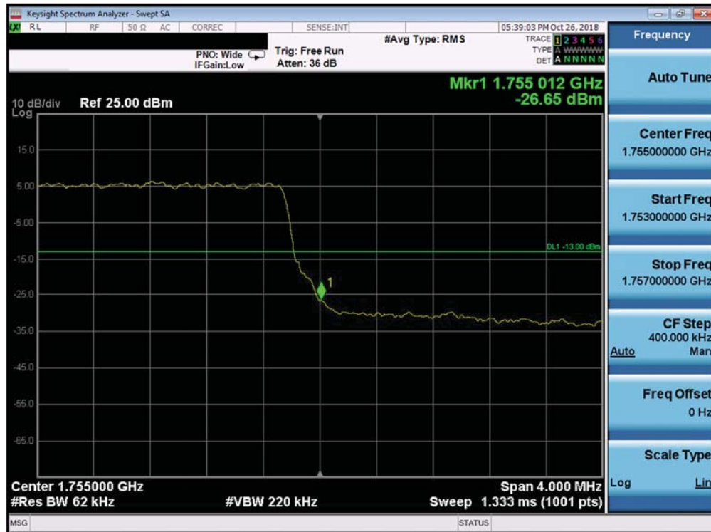
Plot 7-322. Upper Band Edge Plot (Band 4 - 5.0MHz QPSK - Full RB Configuration)
