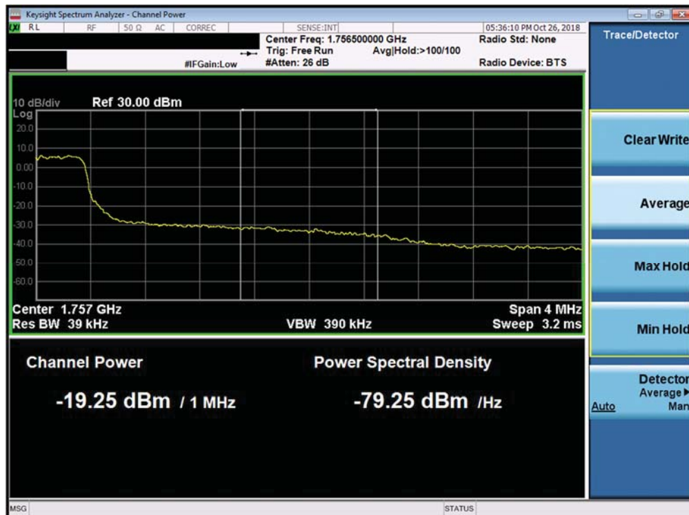
Plot 7-317. Upper Extended Band Edge Plot (Band 4 - 3.0MHz QPSK - Full RB Configuration)
