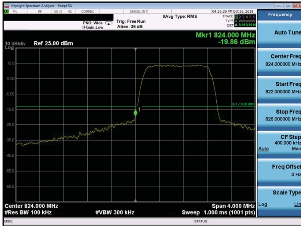
Plot 7-298. Lower Band Edge Plot (Band 26/5 - 1.4MHz QPSK - Full RB Configuration)
