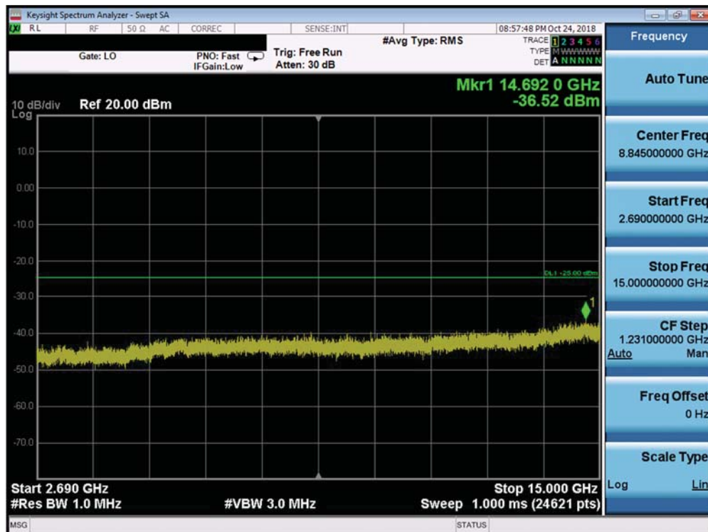
Plot 7-266. Conducted Spurious Plot (Band 41 PC3 / Band 38 - 20.0MHz QPSK - RB Size 1, RB Offset 0 - Low Channel)
