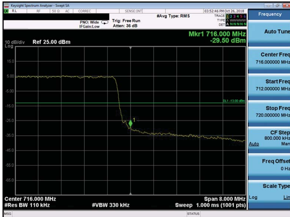
Plot 7-289. Upper Band Edge Plot (Band 12 - 10.0MHz QPSK - Full RB Configuration)
