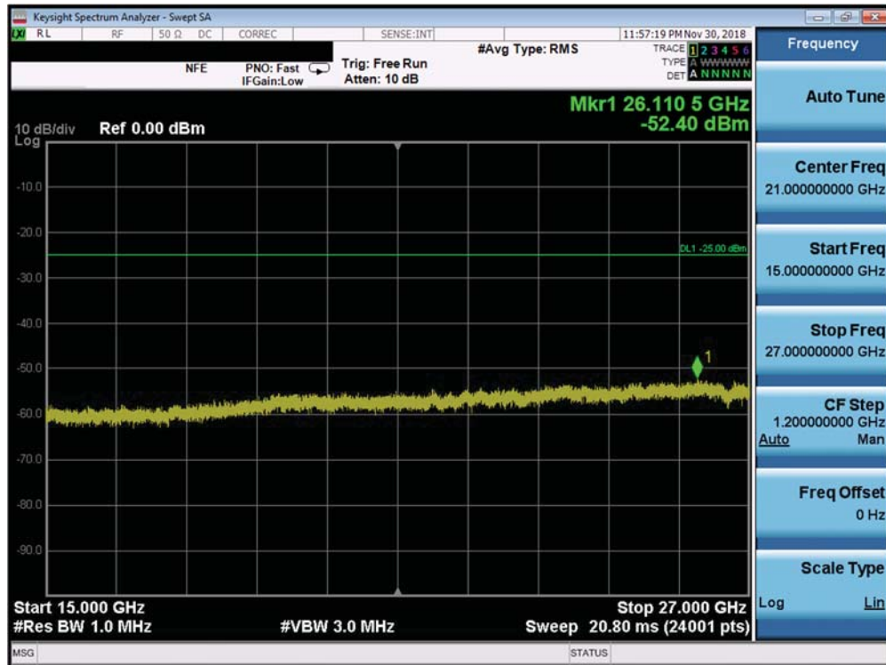
Plot 7-255. Conducted Spurious Plot (Band 7 ANT B - 20.0MHz QPSK - RB Size 1, RB Offset 0 - High Channel)
