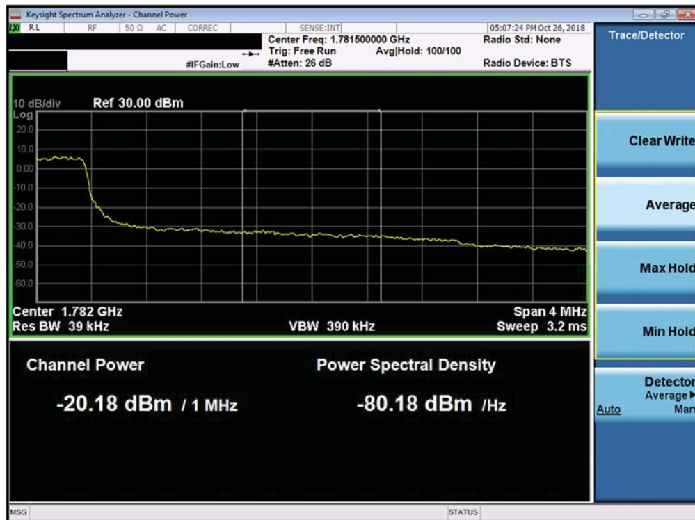
Plot 7-319. Upper Extended Band Edge Plot (Band 66 - 3.0MHz QPSK - Full RB Configuration)
