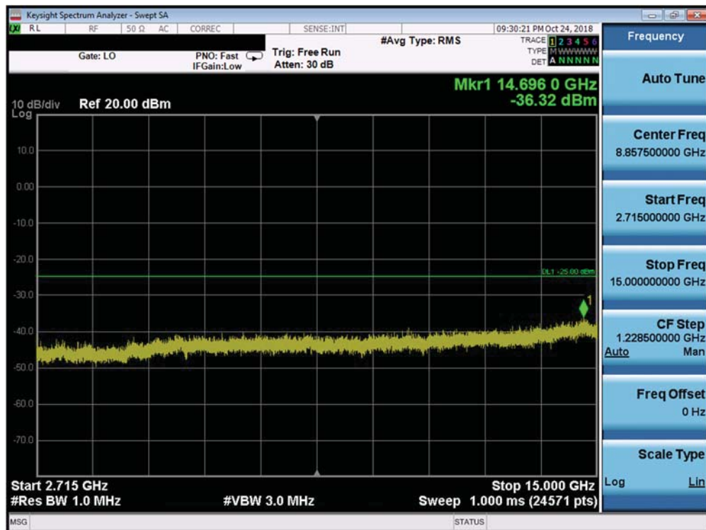
Plot 7-263. Conducted Spurious Plot (Band 41 PC2 - 20.0MHz QPSK - RB Size 1, RB Offset 0 - High Channel)
