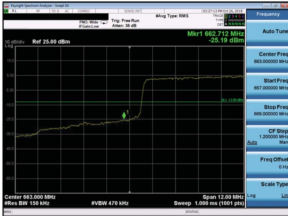
Plot 7-278. Lower Band Edge Plot (Band 71 - 15.0MHz QPSK - Full RB Configuration)
