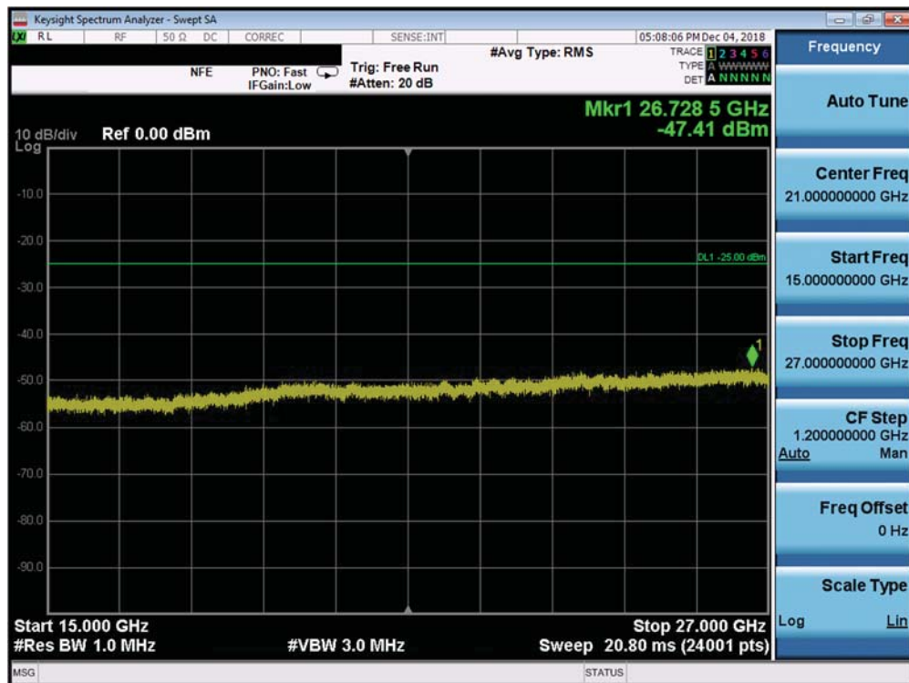
Plot 7-243. Conducted Spurious Plot (Band 7 Ant A - 20.0MHz QPSK - RB Size 1, RB Offset 0 - Mid Channel)
