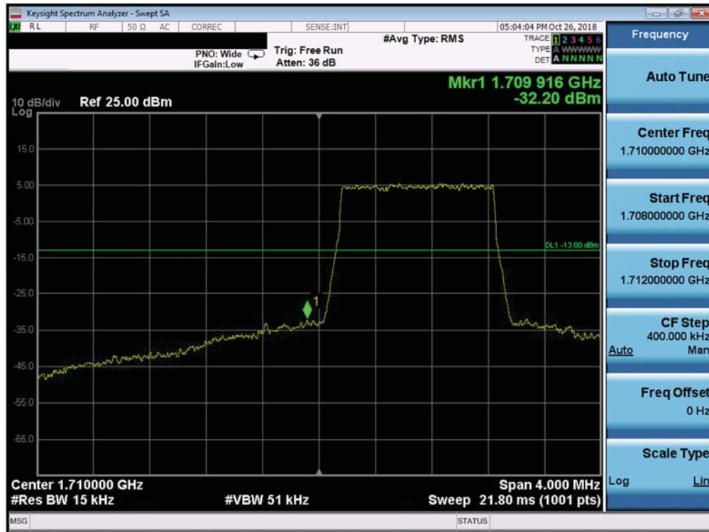
Plot 7-308. Lower Band Edge Plot (Band 66/4 - 1.4MHz QPSK - Full RB Configuration)
