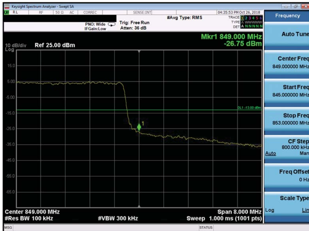
Plot 7-305. Upper Band Edge Plot (Band 26/5 - 10.0MHz QPSK - Full RB Configuration)
