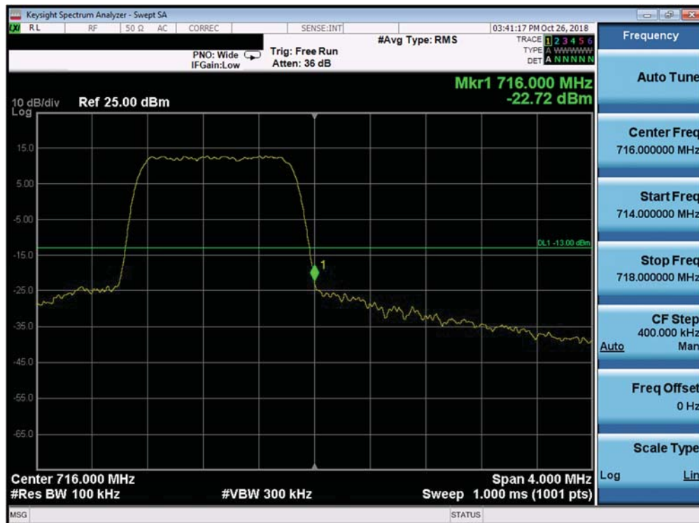
Plot 7-283. Upper Band Edge Plot (Band 12 - 1.4MHz QPSK - Full RB Configuration)
