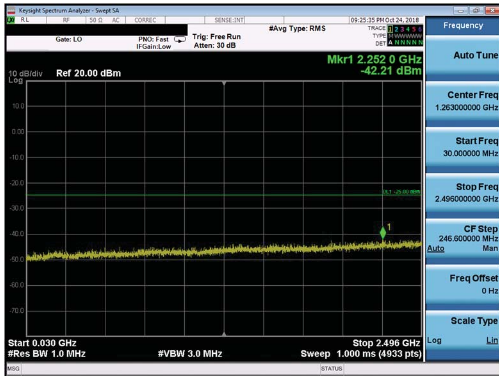
Plot 7-259. Conducted Spurious Plot (Band 41 PC2 - 20.0MHz QPSK - RB Size 1, RB Offset 0 - Mid Channel)
