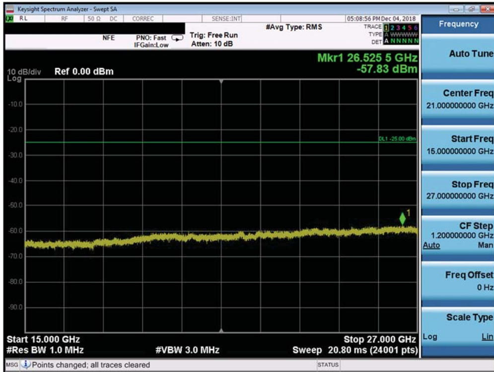
Plot 7-240. Conducted Spurious Plot (Band 7 Ant A - 20.0MHz QPSK - RB Size 1, RB Offset 0 - Low Channel)
