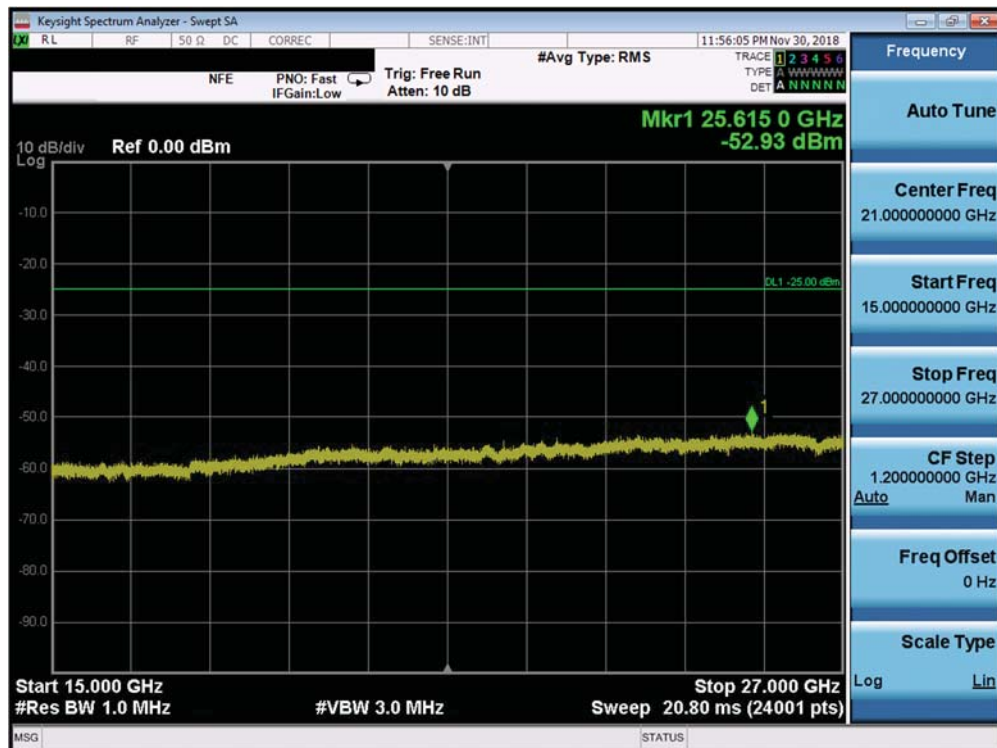
Plot 7-252. Conducted Spurious Plot (Band 7 ANT B - 20.0MHz QPSK - RB Size 1, RB Offset 0 - Mid Channel)
