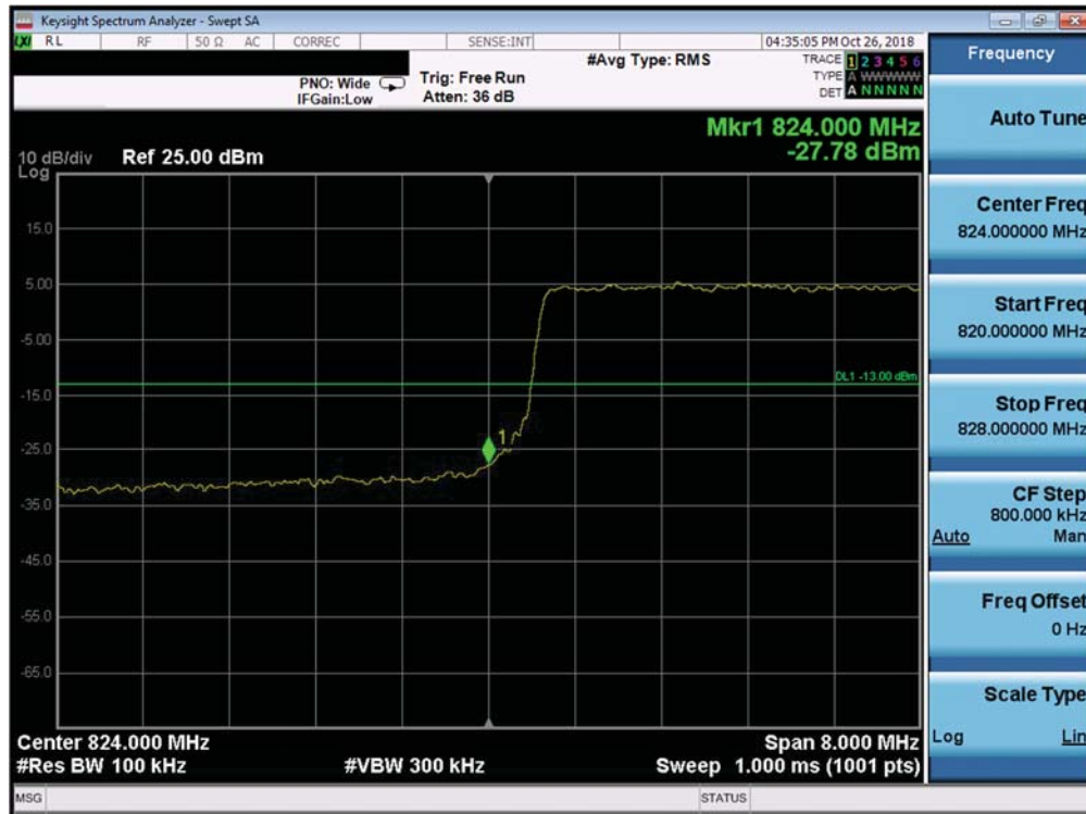
Plot 7-304. Lower Band Edge Plot (Band 26/5 - 10.0MHz QPSK - Full RB Configuration)
