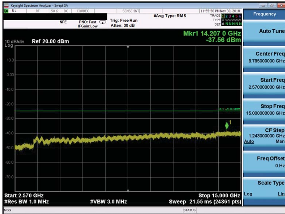
Plot 7-251. Conducted Spurious Plot (Band 7 ANT B - 20.0MHz QPSK - RB Size 1, RB Offset 0 - Mid Channel)
