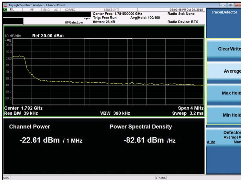
Plot 7-325. Upper Extended Band Edge Plot (Band 66 - 5.0MHz QPSK - Full RB Configuration)
