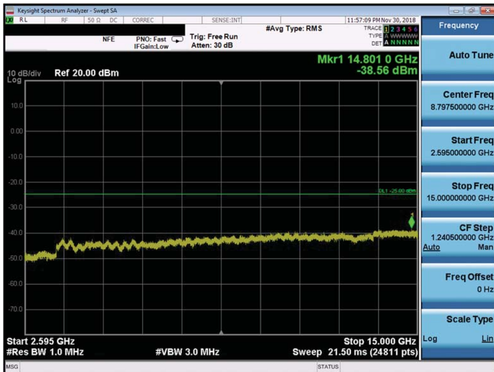
Plot 7-254. Conducted Spurious Plot (Band 7 ANT B - 20.0MHz QPSK - RB Size 1, RB Offset 0 - High Channel)
