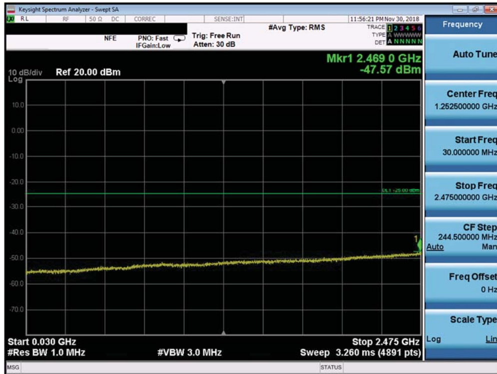
Plot 7-247. Conducted Spurious Plot (Band 7 ANT B - 20.0MHz QPSK - RB Size 1, RB Offset 0 - Low Channel)
