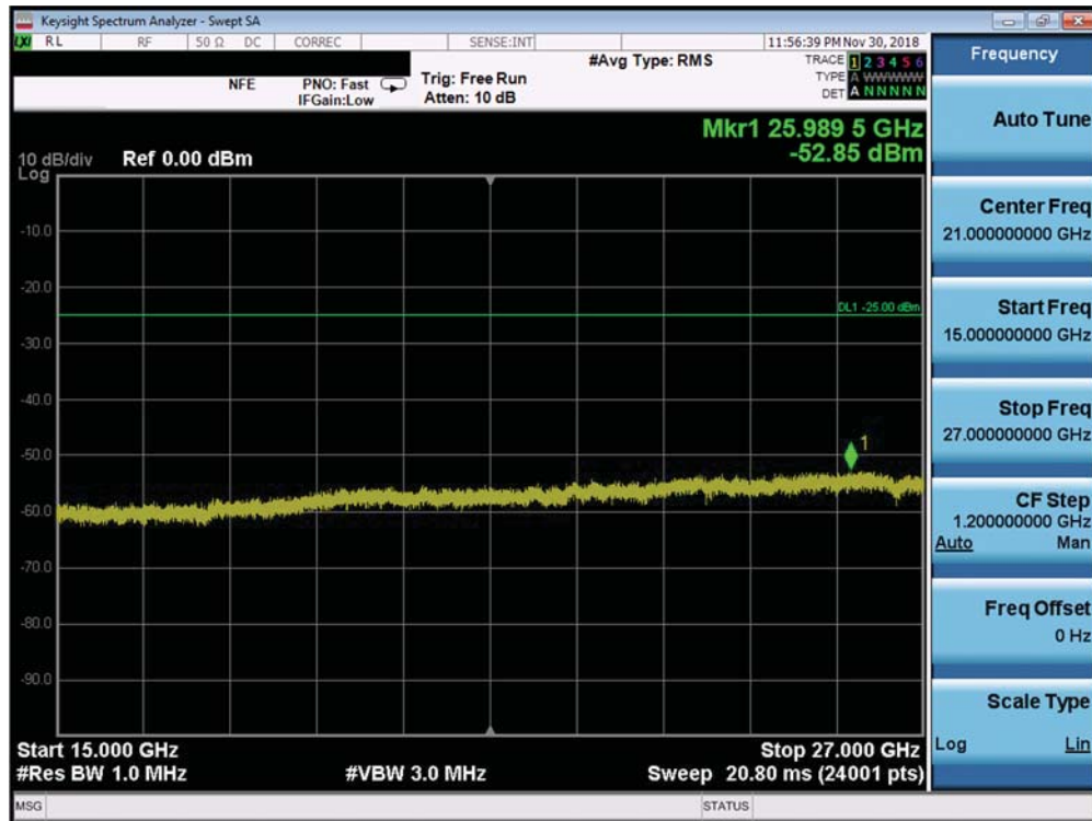
Plot 7-249. Conducted Spurious Plot (Band 7 ANT B - 20.0MHz QPSK - RB Size 1, RB Offset 0 - Low Channel)
