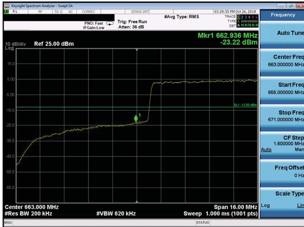
Plot 7-280. Lower Band Edge Plot (Band 71 - 20.0MHz QPSK - Full RB Configuration)
