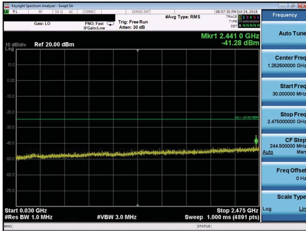
Plot 7-265. Conducted Spurious Plot (Band 41 PC3 / Band 38 - 20.0MHz QPSK - RB Size 1, RB Offset 0 - Low Channel)
