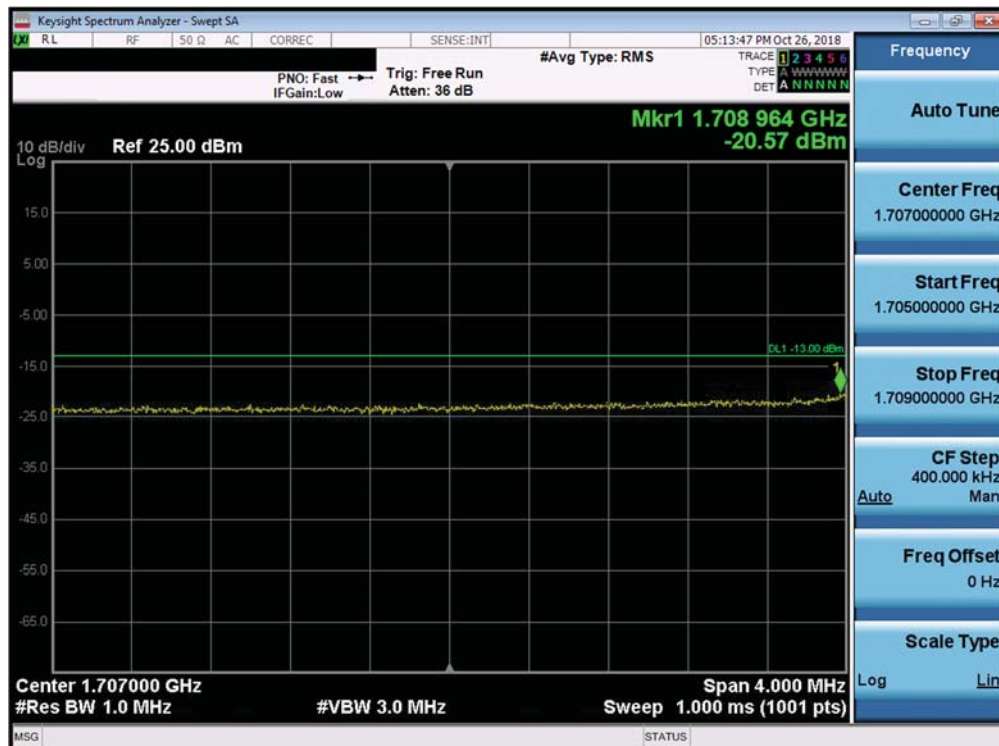
Plot 7-327. Lower Extended Band Edge Plot (Band 66/4 - 10.0MHz QPSK - Full RB Configuration)
