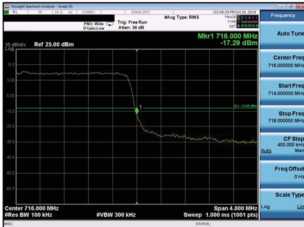
Plot 7-285. Upper Band Edge Plot (Band 12 - 3.0MHz QPSK - Full RB Configuration)
