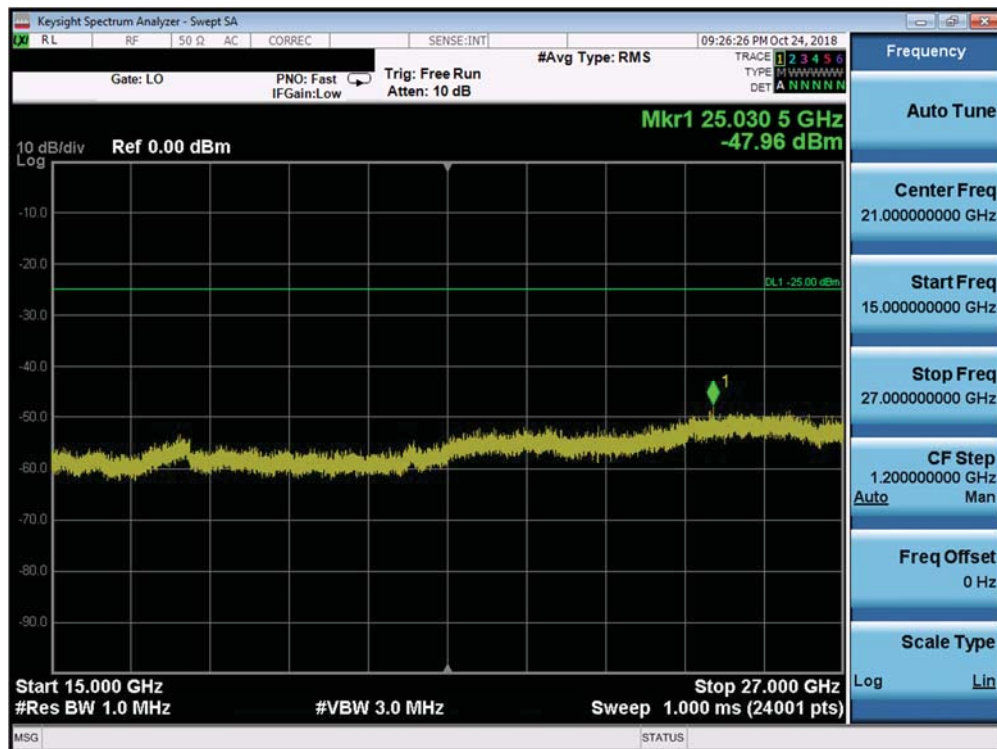
Plot 7-261. Conducted Spurious Plot (Band 41 PC2 - 20.0MHz QPSK - RB Size 1, RB Offset 0 - Mid Channel)
