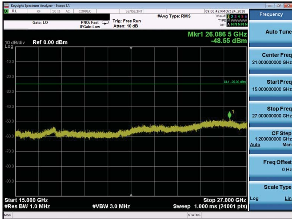
Plot 7-273. Conducted Spurious Plot (Band 41 PC3 / Band 38 - 20.0MHz QPSK - RB Size 1, RB Offset 0 - High Channel)
