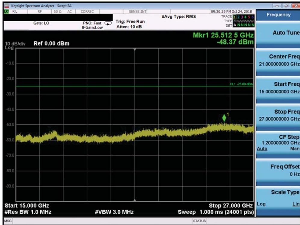
Plot 7-264. Conducted Spurious Plot (Band 41 PC2 - 20.0MHz QPSK - RB Size 1, RB Offset 0 - High Channel)
