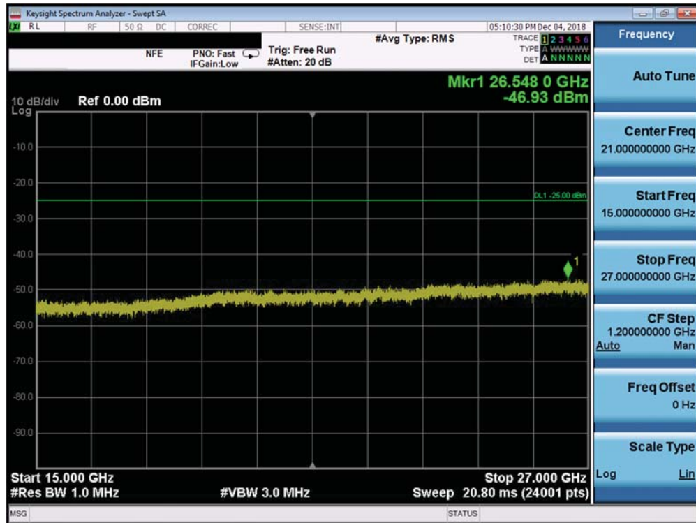
Plot 7-246. Conducted Spurious Plot (Band 7 Ant A - 20.0MHz QPSK - RB Size 1, RB Offset 0 - High Channel)
