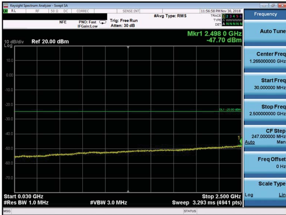
Plot 7-253. Conducted Spurious Plot (Band 7 ANT B - 20.0MHz QPSK - RB Size 1, RB Offset 0 - High Channel)
