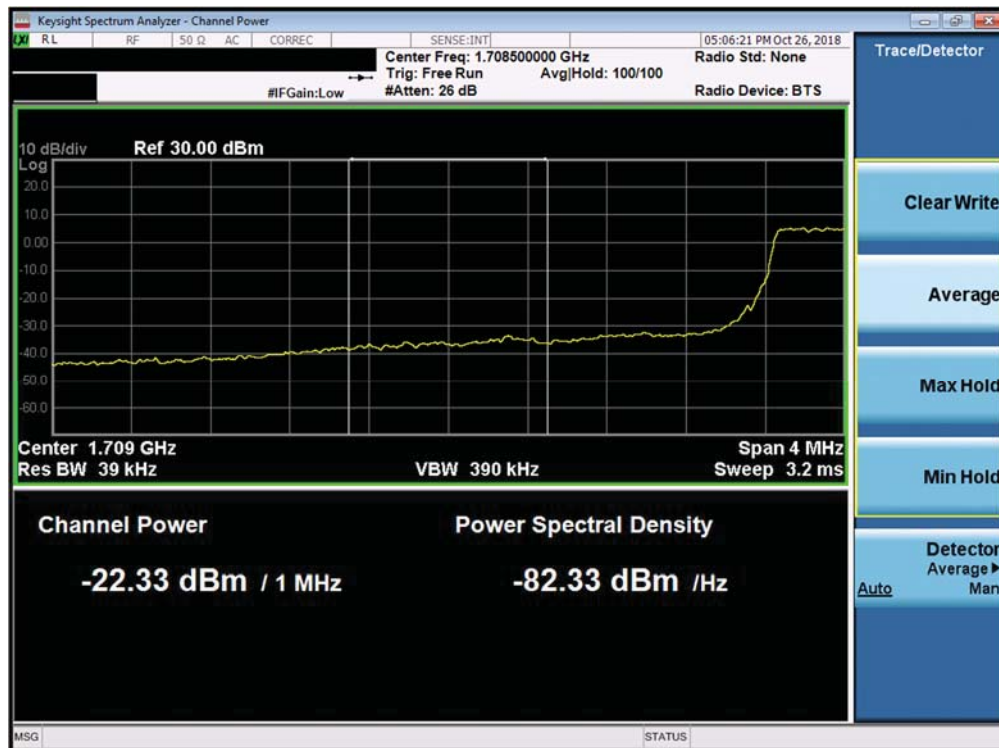
Plot 7-315. Lower Extended Band Edge Plot (Band 66/4 - 3.0MHz QPSK - Full RB Configuration)
