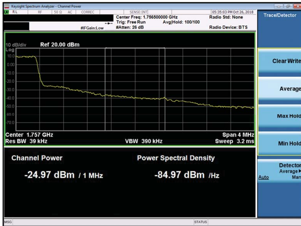
Plot 7-311. Upper Extended Band Edge Plot (Band 4 - 1.4MHz QPSK - Full RB Configuration)
