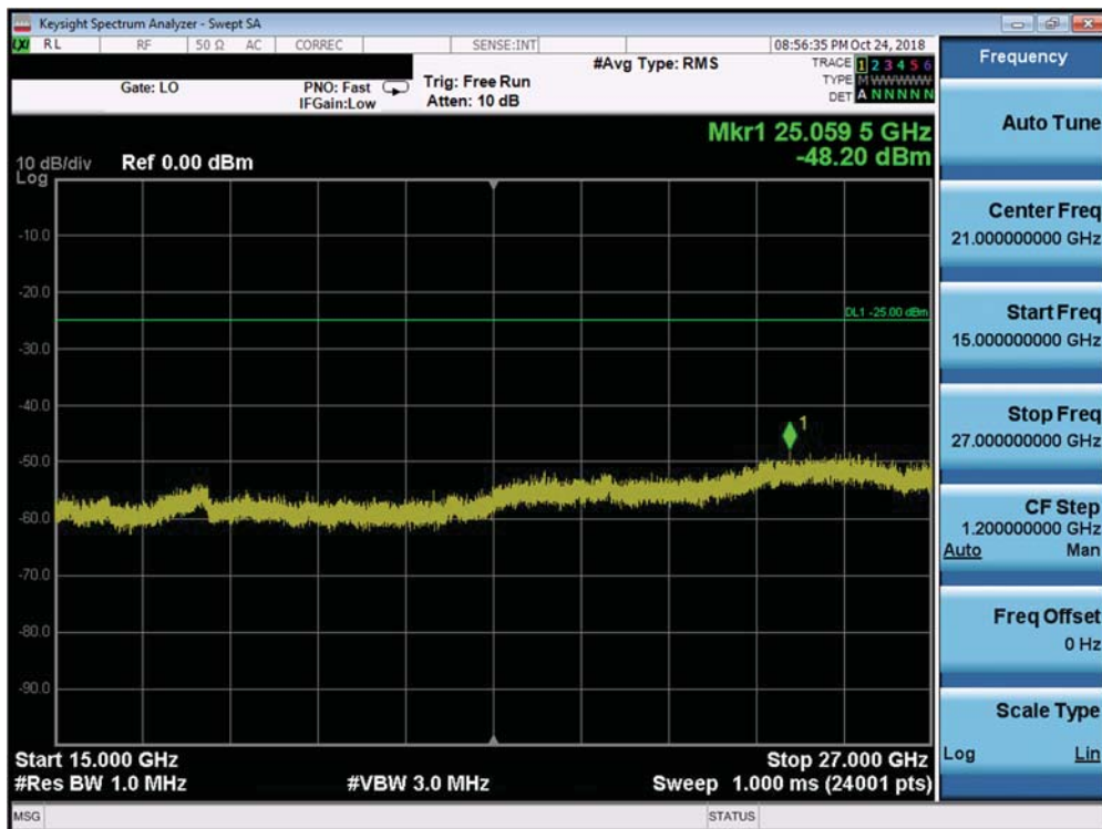
Plot 7-270. Conducted Spurious Plot (Band 41 PC3 / Band 38 - 20.0MHz QPSK - RB Size 1, RB Offset 0 - Mid Channel)
