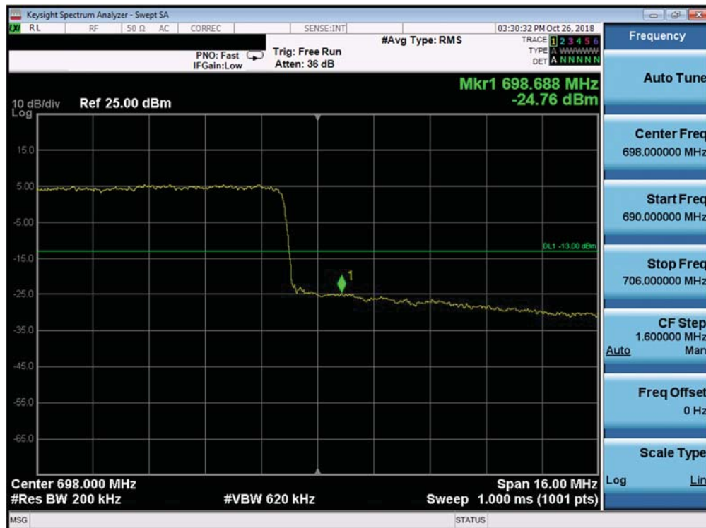
Plot 7-281. Upper Band Edge Plot (Band 71 - 20.0MHz QPSK - Full RB Configuration)
