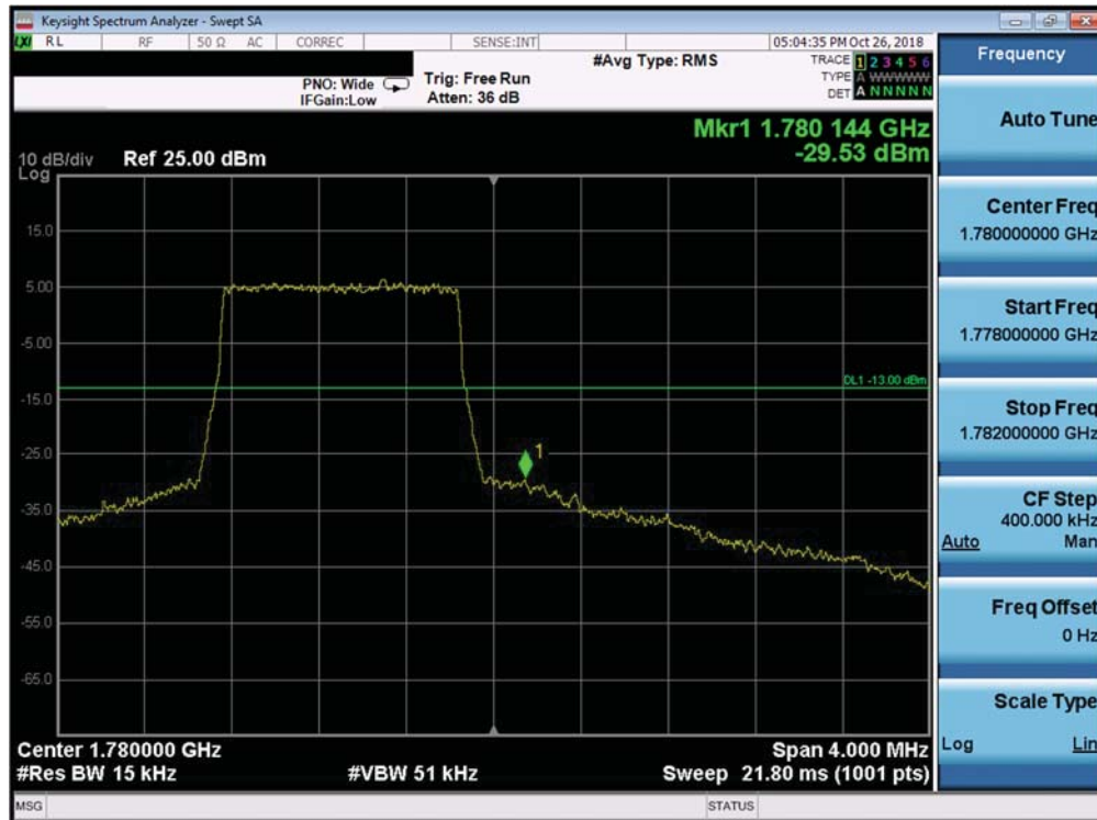
Plot 7-312. Upper Band Edge Plot (Band 66 - 1.4MHz QPSK - Full RB Configuration)
