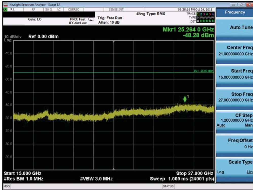
Plot 7-258. Conducted Spurious Plot (Band 41 PC2 - 20.0MHz QPSK - RB Size 1, RB Offset 0 - Low Channel)
