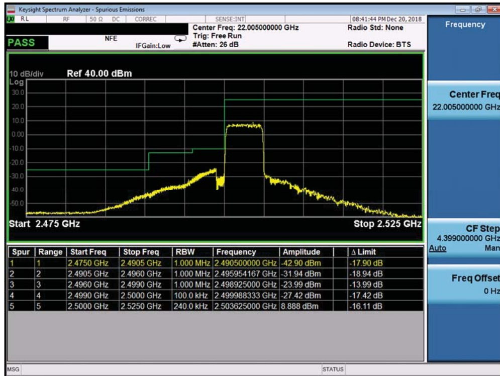
Plot 7-388. Lower ACP Plot (Band 7 ANT B - 5.0MHz QPSK - Full RB Configuration)
