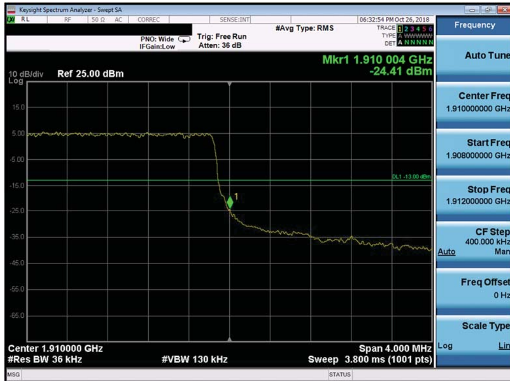
Plot 7-352. Upper Band Edge Plot (Band 2 - 3.0MHz QPSK - Full RB Configuration)
