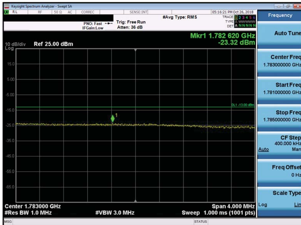
Plot 7-337. Upper Extended Band Edge Plot (Band 66 - 15.0MHz QPSK - Full RB Configuration)
