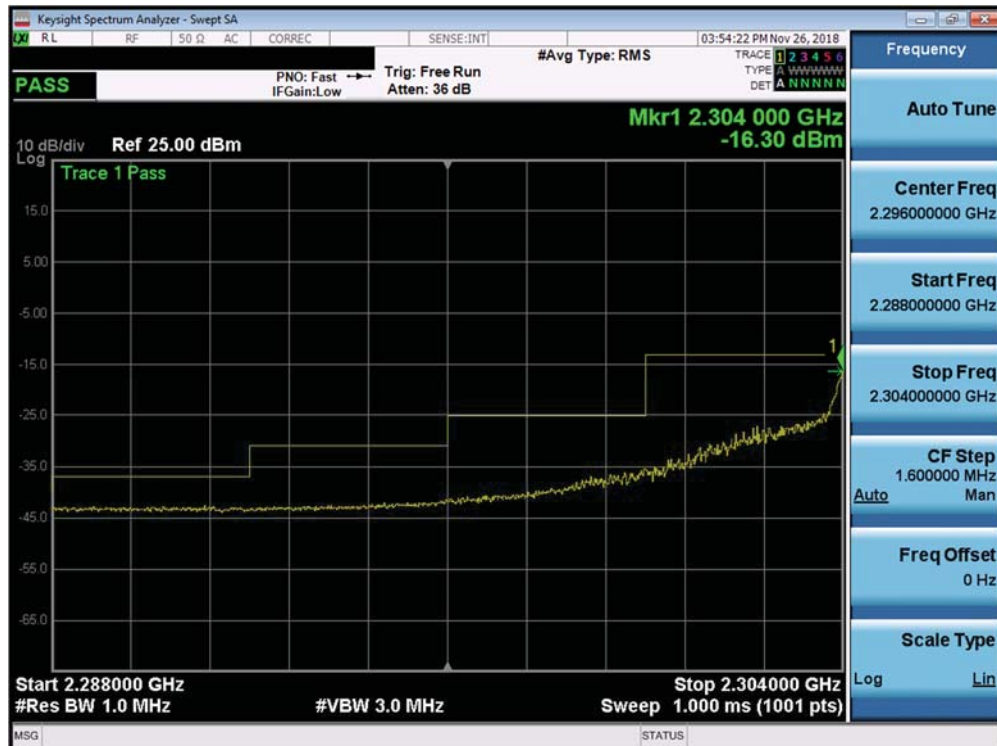
Plot 7-381. Lower Extended Band Edge Plot (Band 30 - 5.0MHz QPSK - Full RB Configuration)
