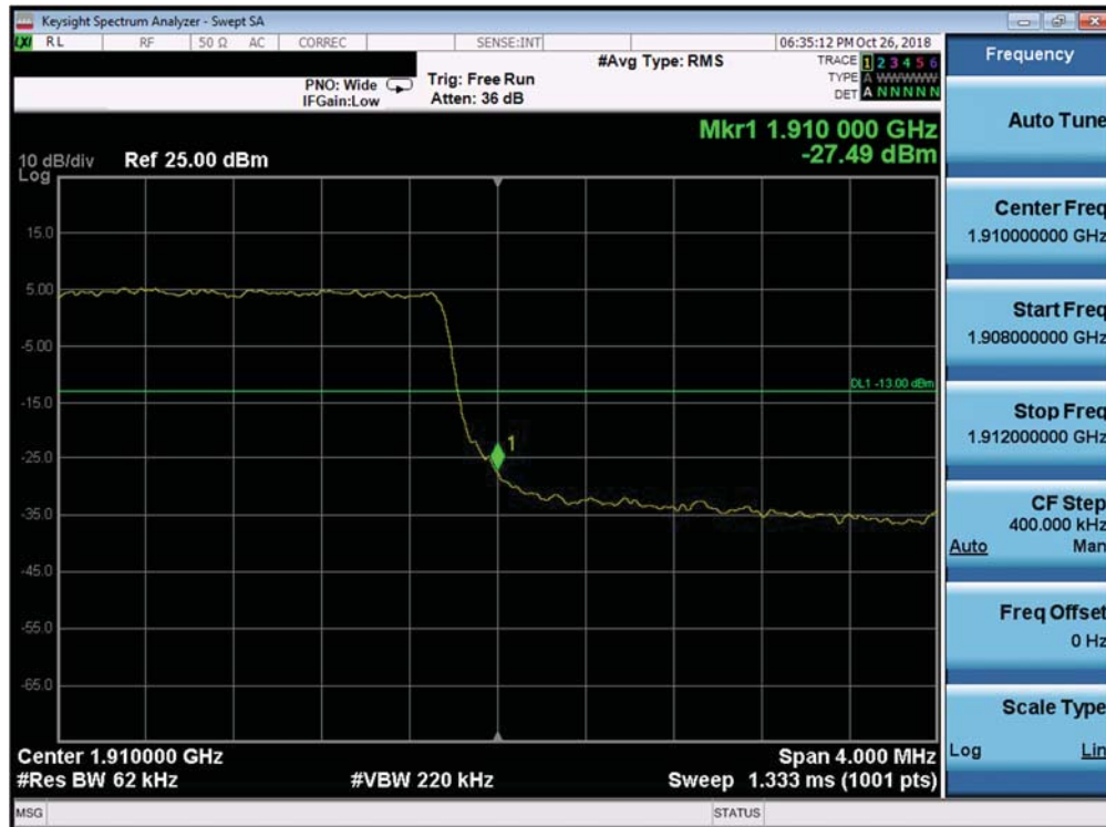
Plot 7-358. Upper Band Edge Plot (Band 2 - 5.0MHz QPSK - Full RB Configuration)
