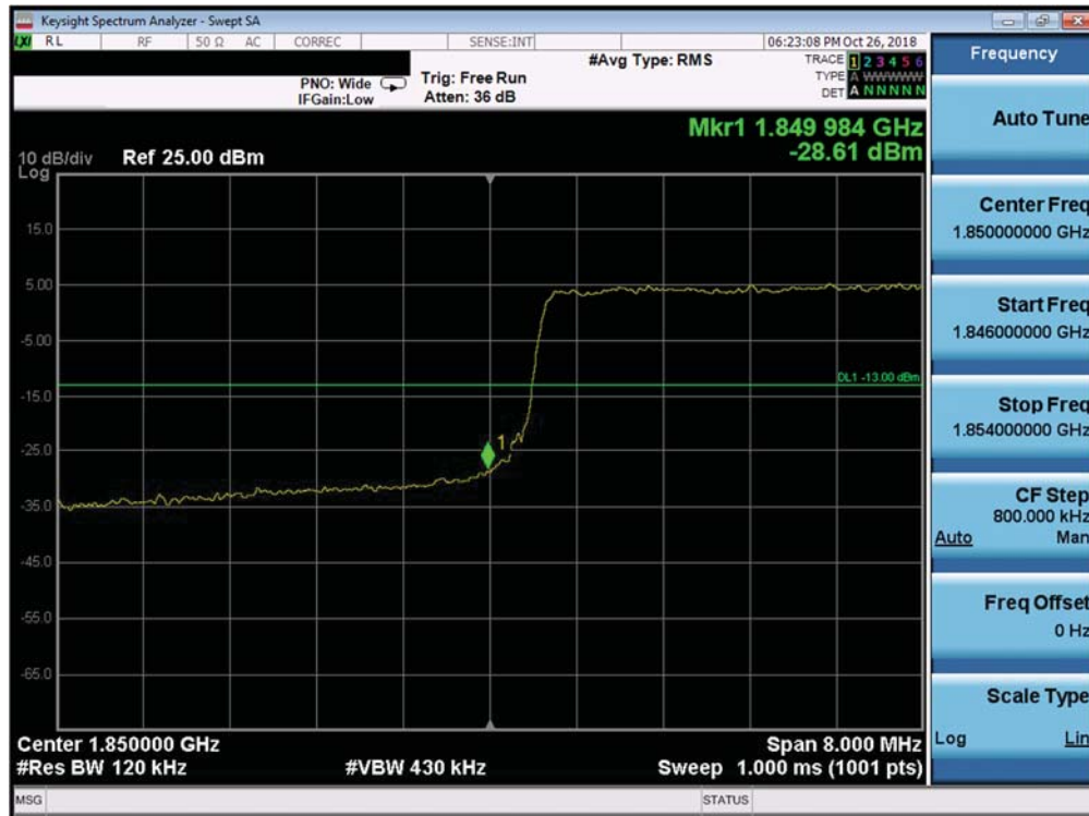
Plot 7-362. Lower Band Edge Plot (Band 25/2 - 10.0MHz QPSK - Full RB Configuration)
