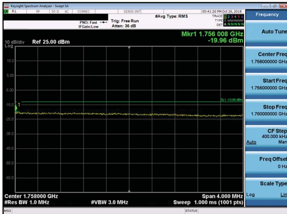
Plot 7-335. Upper Extended Band Edge Plot (Band 4 - 15.0MHz QPSK - Full RB Configuration)
