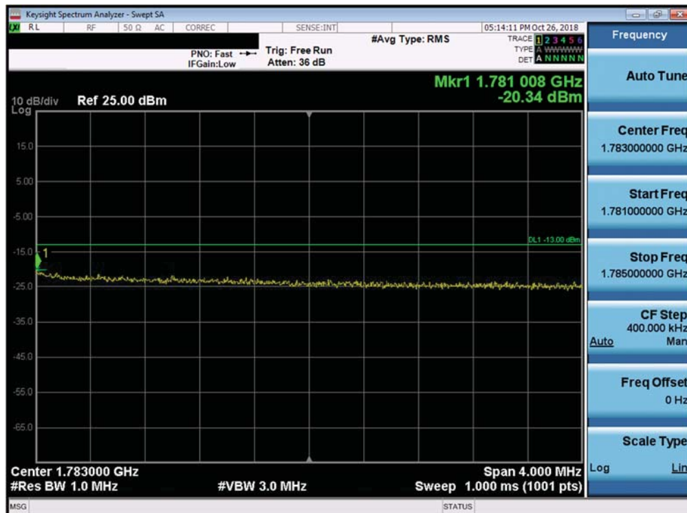
Plot 7-331. Upper Extended Band Edge Plot (Band 66 - 10.0MHz QPSK - Full RB Configuration)
