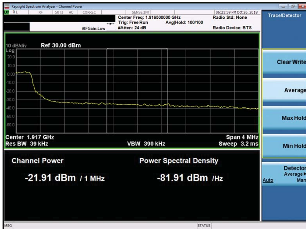
Plot 7-361. Upper Extended Band Edge Plot (Band 25 - 5.0MHz QPSK - Full RB Configuration)
