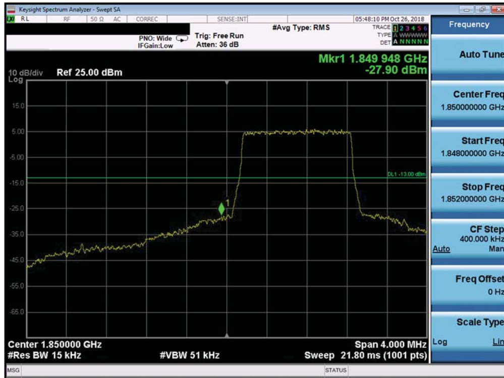
Plot 7-344. Lower Band Edge Plot (Band 25/2 - 1.4MHz QPSK - Full RB Configuration)
