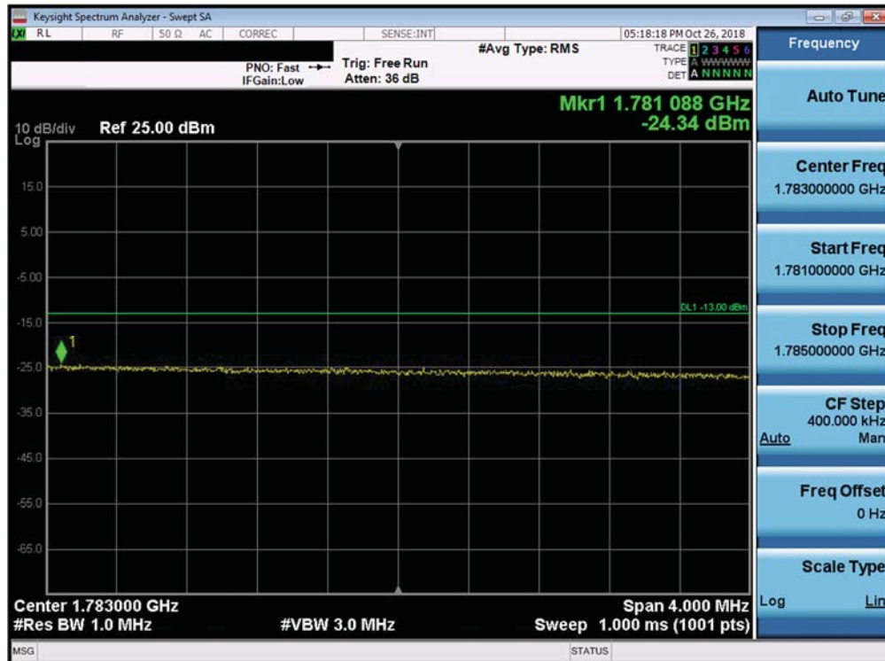
Plot 7-343. Upper Extended Band Edge Plot (Band 66 - 20.0MHz QPSK - Full RB Configuration)
