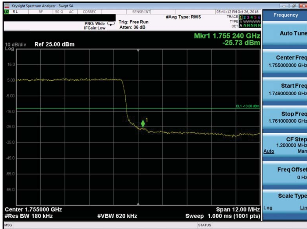
Plot 7-334. Upper Band Edge Plot (Band 4 - 15.0MHz QPSK - Full RB Configuration)
