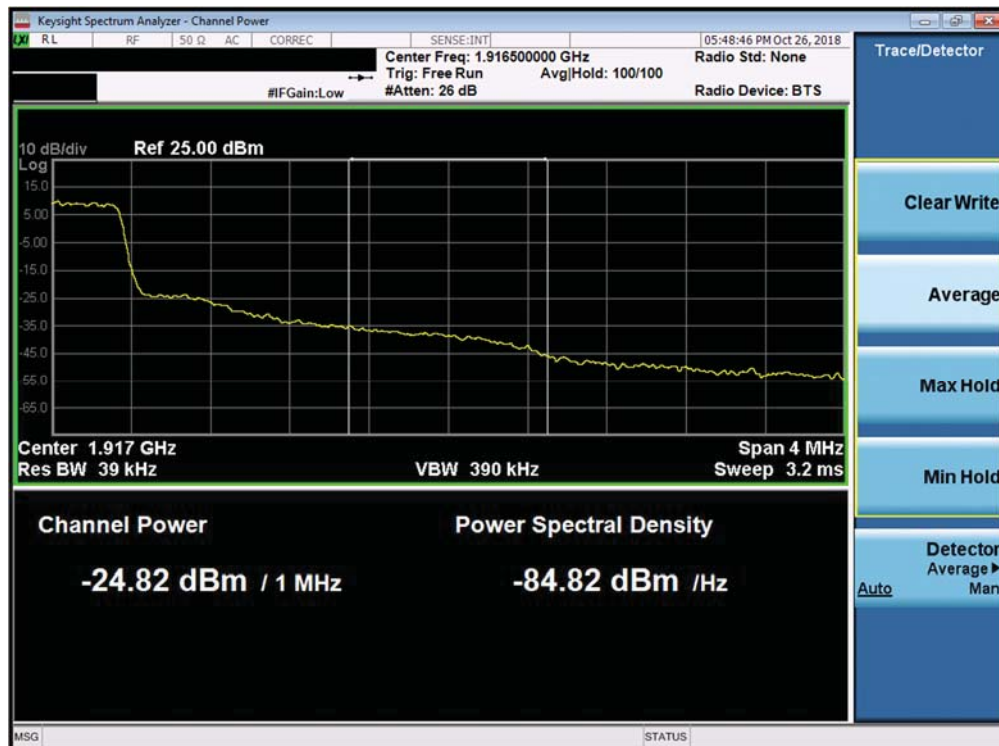
Plot 7-349. Upper Extended Band Edge Plot (Band 25 - 1.4MHz QPSK - Full RB Configuration)
