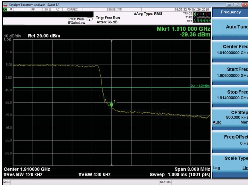
Plot 7-364. Upper Band Edge Plot (Band 2 - 10.0MHz QPSK - Full RB Configuration)
