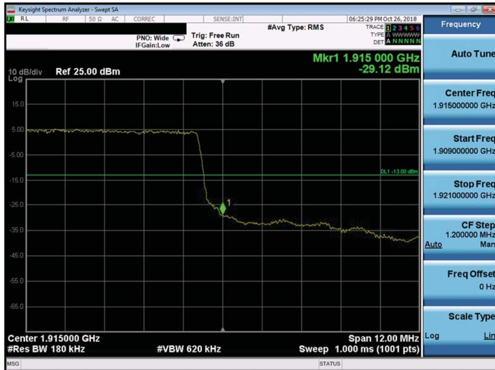
Plot 7-372. Upper Band Edge Plot (Band 25 - 15.0MHz QPSK - Full RB Configuration)
