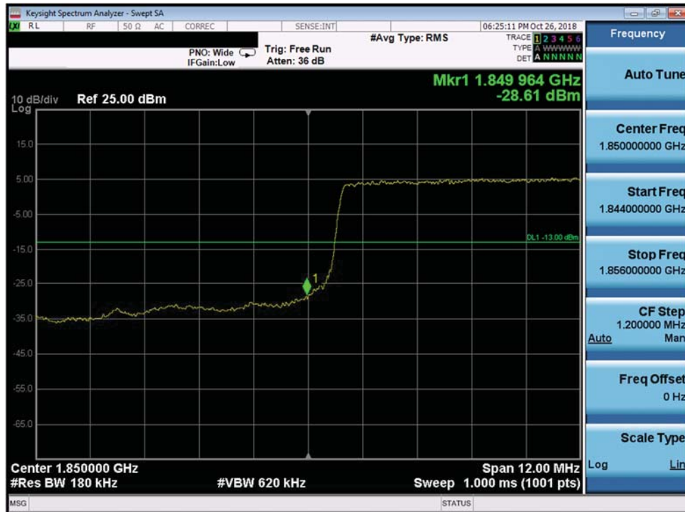
Plot 7-368. Lower Band Edge Plot (Band 25/2 - 15.0MHz QPSK - Full RB Configuration)
