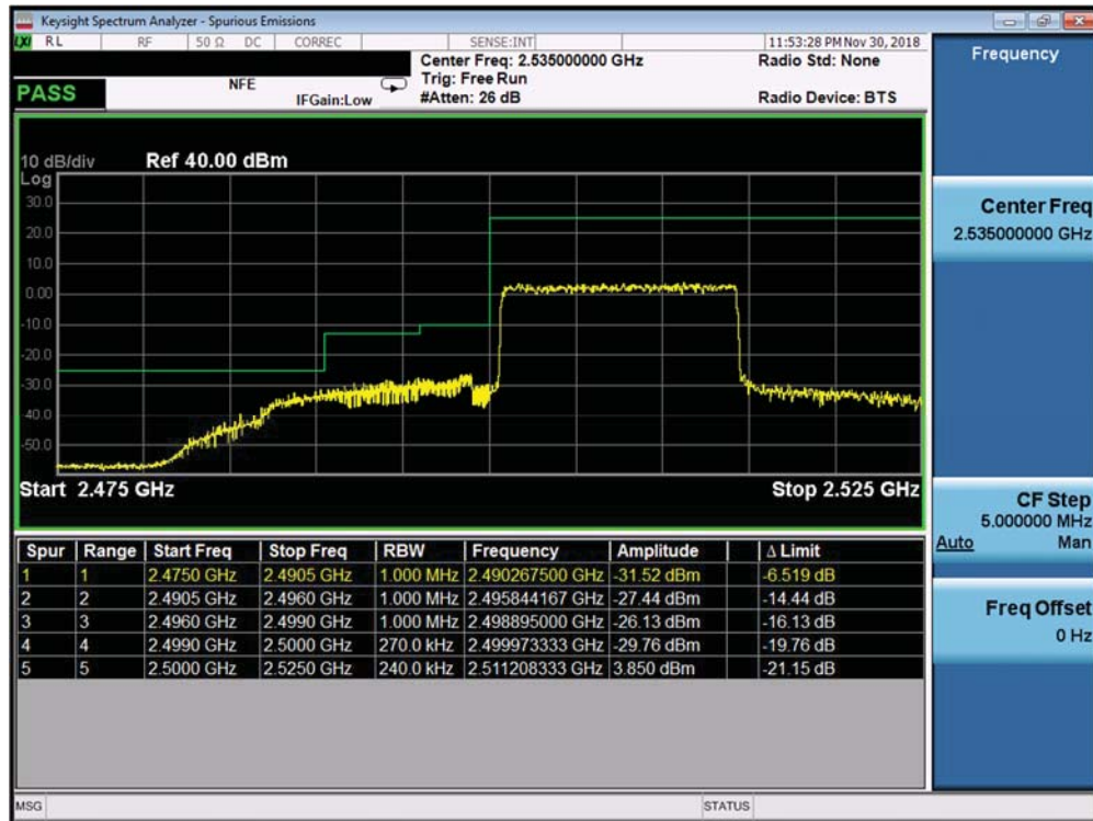
Plot 7-392. Lower ACP Plot (Band 7 ANT B - 15.0MHz QPSK - Full RB Configuration)
