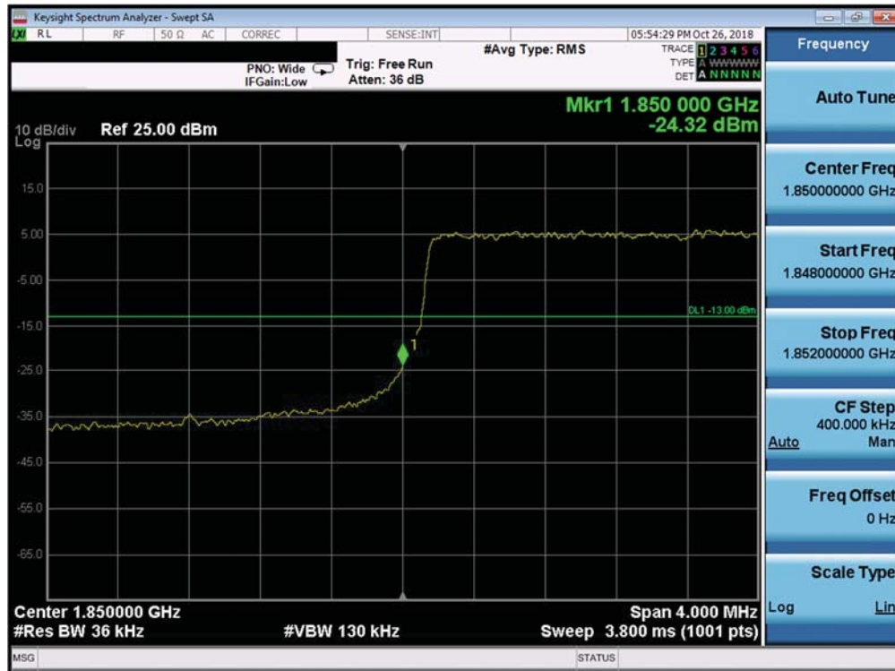
Plot 7-350. Lower Band Edge Plot (Band 25/2 - 3.0MHz QPSK - Full RB Configuration)
