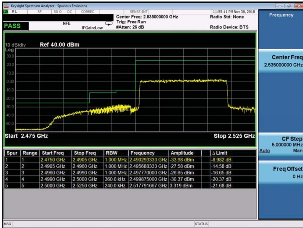
Plot 7-394. Lower ACP Plot (Band 7 ANT B - 20.0MHz QPSK - Full RB Configuration)
