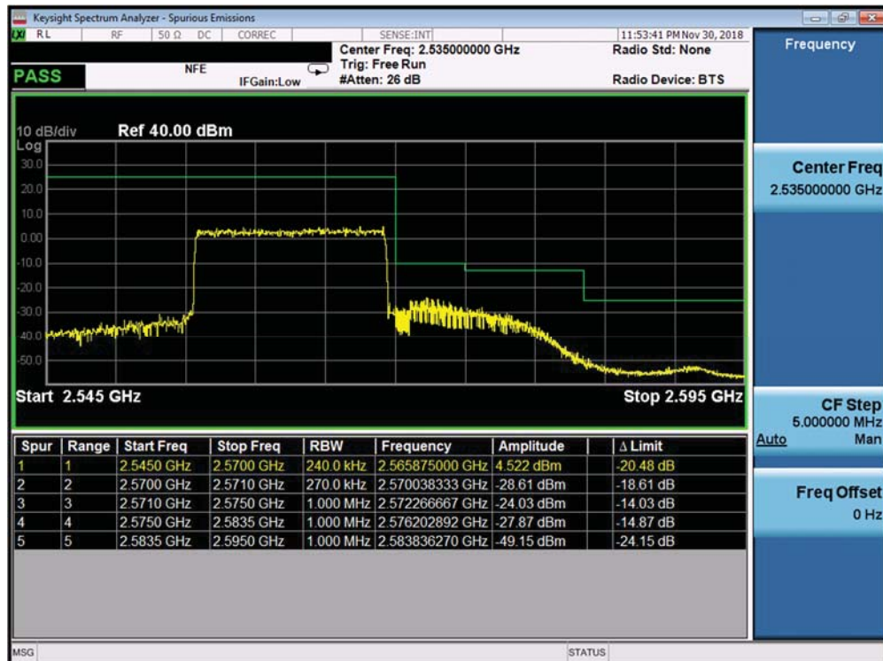
Plot 7-393. Upper ACP Plot (Band 7 ANT B - 15.0MHz QPSK - Full RB Configuration)
