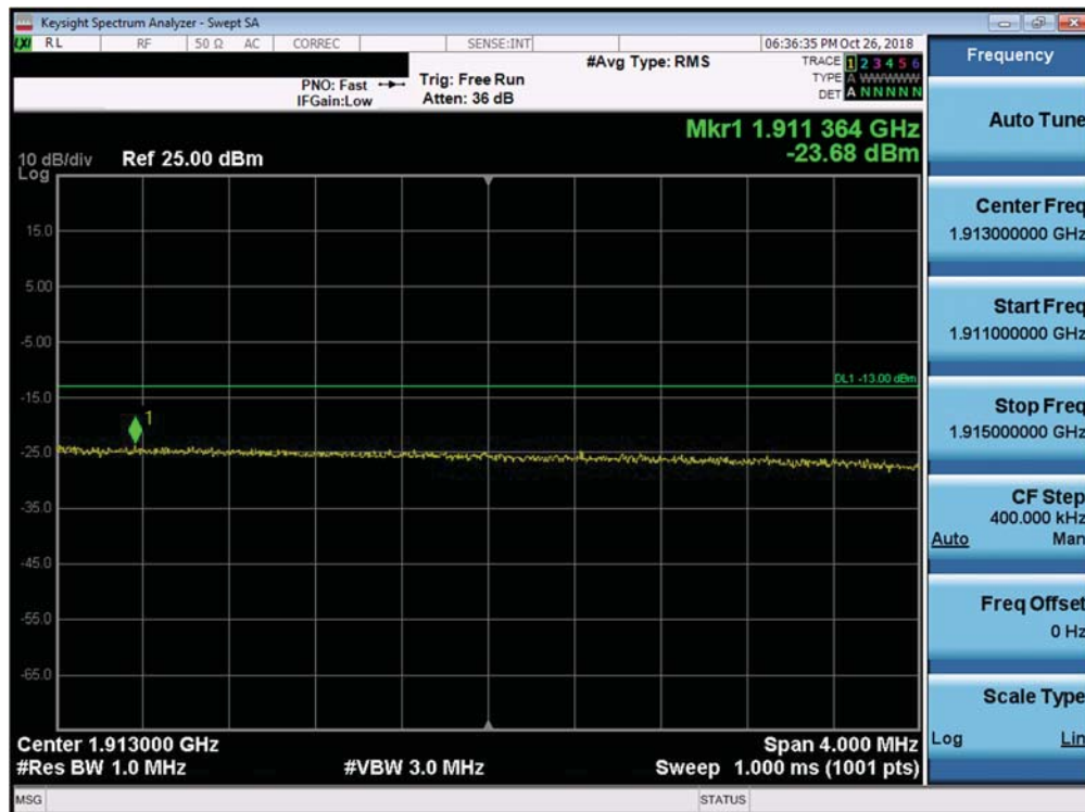
Plot 7-371. Upper Extended Band Edge Plot (Band 2 - 15.0MHz QPSK - Full RB Configuration)
