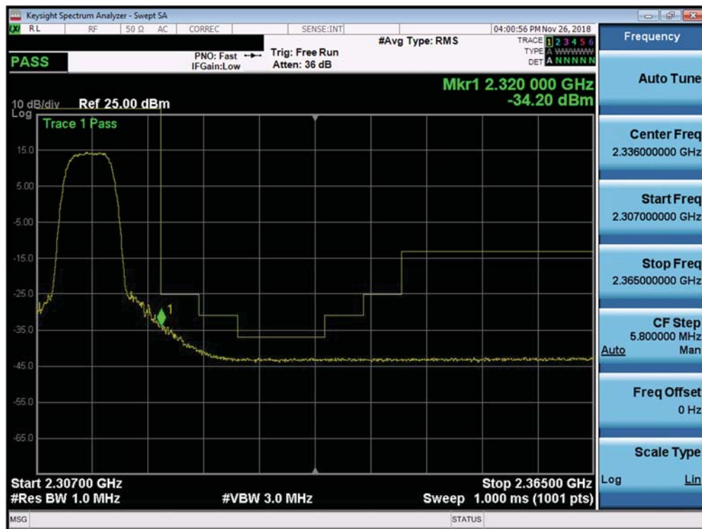
Plot 7-383. Upper Extended Band Edge Plot (Band 30 - 5.0MHz QPSK - Full RB Configuration)
