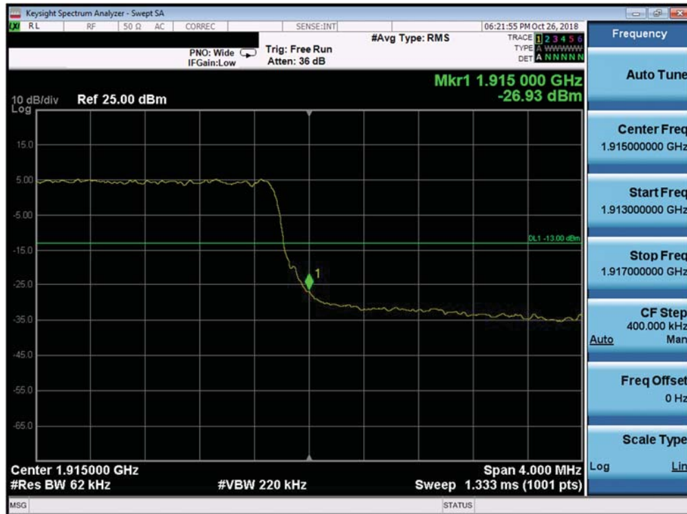
Plot 7-360. Upper Band Edge Plot (Band 25 - 5.0MHz QPSK - Full RB Configuration)
