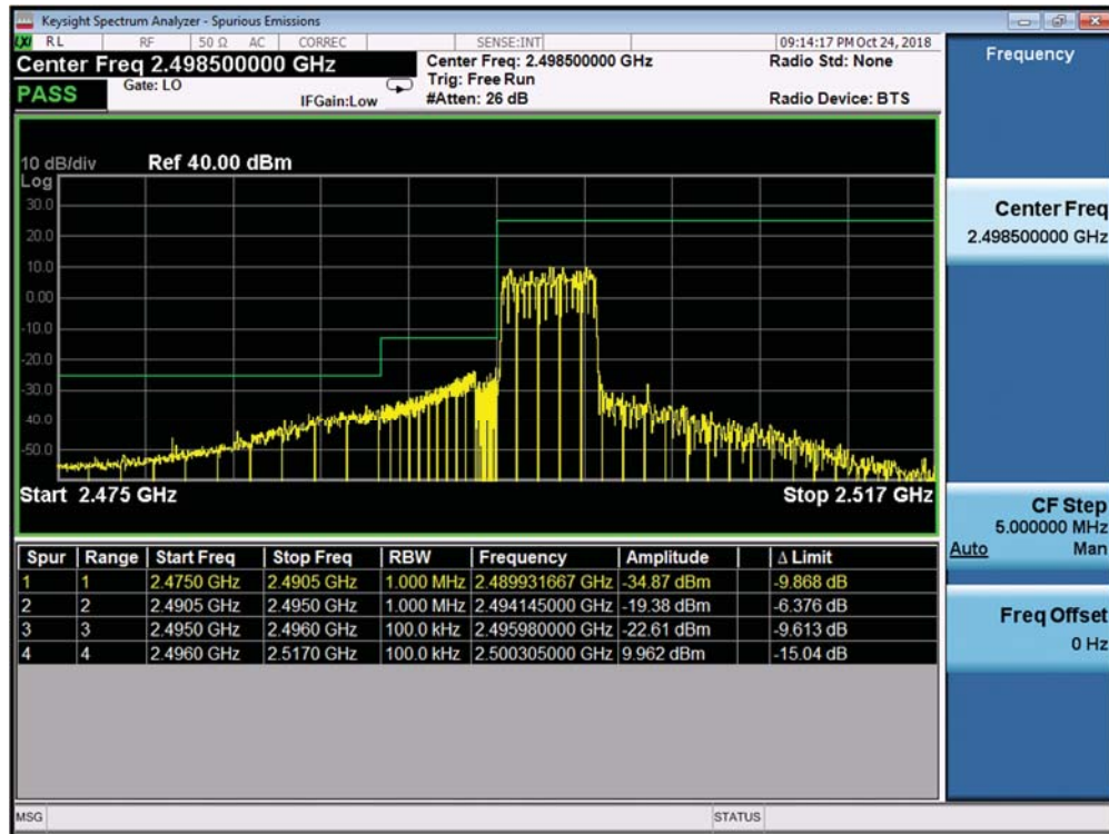
Plot 7-404. Lower ACP Plot (Band 41 PC2 - 5.0MHz QPSK - Full RB Configuration)
