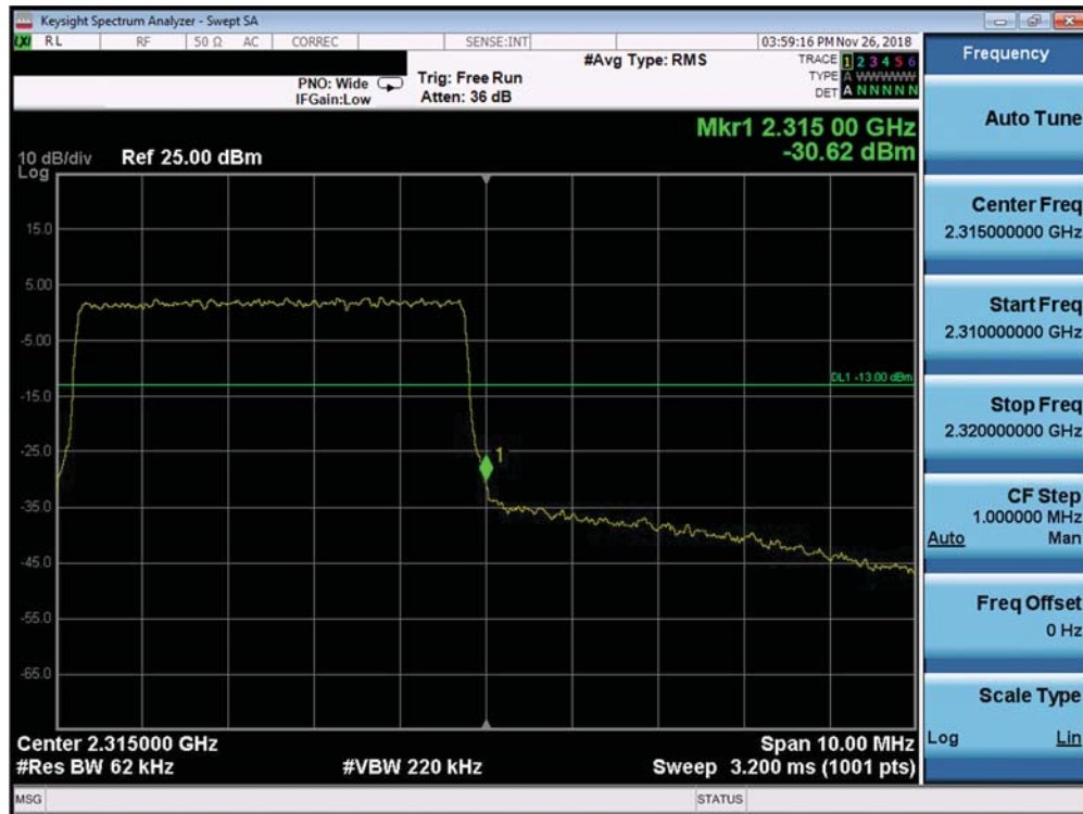
Plot 7-382. Upper Band Edge Plot (Band 30 - 5.0MHz QPSK - Full RB Configuration)
