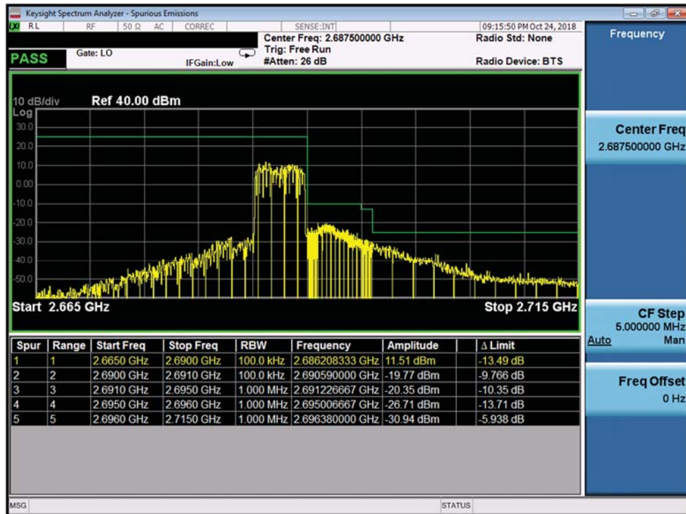
Plot 7-405. Upper ACP Plot (Band 41 PC2 - 5.0MHz QPSK - Full RB Configuration)
