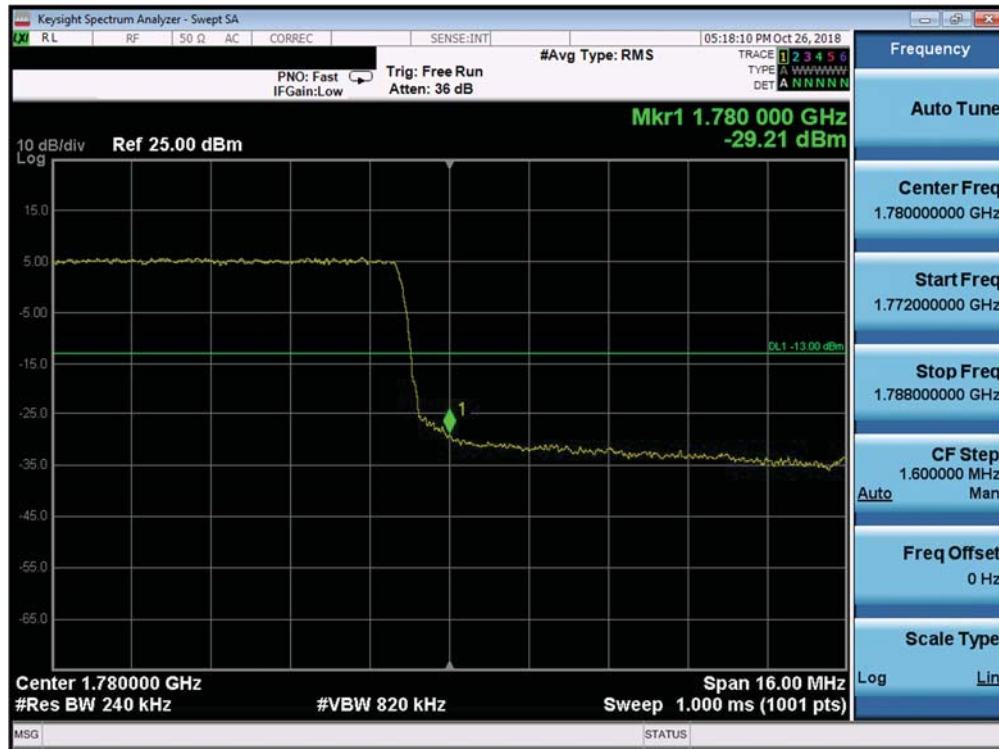
Plot 7-342. Upper Band Edge Plot (Band 66 - 20.0MHz QPSK - Full RB Configuration)
