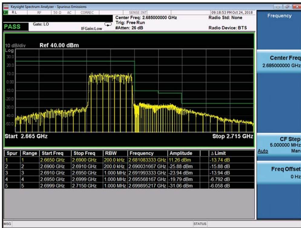
Plot 7-407. Upper ACP Plot (Band 41 PC2 - 10.0MHz QPSK - Full RB Configuration)
