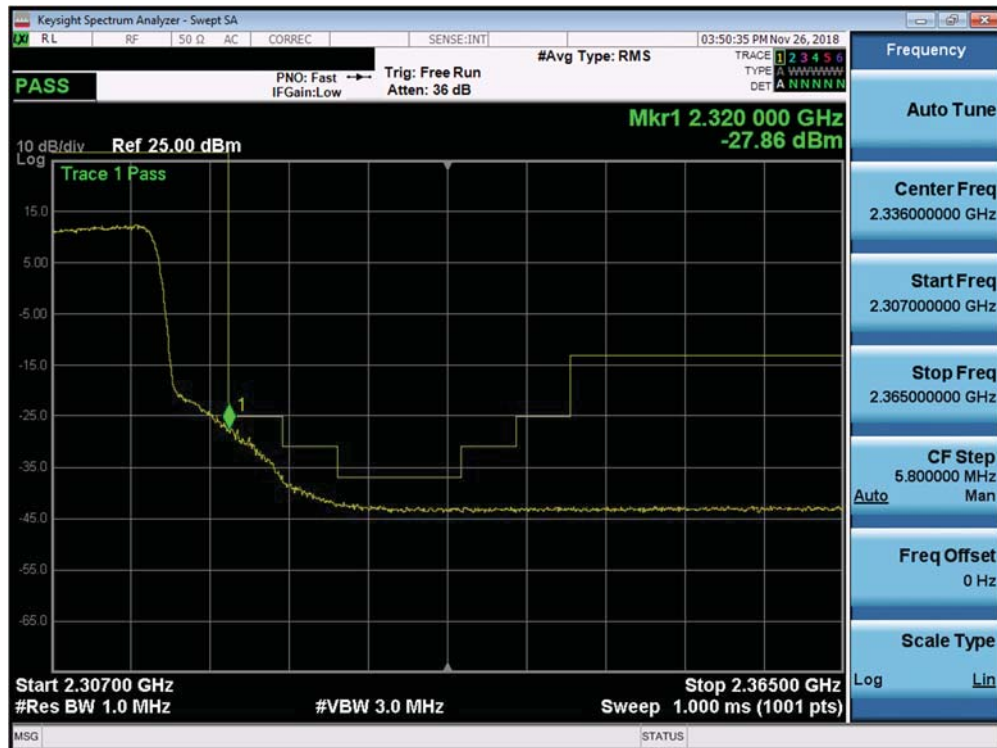
Plot 7-387. Upper Extended Band Edge Plot (Band 30 - 10.0MHz QPSK - Full RB Configuration)
