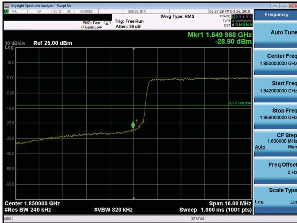
Plot 7-374. Lower Band Edge Plot (Band 25/2 - 20.0MHz QPSK - Full RB Configuration)
