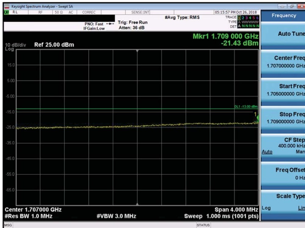
Plot 7-333. Lower Extended Band Edge Plot (Band 66/4 - 15.0MHz QPSK - Full RB Configuration)
