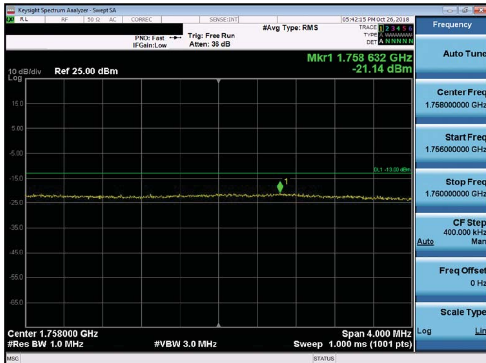
Plot 7-341. Upper Extended Band Edge Plot (Band 4 - 20.0MHz QPSK - Full RB Configuration)
