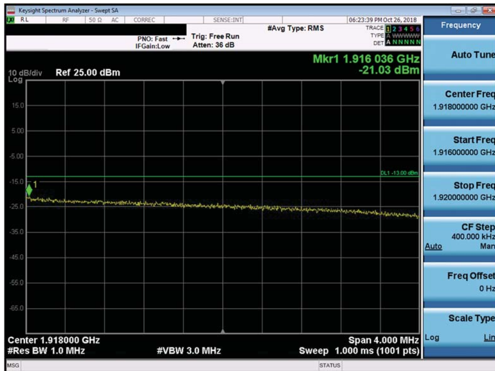
Plot 7-367. Upper Extended Band Edge Plot (Band 25 - 10.0MHz QPSK - Full RB Configuration)
