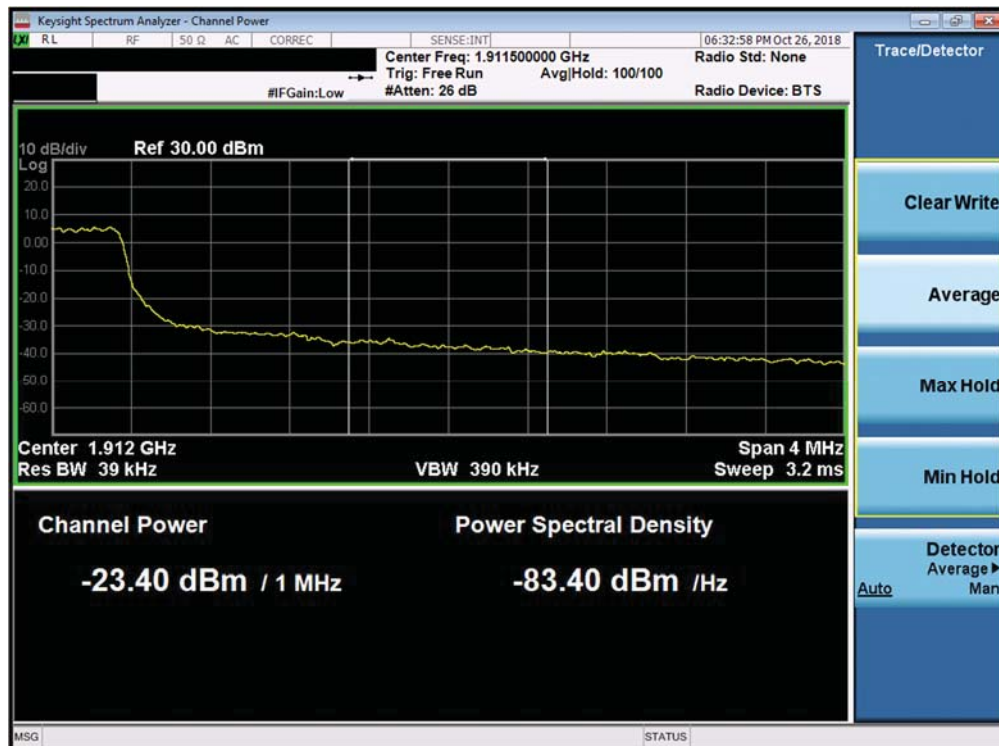
Plot 7-353. Upper Extended Band Edge Plot (Band 2 - 3.0MHz QPSK - Full RB Configuration)
