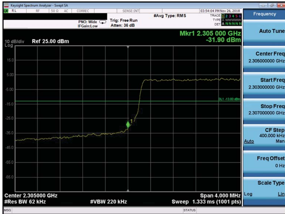
Plot 7-380. Lower Band Edge Plot (Band 30 - 5.0MHz QPSK - Full RB Configuration)
