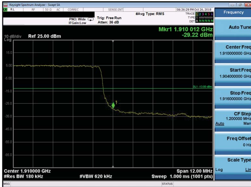
Plot 7-370. Upper Band Edge Plot (Band 2 - 15.0MHz QPSK - Full RB Configuration)
