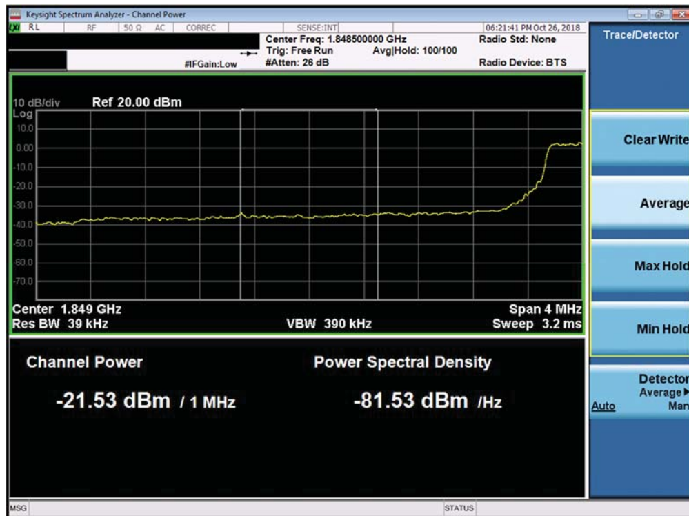
Plot 7-357. Lower Extended Band Edge Plot (Band 25/2 - 5.0MHz QPSK - Full RB Configuration)
