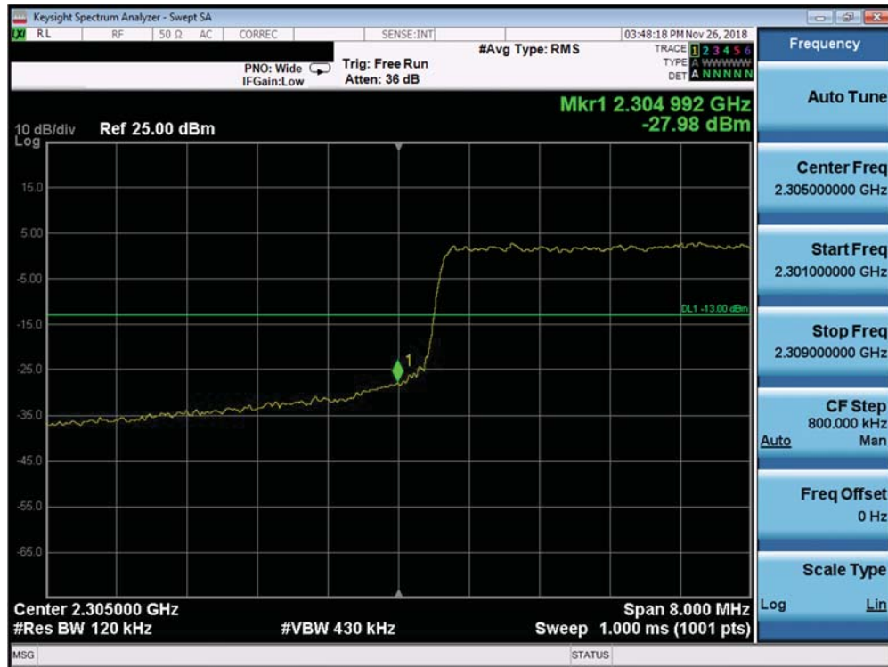
Plot 7-384. Lower Band Edge Plot (Band 30 - 10.0MHz QPSK - Full RB Configuration)
