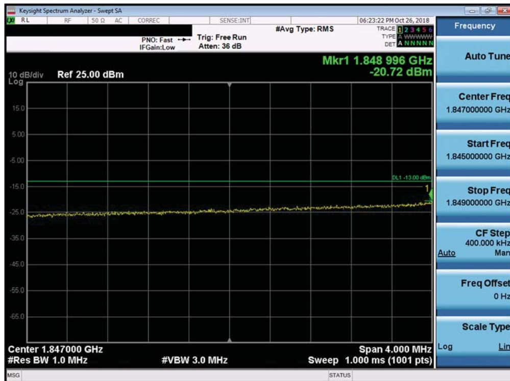
Plot 7-363. Lower Extended Band Edge Plot (Band 25/2 - 10.0MHz QPSK - Full RB Configuration)
