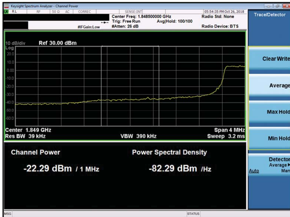
Plot 7-351. Lower Extended Band Edge Plot (Band 25/2 - 3.0MHz QPSK - Full RB Configuration)
