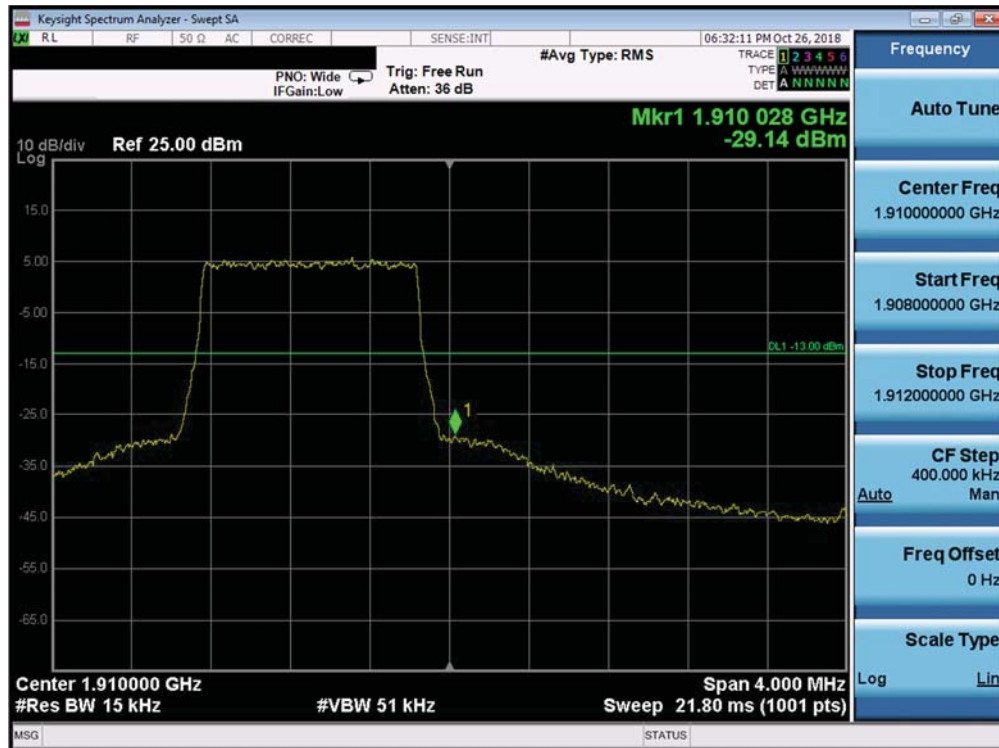
Plot 7-346. Upper Band Edge Plot (Band 2 - 1.4MHz QPSK - Full RB Configuration)
