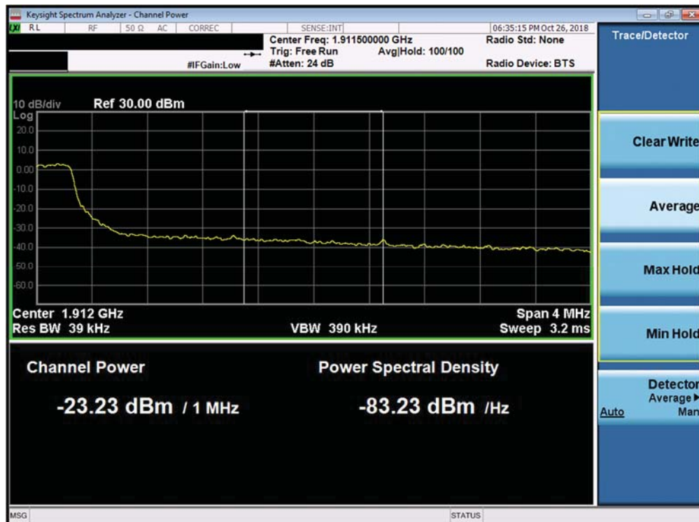
Plot 7-359. Upper Extended Band Edge Plot (Band 2 - 5.0MHz QPSK - Full RB Configuration)
