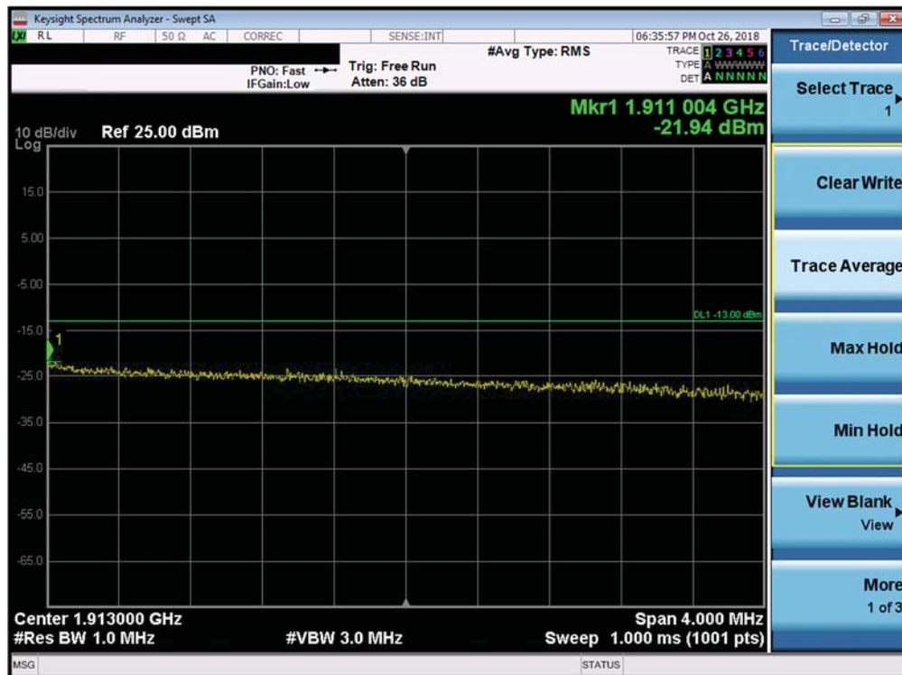
Plot 7-365. Upper Extended Band Edge Plot (Band 2 - 10.0MHz QPSK - Full RB Configuration)
