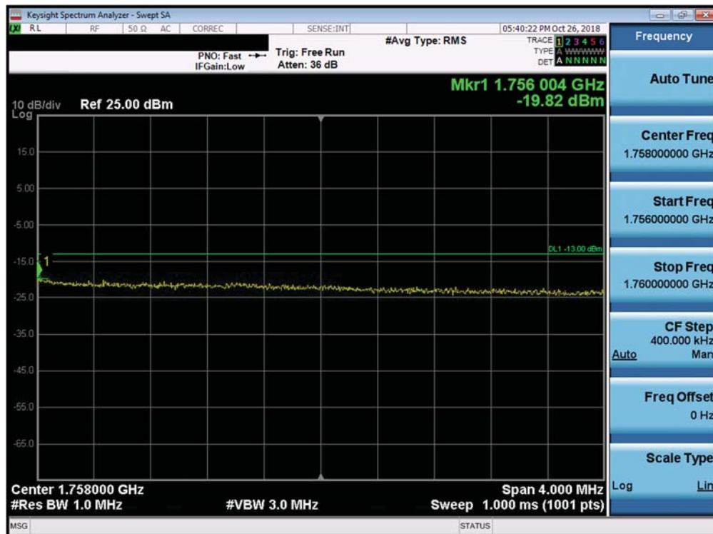
Plot 7-329. Upper Extended Band Edge Plot (Band 4 - 10.0MHz QPSK - Full RB Configuration)
