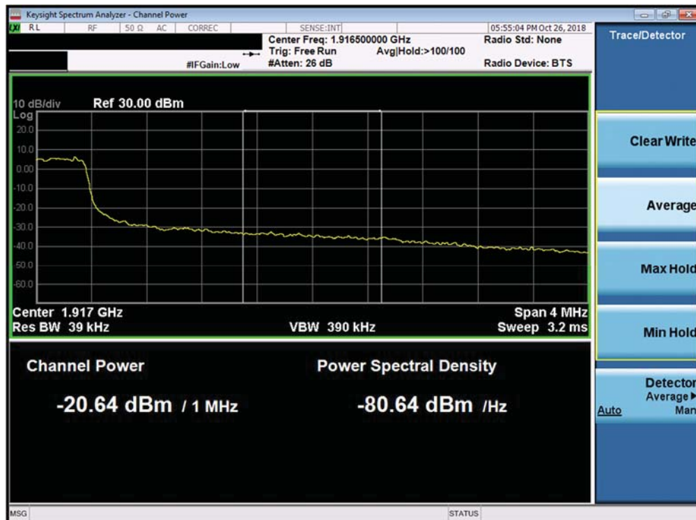
Plot 7-355. Upper Extended Band Edge Plot (Band 25 - 3.0MHz QPSK - Full RB Configuration)
