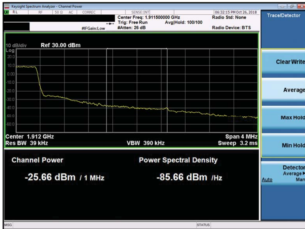
Plot 7-347. Upper Extended Band Edge Plot (Band 2 - 1.4MHz QPSK - Full RB Configuration)
