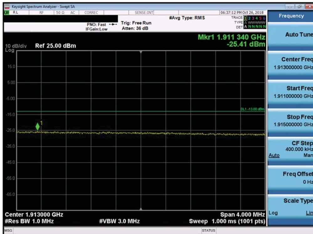
Plot 7-377. Upper Extended Band Edge Plot (Band 2 - 20.0MHz QPSK - Full RB Configuration)
