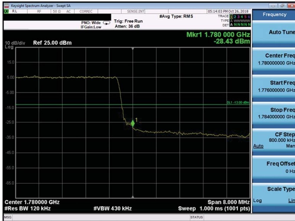
Plot 7-330. Upper Band Edge Plot (Band 66 - 10.0MHz QPSK - Full RB Configuration)
