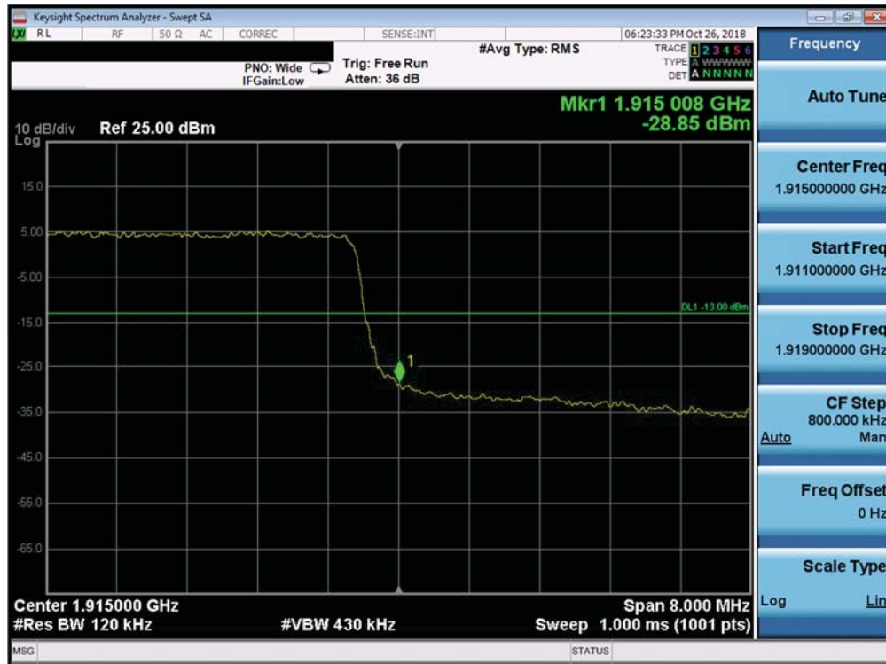
Plot 7-366. Upper Band Edge Plot (Band 25 - 10.0MHz QPSK - Full RB Configuration)
