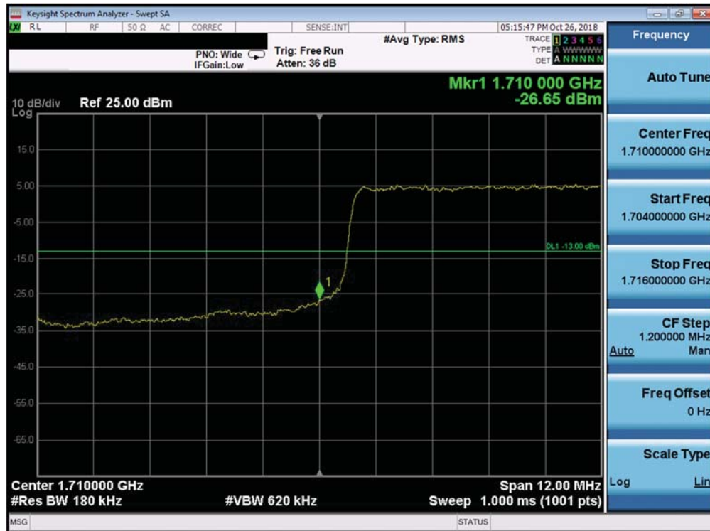
Plot 7-332. Lower Band Edge Plot (Band 66/4 - 15.0MHz QPSK - Full RB Configuration)
