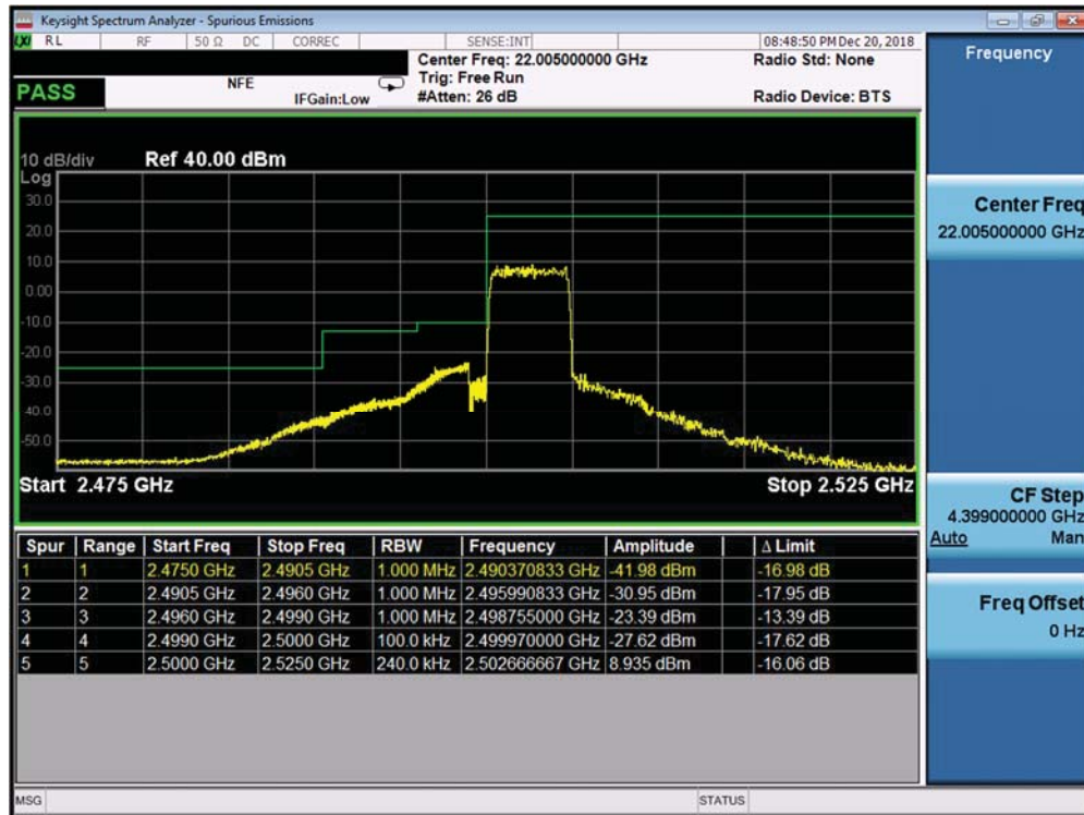
Plot 7-396. Lower ACP Plot (Band 7 Ant A - 5.0MHz QPSK - Full RB Configuration)
