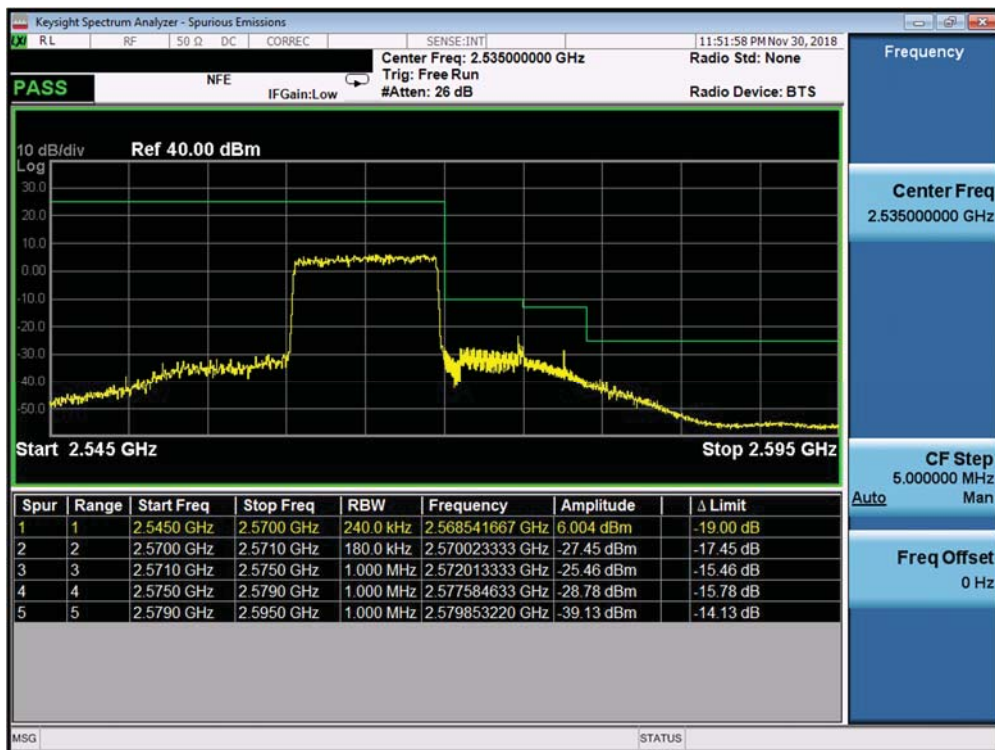
Plot 7-391. Upper ACP Plot (Band 7 ANT B - 10.0MHz QPSK - Full RB Configuration)
