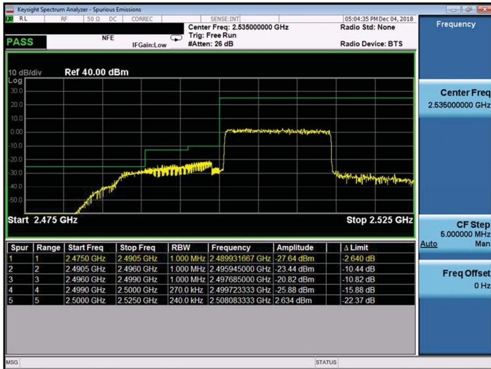
Plot 7-400. Lower ACP Plot (Band 7 Ant A - 15.0MHz QPSK - Full RB Configuration)
