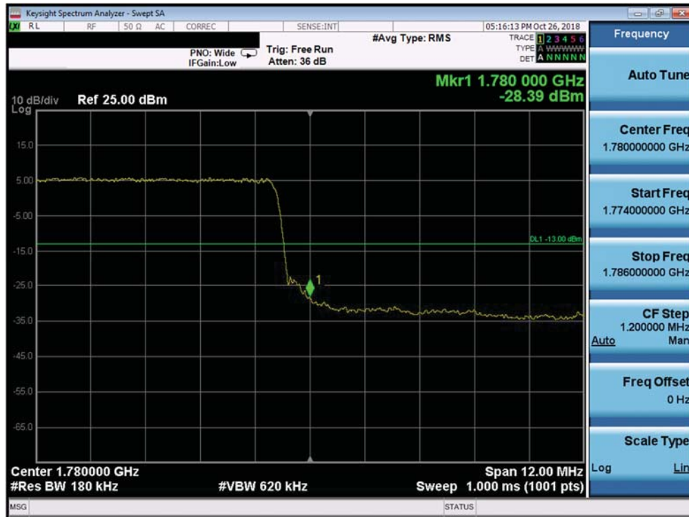
Plot 7-336. Upper Band Edge Plot (Band 66 - 15.0MHz QPSK - Full RB Configuration)
