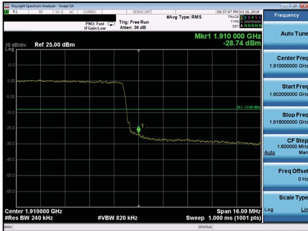
Plot 7-376. Upper Band Edge Plot (Band 2 - 20.0MHz QPSK - Full RB Configuration)
