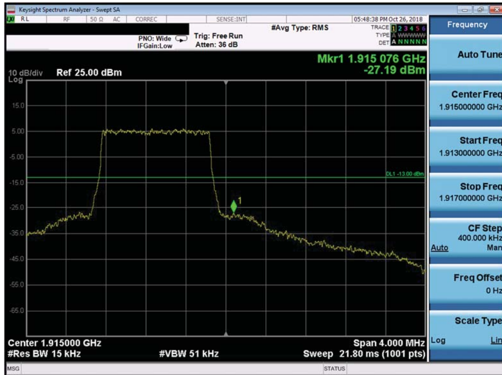
Plot 7-348. Upper Band Edge Plot (Band 25 - 1.4MHz QPSK - Full RB Configuration)
