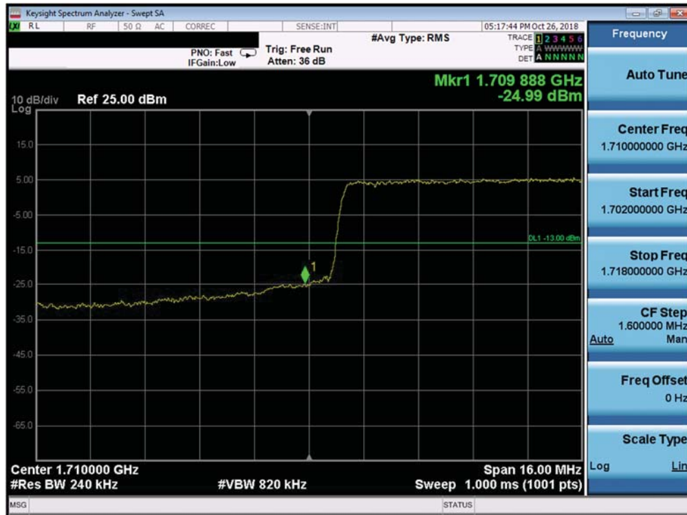
Plot 7-338. Lower Band Edge Plot (Band 66/4 - 20.0MHz QPSK - Full RB Configuration)
