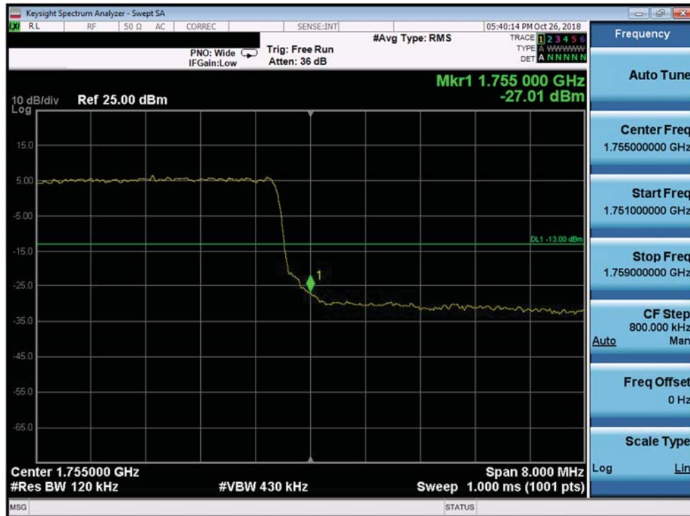
Plot 7-328. Upper Band Edge Plot (Band 4 - 10.0MHz QPSK - Full RB Configuration)
