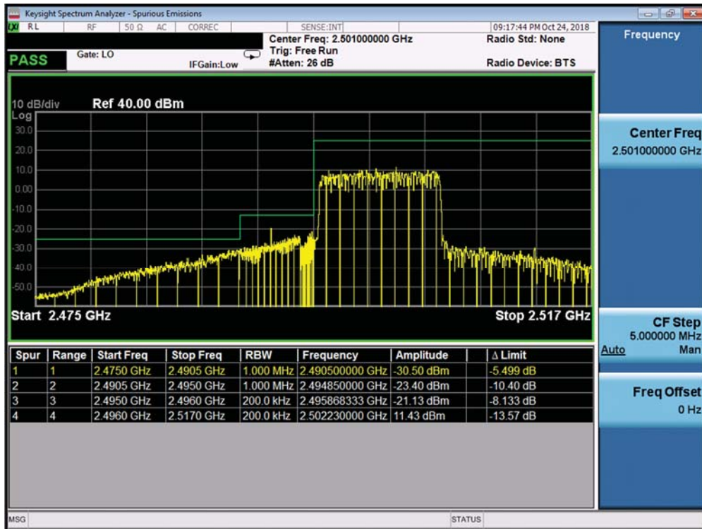
Plot 7-406. Lower ACP Plot (Band 41 PC2 - 10.0MHz QPSK - Full RB Configuration)
