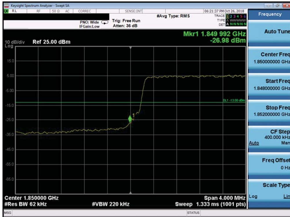
Plot 7-356. Lower Band Edge Plot (Band 25/2 - 5.0MHz QPSK - Full RB Configuration)
