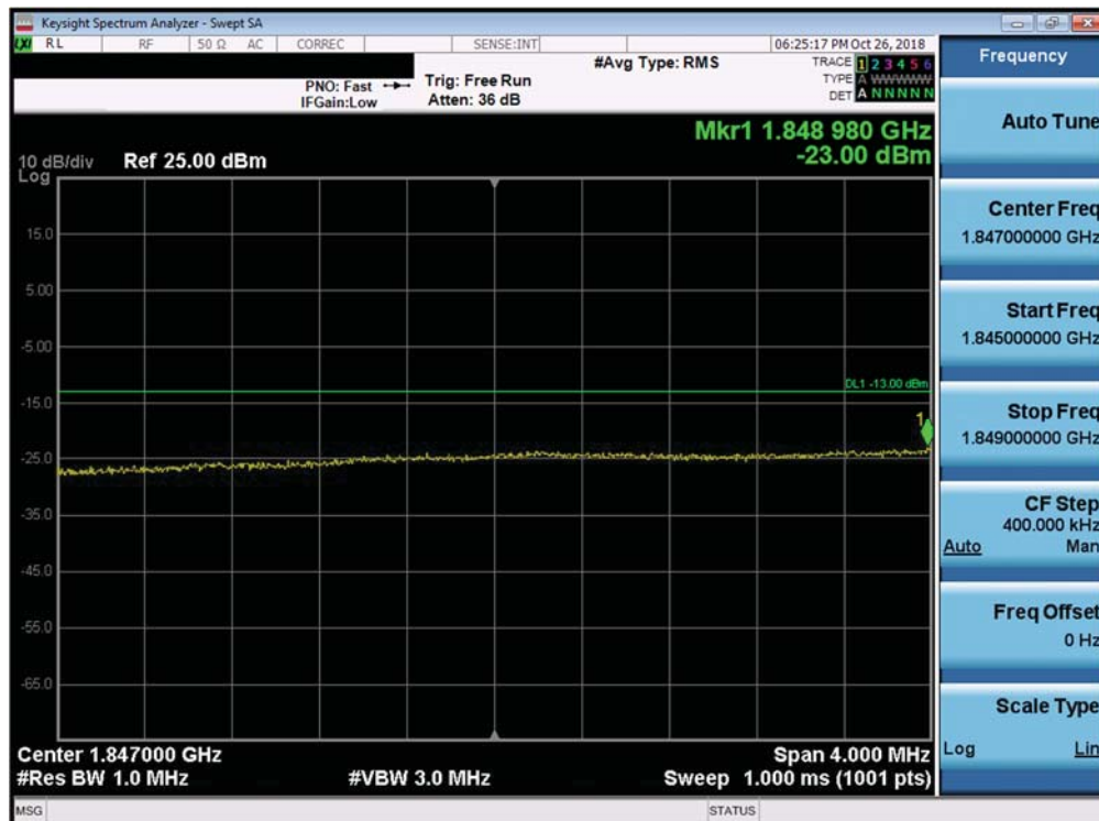
Plot 7-369. Lower Extended Band Edge Plot (Band 25/2 - 15.0MHz QPSK - Full RB Configuration)
