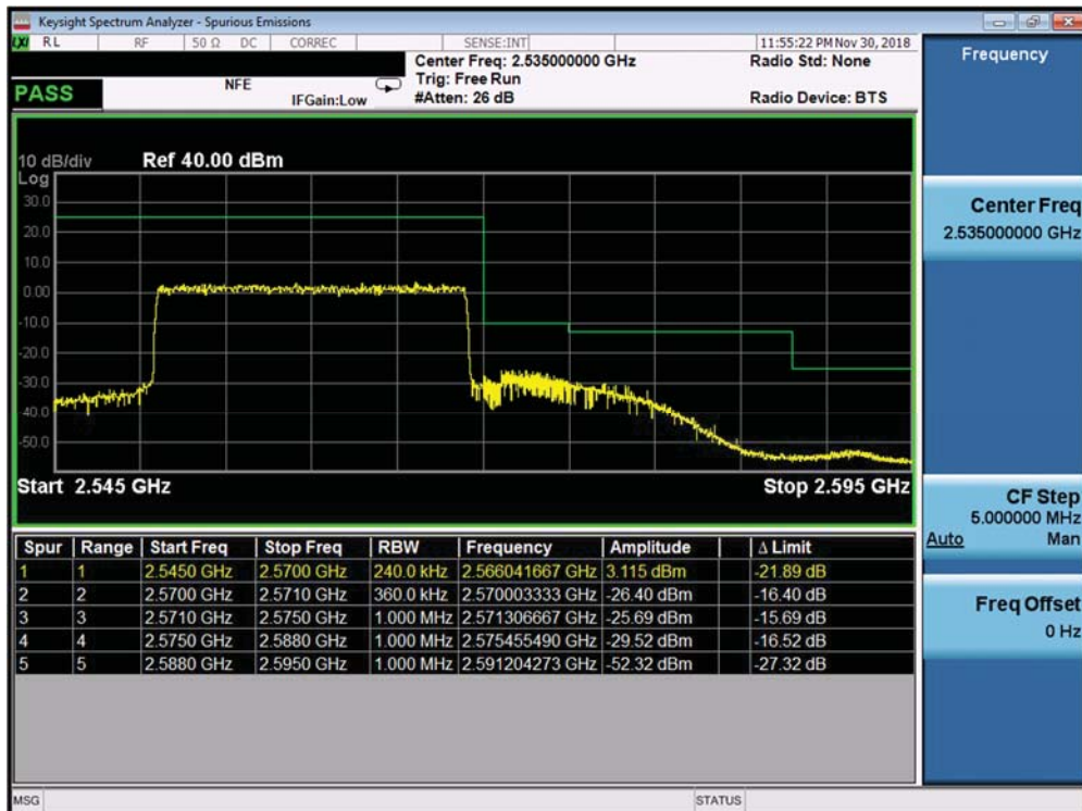
Plot 7-395. Upper ACP Plot (Band 7 ANT B - 20.0MHz QPSK - Full RB Configuration)
