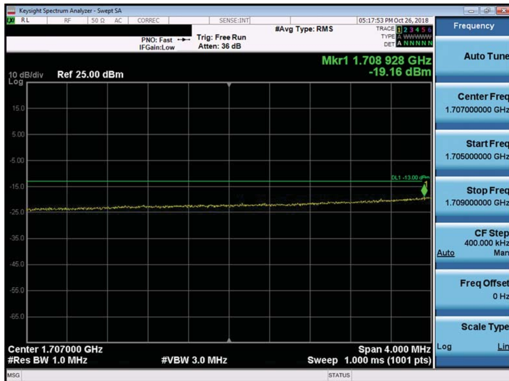
Plot 7-339. Lower Extended Band Edge Plot (Band 66/4 - 20.0MHz QPSK - Full RB Configuration)
