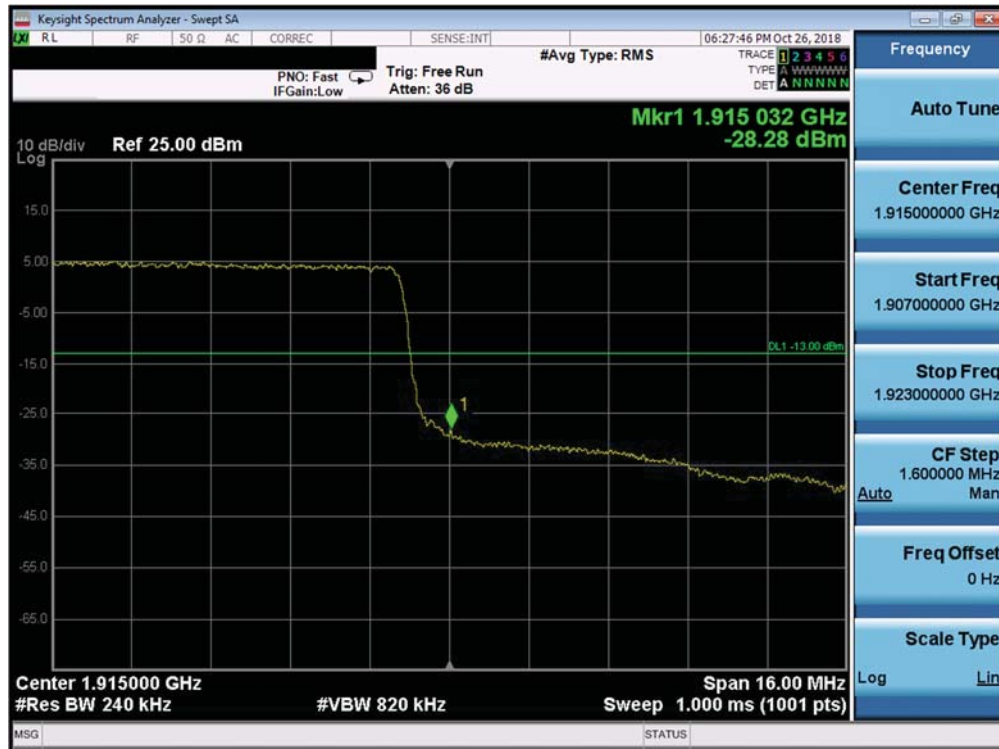
Plot 7-378. Upper Band Edge Plot (Band 25 - 20.0MHz QPSK - Full RB Configuration)
