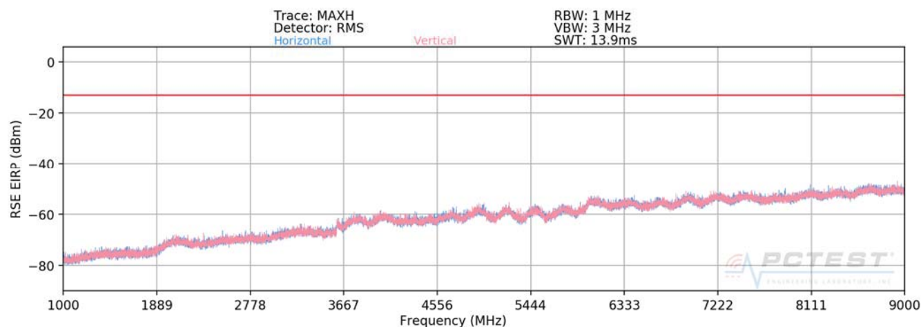
Plot 7-533. Radiated Spurious Plot above 1GHz (Band 26/5)
