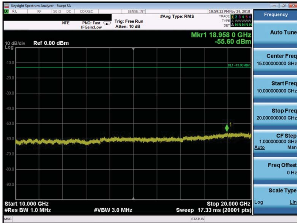
Plot 7-525. Conducted Spurious Plot (Band 66 – 20.0MHz QPSK – PCC 100/0 SCC 100/0 – Mid Channel)
