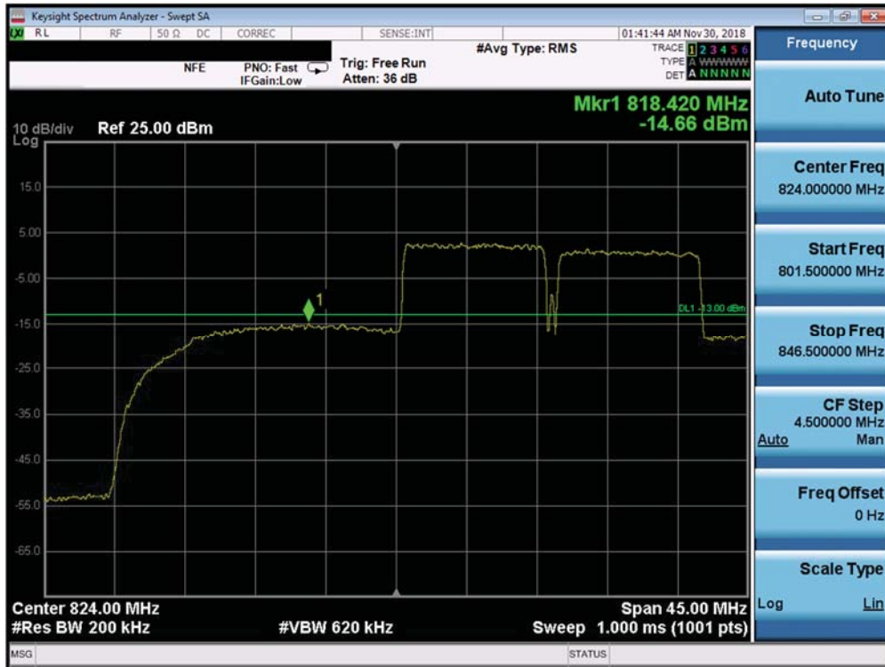
Plot 7-504. Lower Band Edge Plot (Band 5 QPSK – PCC:10 MHz SCC:10 MHz – Full RB)
