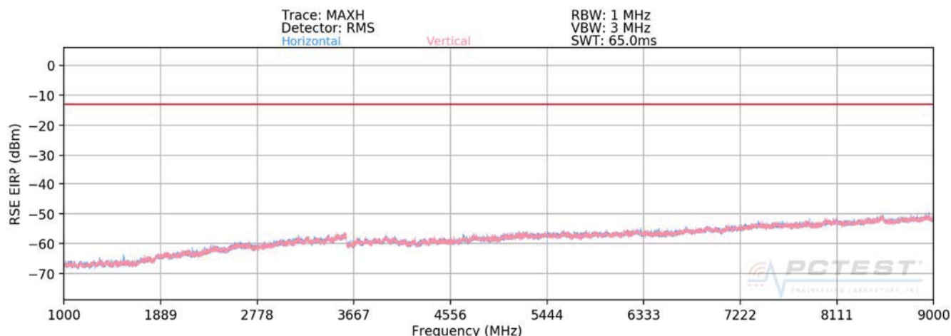
Plot 7-543. Radiated Spurious Plot (ULCA B5 PCC: RB 50 Offset 0, SCC: RB 50 Offset 0 – High Channel)
