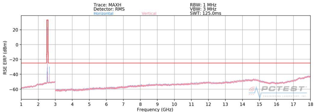
Plot 7-537. Radiated Spurious Plot above 1GHz (Band 7 ANT B)
