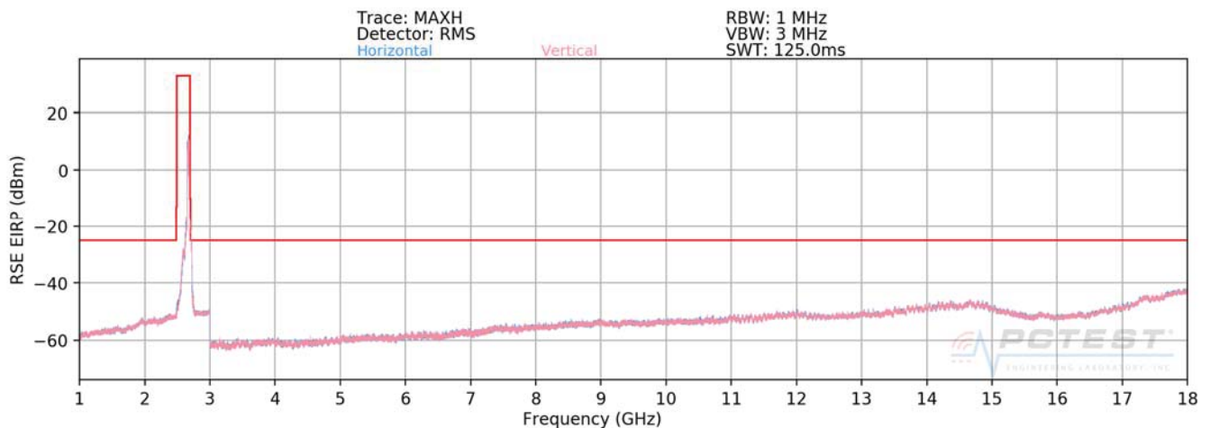
Plot 7-561. Radiated Spurious Plot (ULCA B41 PC2 PCC: RB 100 Offset 0, SCC: RB 100 Offset 0 – High Channel)
