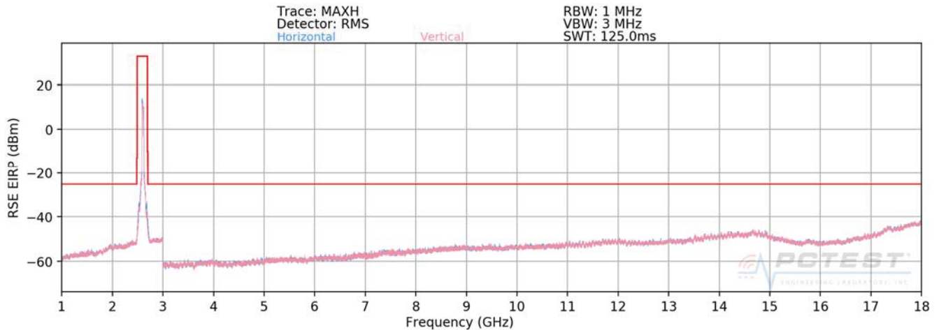
Plot 7-566. Radiated Spurious Plot (ULCA B41 PC3 PCC: RB 100 Offset 0, SCC: RB 100 Offset 0 – Mid Channel)
