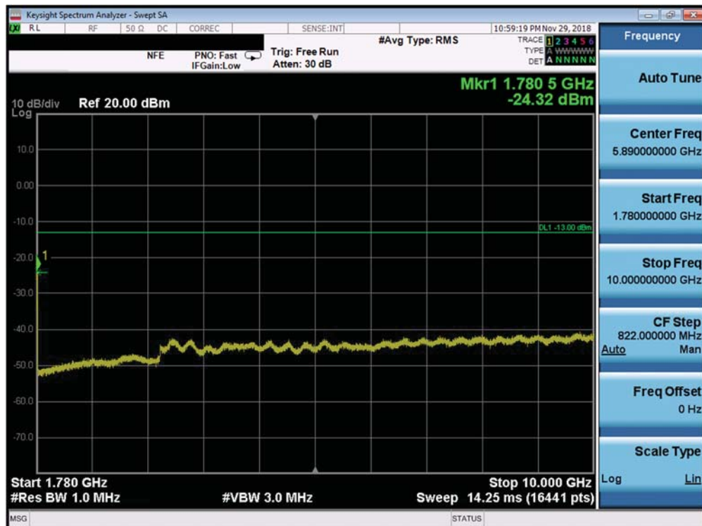
Plot 7-524. Conducted Spurious Plot (Band 66 – 20.0MHz QPSK – PCC 100/0 SCC 100/0 – Mid Channel)
