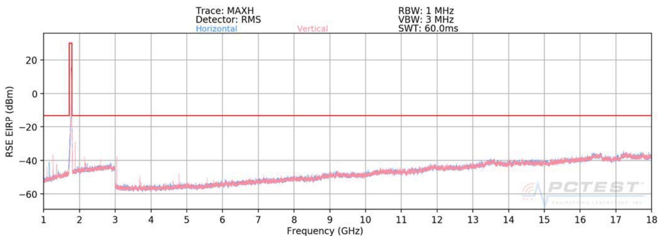
Plot 7-549. Radiated Spurious Plot (ULCA B66 PCC: RB 75 Offset 0, SCC: RB 25 Offset 0 – High Channel)
