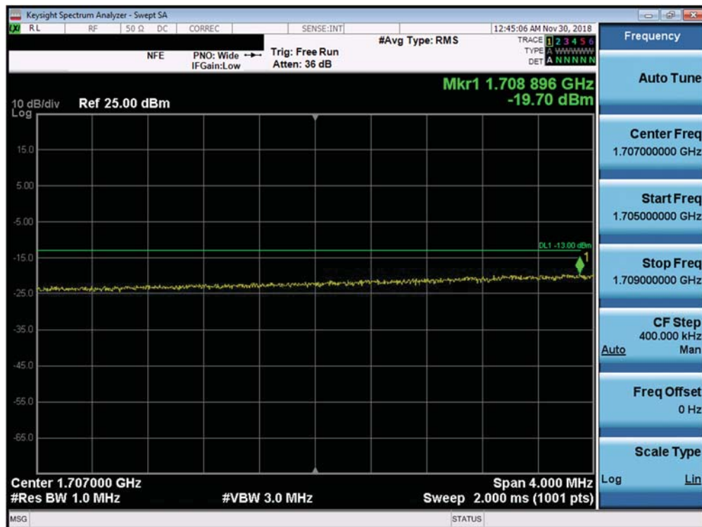
Plot 7-515. Extended Lower Band Edge Plot (Band 66 QPSK – PCC:15 MHz SCC:5 MHz – Full RB)
