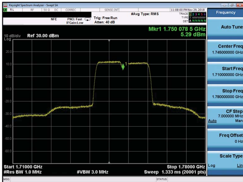
Plot 7-511. Conducted Spurious Plot (Band 66 – 10.0MHz QPSK – PCC 50/0 SCC 50/0 – Mid Channel)
