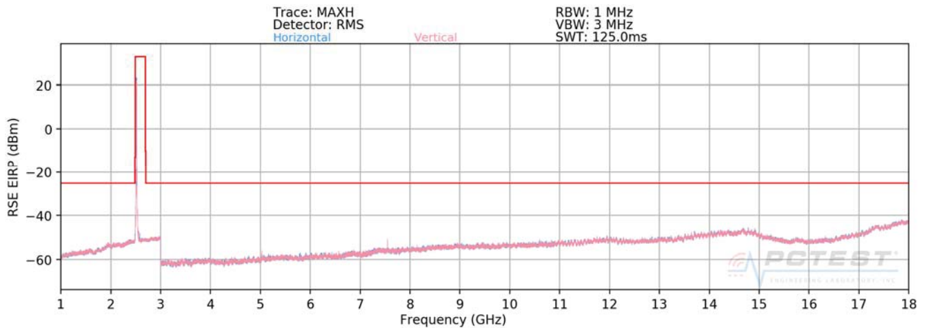
Plot 7-556. Radiated Spurious Plot (ULCA B41 PC2 PCC: RB 1 Offset 99, SCC: RB 1 Offset 0 – Low Channel)
