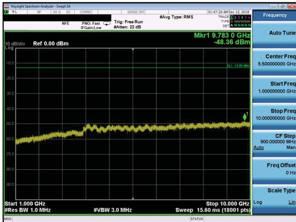
Plot 7-503. Conducted Spurious Plot (Band 5 – 10.0MHz QPSK – PCC 50/0 SCC 50/0 – Mid Channel)
