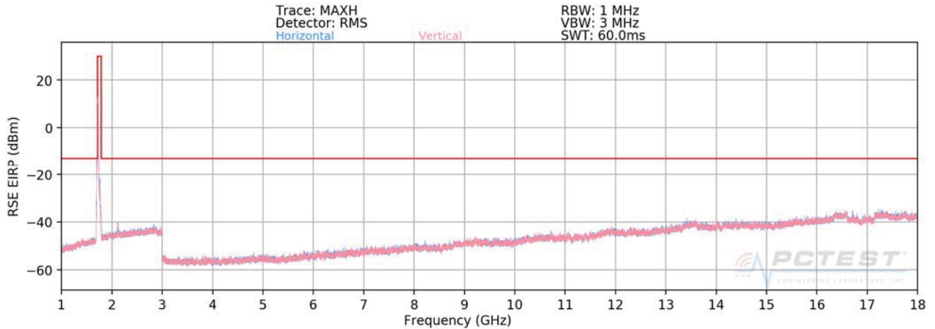
Plot 7-547. Radiated Spurious Plot (ULCA B66 PCC: RB 75 Offset 0, SCC: RB 25 Offset 0 – Low Channel)
