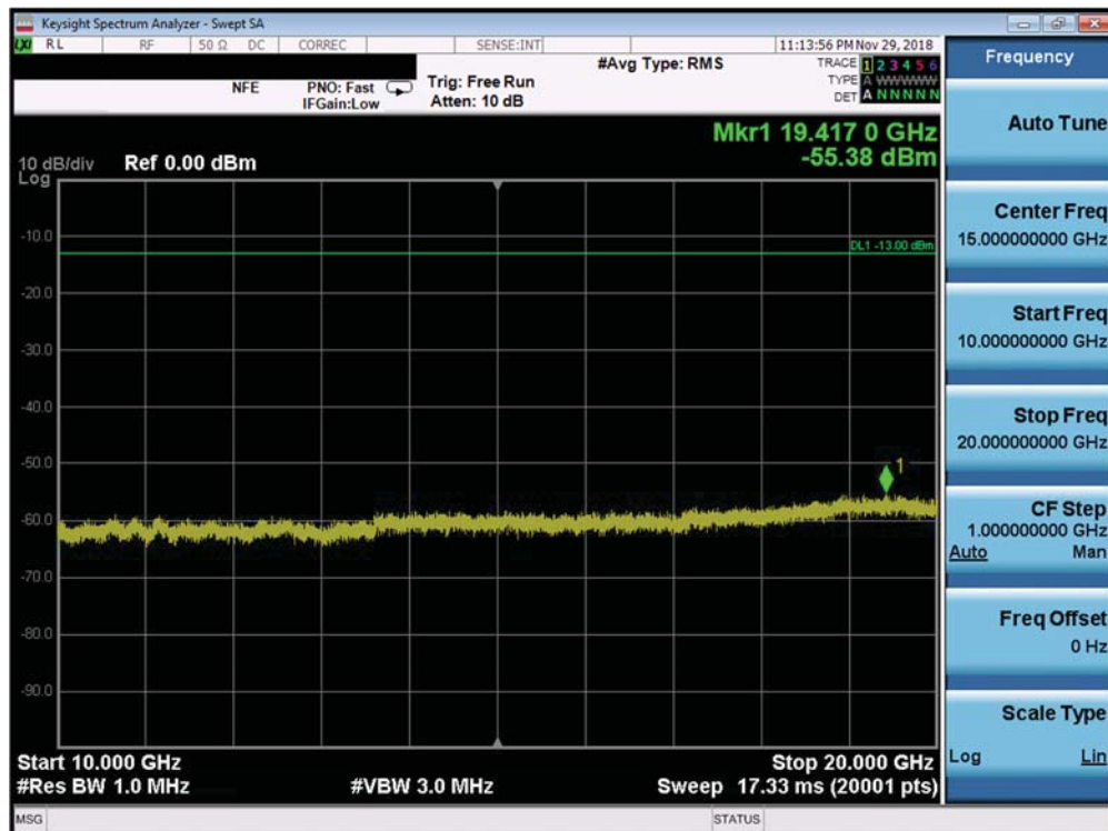
Plot 7-513. Conducted Spurious Plot (Band 66 – 10.0MHz QPSK – PCC 50/0 SCC 50/0 – Mid Channel)
