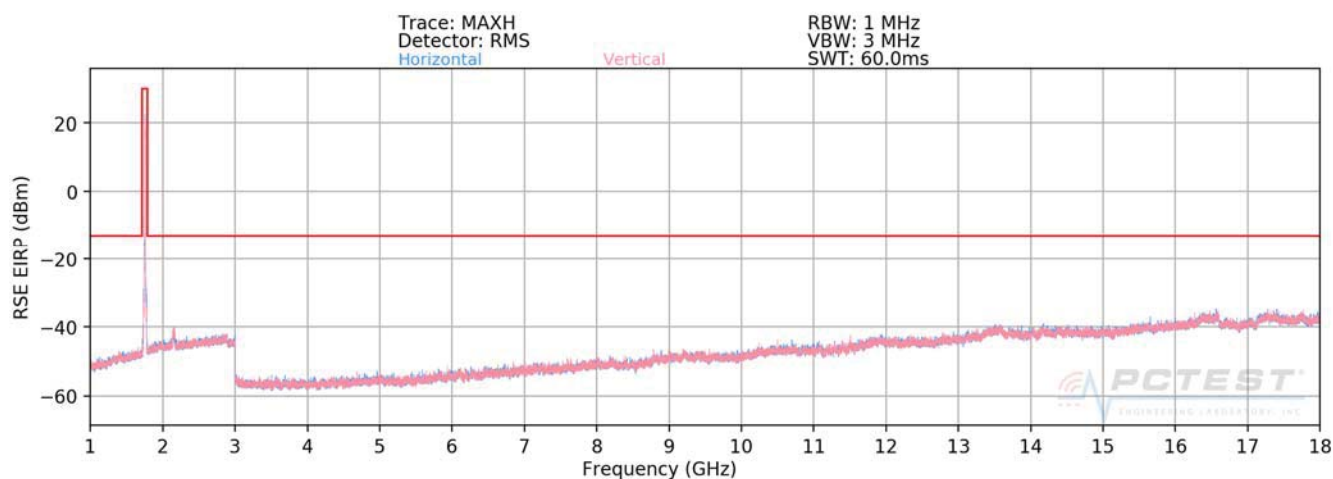
Plot 7-534. Radiated Spurious Plot above 1GHz (Band 66/4)
