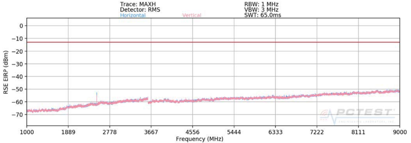
Plot 7-540. Radiated Spurious Plot (ULCA B5 PCC: RB 1 Offset 49, SCC: RB 1 Offset 0 – Low Channel)
