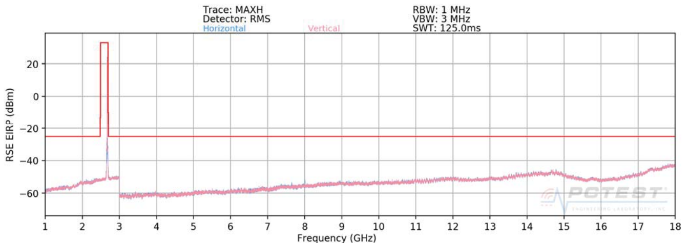
Plot 7-564. Radiated Spurious Plot (ULCA B41 PC3 PCC: RB 1 Offset 0, SCC: RB 1 Offset 99 – High Channel)
