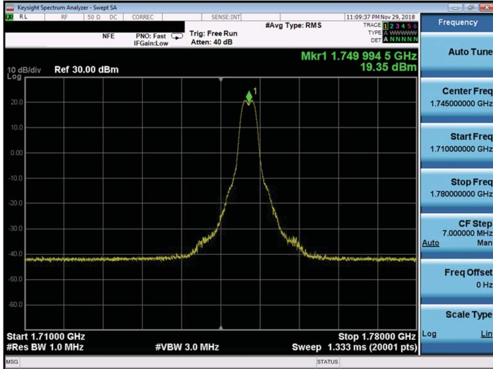
Plot 7-507. Conducted Spurious Plot (Band 66 – 10.0MHz QPSK – PCC 1/49 SCC 1/0 – Mid Channel)
