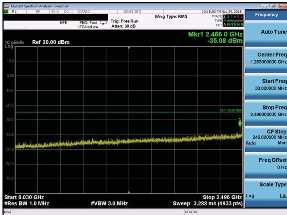
Plot 7-490. Conducted Spurious Plot (Band 41 – PC3 – 20.0MHz QPSK – PCC 100/0 SCC 100/0 – Mid Channel)
