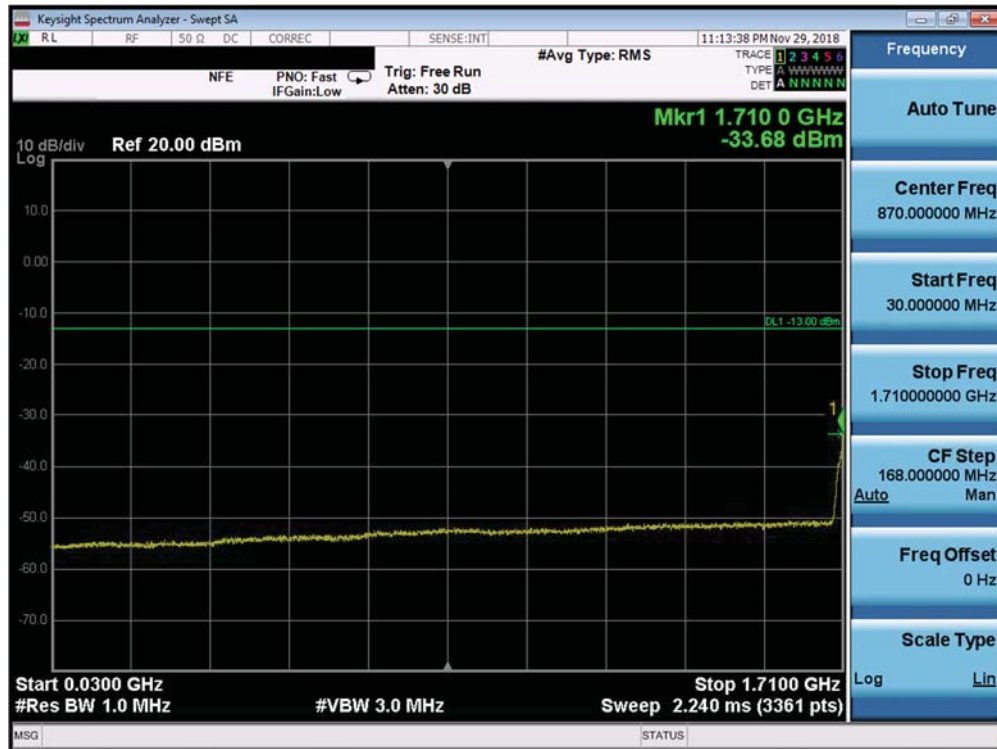
Plot 7-510. Conducted Spurious Plot (Band 66 – 10.0MHz QPSK – PCC 50/0 SCC 50/0 – Mid Channel)
