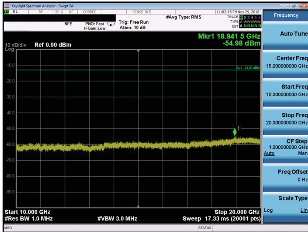
Plot 7-521. Conducted Spurious Plot (Band 66 – 20.0MHz QPSK – PCC 1/99 SCC 1/0 – Mid Channel)
