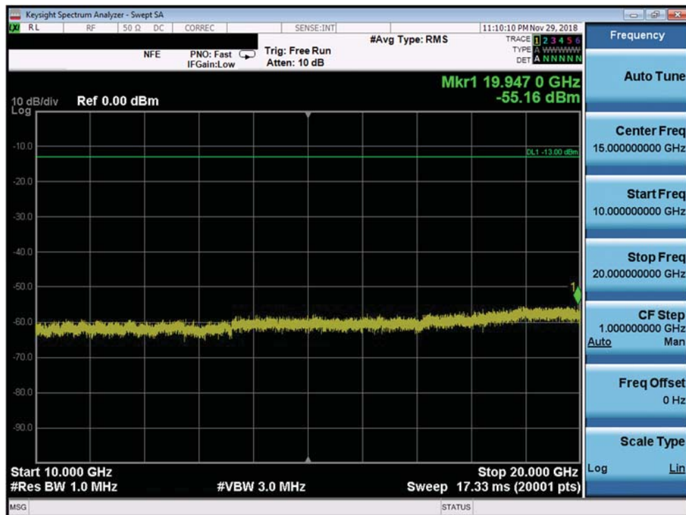
Plot 7-509. Conducted Spurious Plot Band 66 – 10.0MHz QPSK – PCC 1/49 SCC 1/0 – Mid Channel)
