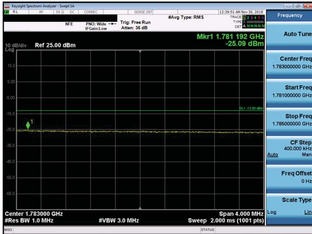
Plot 7-529. Extended Upper Band Edge Plot (Band 66 QPSK – PCC:20 MHz SCC:20 MHz – Full RB)
