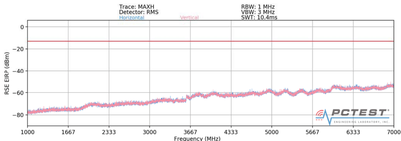
Plot 7-530. Radiated Spurious Plot above 1GHz (Band 71)
