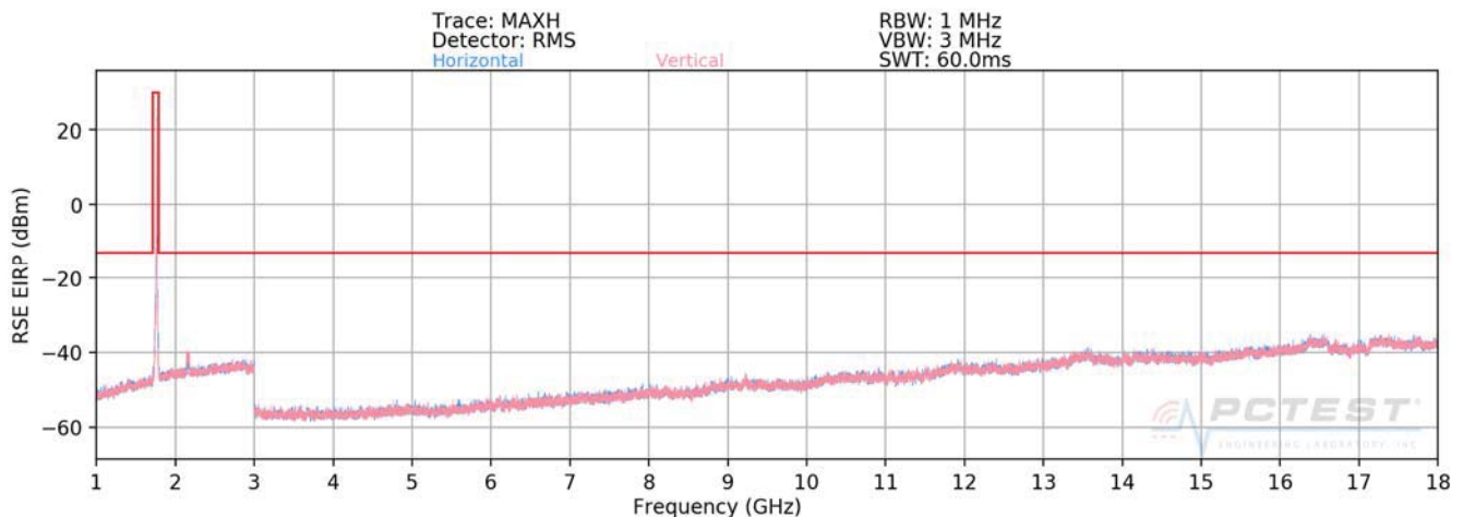
Plot 7-552. Radiated Spurious Plot (ULCA B66 PCC: RB 1 Offset 0, SCC: RB 1 Offset 99 – High Channel)
