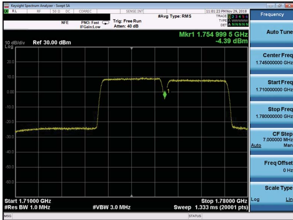
Plot 7-523. Conducted Spurious Plot (Band 66 – 20.0MHz QPSK – PCC 100/0 SCC 100/0 – Mid Channel)
