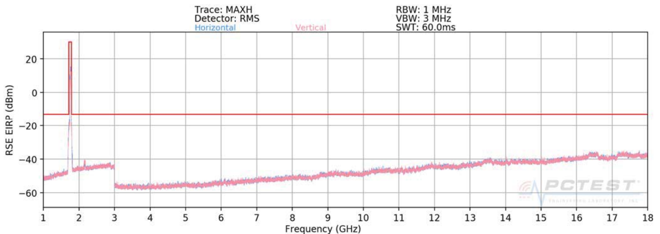
Plot 7-555. Radiated Spurious Plot (ULCA B66 PCC: RB 100 Offset 0, SCC: RB 100 Offset 0 – High Channel)
