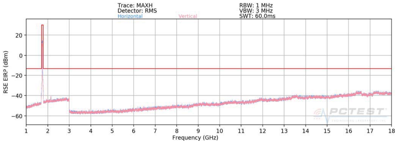
Plot 7-548. Radiated Spurious Plot (ULCA B66 PCC: RB 75 Offset 0, SCC: RB 25 Offset 0 – Mid Channel)
