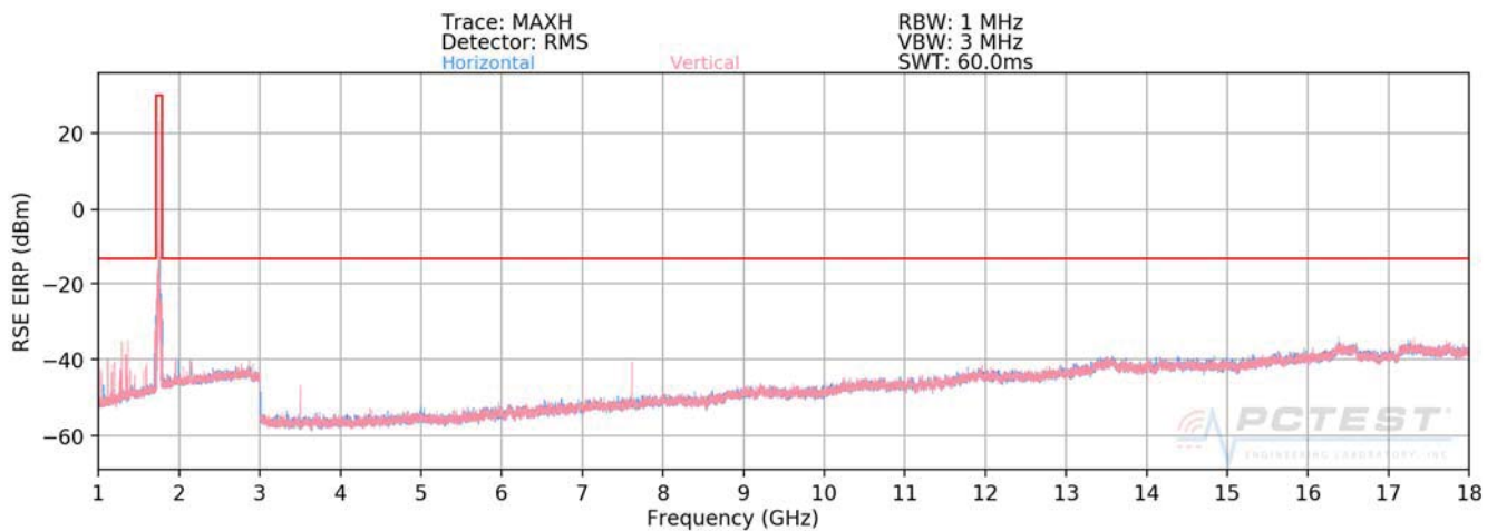
Plot 7-545. Radiated Spurious Plot (ULCA B66 PCC: RB 1 Offset 74, SCC: RB 1 Offset 0 – Mid Channel)
