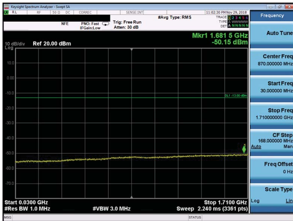
Plot 7-518. Conducted Spurious Plot (Band 66 – 20.0MHz QPSK – PCC 1/99 SCC 1/0 – Mid Channel)
