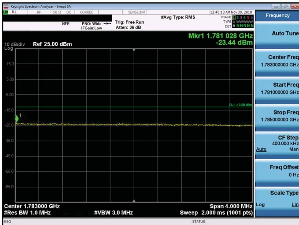
Plot 7-517. Extended Upper Band Edge Plot (Band 66 QPSK – PCC:15 MHz SCC:5 MHz – Full RB)
