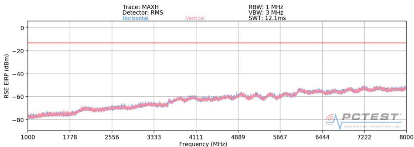
Plot 7-532. Radiated Spurious Plot above 1GHz (Band 13)
