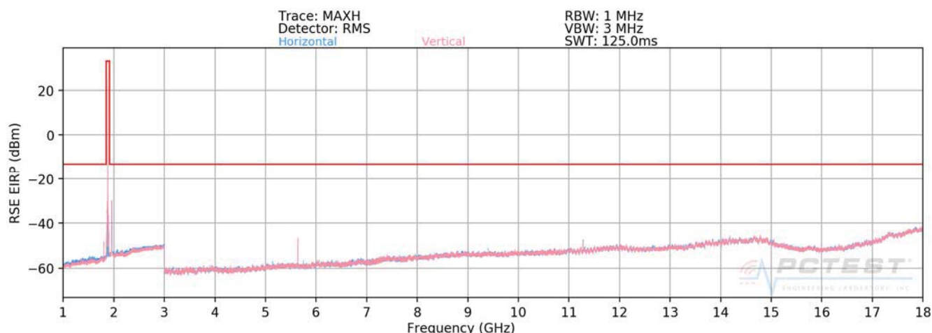
Plot 7-535. Radiated Spurious Plot above 1GHz (Band 25/2)
