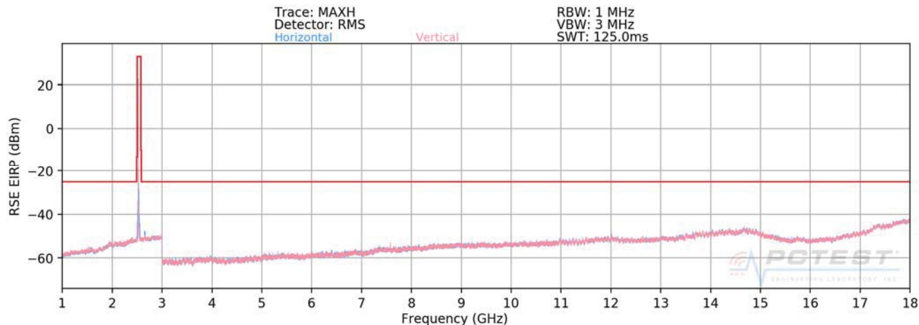
Plot 7-538. Radiated Spurious Plot above 1GHz (Band 7 Ant A)
