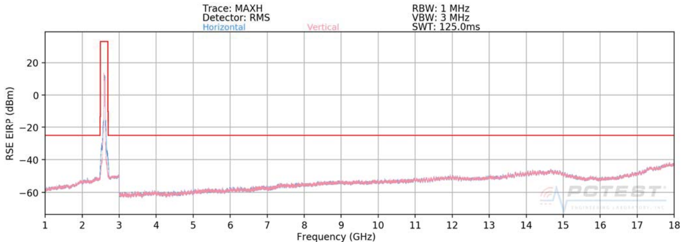
Plot 7-560. Radiated Spurious Plot (ULCA B41 PC2 PCC: RB 100 Offset 0, SCC: RB 100 Offset 0 – Mid Channel)
