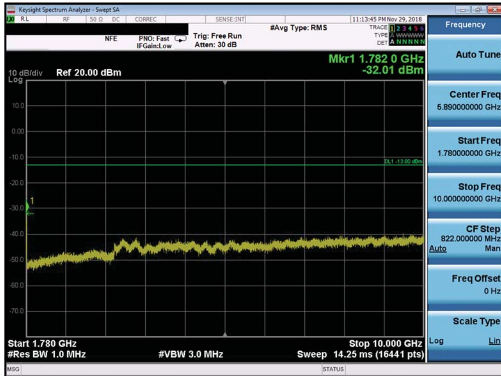
Plot 7-512. Conducted Spurious Plot (Band 66 – 10.0MHz QPSK – PCC 50/0 SCC 50/0 – Mid Channel)
