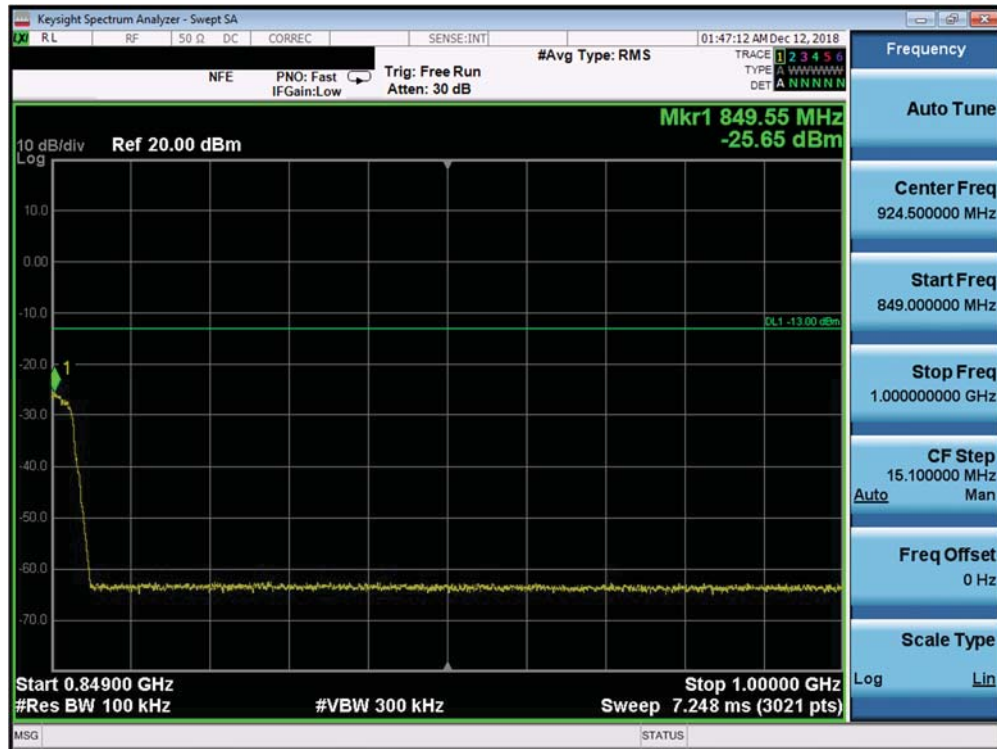
Plot 7-502. Conducted Spurious Plot (Band 5 – 10.0MHz QPSK – PCC 50/0 SCC 50/0 – Mid Channel)
