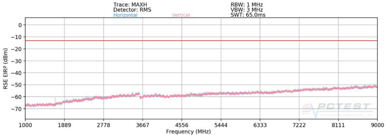
Plot 7-541. Radiated Spurious Plot (ULCA B5 PCC: RB 1 Offset 0, SCC: RB 1 Offset 49 – High Channel)
