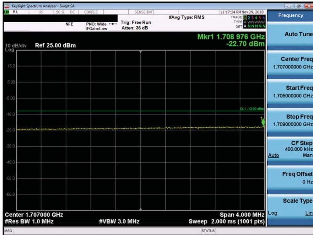
Plot 7-527. Extended Lower Band Edge Plot (Band 66 QPSK – PCC:20 MHz SCC:20 MHz – Full RB)
