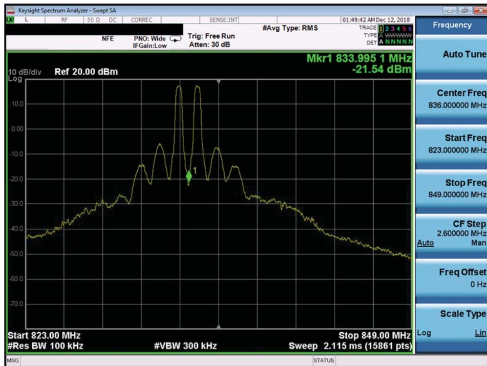
Plot 7-497. Conducted Spurious Plot (Band 5 – 10.0MHz QPSK – PCC 1/49 SCC 1/0 – Mid Channel)
