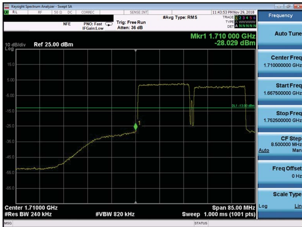
Plot 7-526. Lower Band Edge Plot (Band 66 QPSK – PCC:20 MHz SCC:20 MHz – Full RB)
