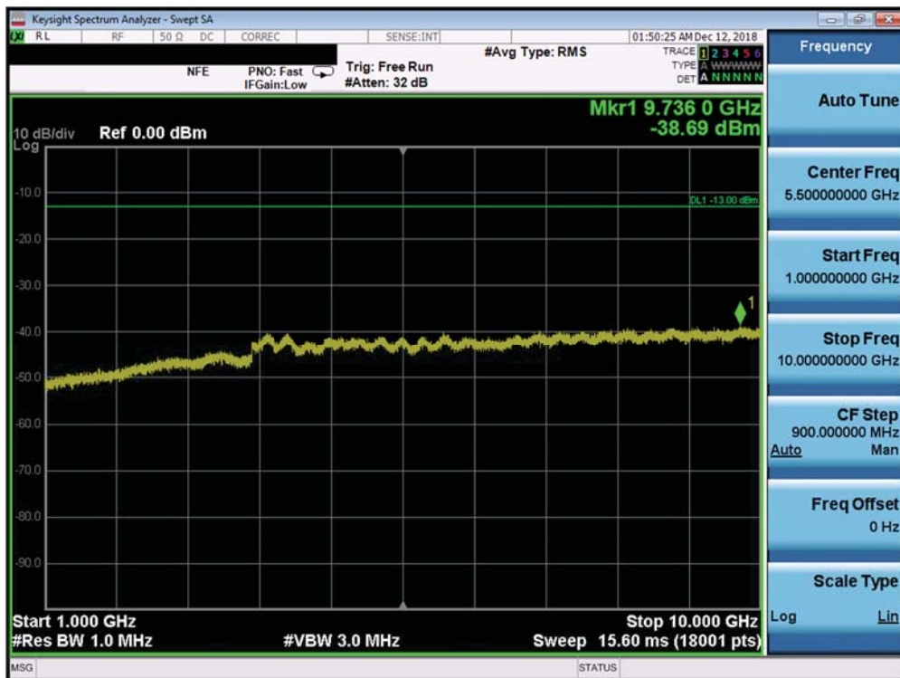
Plot 7-499. Conducted Spurious Plot (Band 5 – 10.0MHz QPSK – PCC 1/49 SCC 1/0 – Mid Channel)
