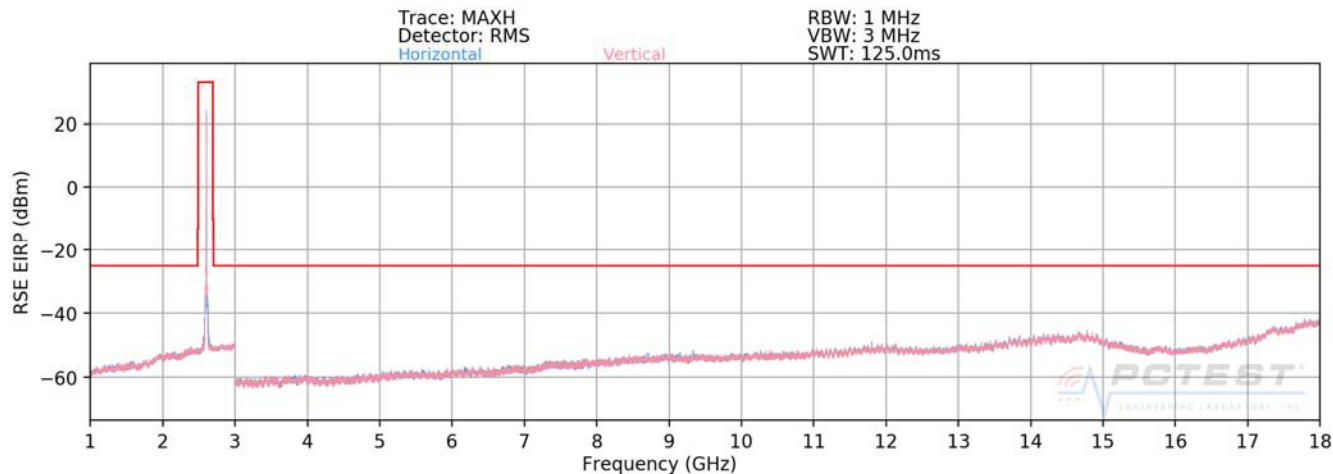
Plot 7-539. Radiated Spurious Plot above 1GHz (Band 41 PC2)
