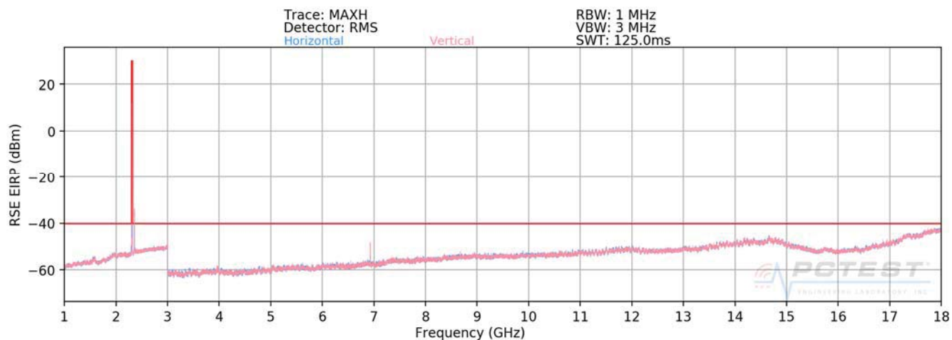
Plot 7-536. Radiated Spurious Plot above 1GHz (Band 30)
