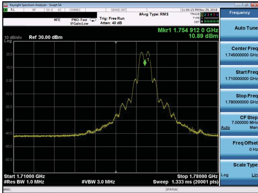
Plot 7-519. Conducted Spurious Plot (Band 66 – 20.0MHz QPSK – PCC 1/99 SCC 1/0 – Mid Channel)
