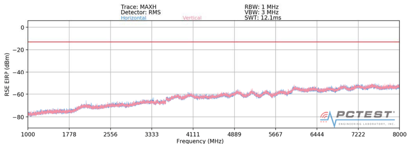
Plot 7-531. Radiated Spurious Plot above 1GHz (Band 12)
