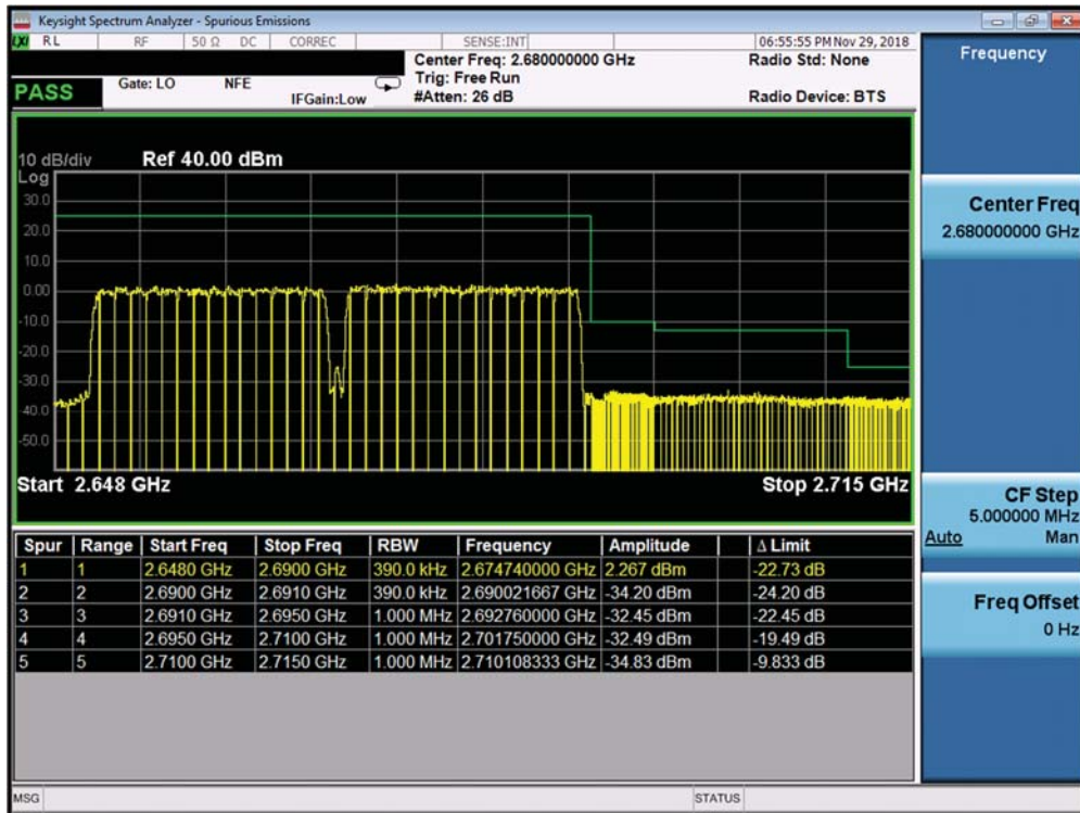
Plot 7-495. Upper Band Edge Plot (Band 41 QPSK – PC3 – PCC:20 MHz SCC:20 MHz – Full RB)
