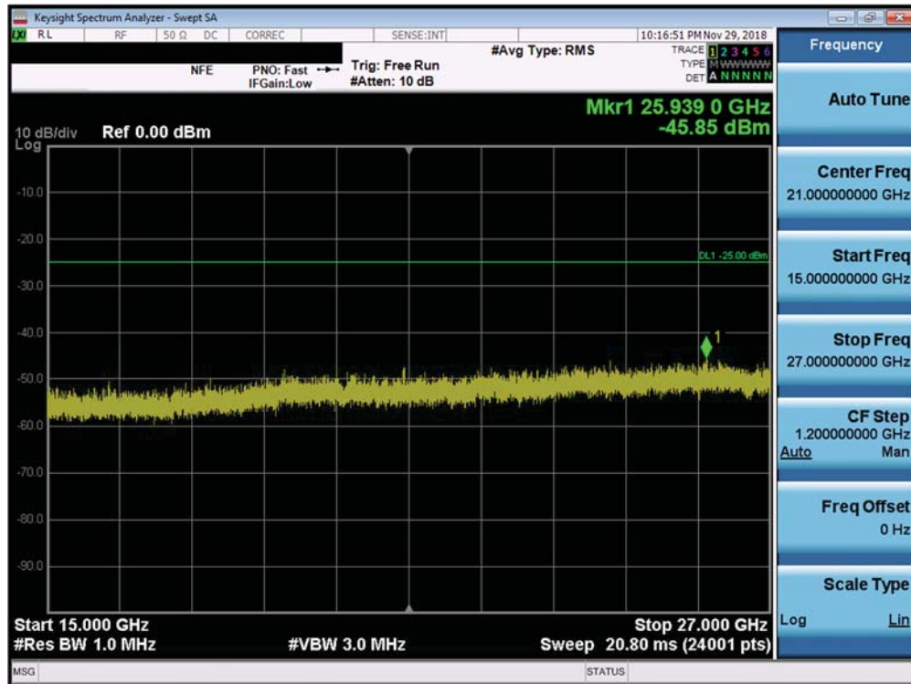
Plot 7-489. Conducted Spurious Plot (Band 41 – PC3 – 20.0MHz QPSK – PCC 1/99 SCC 1/0 – Mid Channel)
