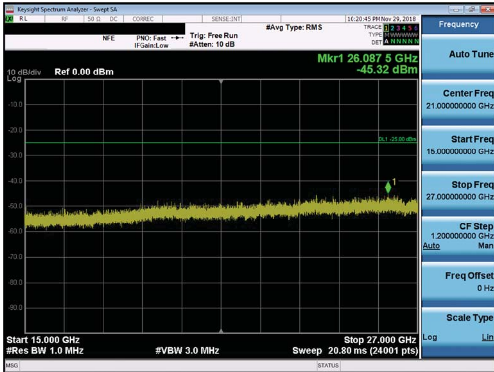
Plot 7-493. Conducted Spurious Plot (Band 41 – PC3 – 20.0MHz QPSK – PCC 100/0 SCC 100/0 – Mid Channel)
