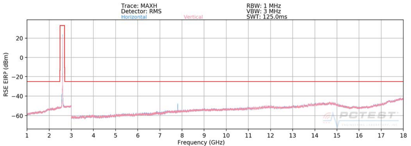
Plot 7-557. Radiated Spurious Plot (ULCA B41 PC2 PCC: RB 1 Offset 99, SCC: RB 1 Offset 0 – Mid Channel)
