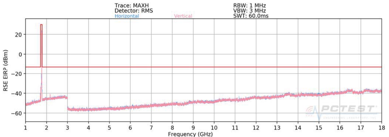
Plot 7-546. Radiated Spurious Plot (ULCA B66 PCC: RB 1 Offset 0, SCC: RB 1 Offset 24 – High Channel)
