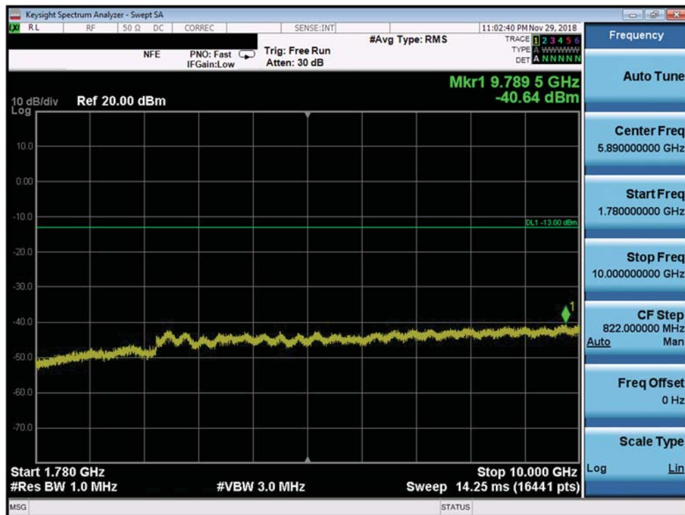
Plot 7-520. Conducted Spurious Plot (Band 66 – 20.0MHz QPSK – PCC 1/99 SCC 1/0 – Mid Channel)
