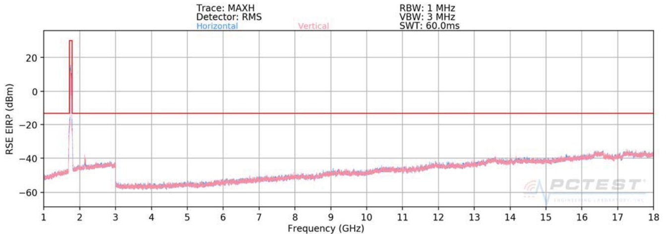
Plot 7-554. Radiated Spurious Plot (ULCA B66 PCC: RB 100 Offset 0, SCC: RB 100 Offset 0 – Mid Channel)
