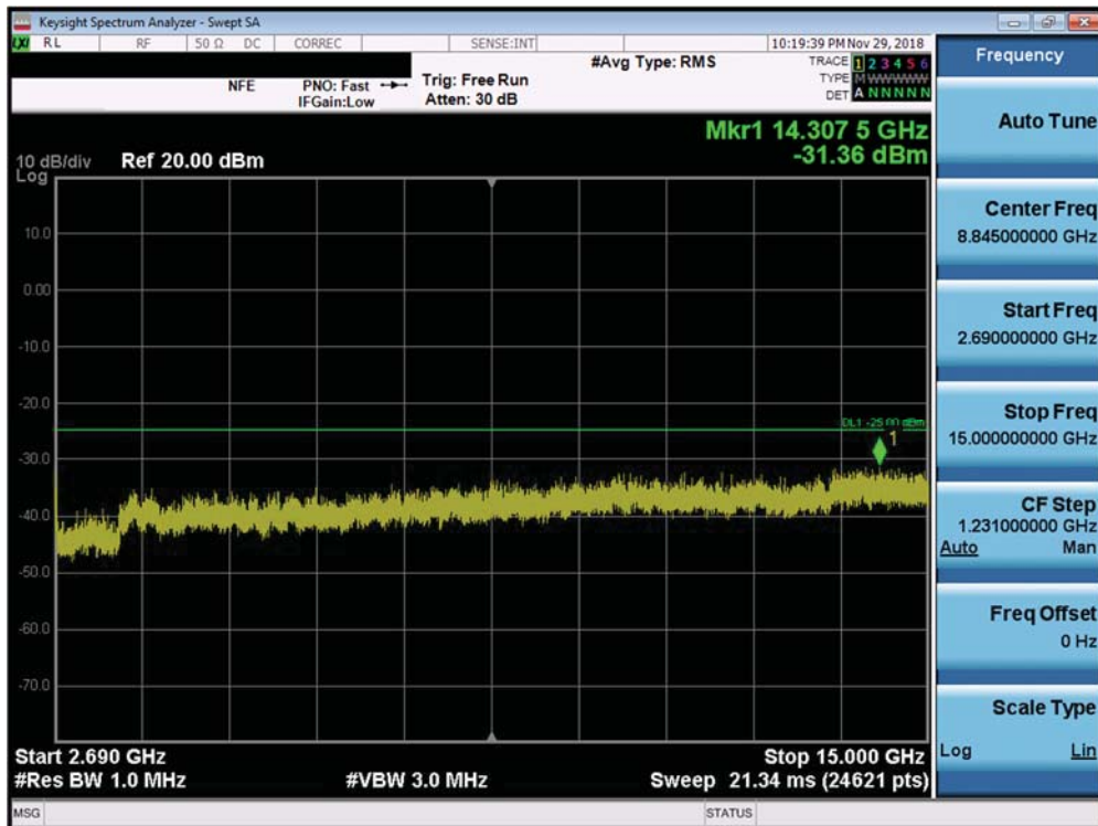
Plot 7-492. Conducted Spurious Plot (Band 41 – PC3 – 20.0MHz QPSK – PCC 100/0 SCC 100/0 – Mid Channel)
