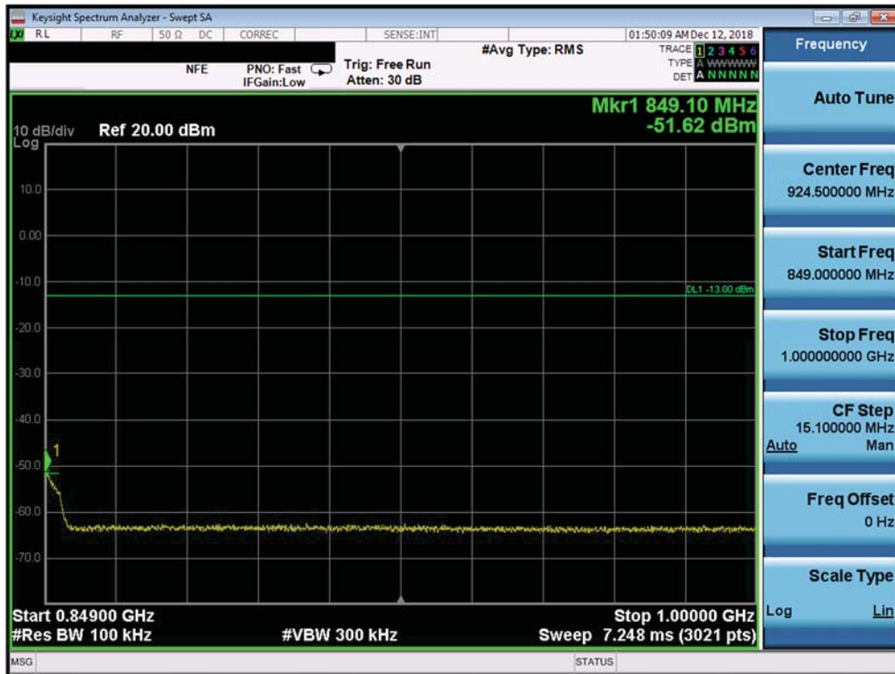
Plot 7-498. Conducted Spurious Plot (Band 5 – 10.0MHz QPSK – PCC 1/49 SCC 1/0 – Mid Channel)
