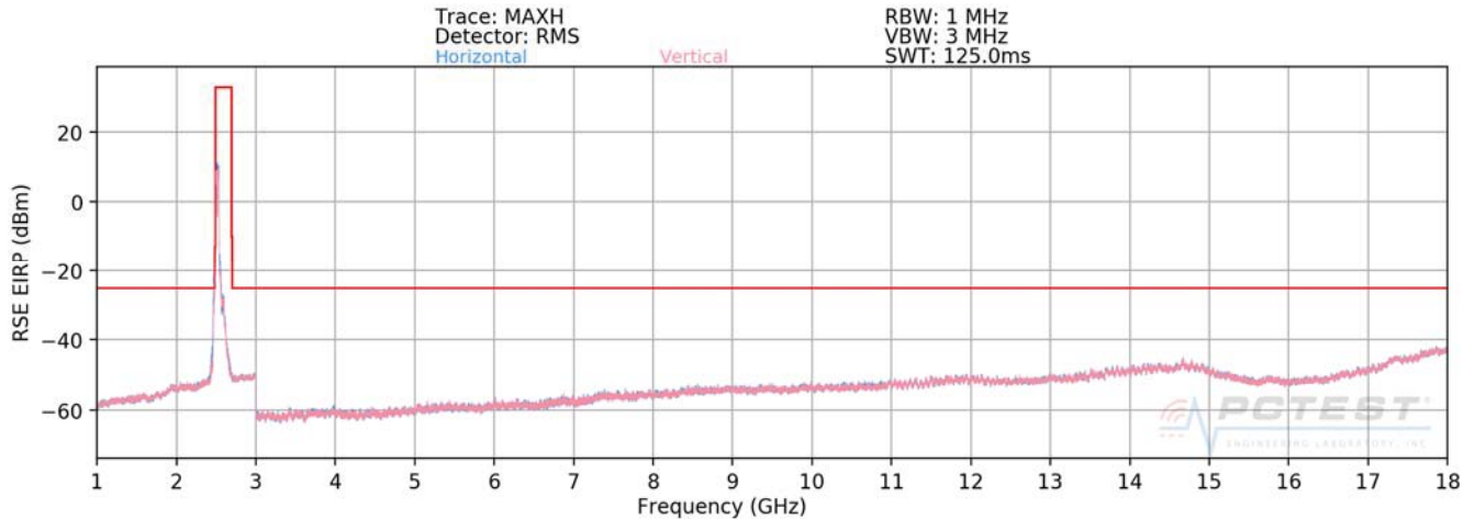
Plot 7-559. Radiated Spurious Plot (ULCA B41 PC2 PCC: RB 100 Offset 0, SCC: RB 100 Offset 0 – Low Channel)
