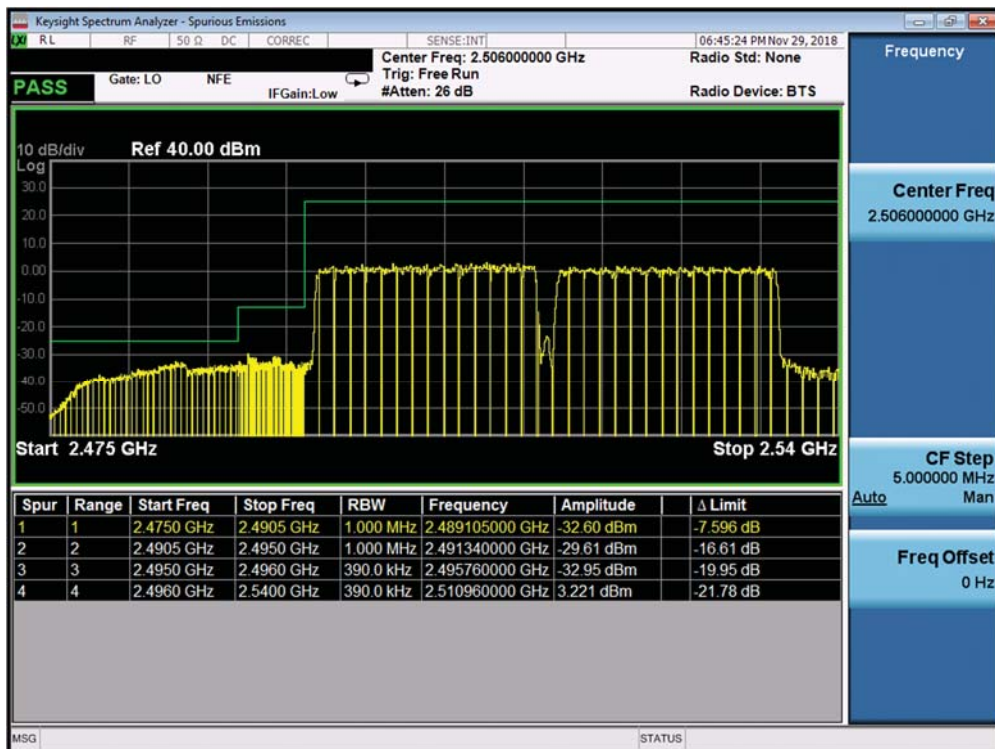
Plot 7-494. Lower Band Edge Plot (Band 41 QPSK – PC3 – PCC:20 MHz SCC:20 MHz – Full RB)
