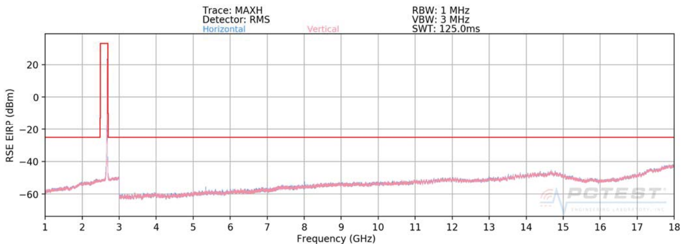
Plot 7-558. Radiated Spurious Plot (ULCA B41 PC2 PCC: RB 1 Offset 0, SCC: RB 1 Offset 99 – High Channel)
