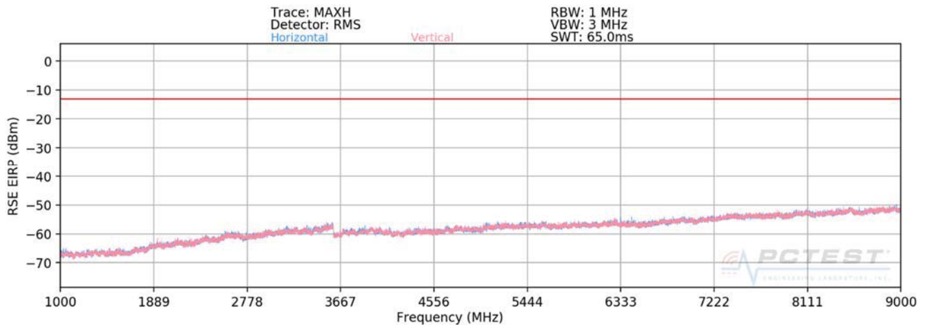
Plot 7-542. Radiated Spurious Plot (ULCA B5 PCC: RB 50 Offset 0, SCC: RB 50 Offset 0 – Low Channel)
