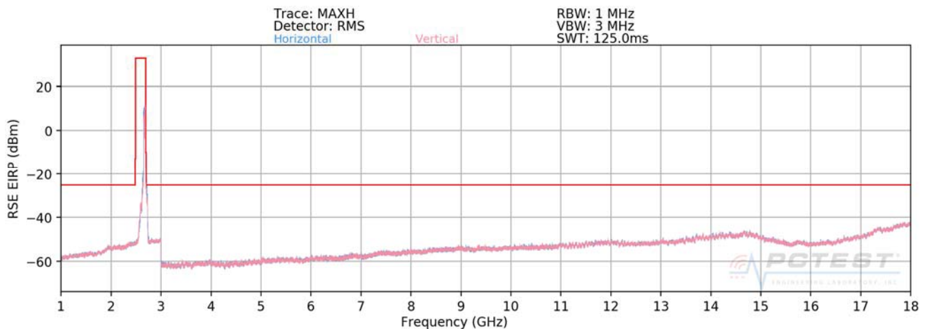
Plot 7-567. Radiated Spurious Plot (ULCA B41 PC3 PCC: RB 100 Offset 0, SCC: RB 100 Offset 0 – High Channel)
