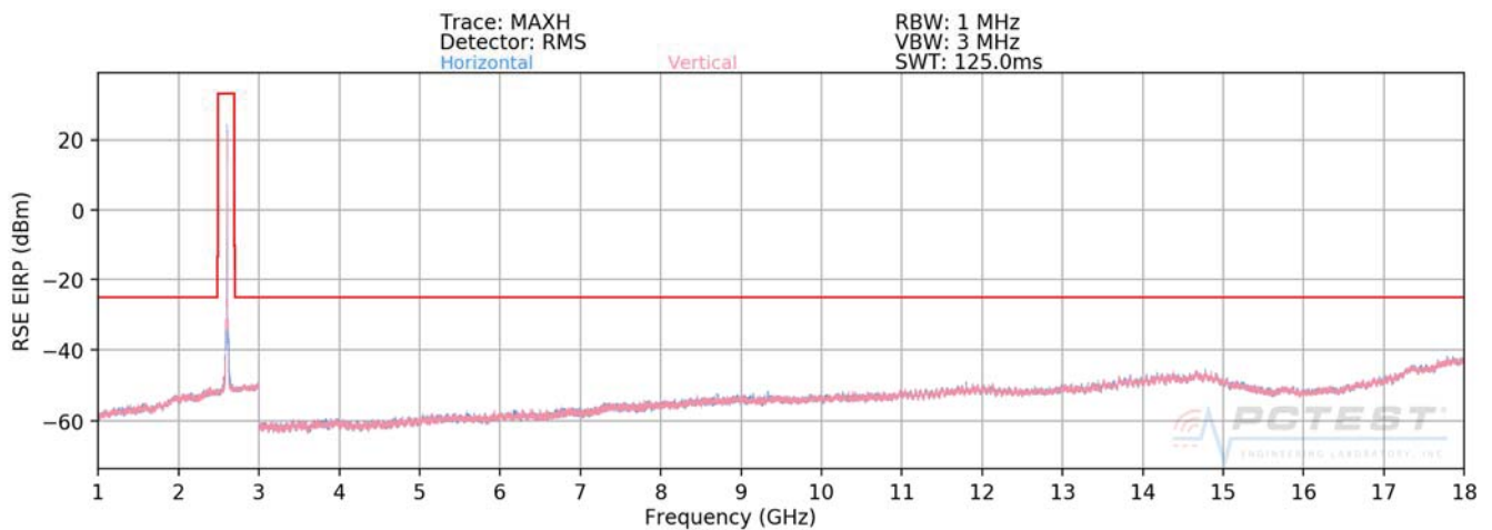
Plot 7-563. Radiated Spurious Plot (ULCA B41 PC3 PCC: RB 1 Offset 99, SCC: RB 1 Offset 0 – Mid Channel)
