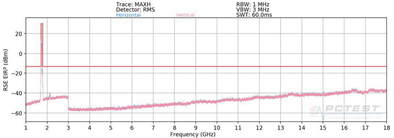
Plot 7-553. Radiated Spurious Plot (ULCA B66 PCC: RB 100 Offset 0, SCC: RB 100 Offset 0 – Low Channel)
