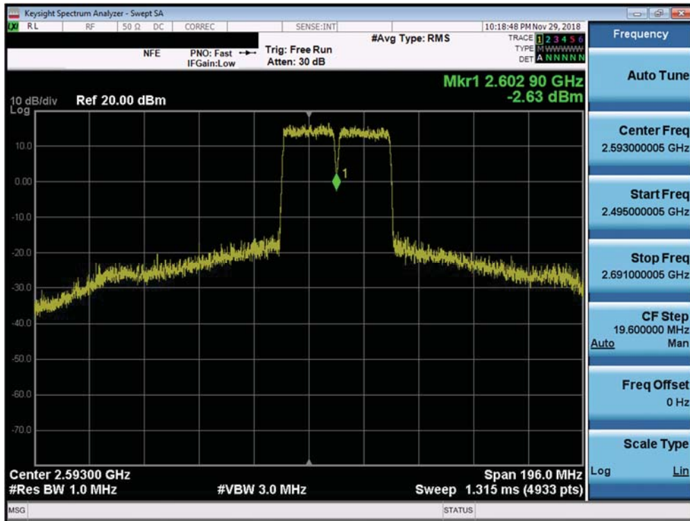
Plot 7-491. Conducted Spurious Plot (Band 41 – PC3 – 20.0MHz QPSK – PCC 100/0 SCC 100/0 – Mid Channel)
