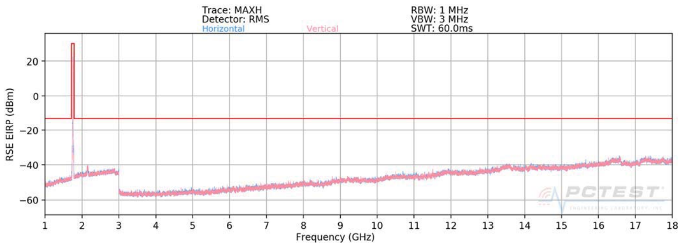
Plot 7-551. Radiated Spurious Plot (ULCA B66 PCC: RB 1 Offset 99, SCC: RB 1 Offset 0 – Mid Channel)
