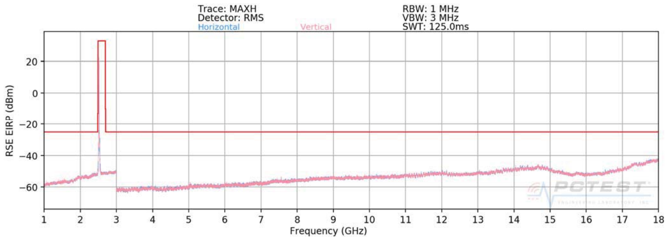
Plot 7-562. Radiated Spurious Plot (ULCA B41 PC3 PCC: RB 1 Offset 99, SCC: RB 1 Offset 0 – Low Channel)
