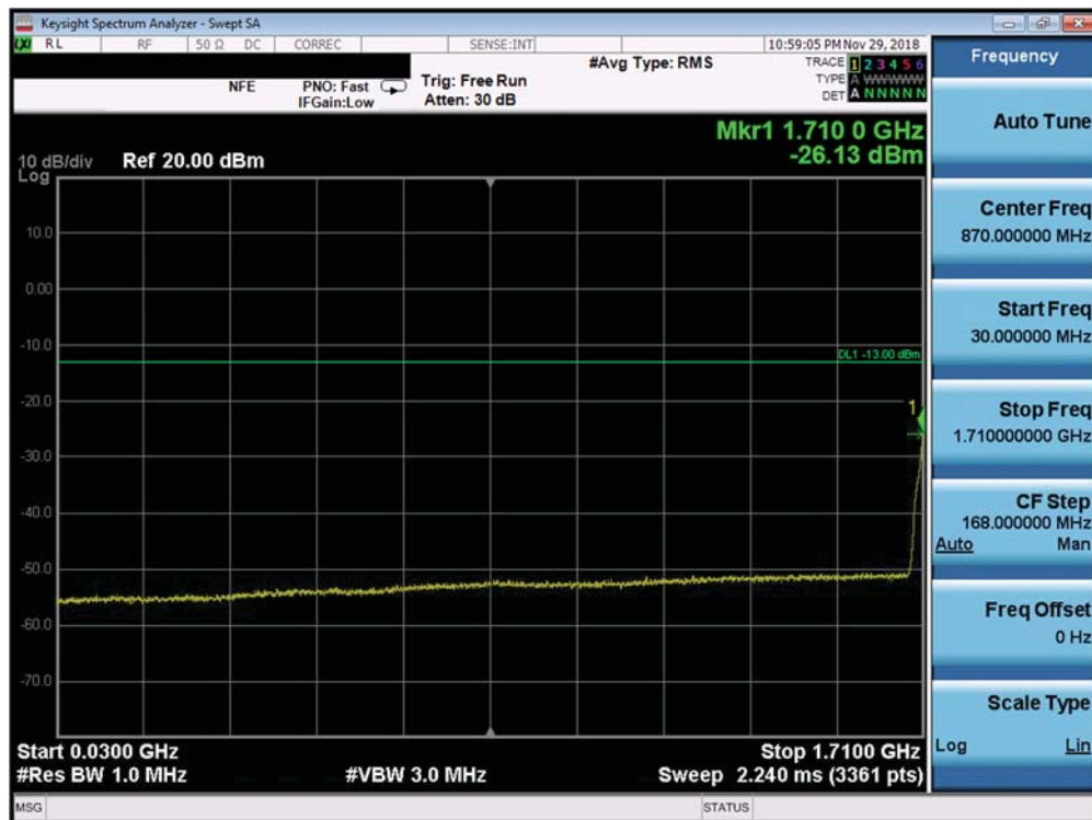
Plot 7-522. Conducted Spurious Plot (Band 66 – 20.0MHz QPSK – PCC 100/0 SCC 100/0 – Mid Channel)
