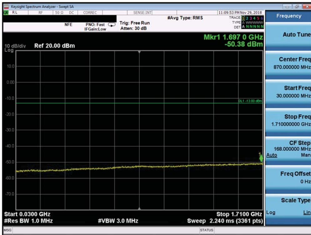
Plot 7-506. Conducted Spurious Plot (Band 66 – 10.0MHz QPSK – PCC 1/49 SCC 1/0 – Mid Channel)
