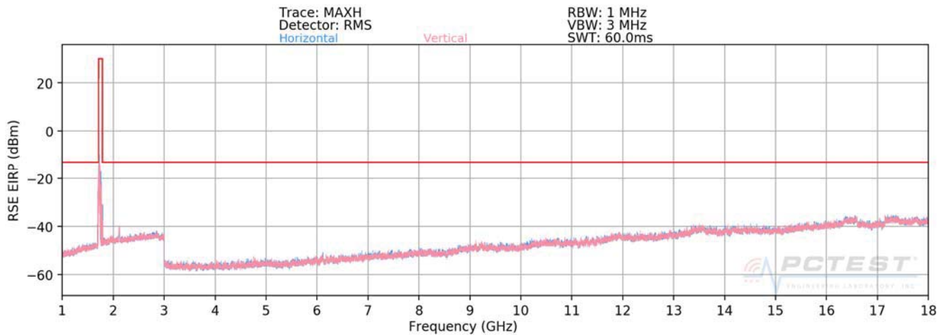
Plot 7-544. Radiated Spurious Plot (ULCA B66 PCC: RB 1 Offset 74, SCC: RB 1 Offset 0 – Low Channel)
