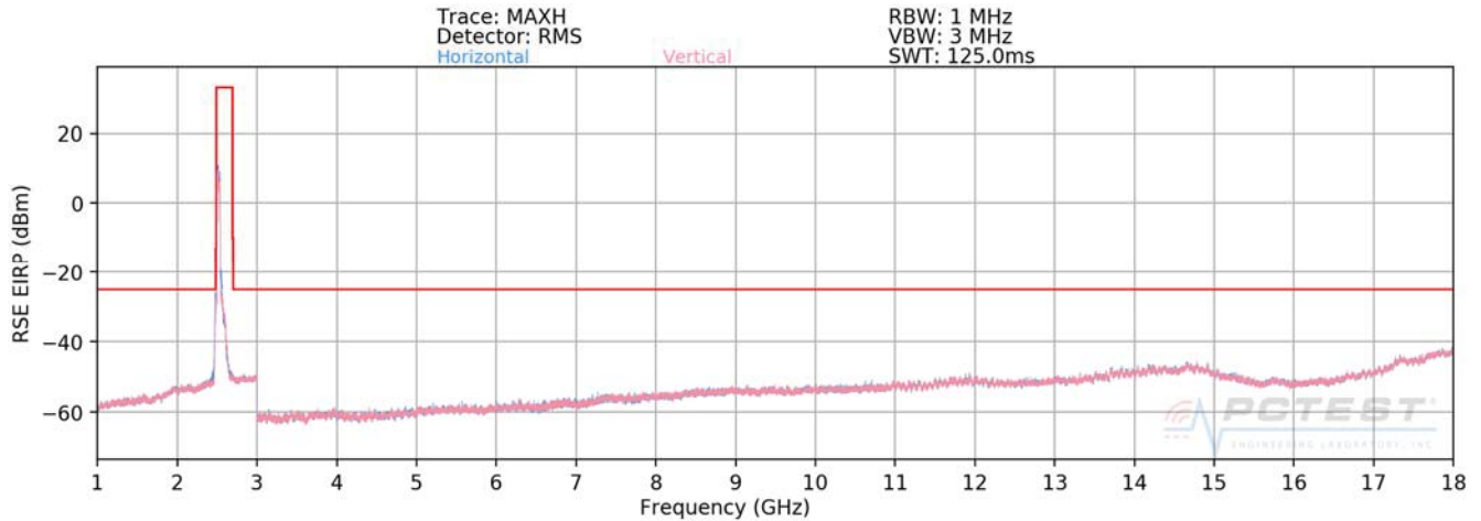
Plot 7-565. Radiated Spurious Plot (ULCA B41 PC3 PCC: RB 100 Offset 0, SCC: RB 100 Offset 0 – Low Channel)
