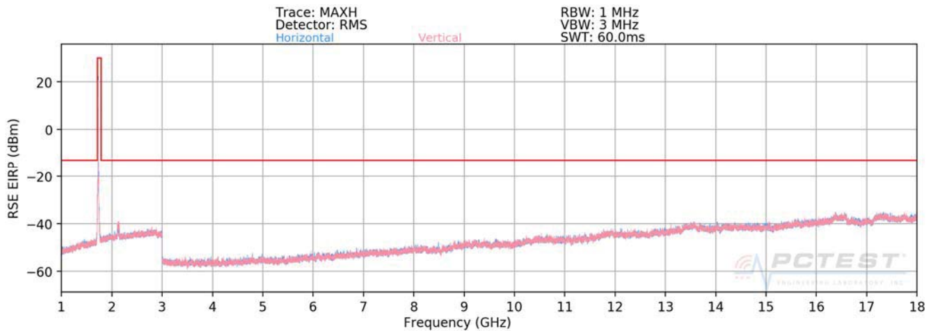
Plot 7-550. Radiated Spurious Plot (ULCA B66 PCC: RB 1 Offset 99, SCC: RB 1 Offset 0 – Low Channel)
