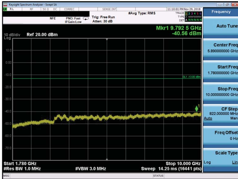
Plot 7-508. Conducted Spurious Plot Band 66 – 10.0MHz QPSK – PCC 1/49 SCC 1/0 – Mid Channel)
