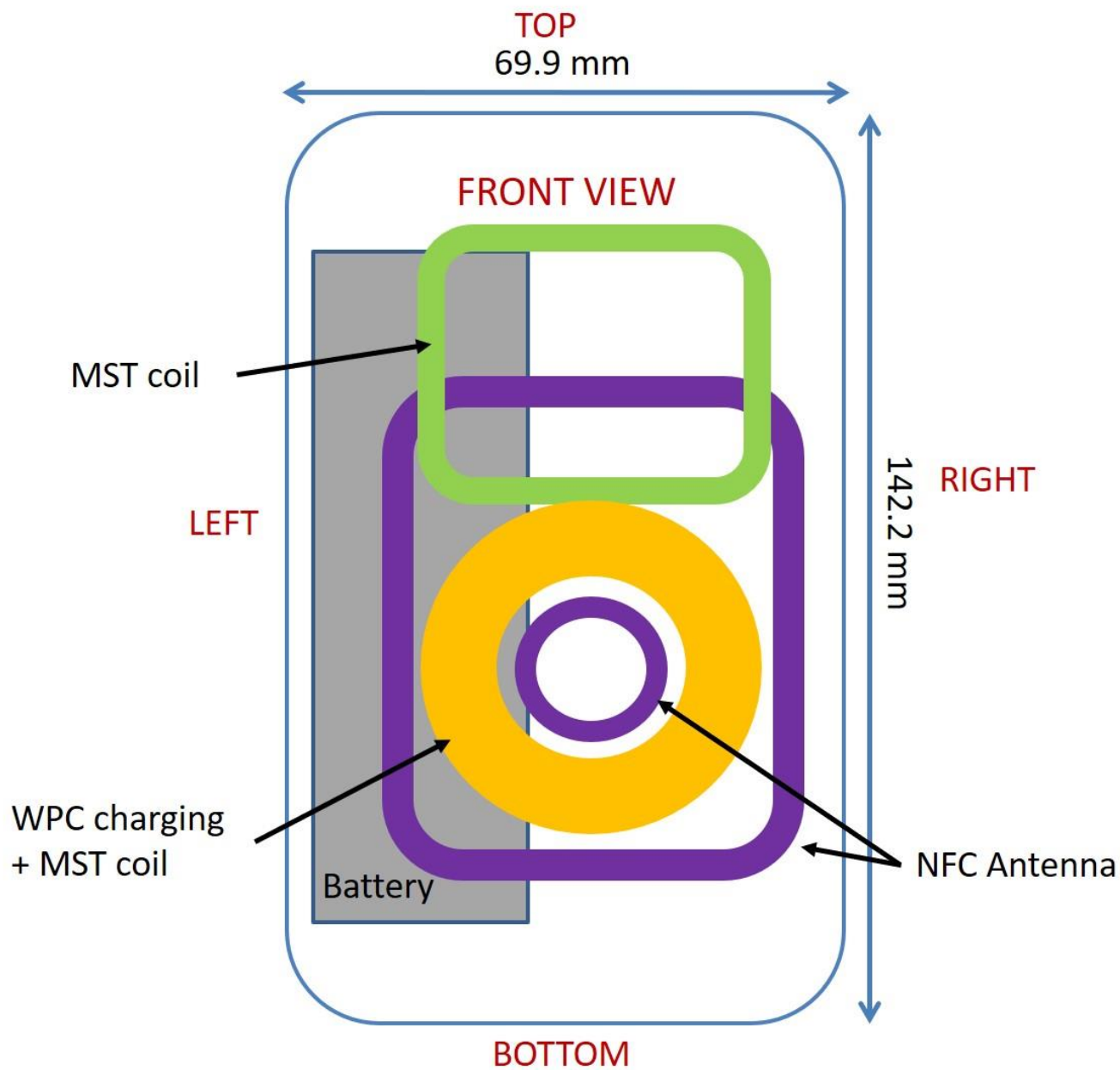
Figure F-2 NFC Antenna Locations
