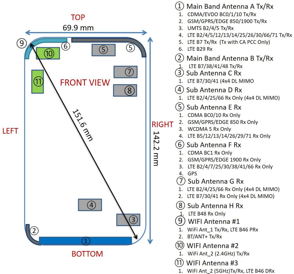
Figure F-1 DUT Antenna Locations
