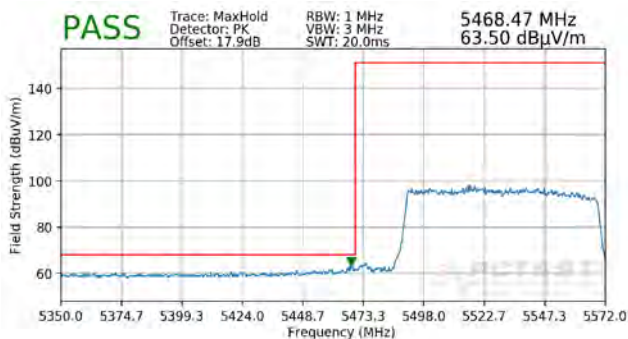
Plot 7-756. Radiated Band Edge Plot SISO ANT2 (Peak – WCP – 996 Tones)
