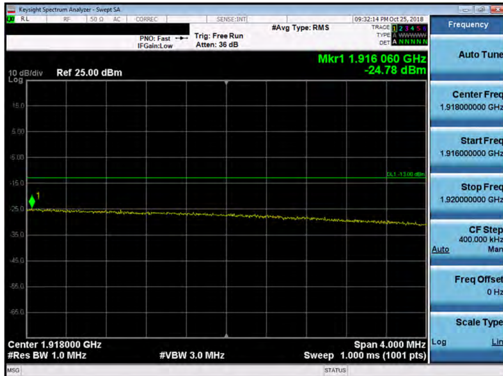
Plot 7-203. Upper Extended Band Edge Plot (Band 25/2 - 20.0MHz QPSK - Full RB Configuration)
