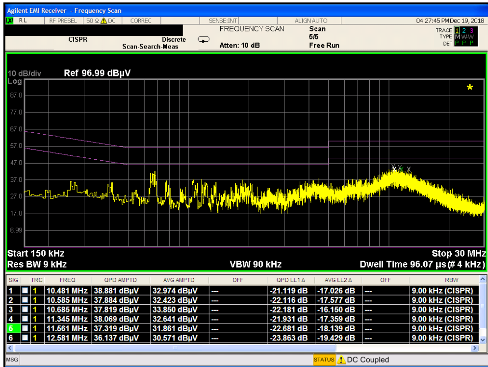
Plot 7-6. Line-Conducted Test Plot (L1) – with Antenna Terminated in 50Ω
