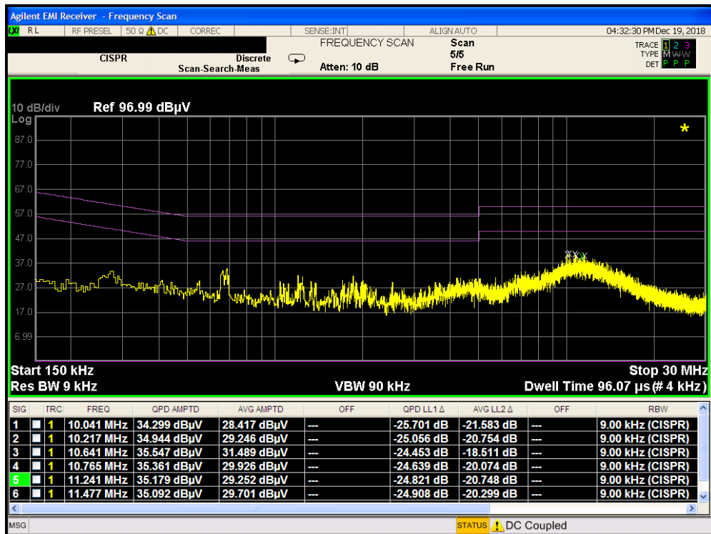
Plot 7-7. Line-Conducted Test Plot (N) – with Antenna Terminated in 50Ω
