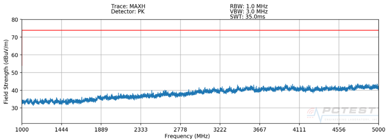
Plot 7-2. Radiated Spurious Plot above 1GHz – H
