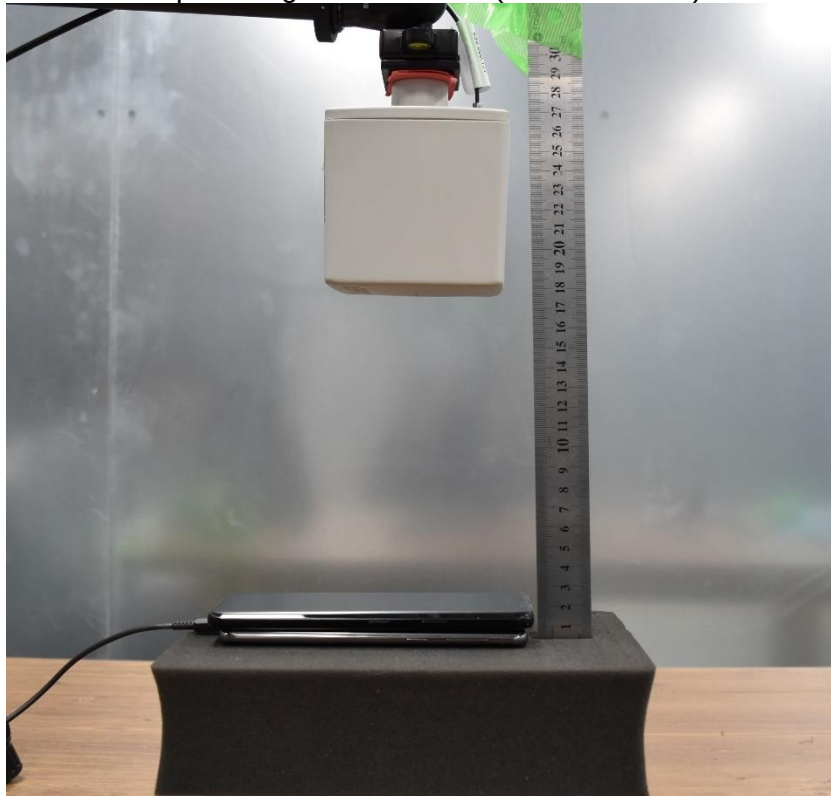
Top – charger below client (20cm distance)
