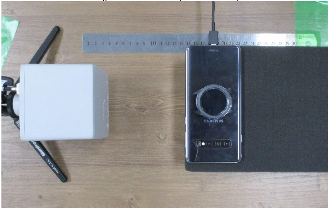
Edge2 with USB cable (15cm distance)
