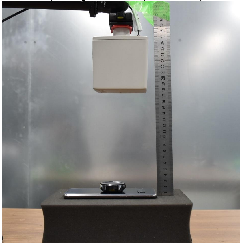
Top – charger below client (20cm distance)
