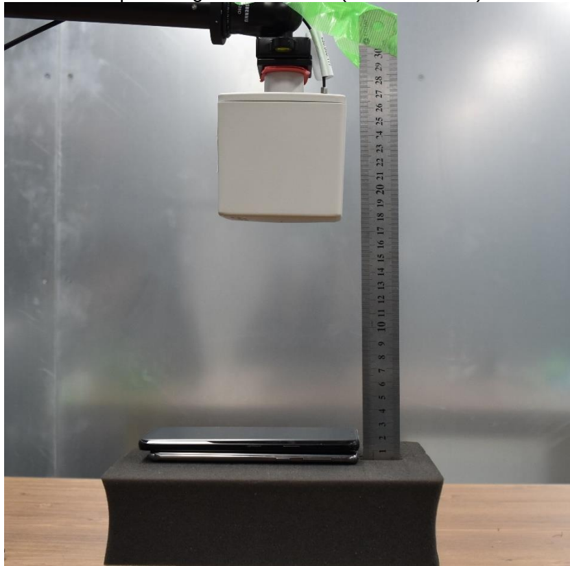
Top – charger above client (20cm distance)
