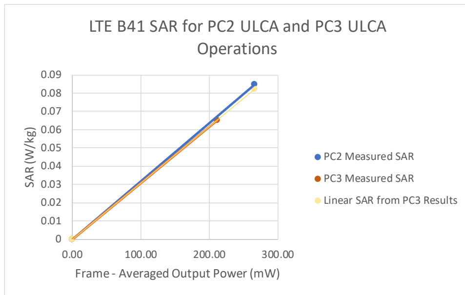
Figure 14-2 LTE Band 41 Head Linearity
