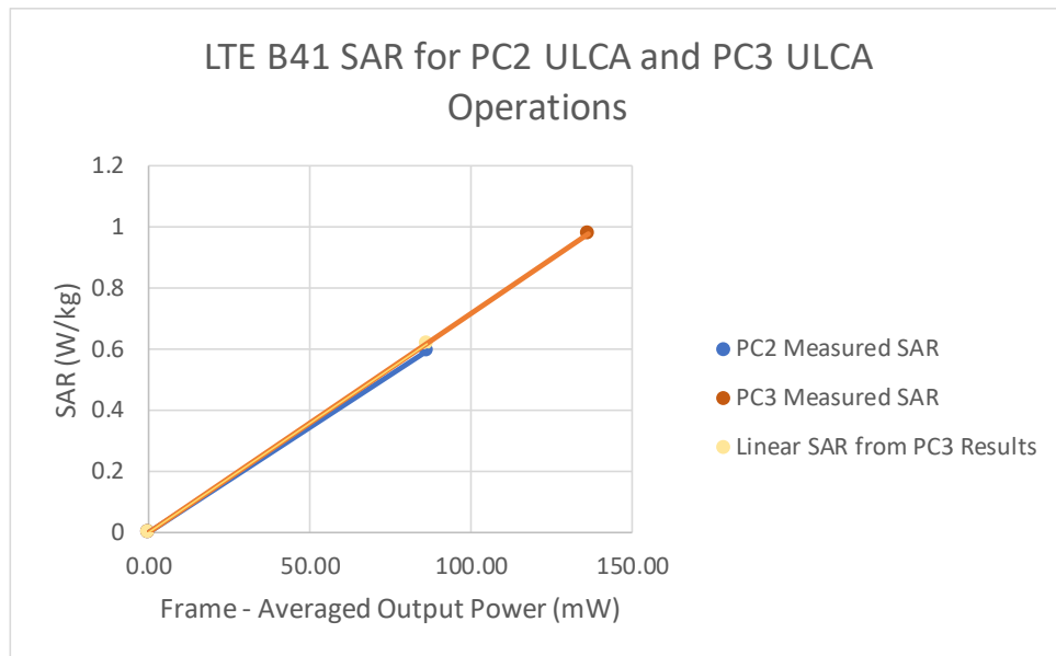
Figure 14-6 LTE Band 41 Hotspot Linearity
