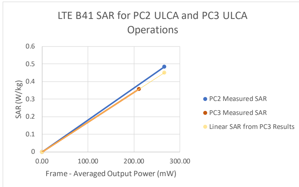
Figure 14-4 LTE Band 41 Body-Worn Linearity
