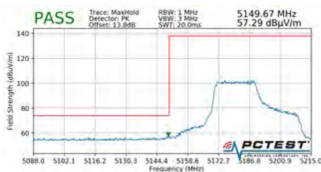
Plot 7-726. Radiated Lower Band Edge Plot SISO ANT2 (Peak – UNII Band 1 – 242 Tones)
