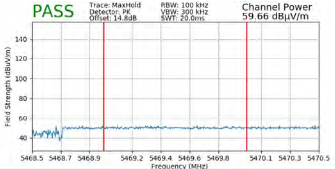
Plot 7-673. Radiated Lower Band Edge Plot SISO ANT1 (Peak - UNII Band 2C - 242 Tones)
