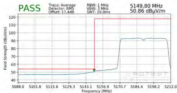
Plot 7-787. Radiated Band Edge Plot MIMO (Average – WCP – 484 Tones)
