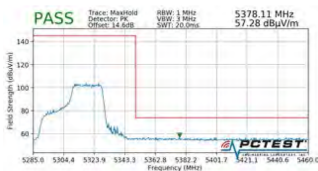
Plot 7-728. Radiated Upper Band Edge Plot SISO ANT2 (Peak – UNII Band 2A – 242 Tones)
