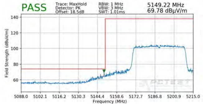
Plot 7-357. Radiated Band Edge Plot ANT (Peak – WCP)
