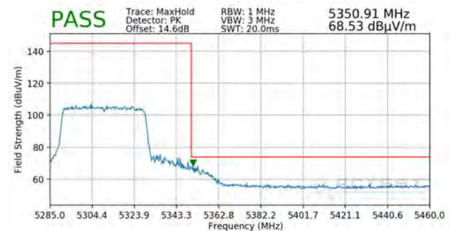
Plot 7-352. Radiated Upper Band Edge Plot MIMO (Peak – UNII Band 2A)
