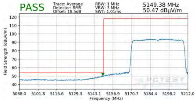
Plot 7-356. Radiated Band Edge Plot ANT (Average – WCP)
