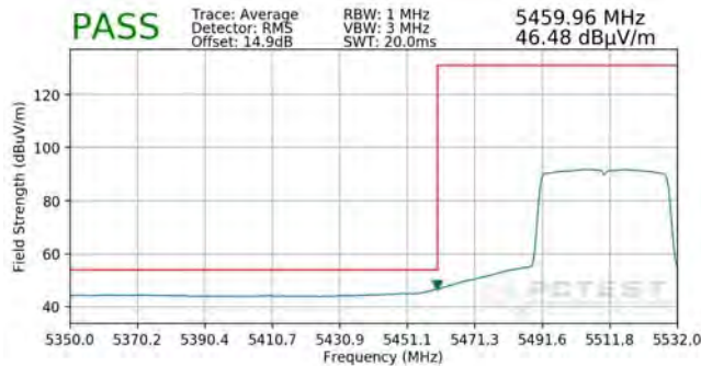
Plot 7-353. Radiated Lower Band Edge Plot MIMO (Average – UNII Band 2C)
