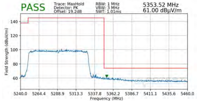
Plot 7-366. Radiated Band Edge Plot ANT (Peak – WCP)
