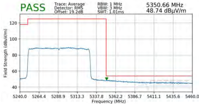
Plot 7-365. Radiated Band Edge Plot ANT (Average – WCP)
