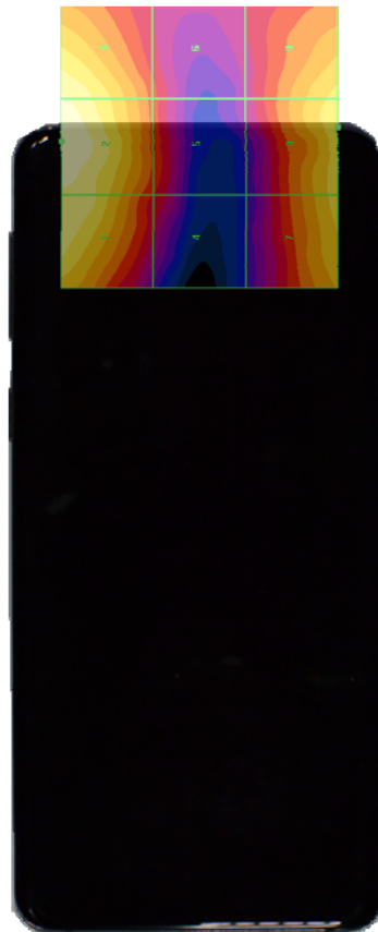
Figure 18-4 E-Field WD Scan overlay
