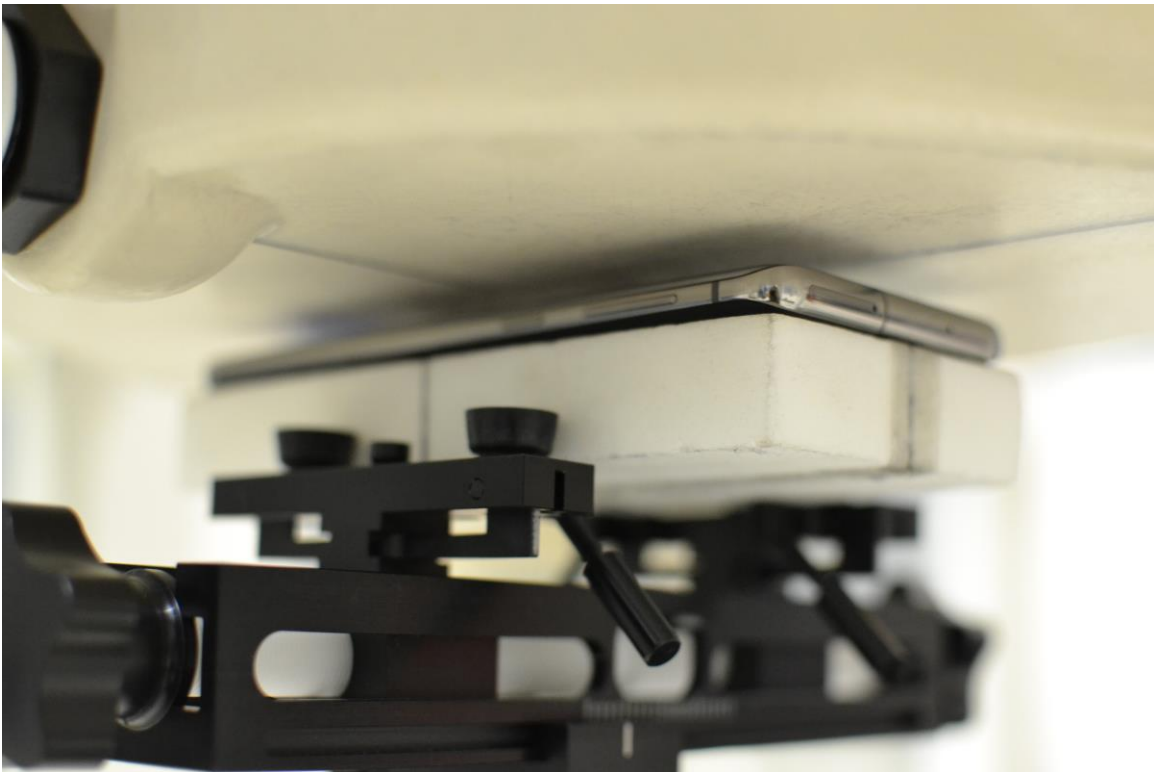
SAR Test Setup Photo 8 – Back Side at 6 mm
