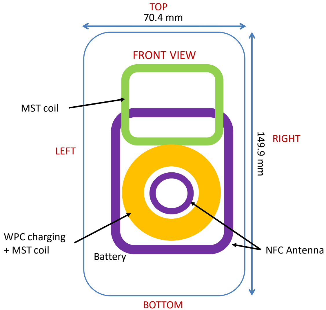
Figure F-2 NFC Antenna Locations
