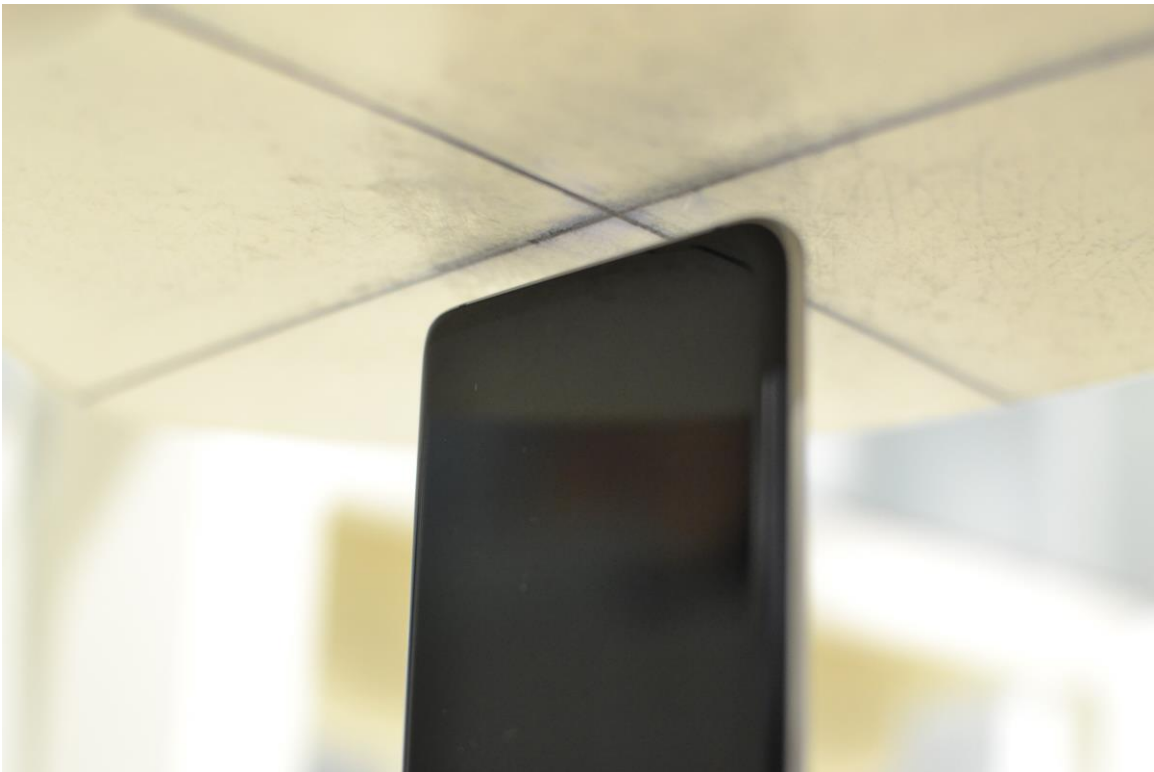
SAR Test Setup Photo 16 – Bottom Side at 8 mm
