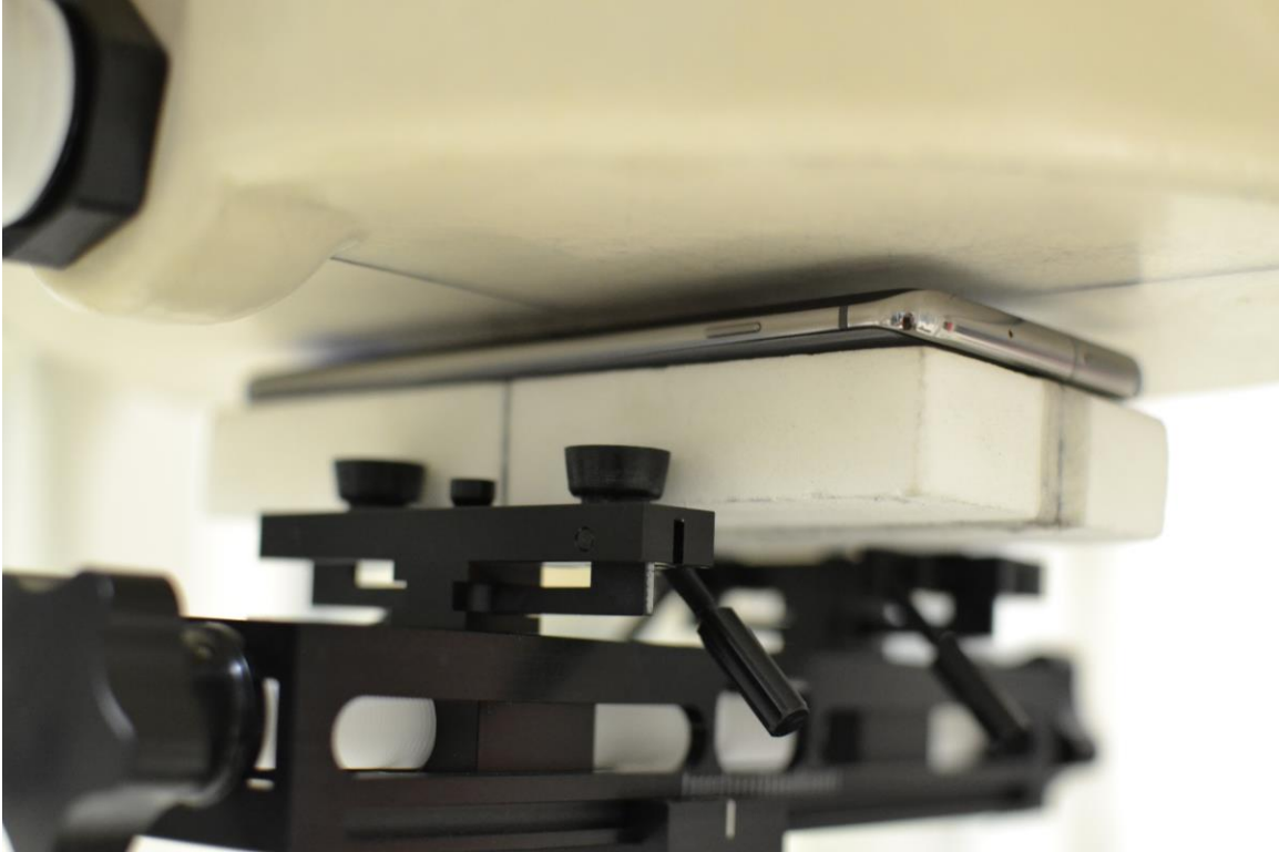
SAR Test Setup Photo 11 – Front Side at 4 mm
