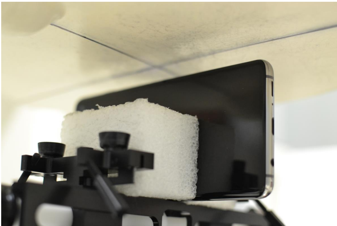
SAR Test Setup Photo 18 – Right Side at 10 mm
