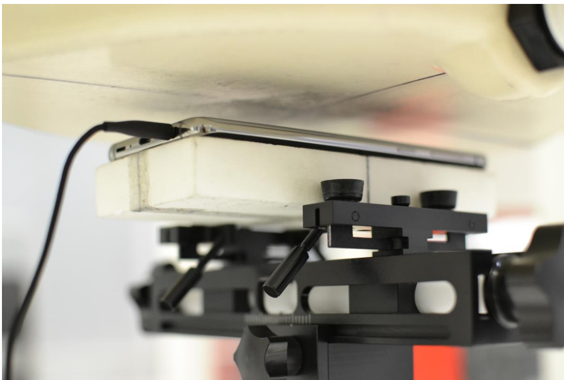
SAR Test Setup Photo 6 – Back Side with Headphone inserted at 15 mm
