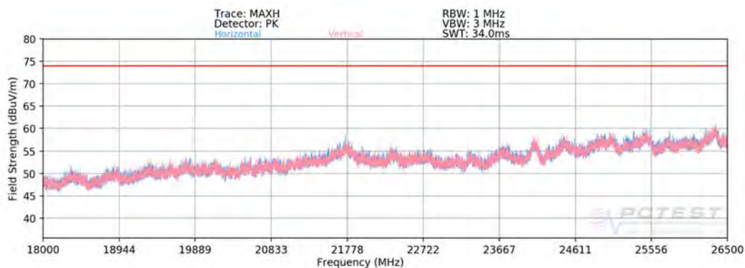
Plot 7-635. Radiated Spurious Plot 18GHz - 26.5GHz SISO ANT1 (802.11ax – 242 Tones)
