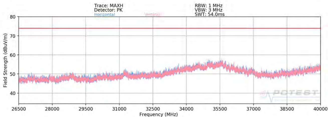
Plot 7-660. Radiated Spurious Plot 26.5GHz - 40GHz MIMO (802.11ax – 242 Tones)
