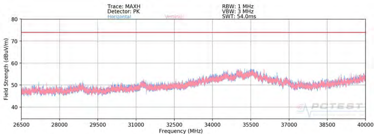
Plot 7-648. Radiated Spurious Plot 26.5GHz - 40GHz SISO ANT2 (802.11ax – 242 Tones)
