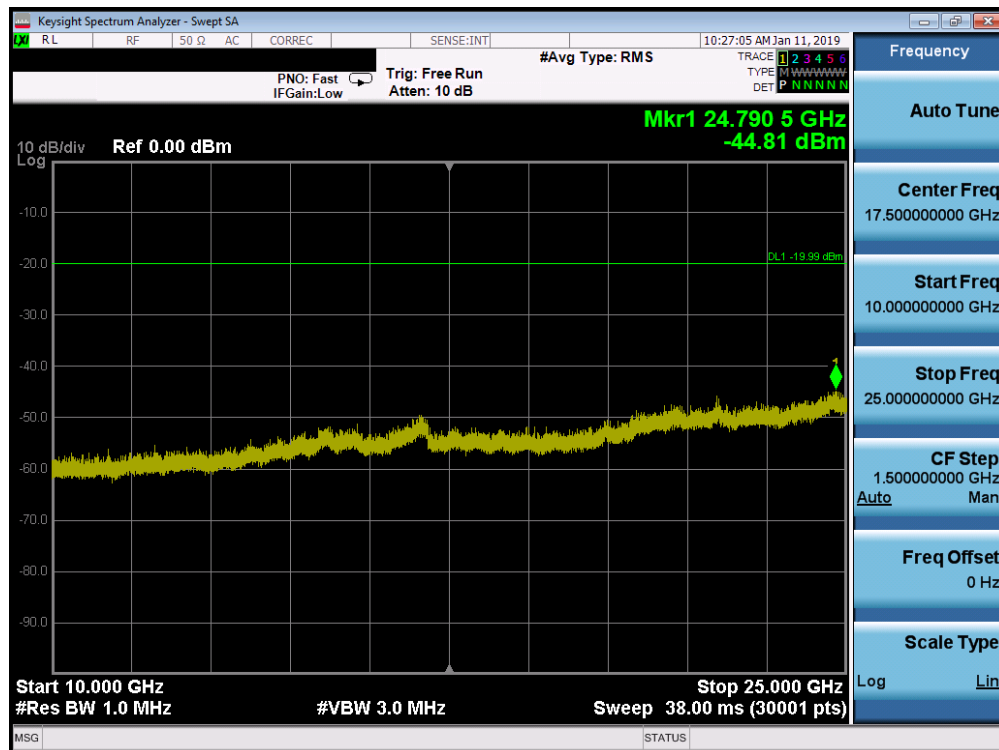
Plot 7-90. Conducted Spurious Plot SISO ANT1 (802.11ax OFDMA– 26 Tones – Ch. 1)
