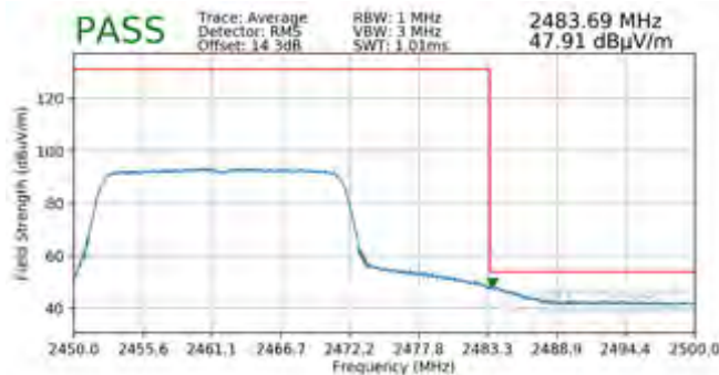
Plot 7-175. Radiated Restricted Upper Band Edge Measurement SISO ANT1 (Average – 242 Tones)
