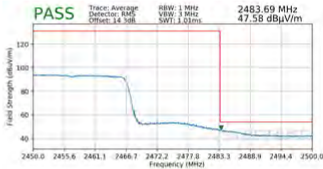
Plot 7-195. Radiated Restricted Upper Band Edge Measurement SISO ANT2 (Average – 242 Tones)
