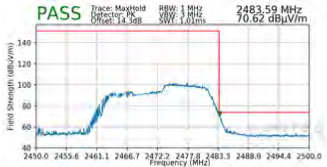
Plot 7-190. Radiated Restricted Upper Band Edge Measurement SISO ANT2 (Peak – 242 Tones)
