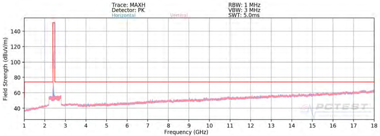
Plot 7-137. Radiated Spurious Plot above 1GHz SISO ANT1 (802.11ax OFDMA – 52 Tones – Ch. 1)
