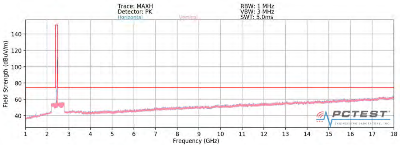
Plot 7-142. Radiated Spurious Plot above 1GHz SISO ANT1 (802.11ax OFDMA – 242 Tones – Ch. 11)
