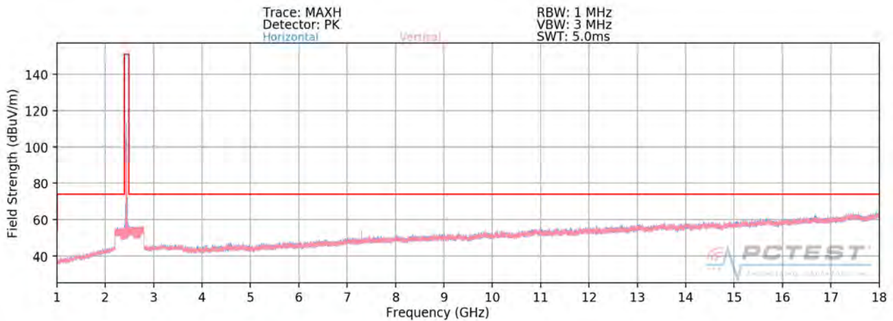
Plot 7-138. Radiated Spurious Plot above 1GHz SISO ANT1 (802.11ax OFDMA – 52 Tones – Ch. 6)
