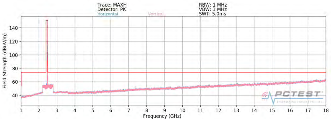
Plot 7-139. Radiated Spurious Plot above 1GHz SISO ANT1 (802.11ax OFDMA – 52 Tones – Ch. 11)
