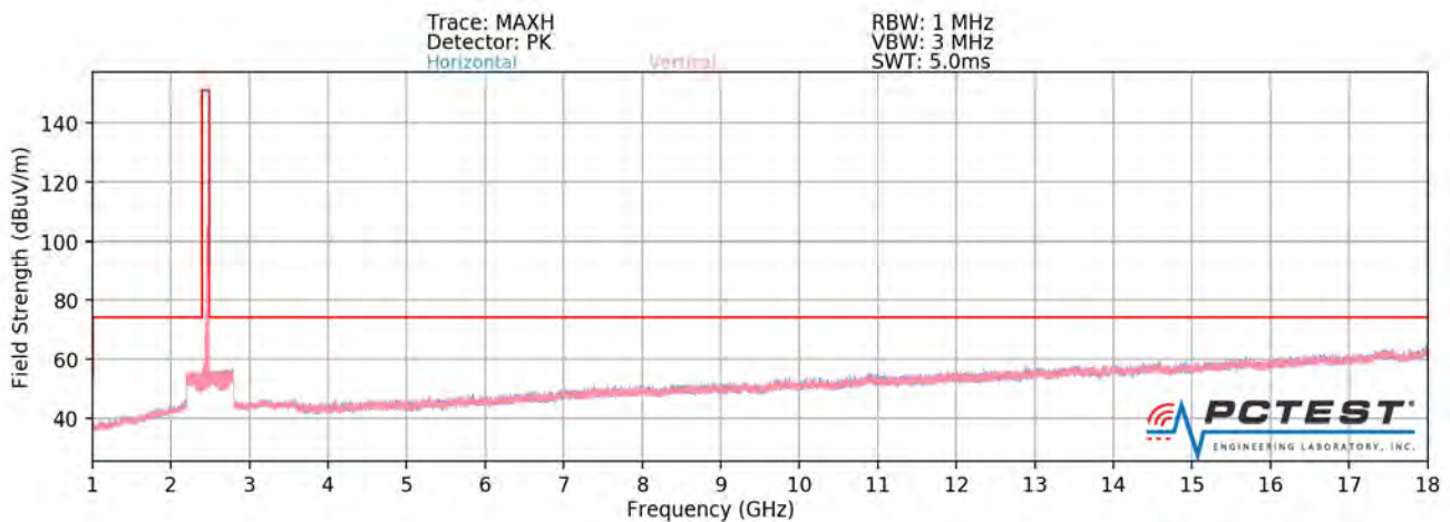
Plot 7-150. Radiated Spurious Plot above 1GHz SISO ANT2 (802.11ax OFDMA – 242 Tones – Ch. 11)
