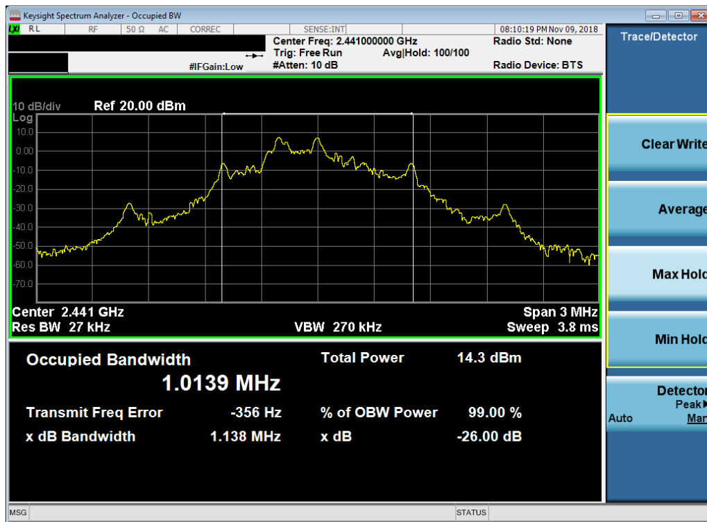
Plot 7-1. Occupied Bandwidth Plot (ANT+ – Ch. 39)
