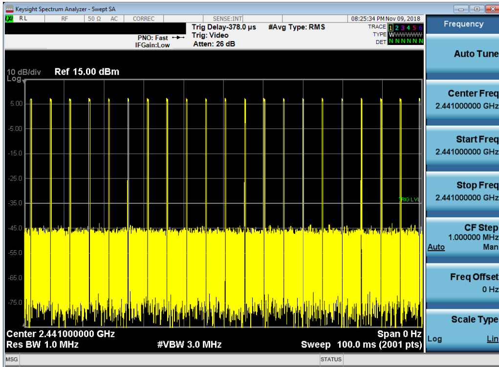
Plot 7-3. Worst Case 100ms Operation
