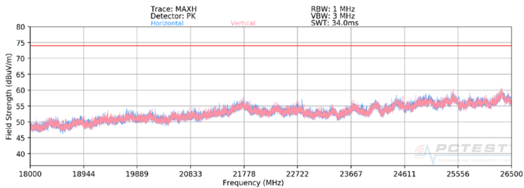
Plot 7-45. Radiated Spurious Plot above 18GHz
