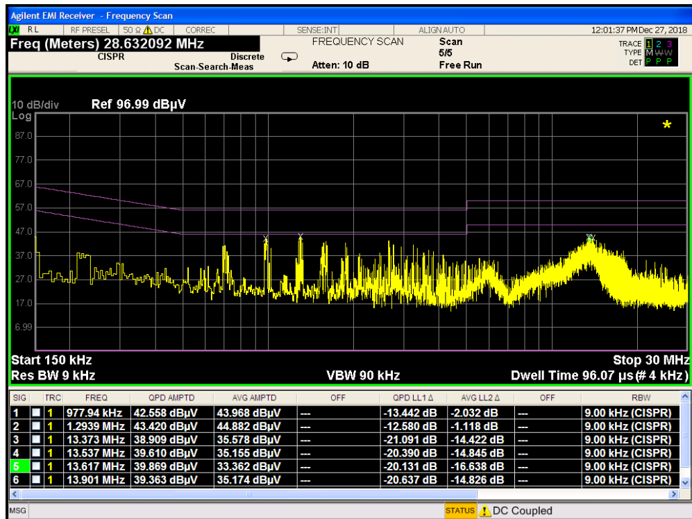
Plot 7-58. Line Conducted Plot with Bluetooth LE with WCC (N)
