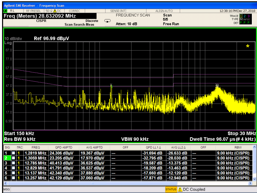
Plot 7-57. Line Conducted Plot with Bluetooth LE with WCC (L1)
