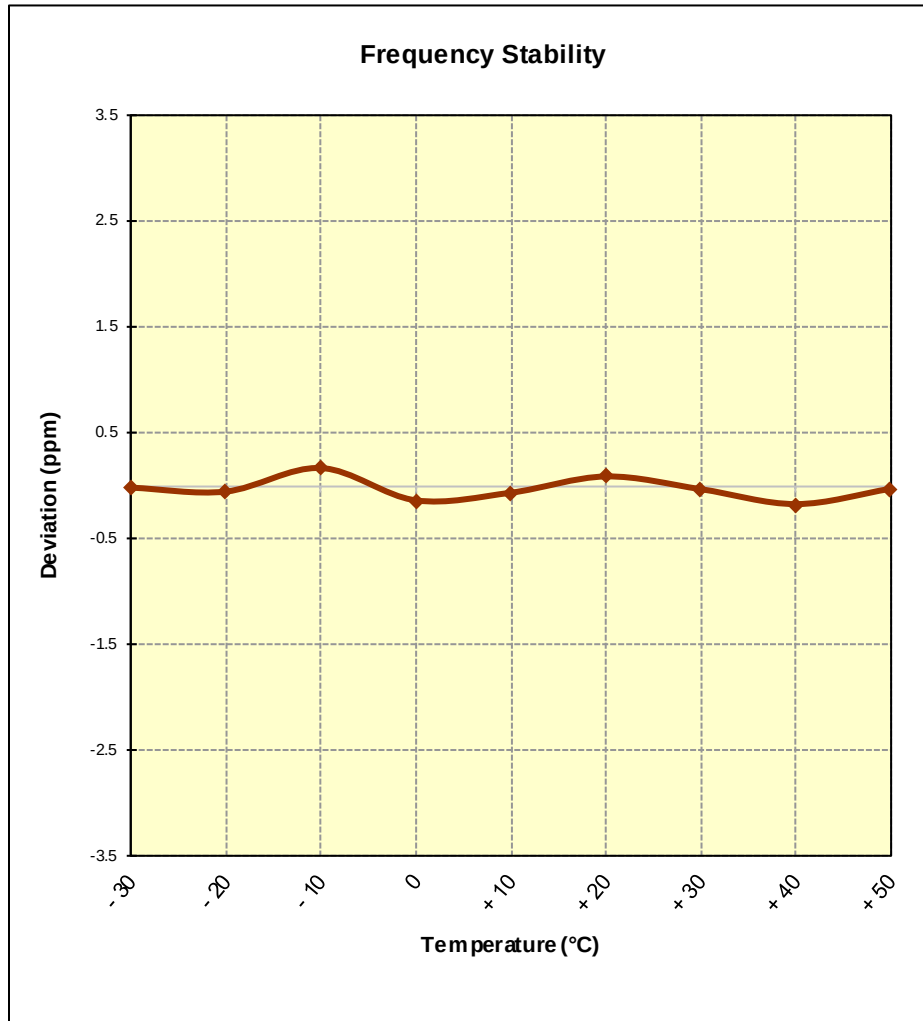
Figure 7-13. Frequency Stability Graph (Band 4)
