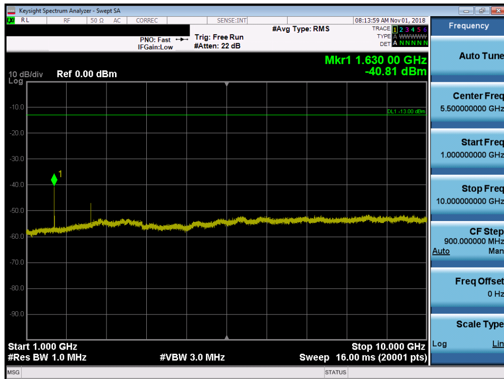
Plot 7-18. Conducted Spurious Plot (LTE Band 26, 15MHz QPSK – RB Size 1, RB Offset 0 – Mid Channel)
