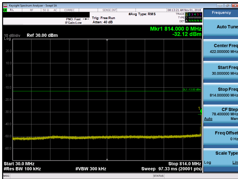
Plot 7-16. Conducted Spurious Plot (LTE Band 26, 15MHz QPSK – RB Size 1, RB Offset 0 – Mid Channel)
