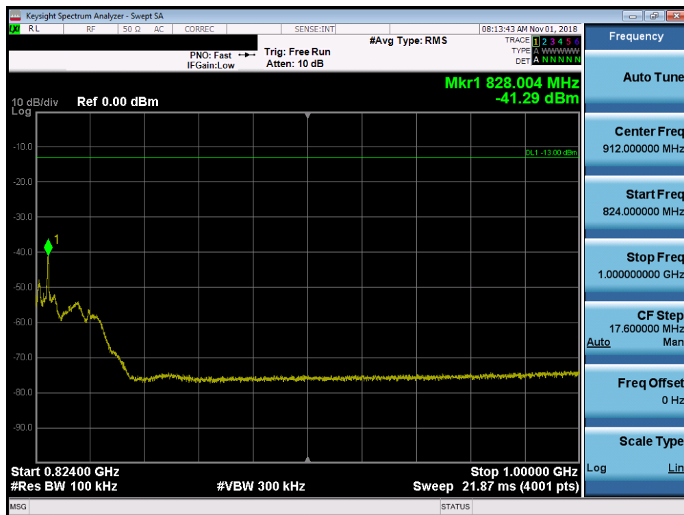
Plot 7-17. Conducted Spurious Plot (LTE Band 26, 15MHz QPSK – RB Size 1, RB Offset 0 – Mid Channel)
