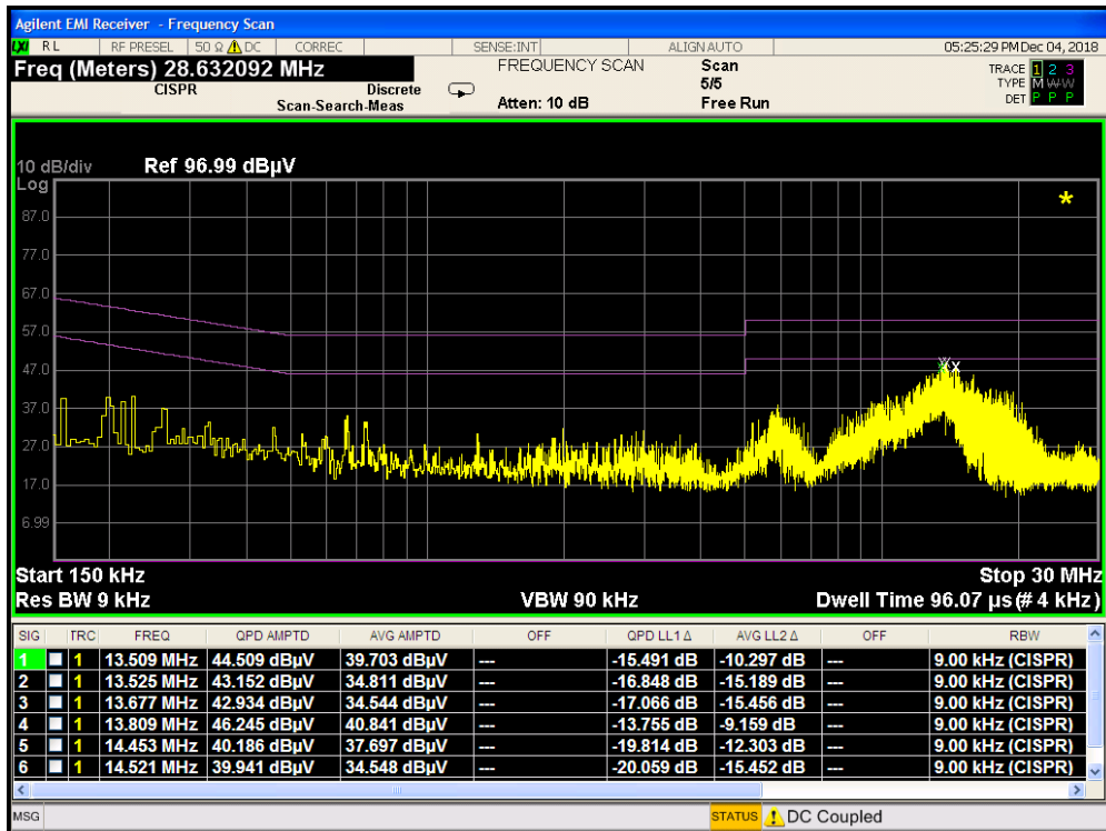
Plot 7-24. Line Conducted Plot (N - Configuration 2)
