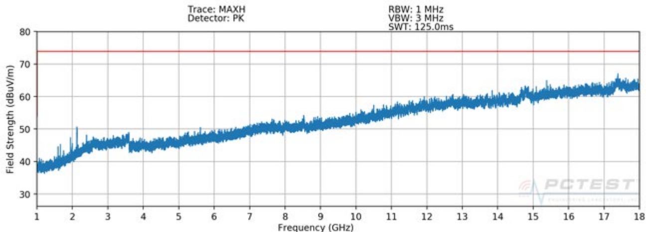
Plot 7-20. Radiated Spurious Plot above 1GHz (Configuration 5 - V)
