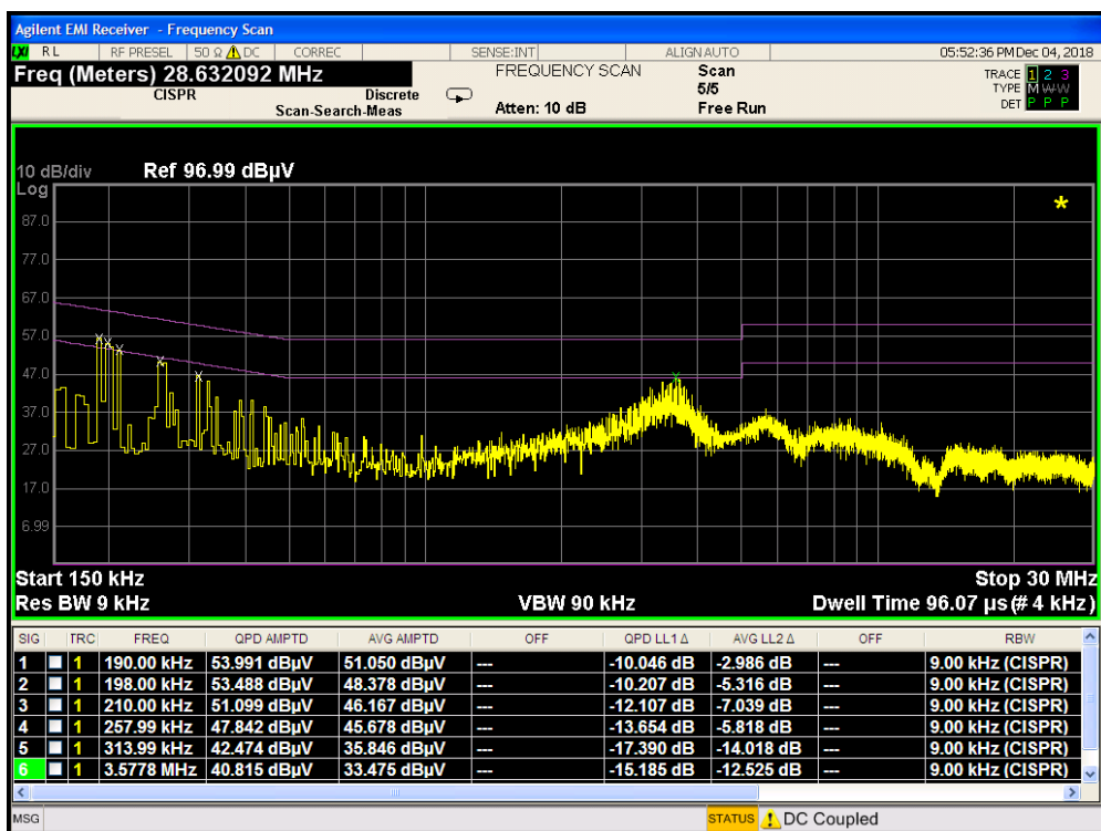
Plot 7-30. Line Conducted Plot (N - Configuration 5)
