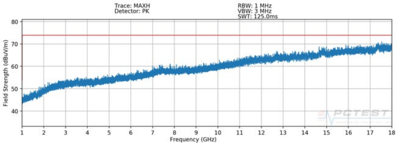
Plot 7-3. Radiated Spurious Plot above 1GHz (Configuration 1 - H)
