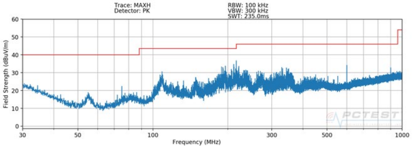
Plot 7-17. Radiated Spurious Plot below 1GHz (Configuration 5 - H)
