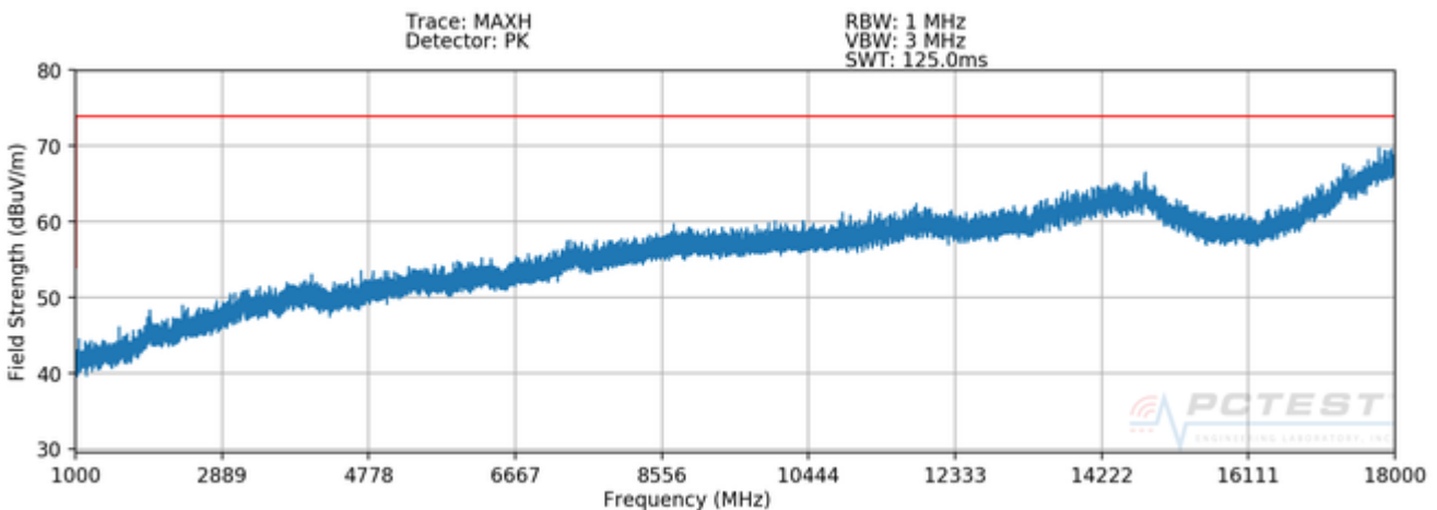
Plot 7-7. Radiated Spurious Plot above 1GHz (Configuration 2 - H)
