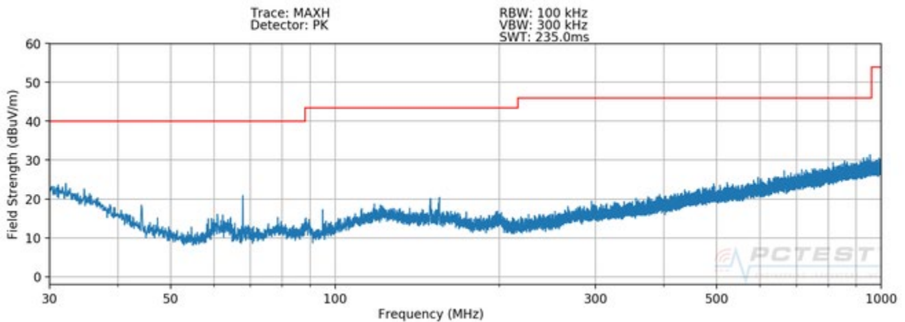
Plot 7-6. Radiated Spurious Plot below 1GHz (Configuration 2 - V)
