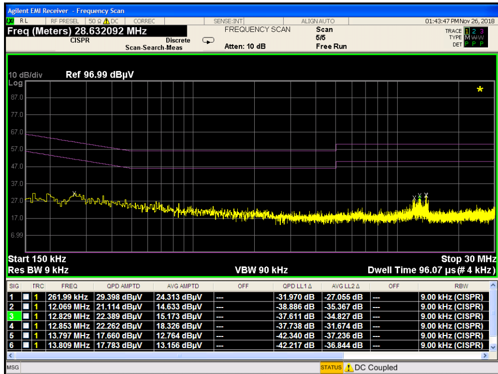
Plot 7-22. Line Conducted Plot (N- Configuration 1)
