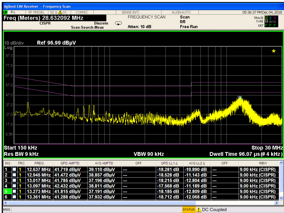
Plot 7-27. Line Conducted Plot (L1 - Configuration 4)
