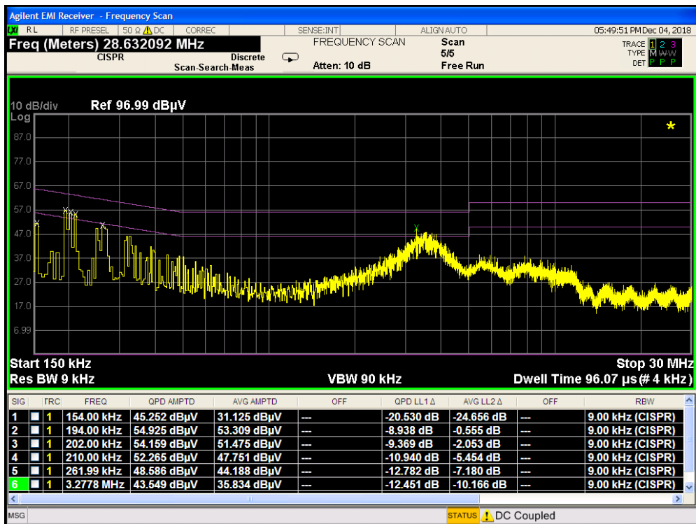
Plot 7-29. Line Conducted Plot (L1 - Configuration 5)
