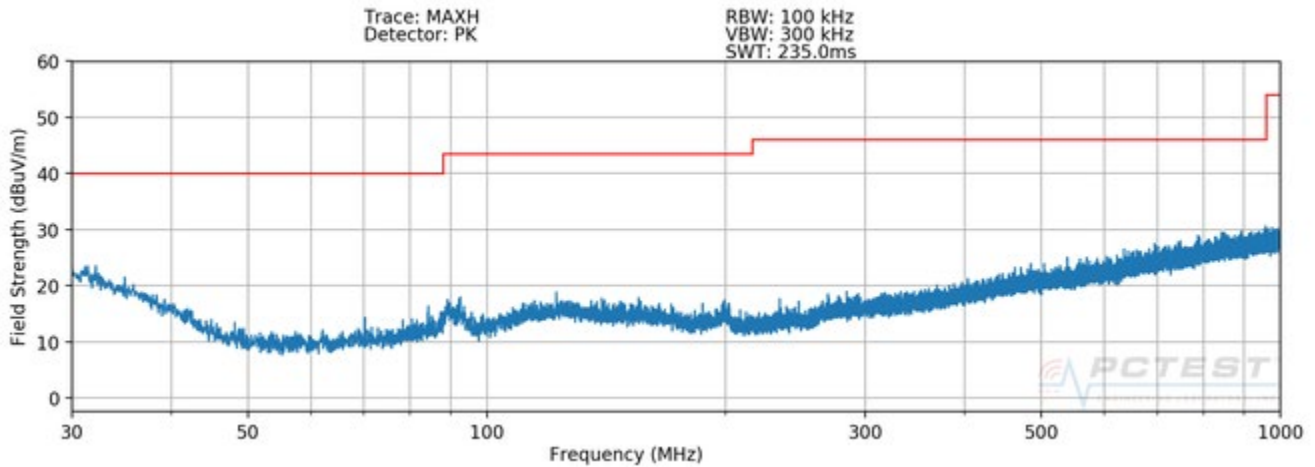
Plot 7-9. Radiated Spurious Plot below 1GHz (Configuration 3 - H)
