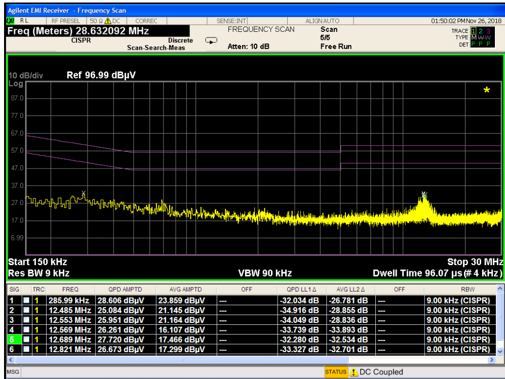
Plot 7-21. Line Conducted Plot (L1- Configuration 1)
