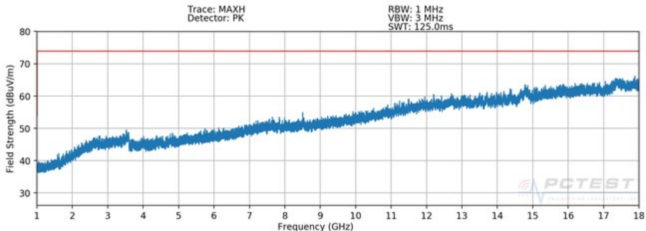
Plot 7-16. Radiated Spurious Plot above 1GHz (Configuration 4 - V)
