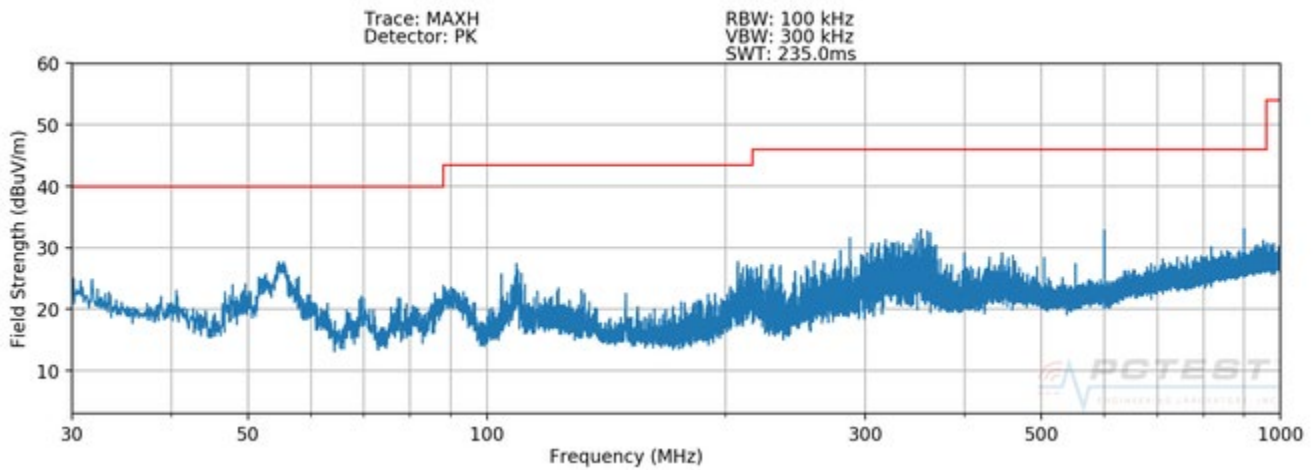
Plot 7-18. Radiated Spurious Plot below 1GHz (Configuration 5 - V)
