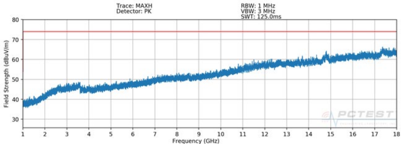
Plot 7-12. Radiated Spurious Plot above 1GHz (Configuration 3 - V)
