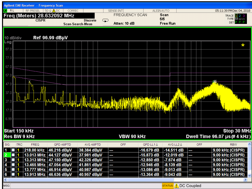
Plot 7-26. Line Conducted Plot (N - Configuration 3)
