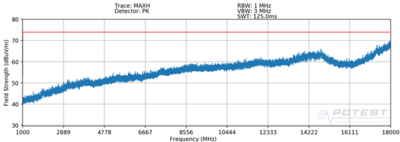
Plot 7-8. Radiated Spurious Plot above 1GHz (Configuration 2 - V)
