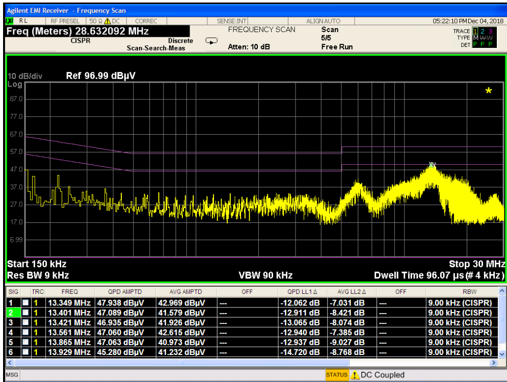
Plot 7-23. Line Conducted Plot (L1 - Configuration 2)
