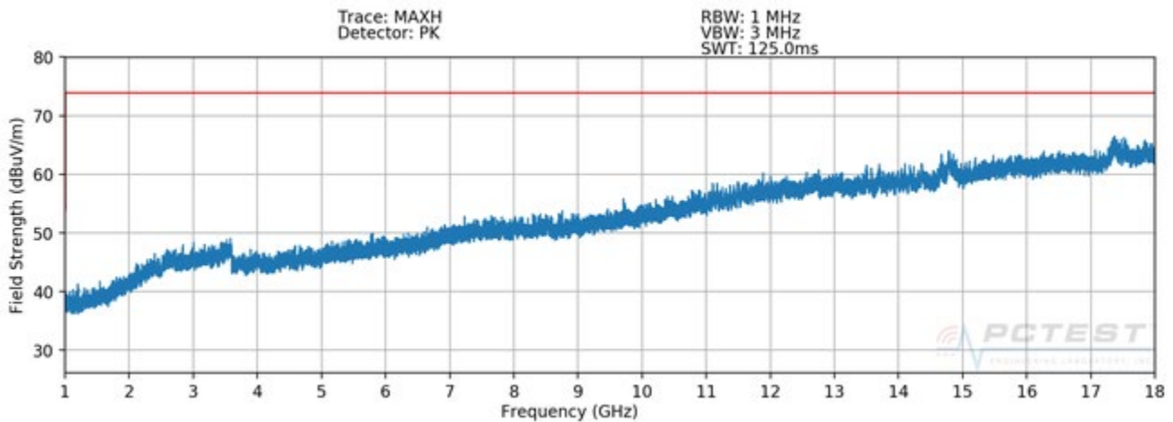
Plot 7-11. Radiated Spurious Plot above 1GHz (Configuration 3 - H)
