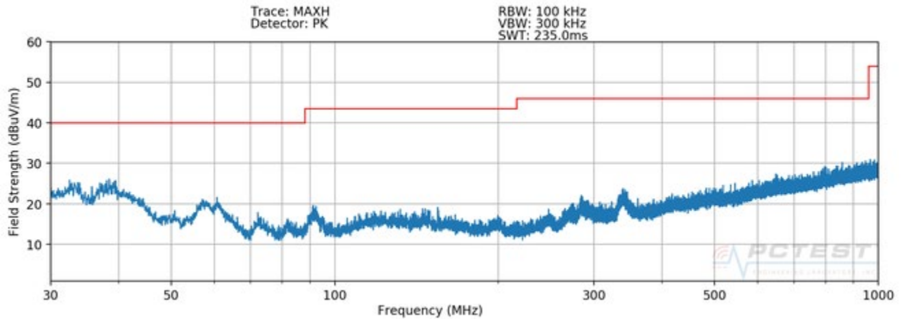
Plot 7-1. Radiated Spurious Plot below 1GHz (Configuration 1 - H)
