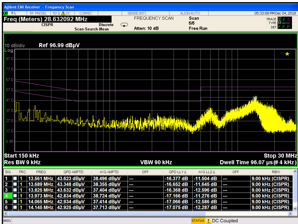
Plot 7-28. Line Conducted Plot (N - Configuration 4)
