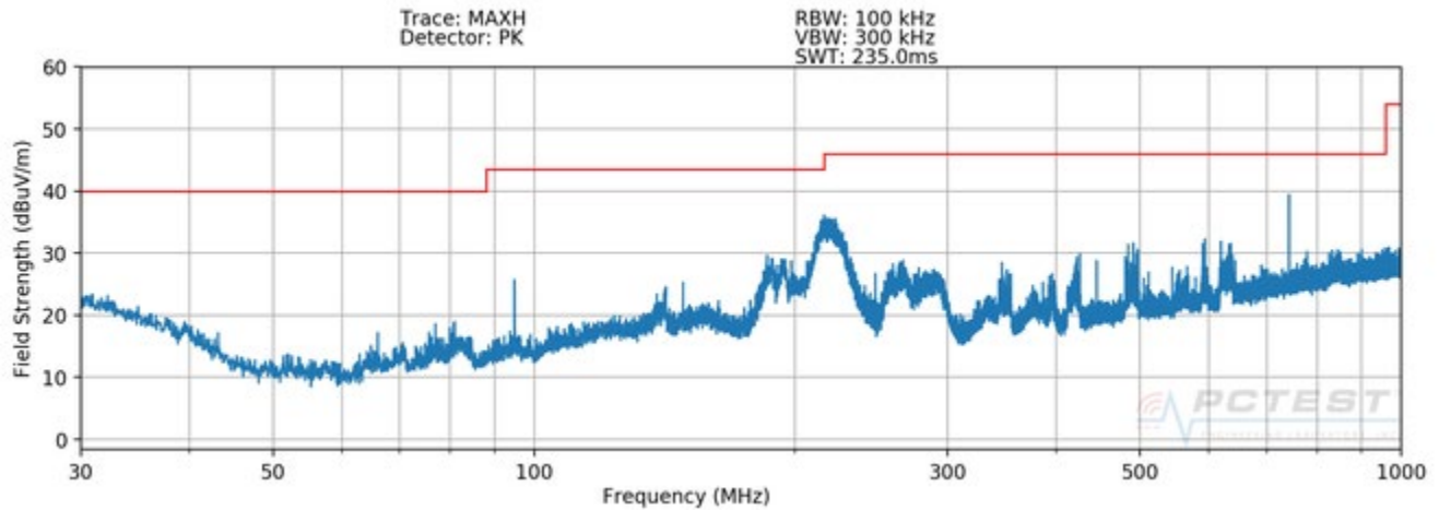
Plot 7-13. Radiated Spurious Plot below 1GHz (Configuration 4 - H)
