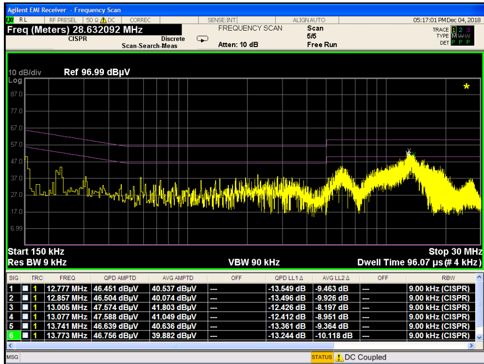
Plot 7-25. Line Conducted Plot (L1 - Configuration 3)
