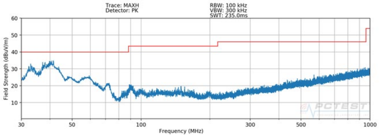
Plot 7-2. Radiated Spurious Plot below 1GHz (Configuration 1 - V)
