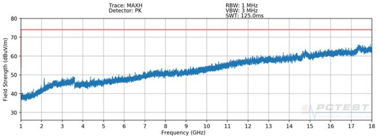
Plot 7-19. Radiated Spurious Plot above 1GHz (Configuration 5 - H)
