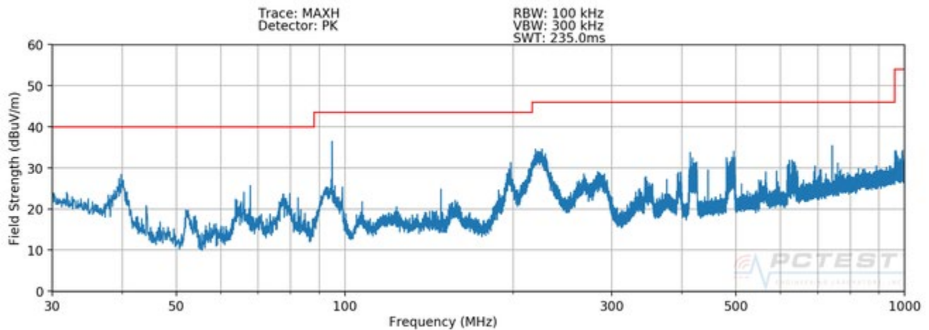
Plot 7-14. Radiated Spurious Plot below 1GHz (Configuration 4 - V)
