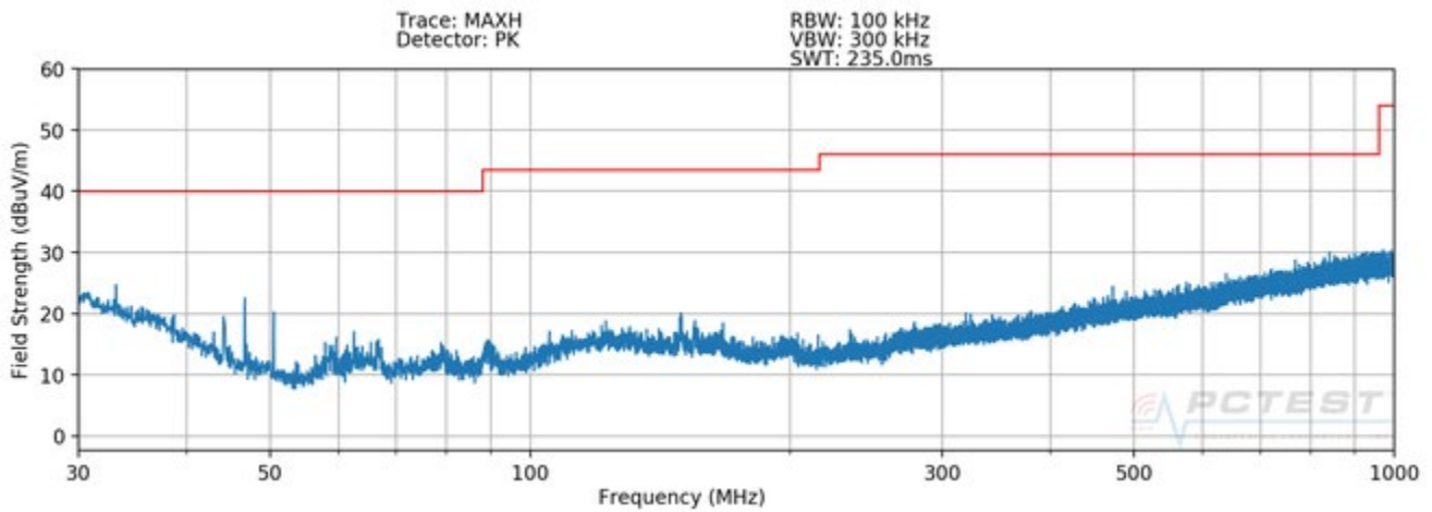
Plot 7-10. Radiated Spurious Plot below 1GHz (Configuration 3 - V)
