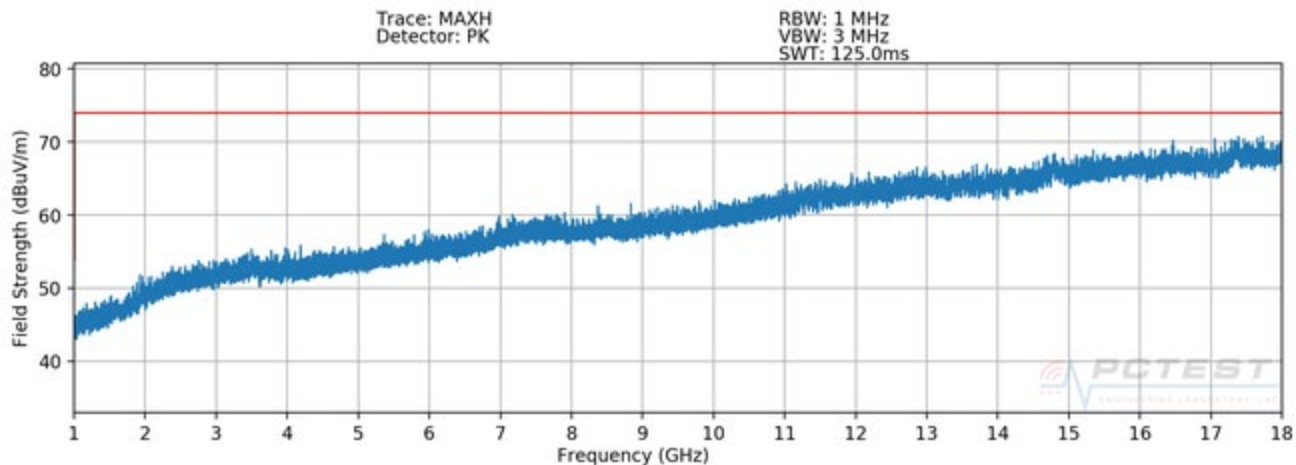
Plot 7-4. Radiated Spurious Plot above 1GHz (Configuration 1 - V)
