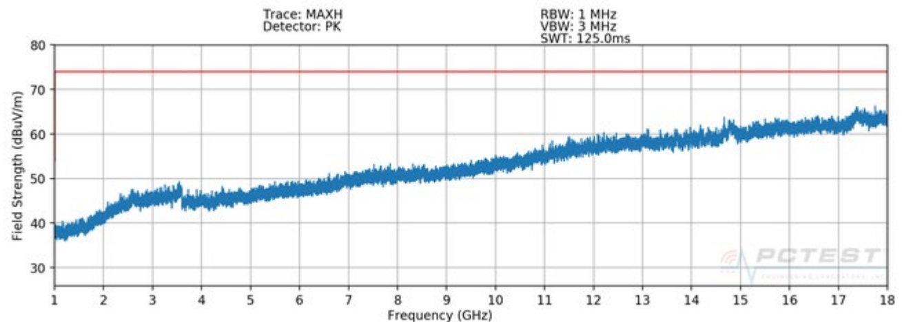
Plot 7-15. Radiated Spurious Plot above 1GHz (Configuration 4 - H)
