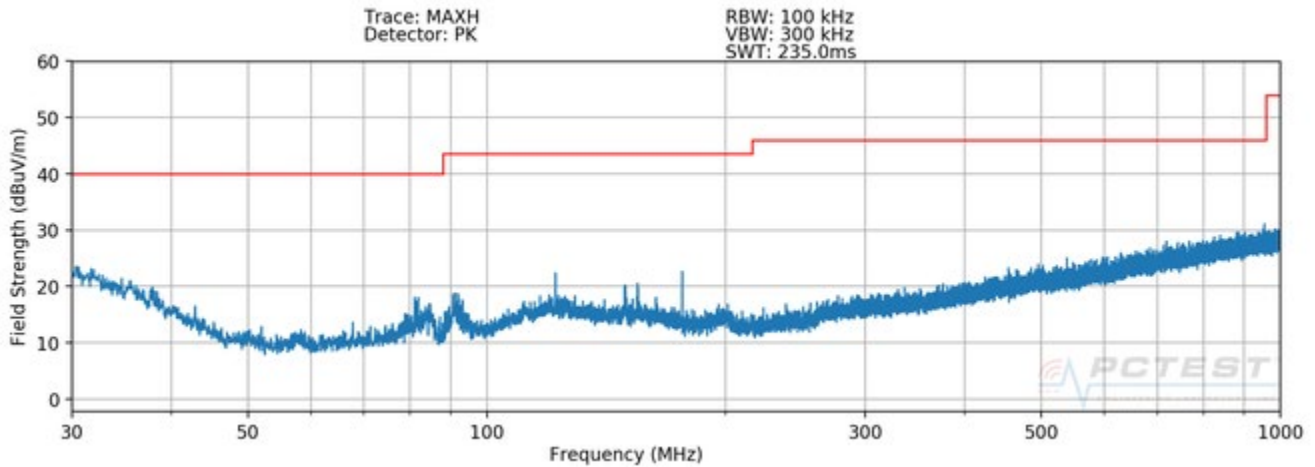
Plot 7-5. Radiated Spurious Plot below 1GHz (Configuration 2 - H)
