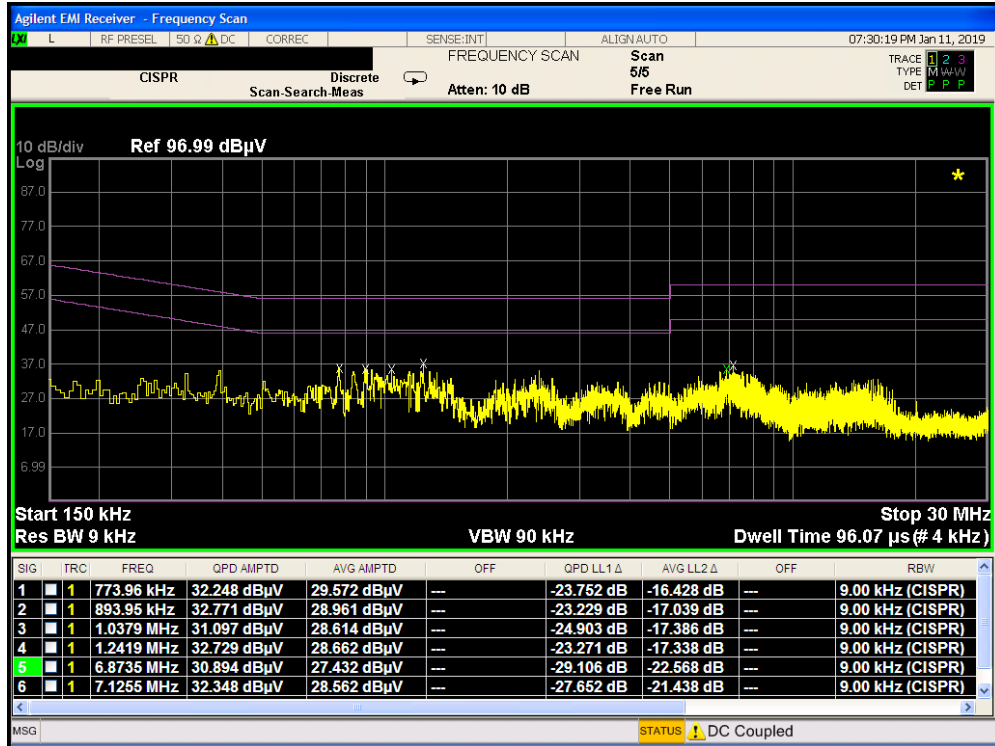
Plot 7-4. Line-Conducted Test Plot (L1)
