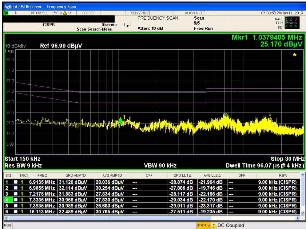
Plot 7-5. Line-Conducted Test Plot (N)
