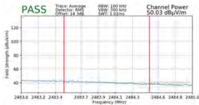
Plot 7-123. Radiated Restricted Upper Band Edge Measurement SISO ANT2 (Average)
