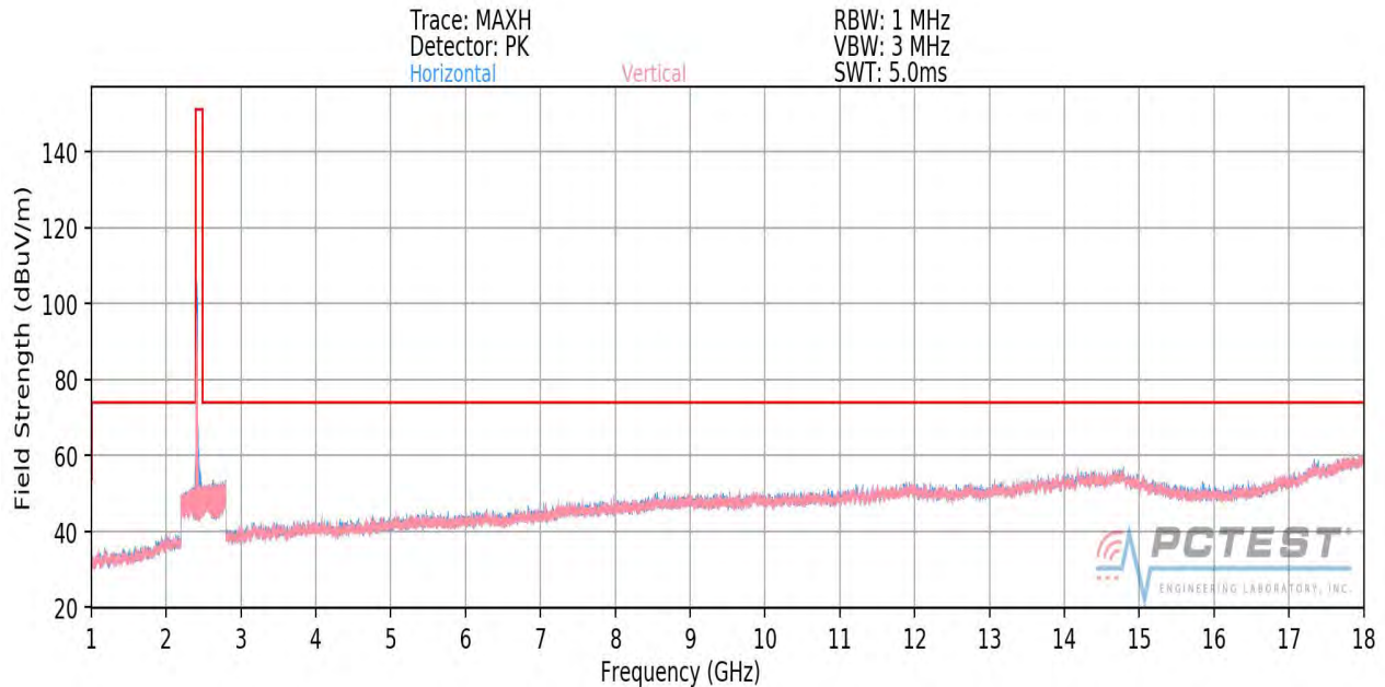
Plot 7-101. Radiated Spurious Plot above 1GHz MIMO/CDD (802.11g – Ch. 1)
