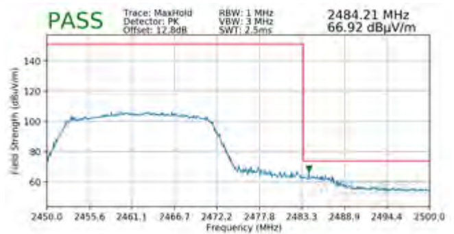
Plot 7-126. Radiated Restricted Upper Band Edge Measurement SISO ANT2 (Peak)
