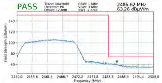
Plot 7-132. Radiated Restricted Band Edge Measurement SISO ANT2 with WCP (Peak)
