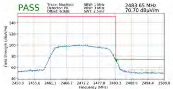
Plot 7-116. Radiated Restricted Upper Band Edge Measurement SISO ANT1 (Peak)
