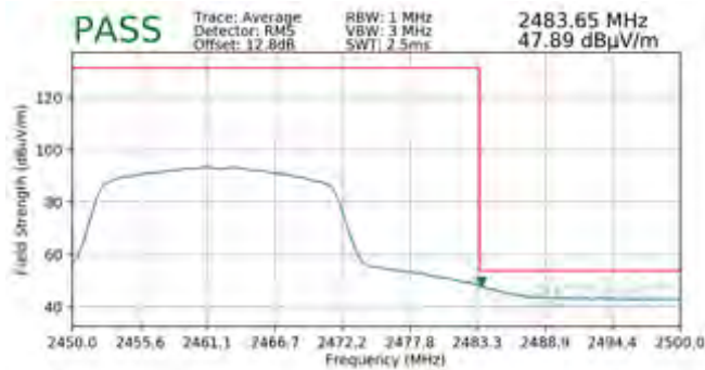
Plot 7-117. Radiated Restricted Band Edge Measurement SISO ANT1 with WCP (Average)
