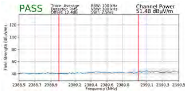
Plot 7-133. Radiated Restricted Lower Band Edge Measurement MIMO (Average)
