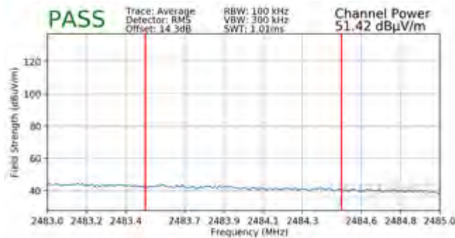
Plot 7-109. Radiated Restricted Upper Band Edge Measurement SISO ANT1 (Average)
