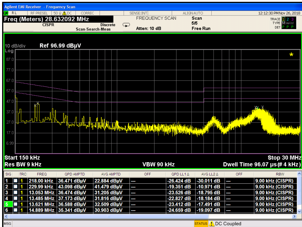
Plot 7-150. Line Conducted Plot 802.11b (N)
