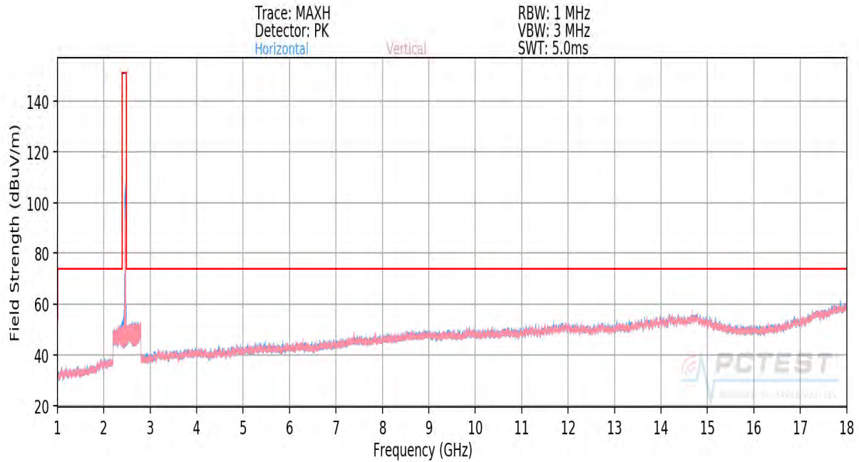
Plot 7-103. Radiated Spurious Plot above 1GHz MIMO/CDD (802.11g – Ch. 11)
