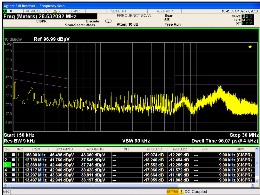
Plot 7-151. Line Conducted Plot 802.11b (L1) with WCC
