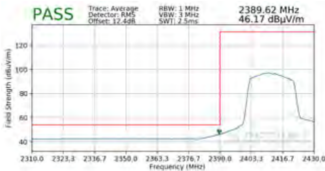
Plot 7-105. Radiated Restricted Lower Band Edge Measurement SISO ANT1 (Average)
