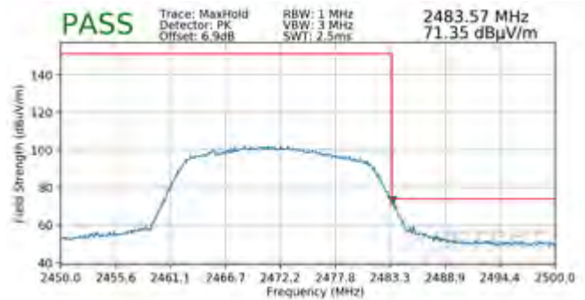
Plot 7-144. Radiated Restricted Upper Band Edge Measurement MIMO (Peak)
