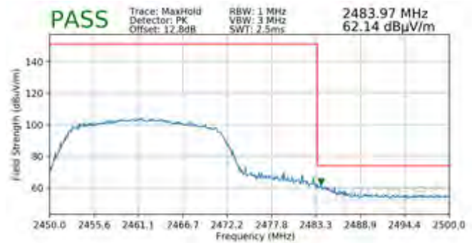
Plot 7-118. Radiated Restricted Band Edge Measurement SISO ANT1 with WCP (Peak)
