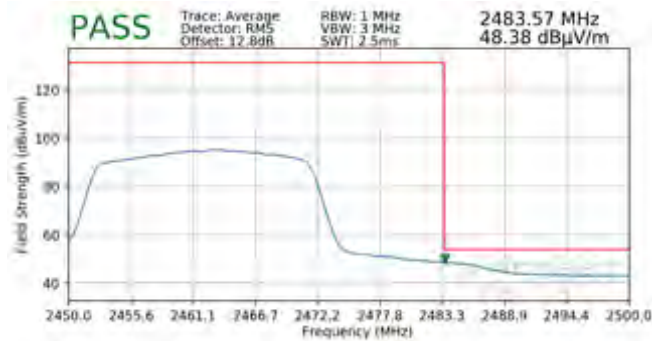
Plot 7-131. Radiated Restricted Band Edge Measurement SISO ANT2 with WCP (Average)
