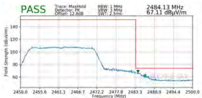
Plot 7-140. Radiated Restricted Upper Band Edge Measurement MIMO (Peak)
