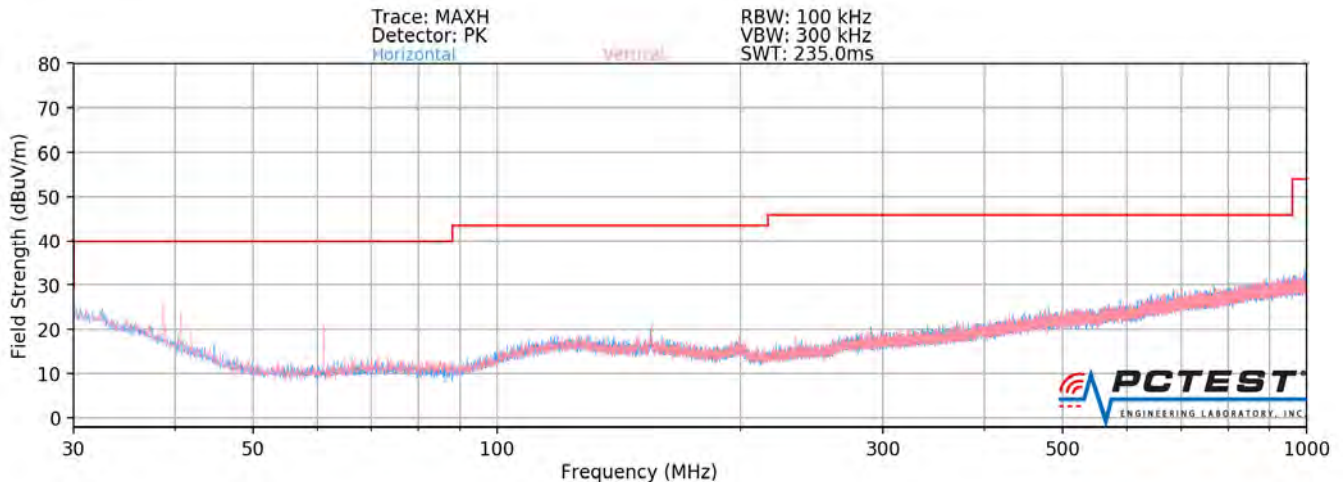
Plot 7-148. Radiated Spurious Plot below 1GHz SISO ANT2
