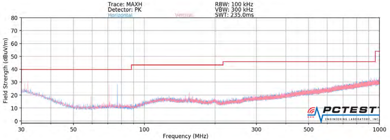
Plot 7-147. Radiated Spurious Plot below 1GHz SISO ANT1
