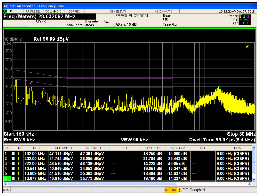
Plot 7-152. Line Conducted Plot 802.11b (N) with WCC
