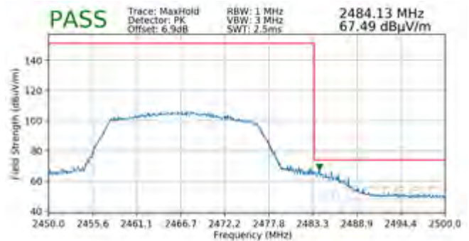
Plot 7-114. Radiated Restricted Upper Band Edge Measurement SISO ANT1 (Peak)
