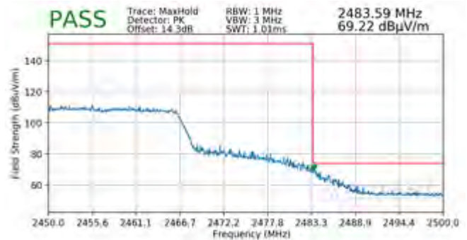
Plot 7-110. Radiated Restricted Upper Band Edge Measurement SISO ANT1 (Peak)
