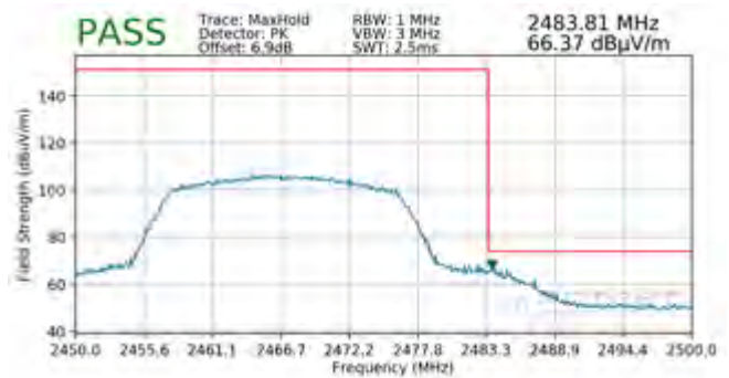
Plot 7-142. Radiated Restricted Upper Band Edge Measurement MIMO (Peak)
