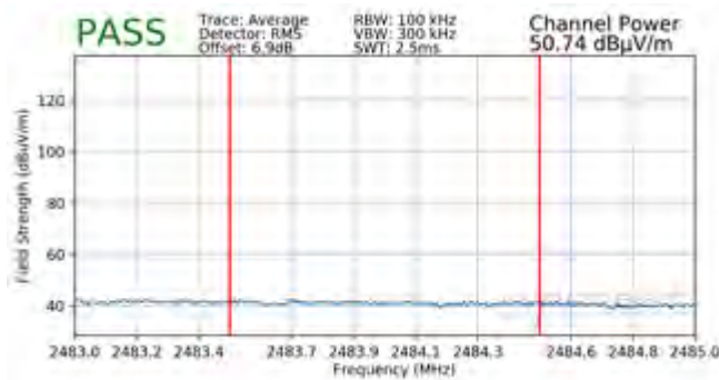
Plot 7-141. Radiated Restricted Upper Band Edge Measurement MIMO (Average)
