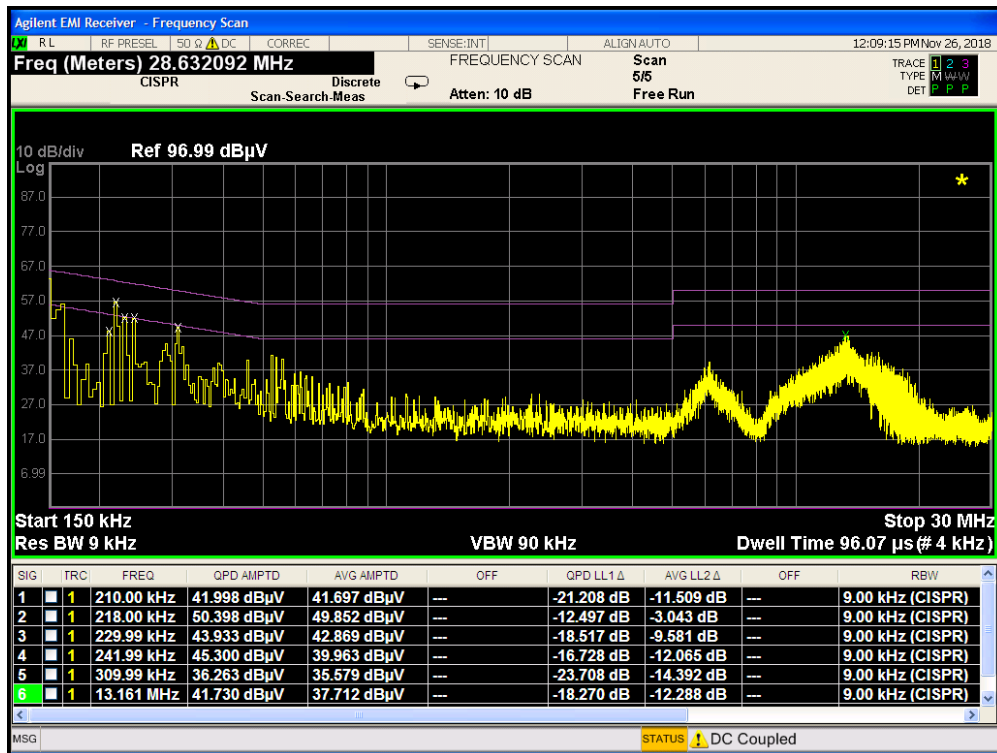
Plot 7-149. Line Conducted Plot 802.11b (L1)
