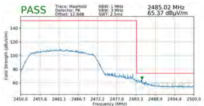
Plot 7-112. Radiated Restricted Upper Band Edge Measurement SISO ANT1 (Peak)
