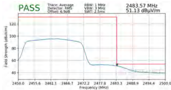
Plot 7-125. Radiated Restricted Upper Band Edge Measurement SISO ANT2 (Average)
