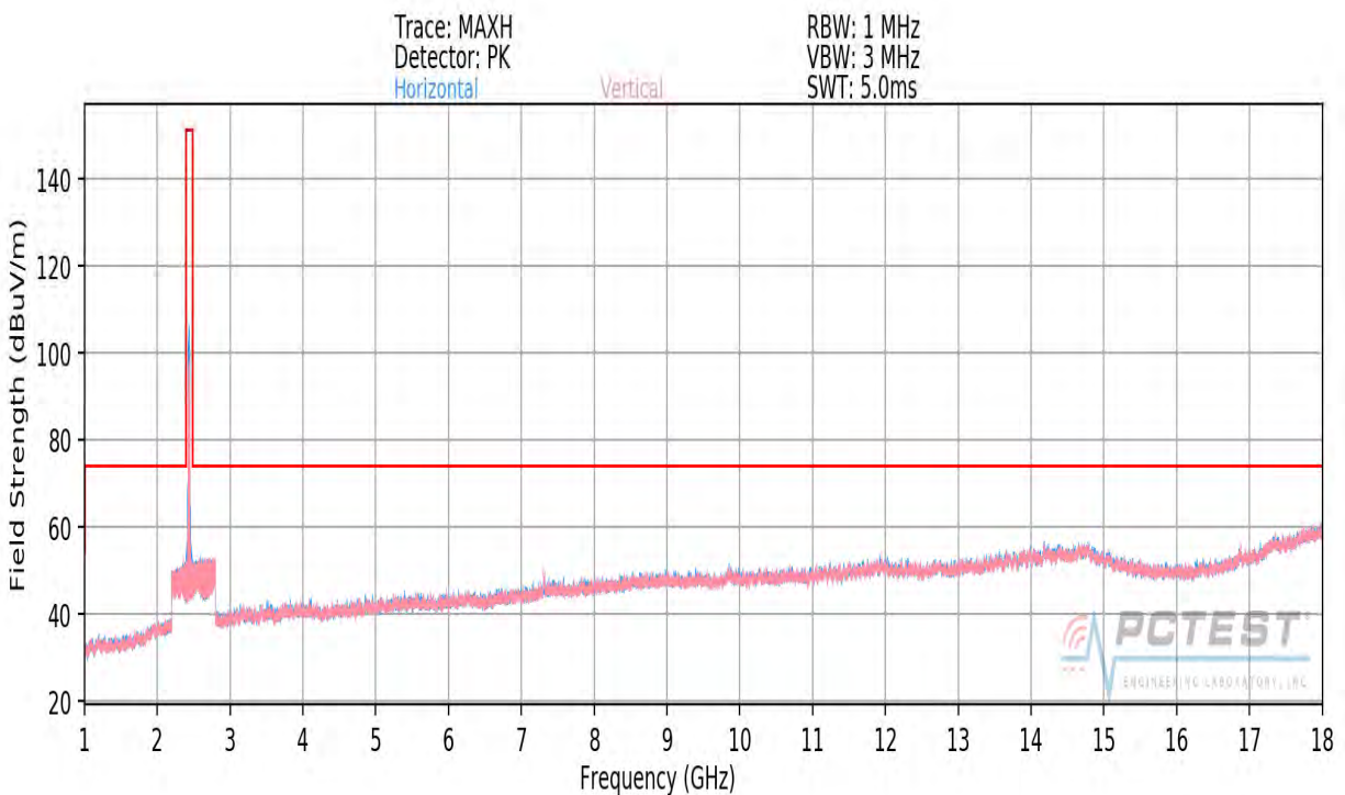
Plot 7-102. Radiated Spurious Plot above 1GHz MIMO/CDD (802.11g – Ch. 6)
