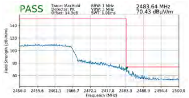
Plot 7-124. Radiated Restricted Upper Band Edge Measurement SISO ANT2 (Peak)
