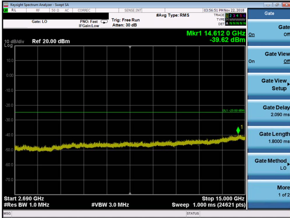
Plot 7-213. Conducted Spurious Plot (Band 41 PC2 - 15.0MHz QPSK -RB Size 1, RB Offset 0 -Mid Channel)
