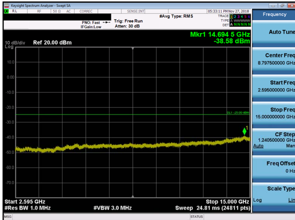
Plot 7-207. Conducted Spurious Plot (Band 7 - 20.0MHz QPSK - RB Size 1, RB Offset 0 - High Channel)
