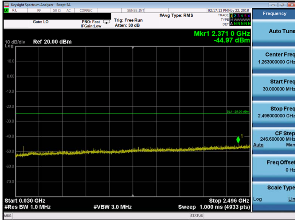
Plot 7-224. Conducted Spurious (Band 41/38 PC3- 15.0MHz QPSK RB Size 1, RB Offset 0 -High Channel)
