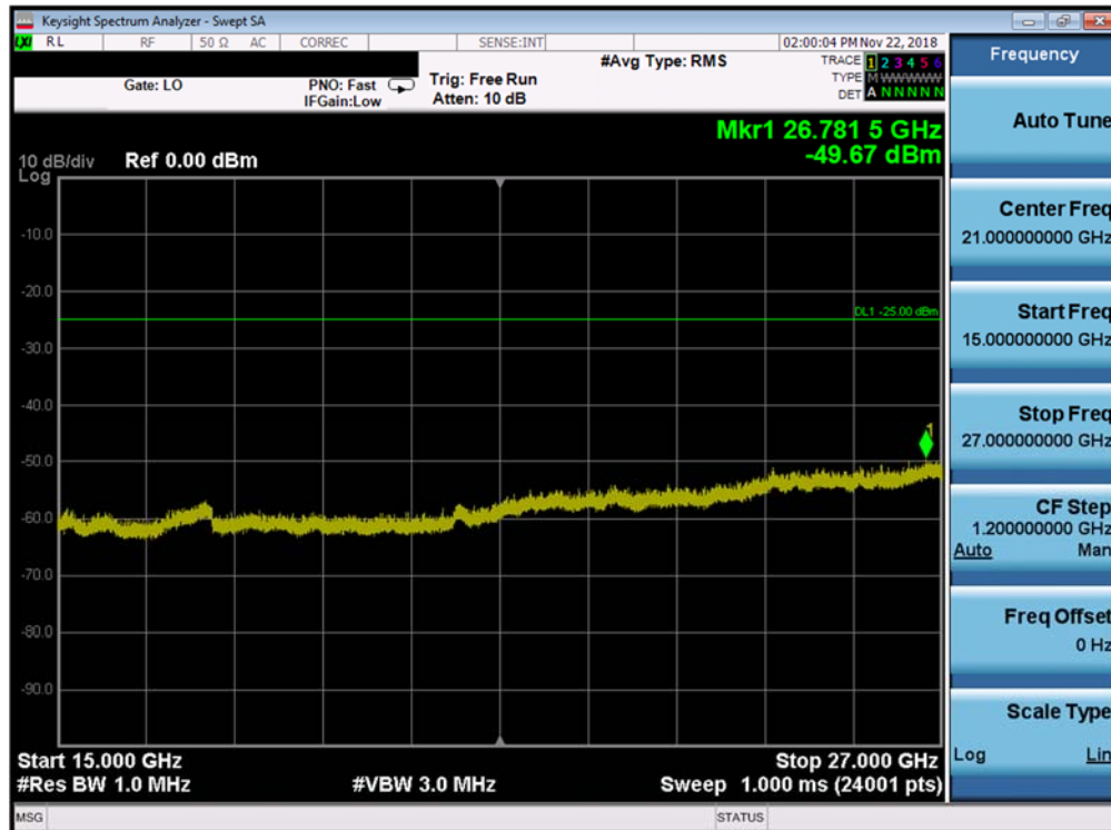
Plot 7-223. Conducted Spurious (Band 41/38 PC3- 15.0MHz QPSK -RB Size 1, RB Offset 0 -Mid Channel)
