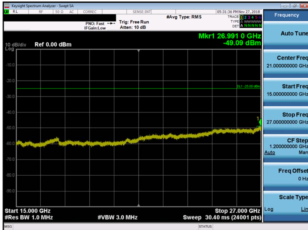
Plot 7-205. Conducted Spurious Plot (Band 7 - 20.0MHz QPSK - RB Size 1, RB Offset 0 - Mid Channel)
