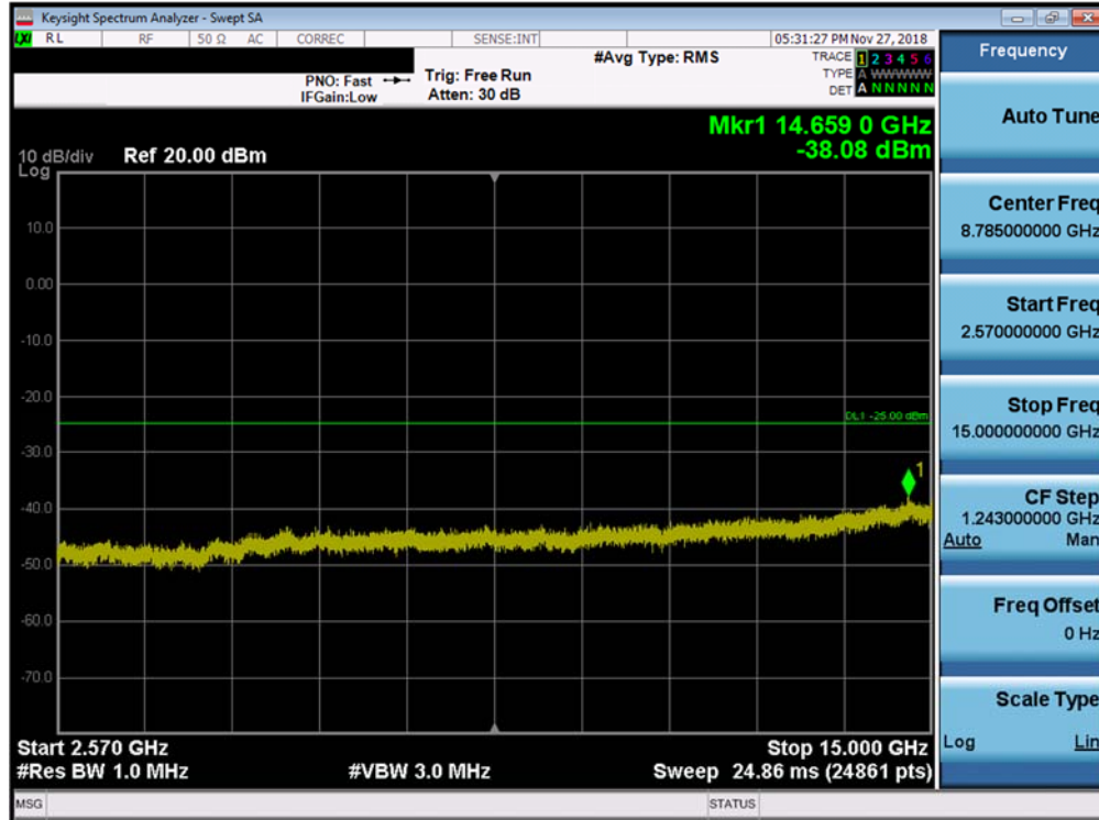
Plot 7-204. Conducted Spurious Plot (Band 7 - 20.0MHz QPSK - RB Size 1, RB Offset 0 - Mid Channel)
