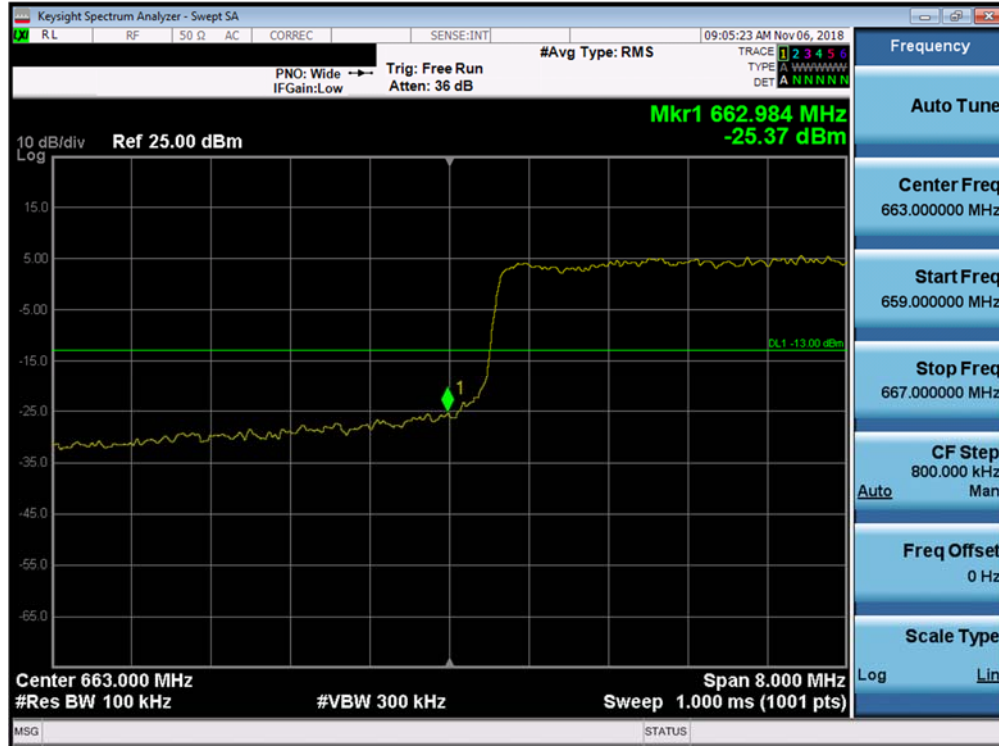
Plot 7-229. Lower Band Edge Plot (Band 71 - 10.0MHz QPSK - Full RB Configuration)
