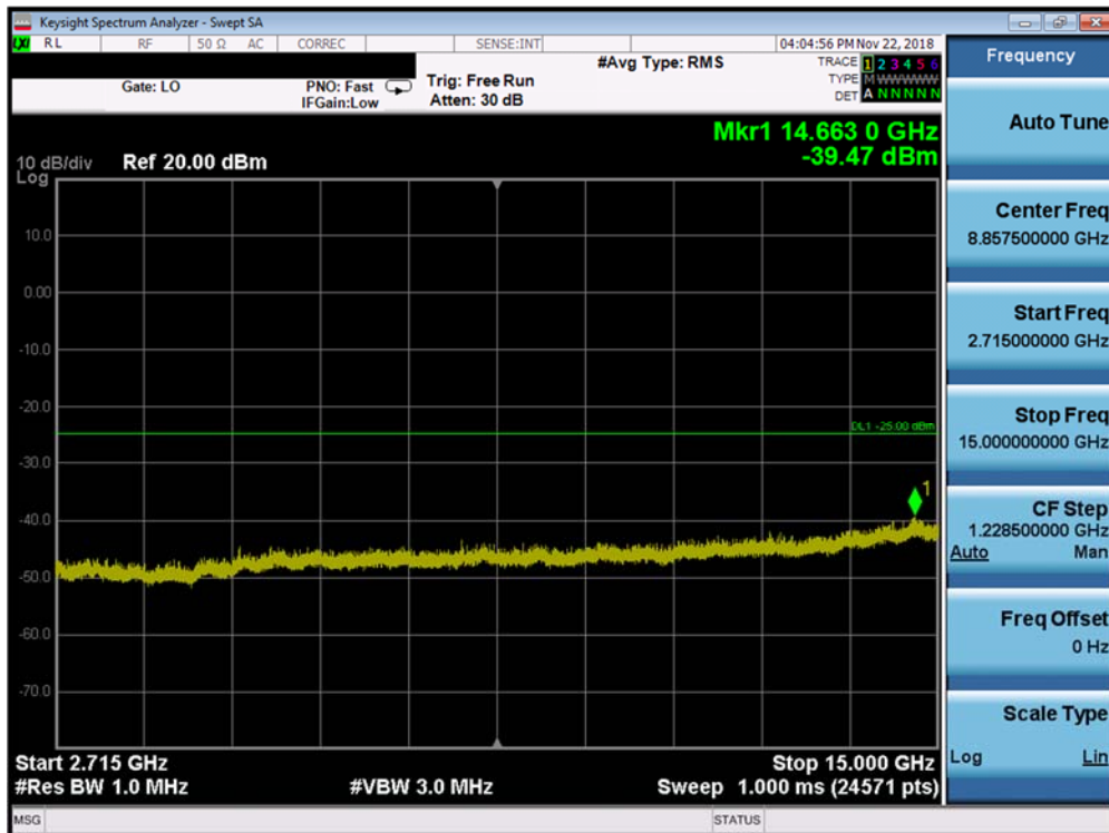
Plot 7-216. Conducted Spurious Plot (Band 41 PC2- 15.0MHz QPSK -RB Size 1, RB Offset 0 -High Channel)
