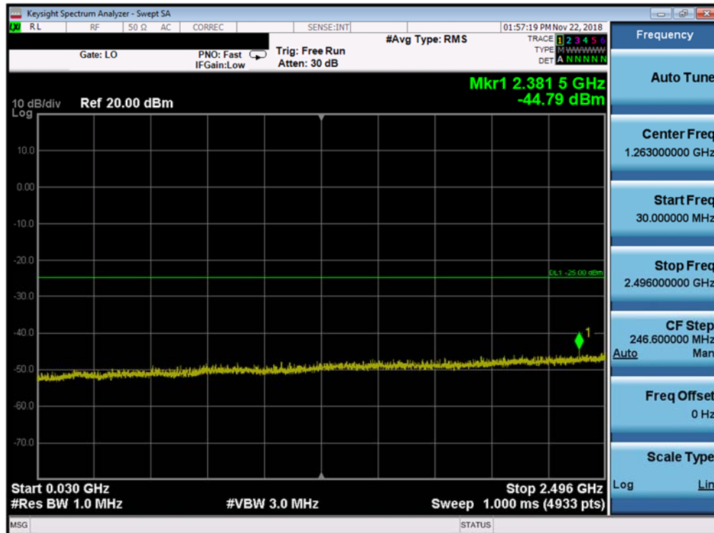
Plot 7-221. Conducted Spurious (Band 41/38 PC3 - 15.0MHz QPSK -RB Size 1, RB Offset 0 -Mid Channel)
