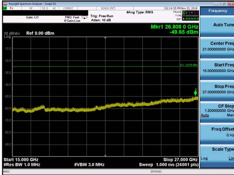
Plot 7-220. Conducted Spurious (Band 41/38 PC3 - 15.0MHz QPSK -RB Size 1, RB Offset 0 -Low Channel)
