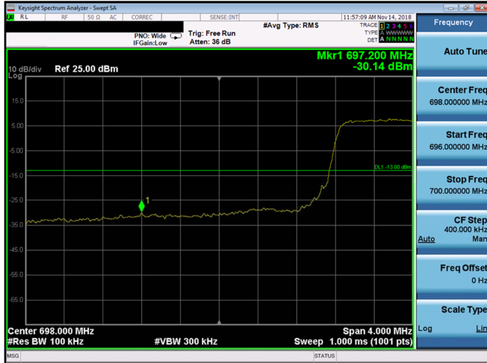
Plot 7-239. Lower Band Edge Plot (Band 12 - 5.0MHz QPSK - Full RB Configuration)
