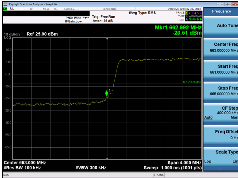
Plot 7-227. Lower Band Edge Plot (Band 71 - 5.0MHz QPSK - Full RB Configuration)
