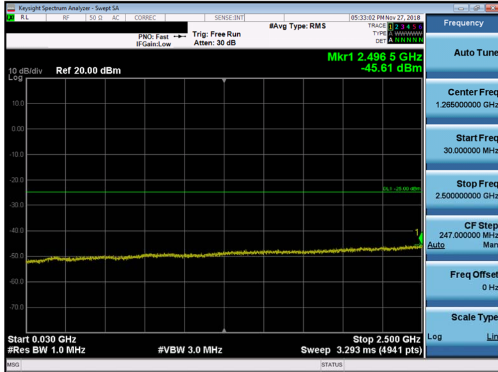
Plot 7-206. Conducted Spurious Plot (Band 7 - 20.0MHz QPSK - RB Size 1, RB Offset 0 - High Channel)
