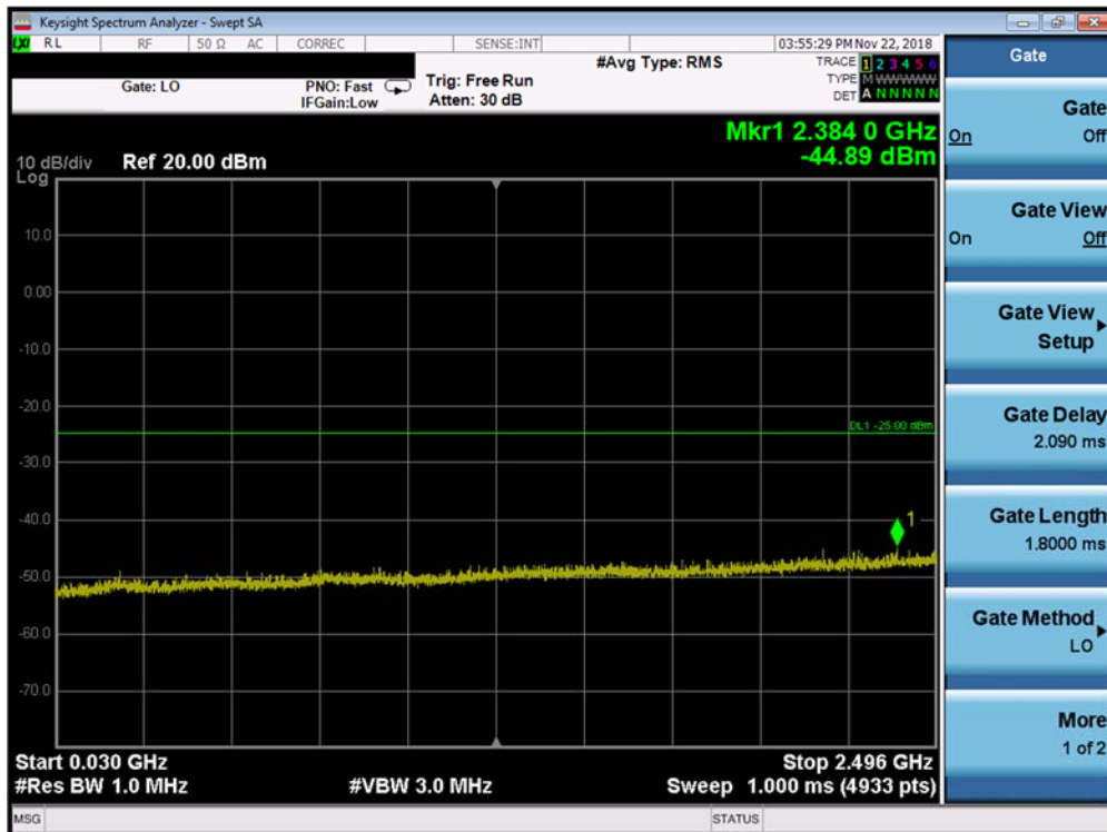
Plot 7-212. Conducted Spurious Plot (Band 41 PC2 - 15.0MHz QPSK -RB Size 1, RB Offset 0 -Mid Channel)
