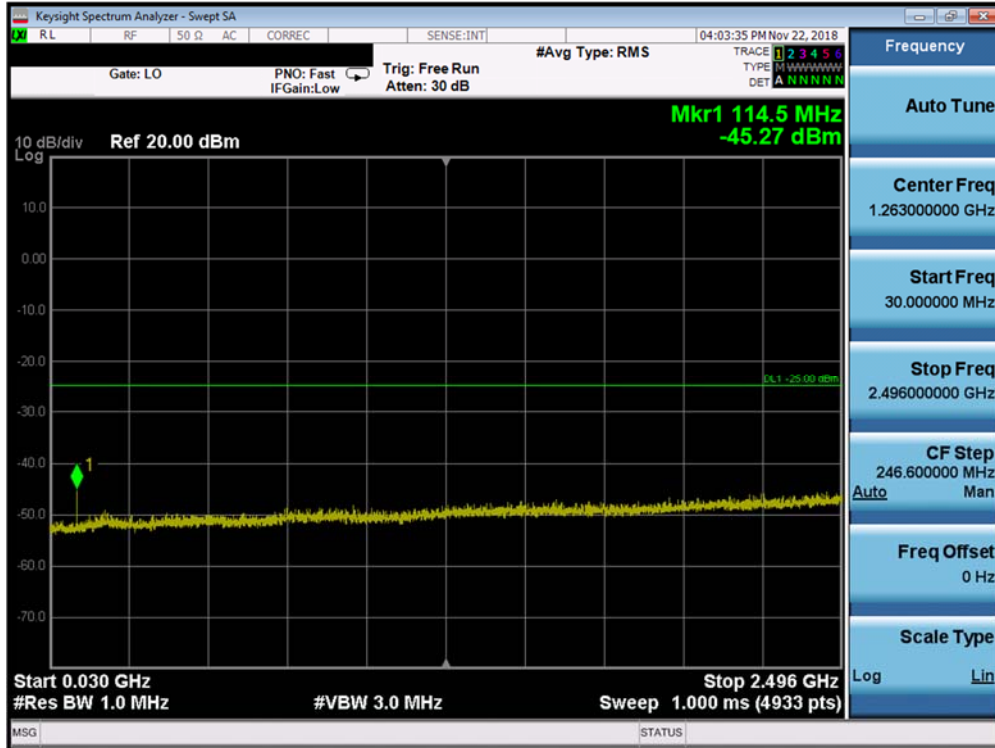
Plot 7-215. Conducted Spurious Plot (Band 41 PC2- 15.0MHz QPSK RB Size 1, RB Offset 0 -High Channel)
