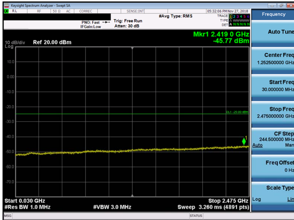
Plot 7-200. Conducted Spurious Plot (Band 7 - 20.0MHz QPSK - RB Size 1, RB Offset 0 - Low Channel)
