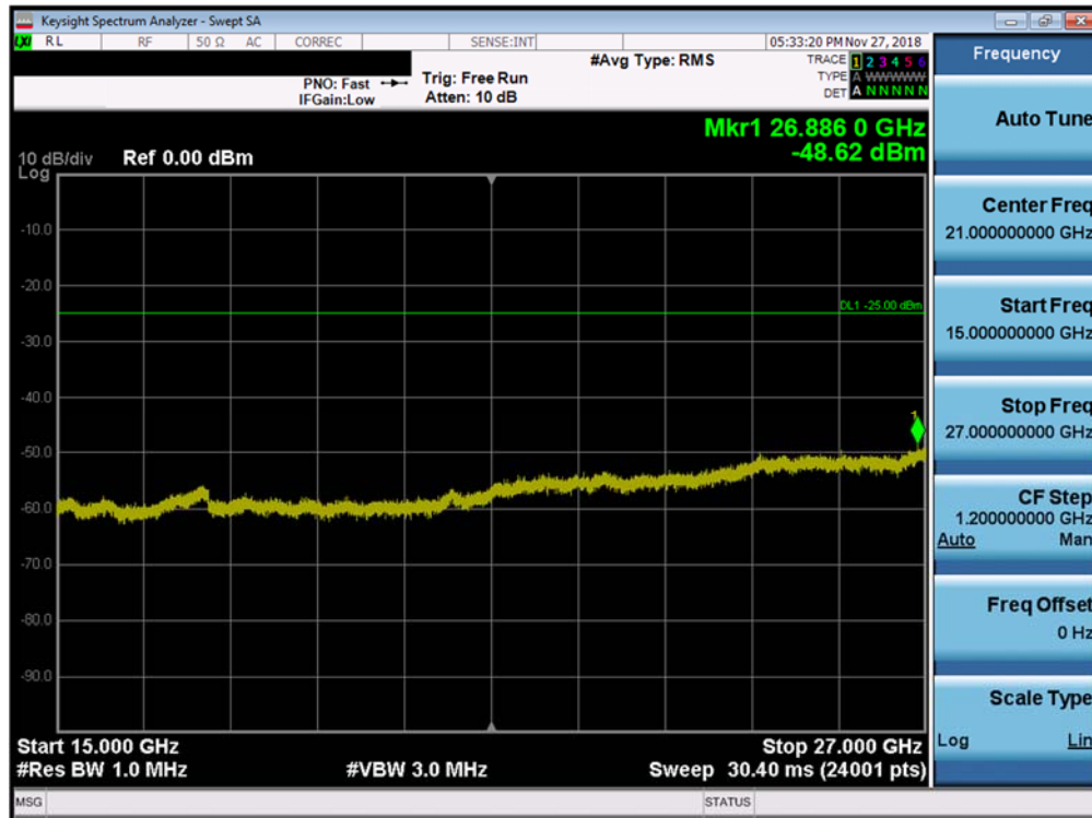
Plot 7-208. Conducted Spurious Plot (Band 7 - 20.0MHz QPSK - RB Size 1, RB Offset 0 - High Channel)
