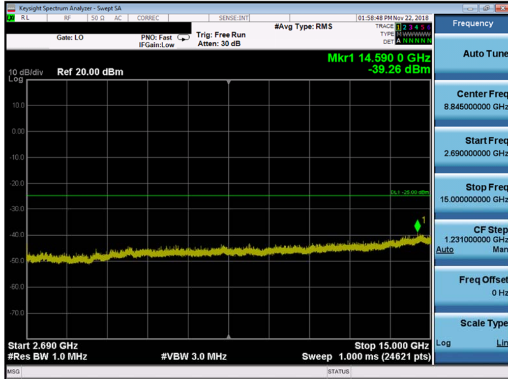
Plot 7-222. Conducted Spurious (Band 41/38 PC3 - 15.0MHz QPSK -RB Size 1, RB Offset 0 -Mid Channel)
