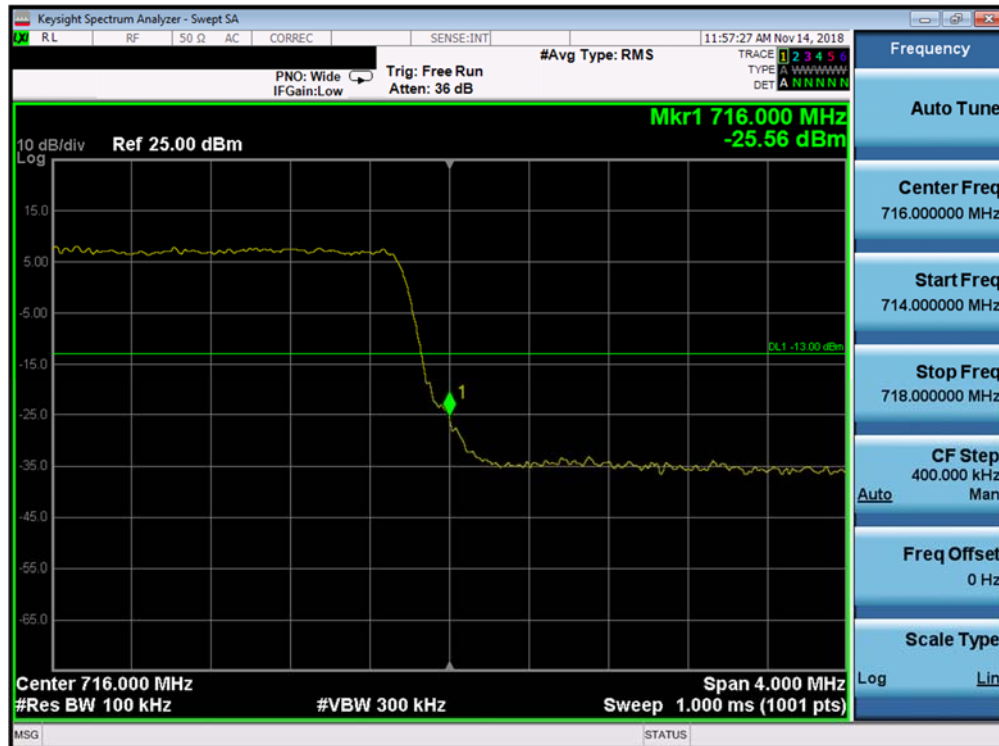
Plot 7-240. Upper Band Edge Plot (Band 12 - 5.0MHz QPSK - Full RB Configuration)
