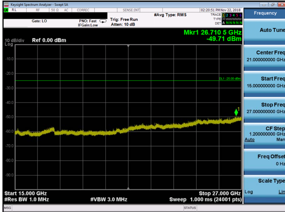
Plot 7-226. Conducted Spurious (Band 41/38 PC3- 15.0MHz QPSK -RB Size 1, RB Offset 0 -High Channel)
