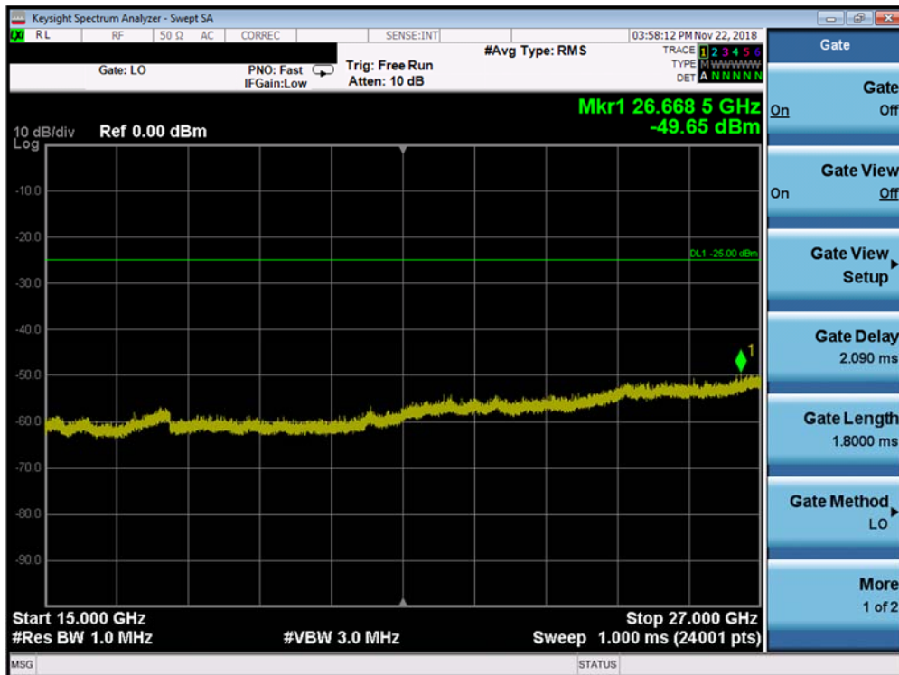
Plot 7-214. Conducted Spurious Plot (Band 41 PC2- 15.0MHz QPSK -RB Size 1, RB Offset 0 -Mid Channel)
