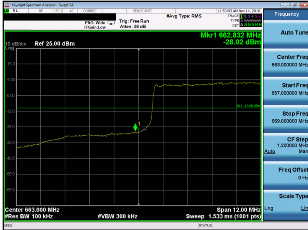
Plot 7-231. Lower Band Edge Plot (Band 71 - 15.0MHz QPSK - Full RB Configuration)
