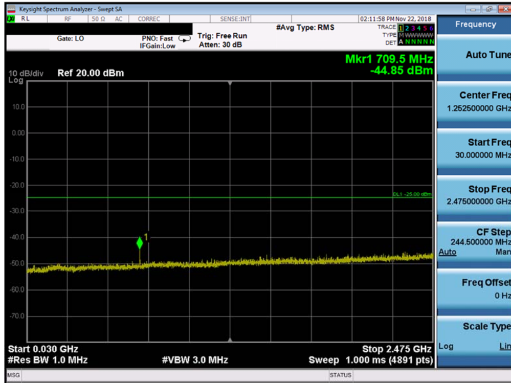
Plot 7-218. Conducted Spurious (Band 41/38 PC3 - 15.0MHz QPSK -RB Size 1, RB Offset 0 -Low Channel)
