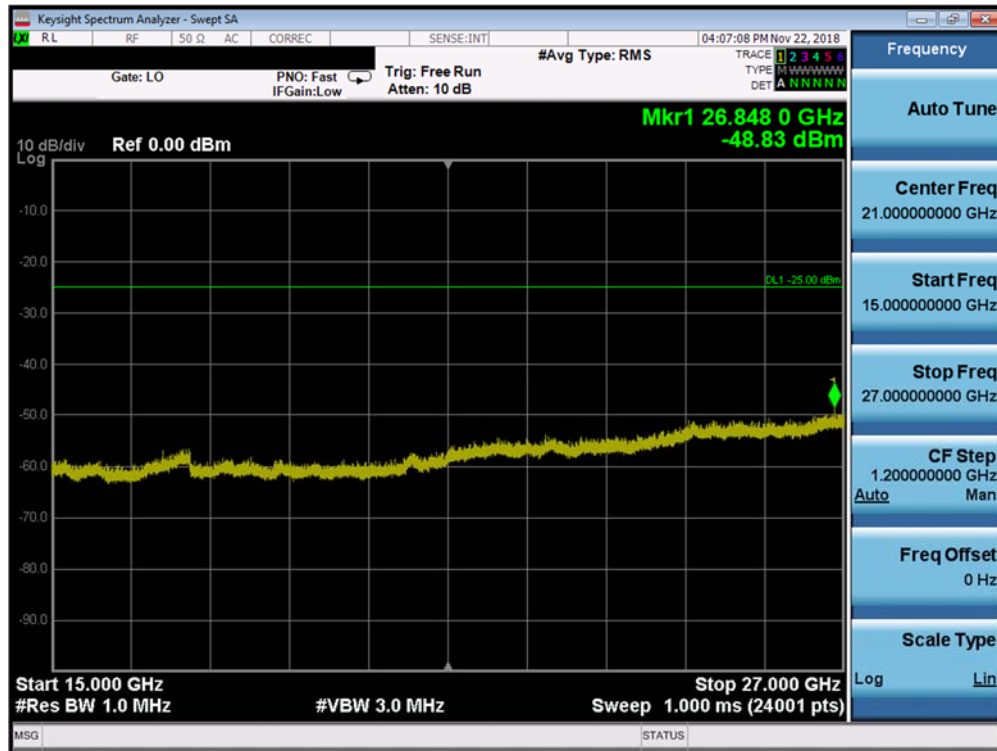
Plot 7-217. Conducted Spurious Plot (Band 41 PC2- 15.0MHz QPSK -RB Size 1, RB Offset 0 -High Channel)
