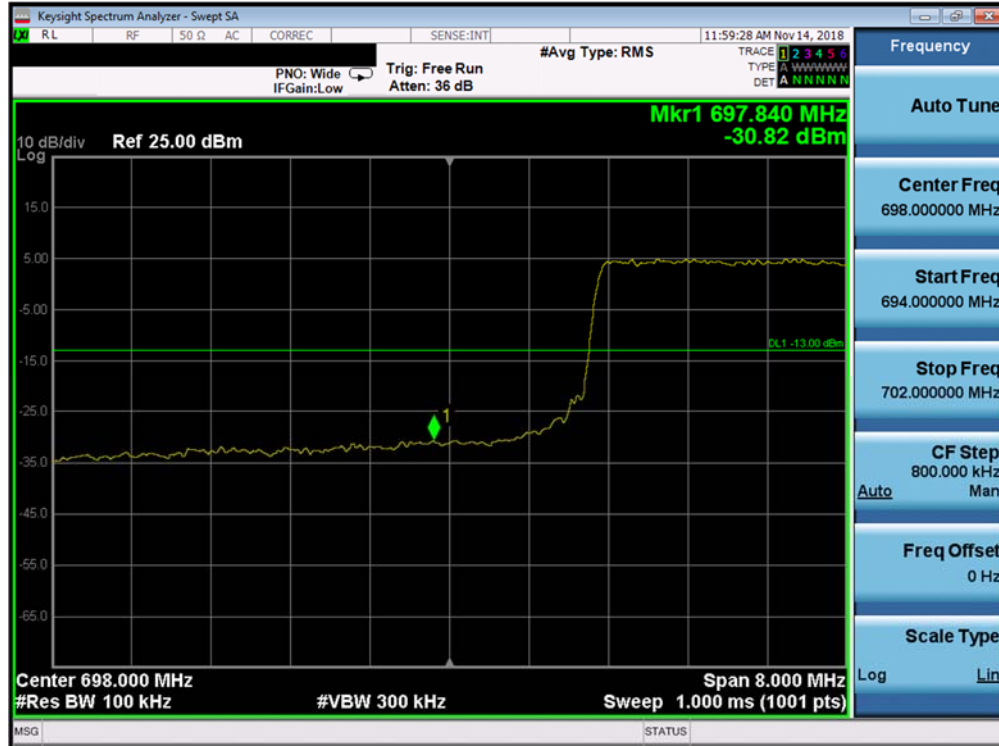
Plot 7-241. Lower Band Edge Plot (Band 12 - 10.0MHz QPSK - Full RB Configuration)
