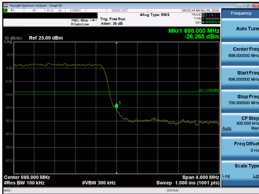
Plot 7-228. Upper Band Edge Plot (Band 71 - 5.0MHz QPSK - Full RB Configuration)
