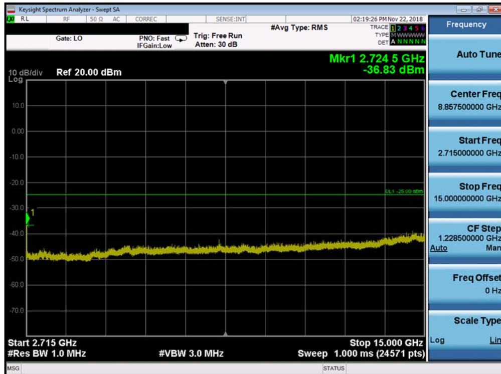
Plot 7-225. Conducted Spurious (Band 41/38 PC3- 15.0MHz QPSK -RB Size 1, RB Offset 0 -High Channel)
