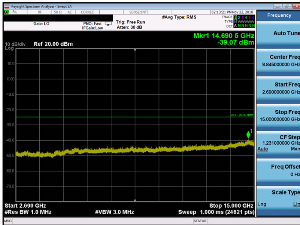
Plot 7-219. Conducted Spurious (Band 41/38 PC3- 15.0MHz QPSK - RB Size 1, RB Offset 0 -Low Channel)
