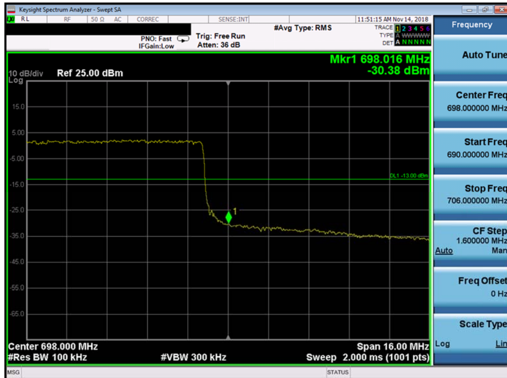
Plot 7-234. Upper Band Edge Plot (Band 71 - 20.0MHz QPSK - Full RB Configuration)
