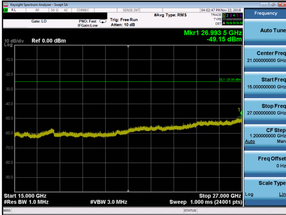
Plot 7-211. Conducted Spurious Plot (Band 41 PC2 - 15.0MHz QPSK -RB Size 1, RB Offset 0 -Low Channel)
