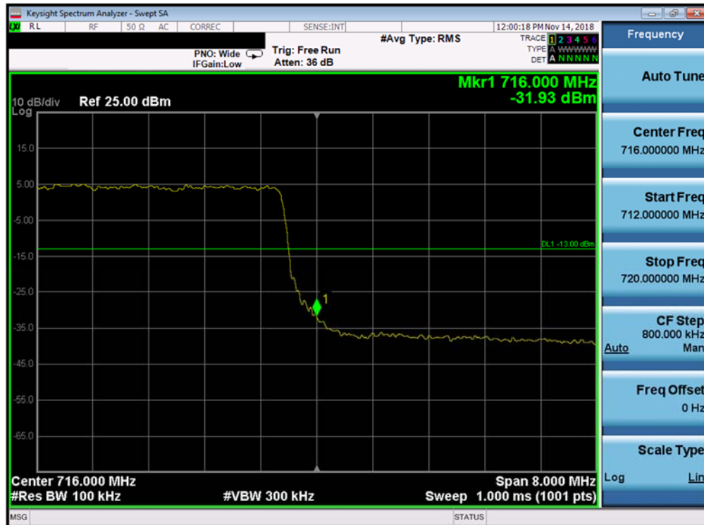
Plot 7-242. Upper Band Edge Plot (Band 12 - 10.0MHz QPSK - Full RB Configuration)
