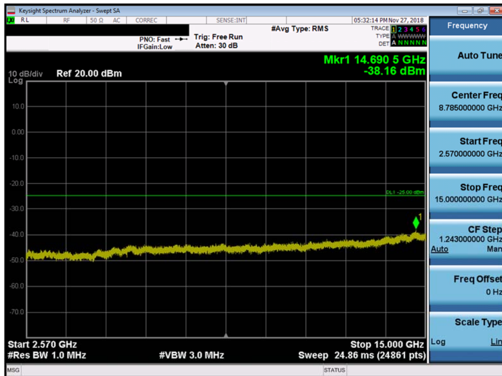
Plot 7-201. Conducted Spurious Plot (Band 7 - 20.0MHz QPSK - RB Size 1, RB Offset 0 - Low Channel)
