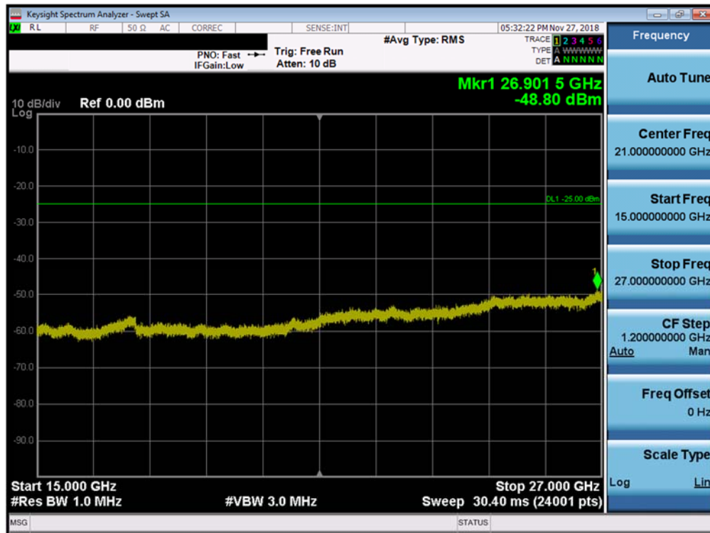
Plot 7-202. Conducted Spurious Plot (Band 7 - 20.0MHz QPSK - RB Size 1, RB Offset 0 - Low Channel)
