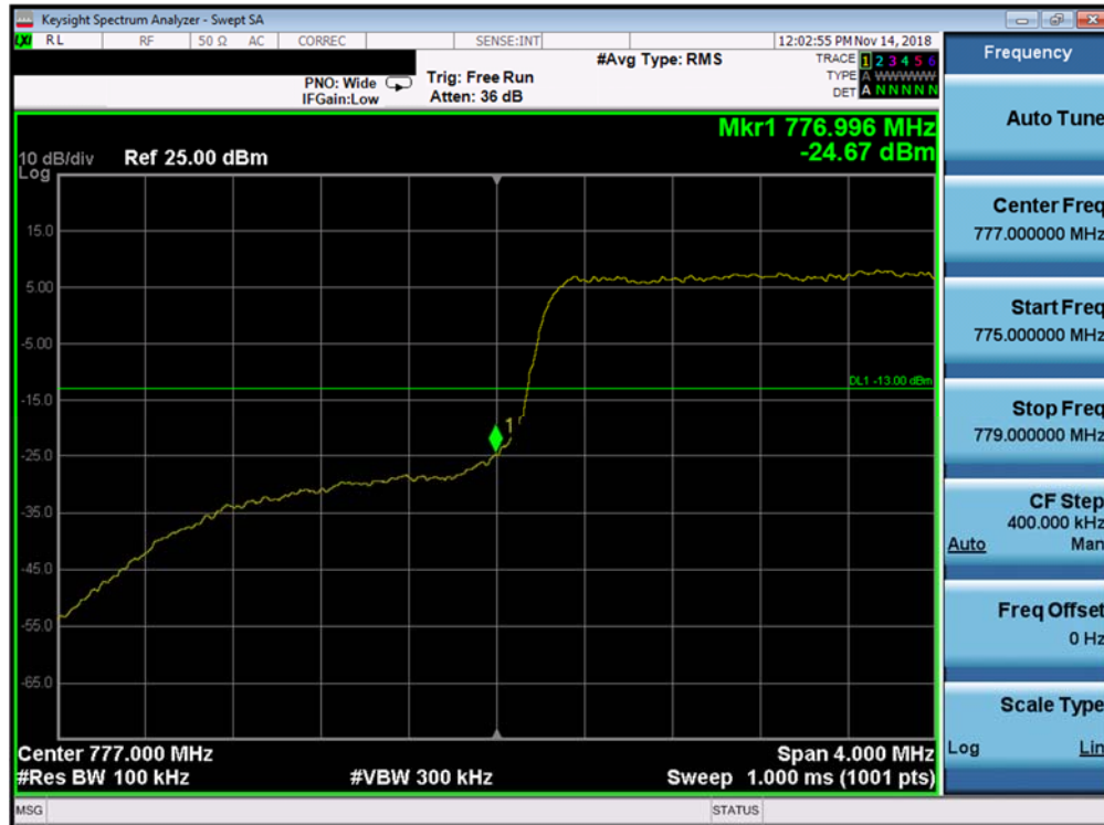
Plot 7-243. Lower Band Edge Plot (Band 13 - 5.0MHz QPSK - Full RB Configuration)
