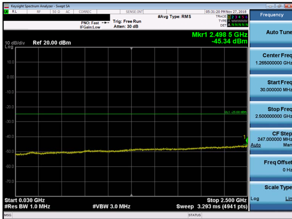
Plot 7-203. Conducted Spurious Plot (Band 7 - 20.0MHz QPSK - RB Size 1, RB Offset 0 - Mid Channel)
