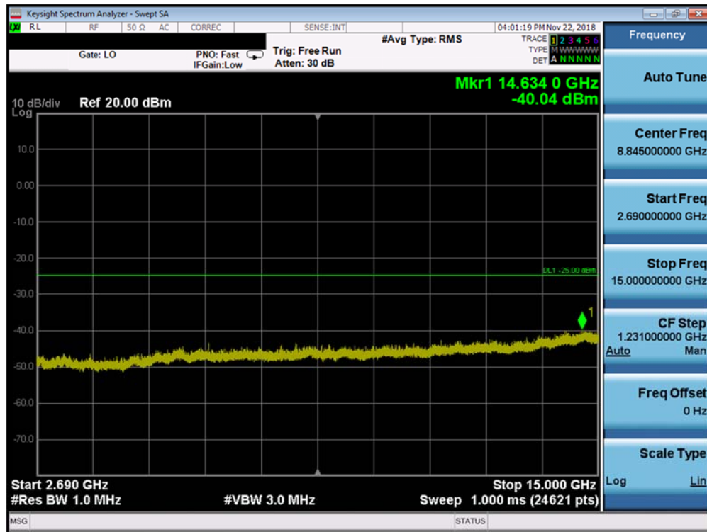
Plot 7-210. Conducted Spurious Plot (Band 41 PC2- 15.0MHz QPSK - RB Size 1, RB Offset 0 -Low Channel)
