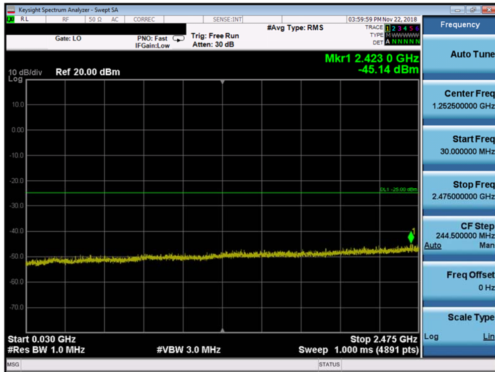
Plot 7-209. Conducted Spurious Plot (Band 41 PC2 - 15.0MHz QPSK -RB Size 1, RB Offset 0 -Low Channel)
