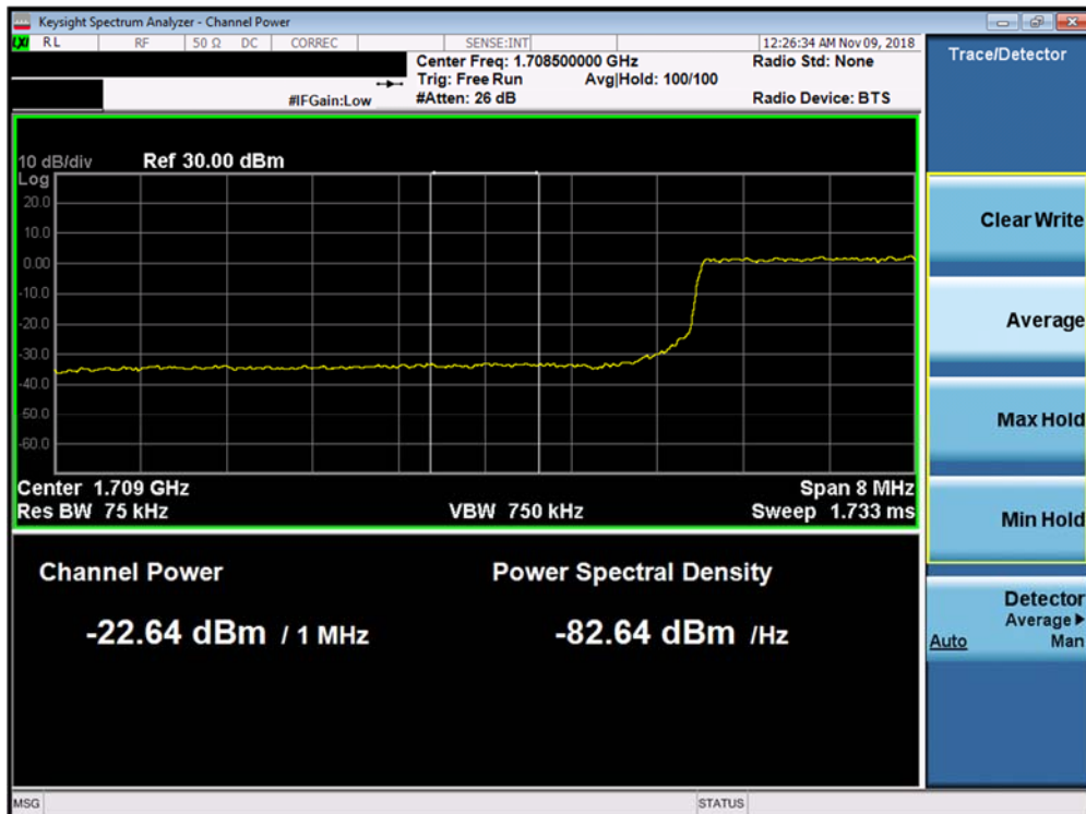
Plot 7-280. Lower Extended Band Edge Plot (Band 66/4 - 10.0MHz QPSK - Full RB Configuration)
