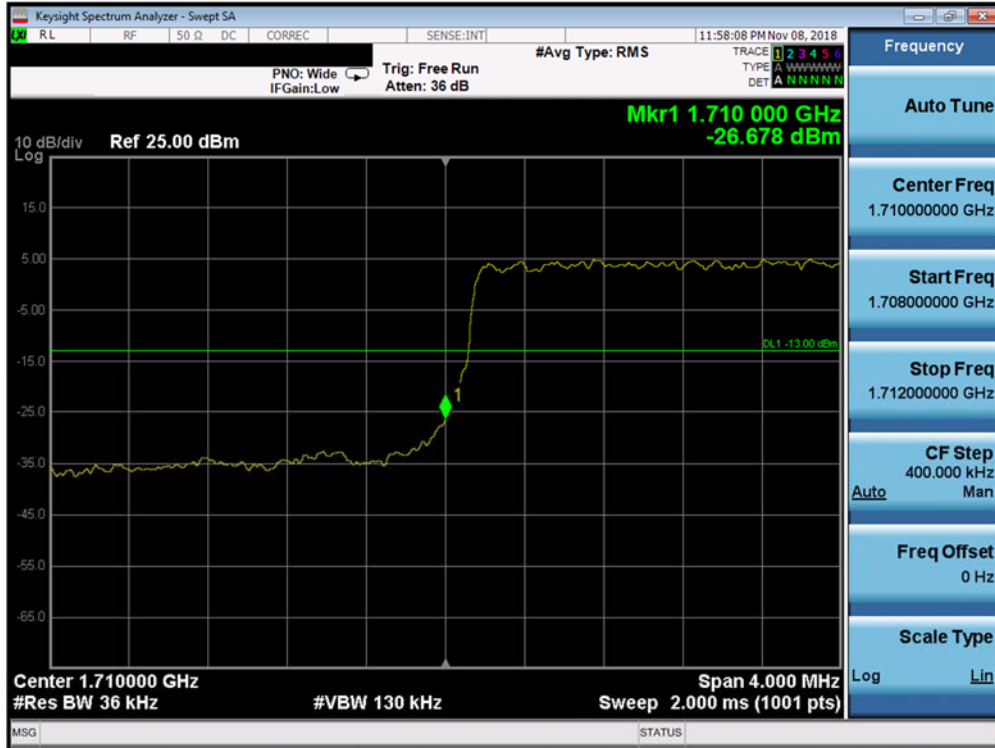
Plot 7-267. Lower Band Edge Plot (Band 66/4 - 3.0MHz QPSK - Full RB Configuration)
