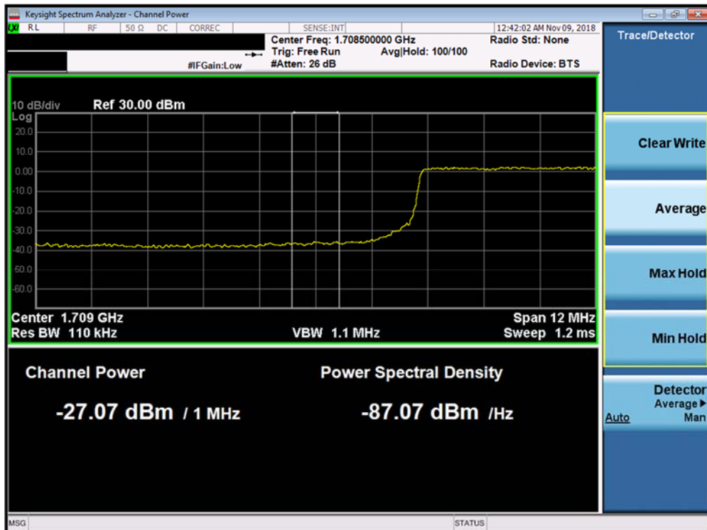
Plot 7-286. Lower Extended Band Edge Plot (Band 66/4 - 15.0MHz QPSK - Full RB Configuration)
