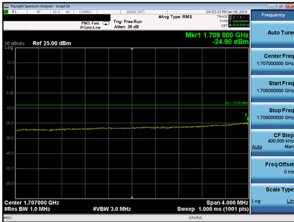
Plot 7-292. Lower Extended Band Edge Plot (Band 66/4 - 20.0MHz QPSK - Full RB Configuration)
