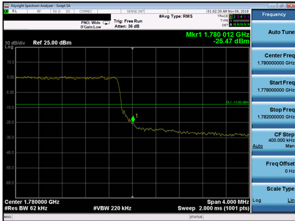
Plot 7-277. Upper Band Edge Plot (Band 66 - 5.0MHz QPSK - Full RB Configuration)
