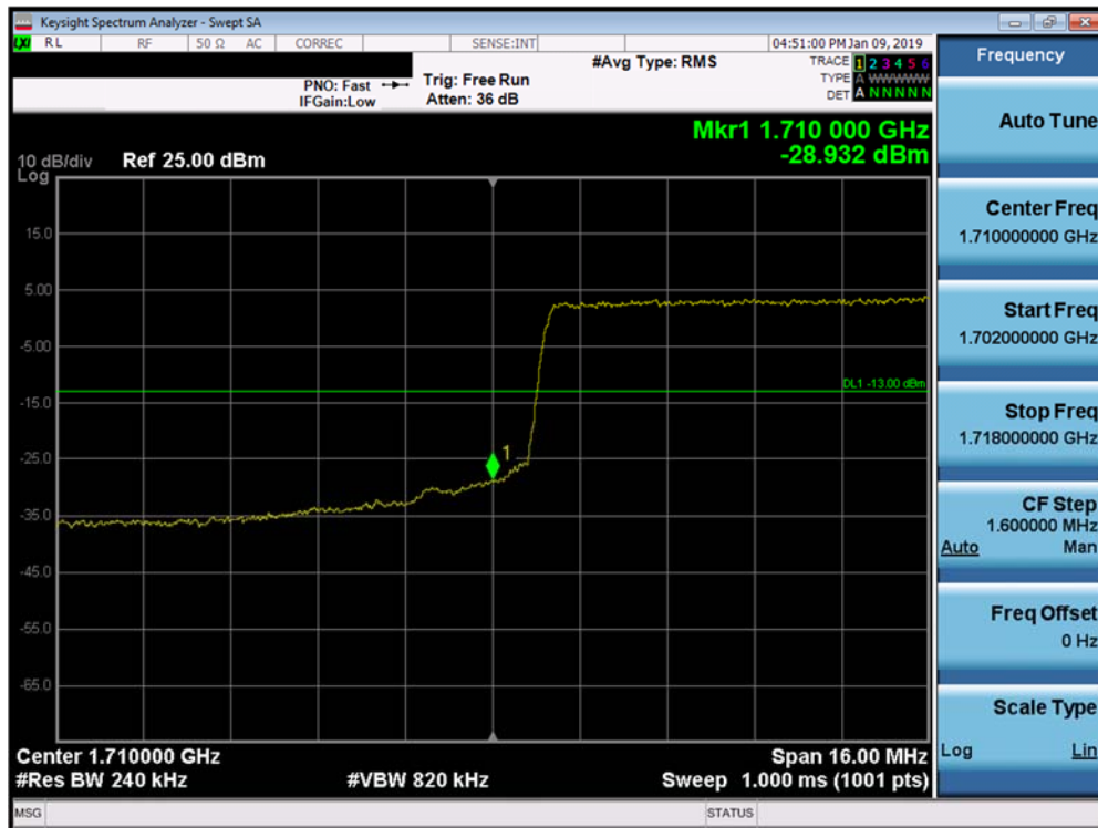
Plot 7-291. Lower Band Edge Plot (Band 66/4 - 20.0MHz QPSK - Full RB Configuration)
