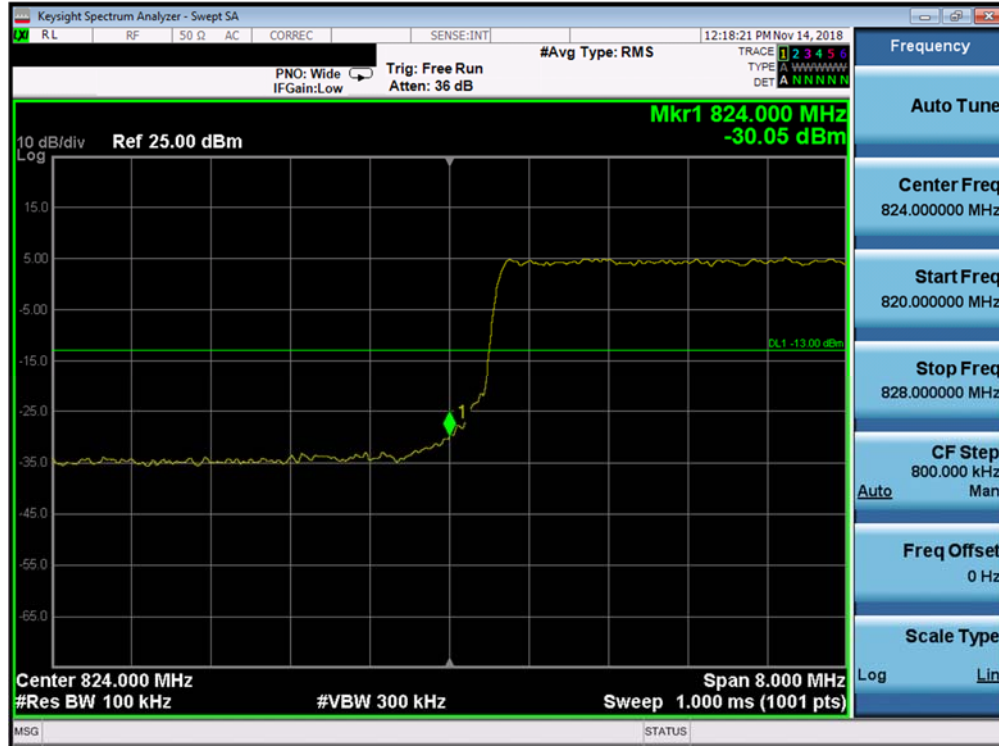
Plot 7-257. Lower Band Edge Plot (Band 26/5 - 10.0MHz QPSK - Full RB Configuration)
