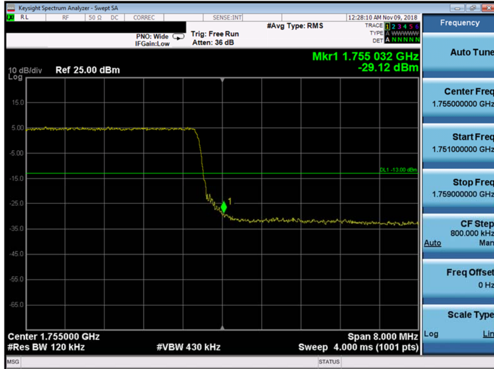
Plot 7-281. Upper Band Edge Plot (Band 4 - 10.0MHz QPSK - Full RB Configuration)
