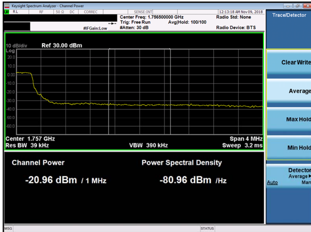
Plot 7-276. Upper Extended Band Edge Plot (Band 4 - 5.0MHz QPSK - Full RB Configuration)
