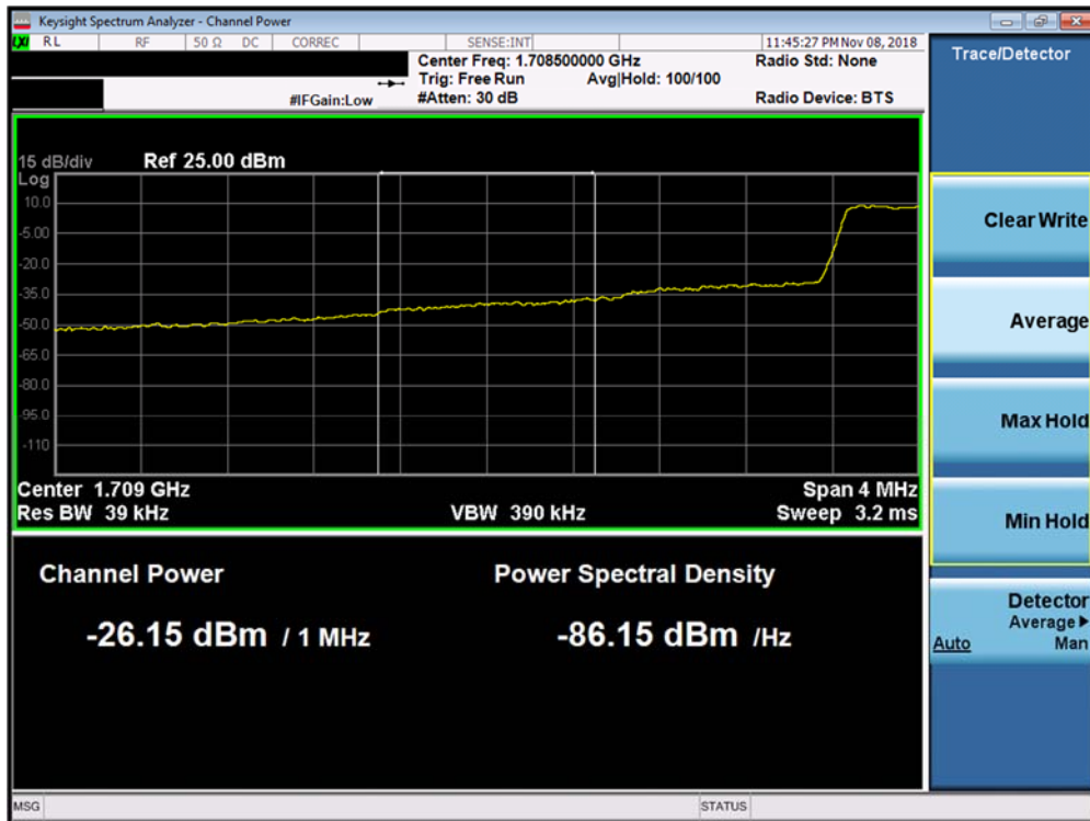
Plot 7-262. Lower Extended Band Edge Plot (Band 66/4 - 1.4MHz QPSK - Full RB Configuration)
