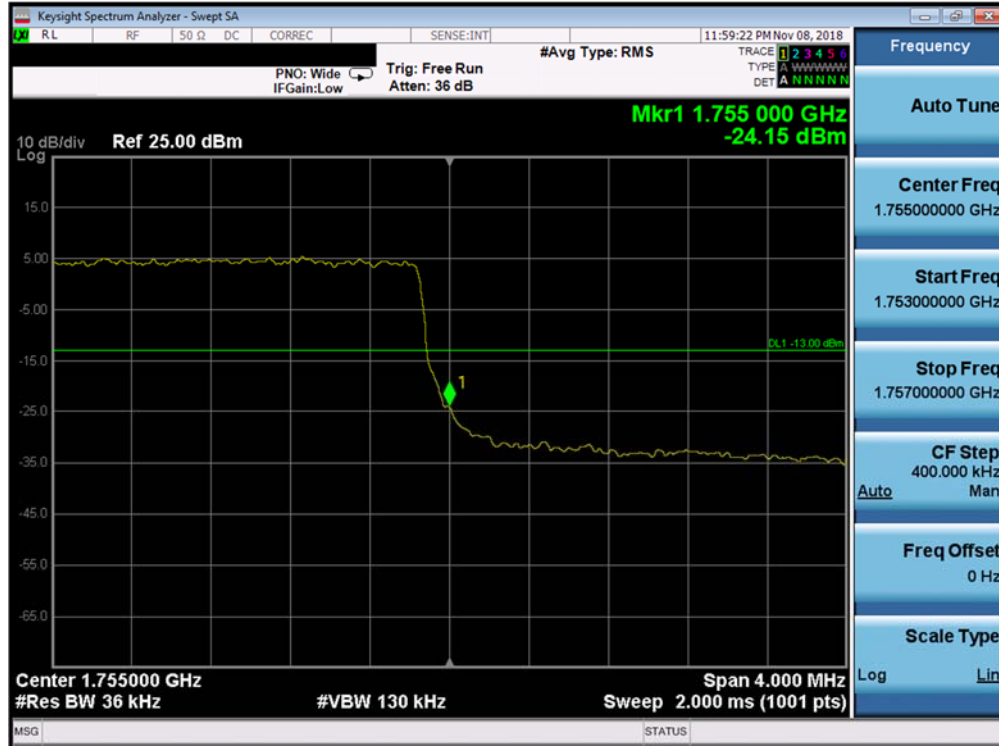
Plot 7-269. Upper Band Edge Plot (Band 4 - 3.0MHz QPSK - Full RB Configuration)
