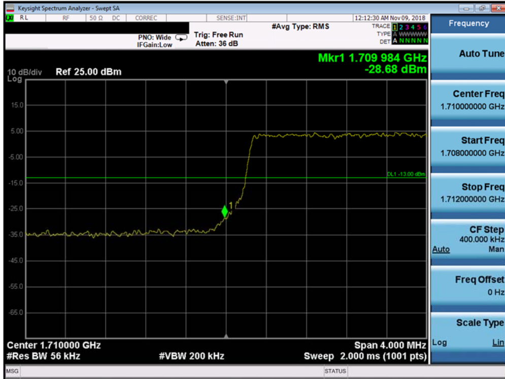
Plot 7-273. Lower Band Edge Plot (Band 66/4 - 5.0MHz QPSK - Full RB Configuration)
