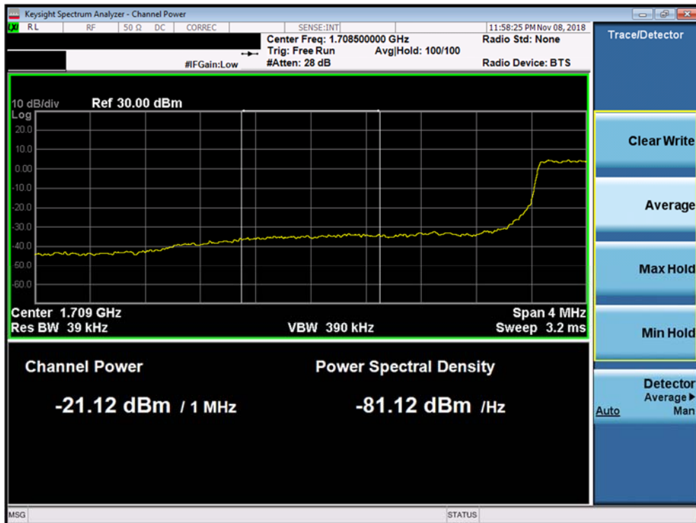
Plot 7-268. Lower Extended Band Edge Plot (Band 66/4 - 3.0MHz QPSK - Full RB Configuration)
