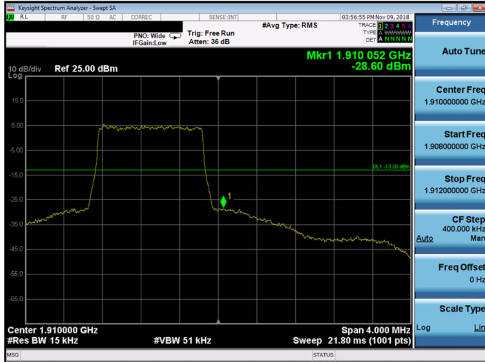
Plot 7-299. Upper Band Edge Plot (Band 2 - 1.4MHz QPSK - Full RB Configuration)
