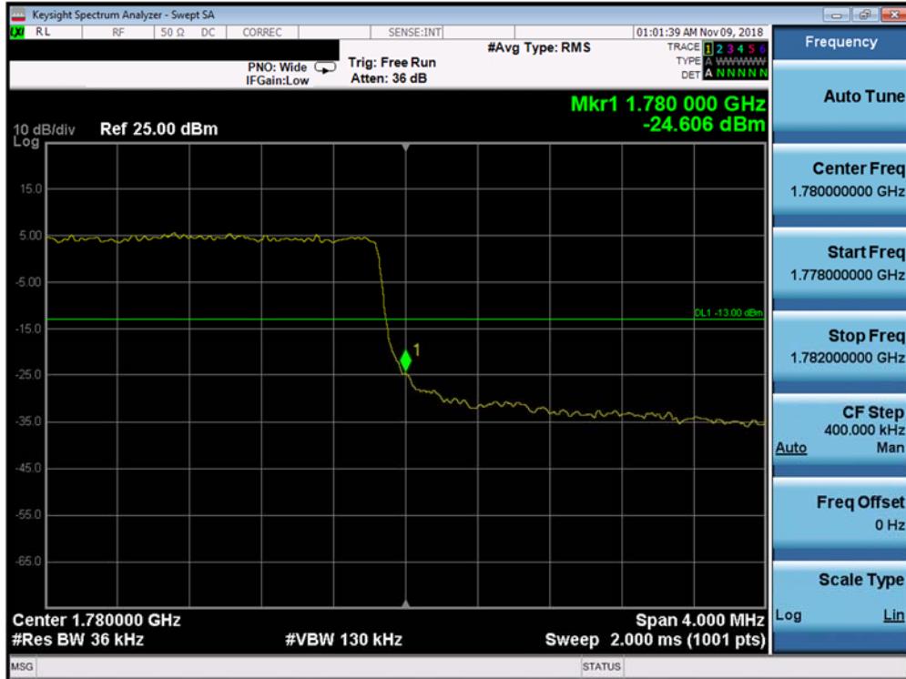
Plot 7-271. Upper Band Edge Plot (Band 66 - 3.0MHz QPSK - Full RB Configuration)
