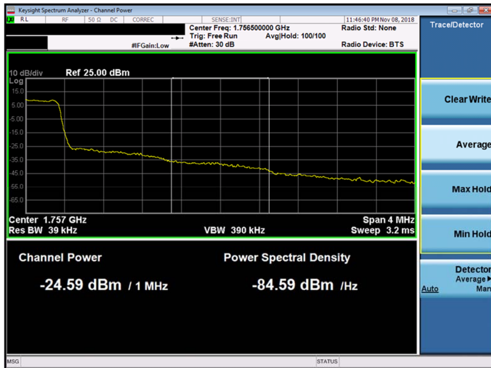
Plot 7-264. Upper Extended Band Edge Plot (Band 4 - 1.4MHz QPSK - Full RB Configuration)
