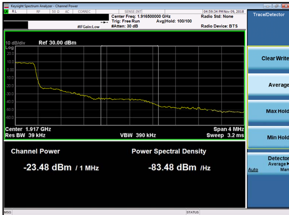
Plot 7-302. Upper Extended Band Edge Plot (Band 25 - 1.4MHz QPSK - Full RB Configuration)
