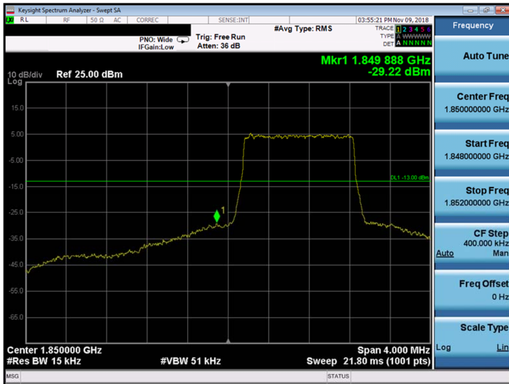
Plot 7-297. Lower Band Edge Plot (Band 25/2 - 1.4MHz QPSK - Full RB Configuration)
