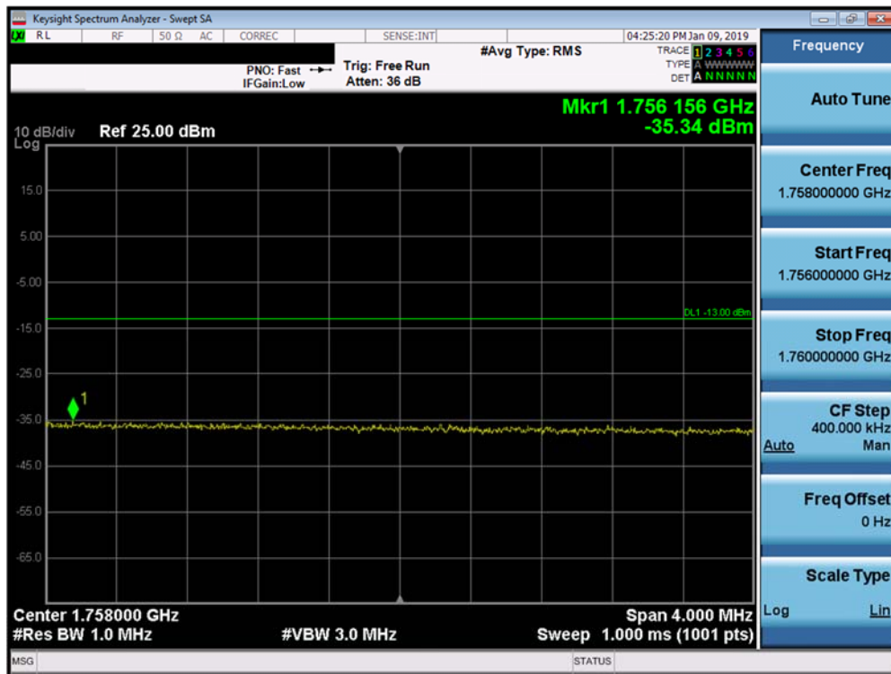
Plot 7-294. Upper Extended Band Edge Plot (Band 4 - 20.0MHz QPSK - Full RB Configuration)
