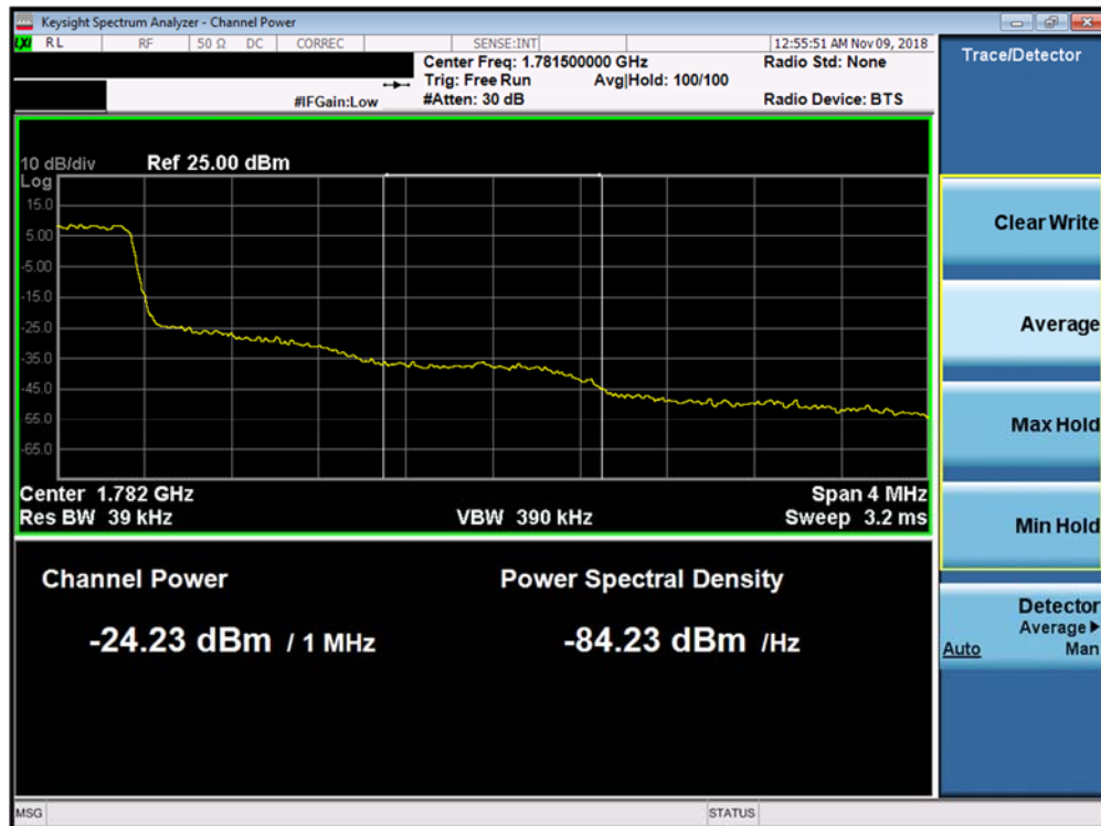
Plot 7-266. Upper Extended Band Edge Plot (Band 66 - 1.4MHz QPSK - Full RB Configuration)
