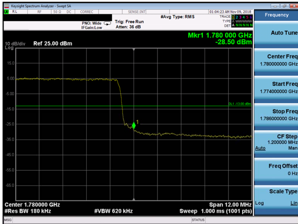
Plot 7-289. Upper Band Edge Plot (Band 66 - 15.0MHz QPSK - Full RB Configuration)
