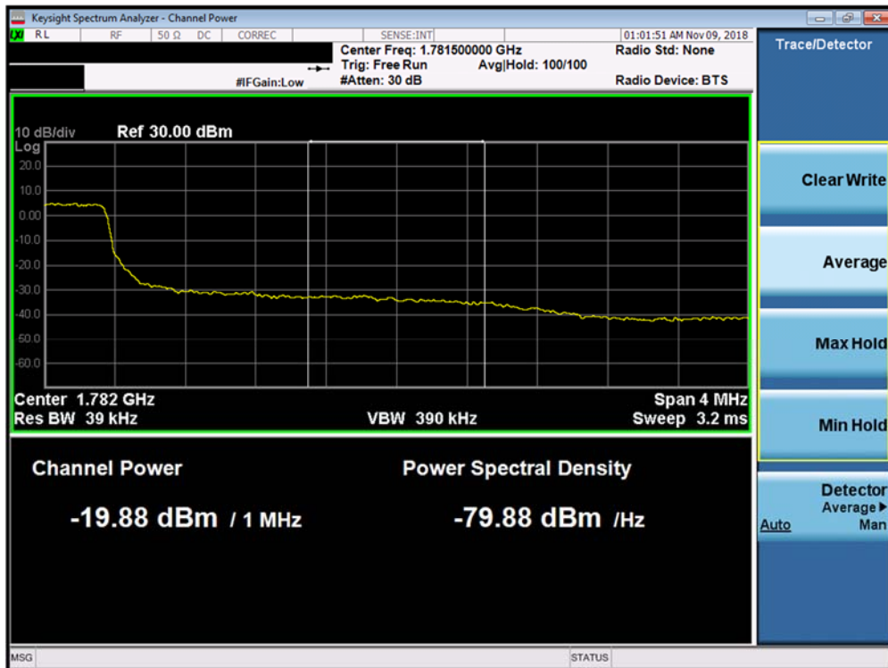
Plot 7-272. Upper Extended Band Edge Plot (Band 66 - 3.0MHz QPSK - Full RB Configuration)
