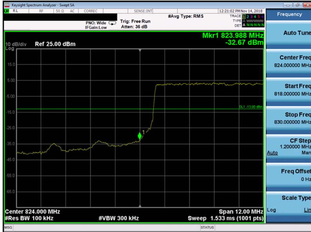
Plot 7-259. Lower Band Edge Plot (Band 26 - 15.0MHz QPSK - Full RB Configuration)
