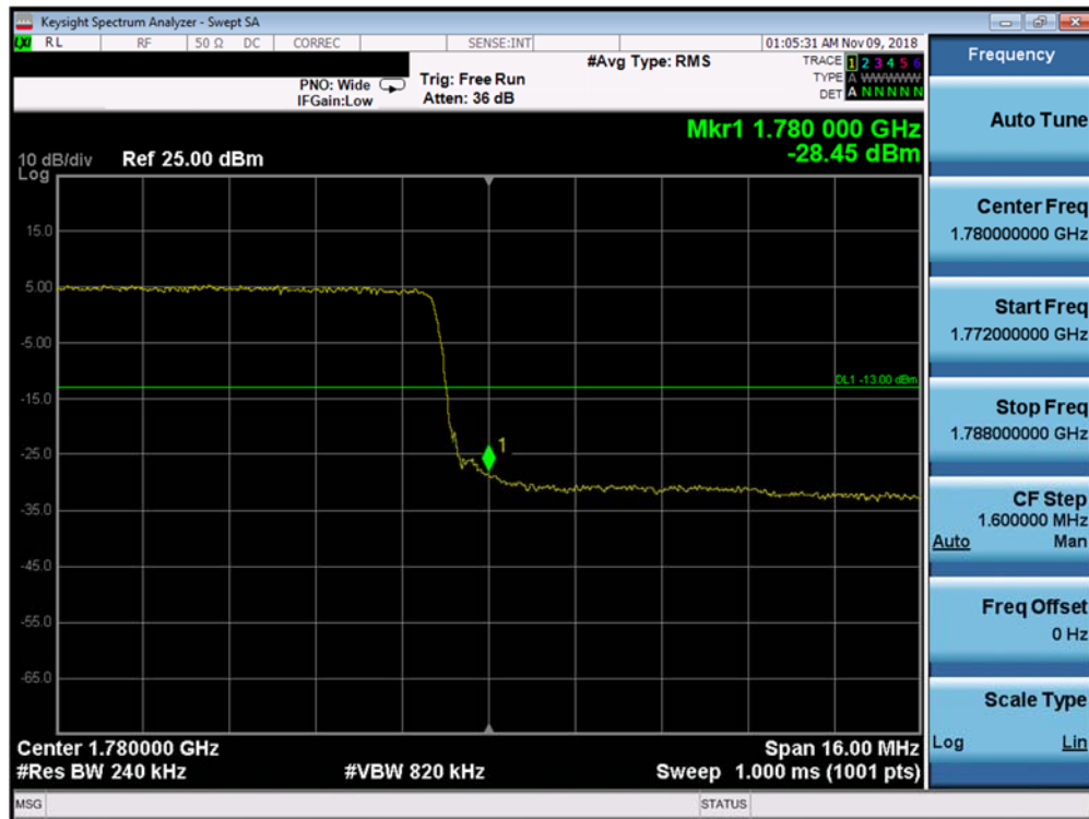
Plot 7-295. Upper Band Edge Plot (Band 66 - 20.0MHz QPSK - Full RB Configuration)
