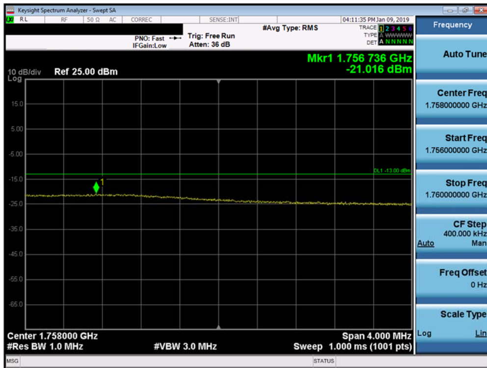
Plot 7-288. Upper Extended Band Edge Plot (Band 4 - 15.0MHz QPSK - Full RB Configuration)
