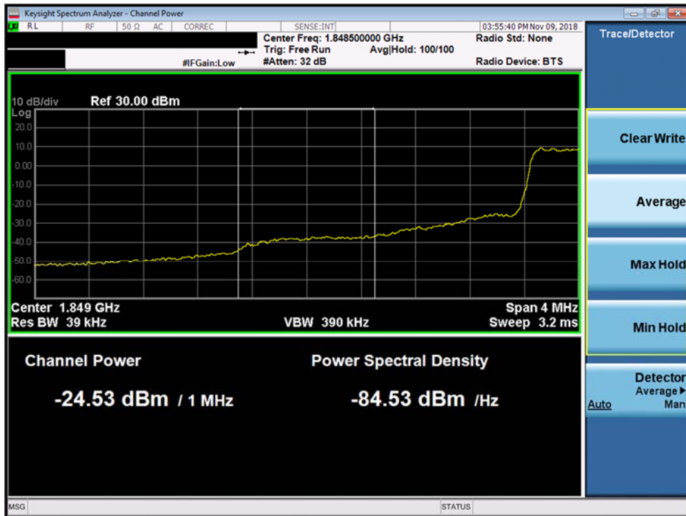
Plot 7-298. Lower Extended Band Edge Plot (Band 25/2 - 1.4MHz QPSK - Full RB Configuration)
