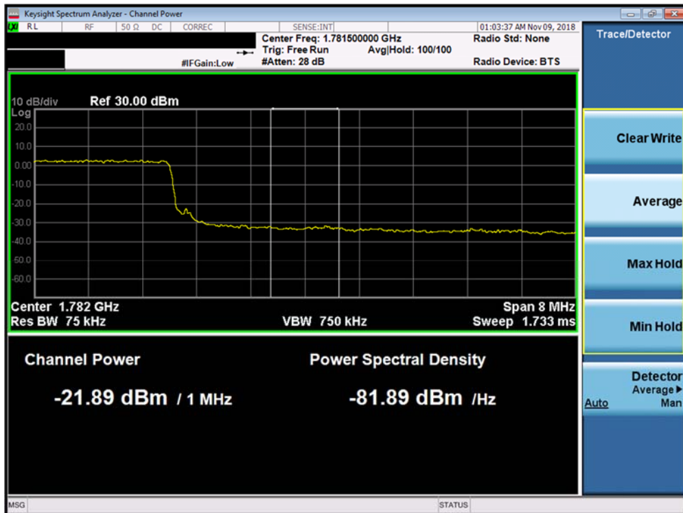
Plot 7-284. Upper Extended Band Edge Plot (Band 66 - 10.0MHz QPSK - Full RB Configuration)
