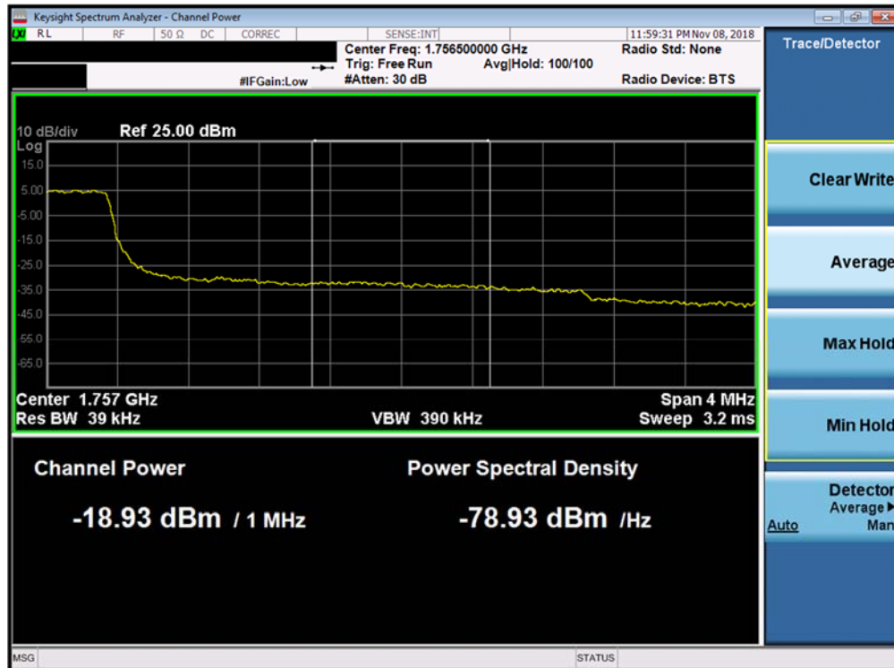
Plot 7-270. Upper Extended Band Edge Plot (Band 4 - 3.0MHz QPSK - Full RB Configuration)
