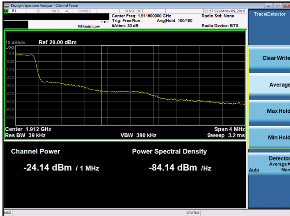
Plot 7-300. Upper Extended Band Edge Plot (Band 2 - 1.4MHz QPSK - Full RB Configuration)
