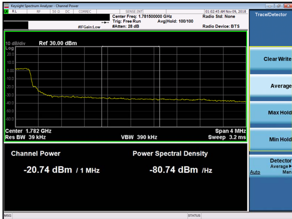
Plot 7-278. Upper Extended Band Edge Plot (Band 66 - 5.0MHz QPSK - Full RB Configuration)
