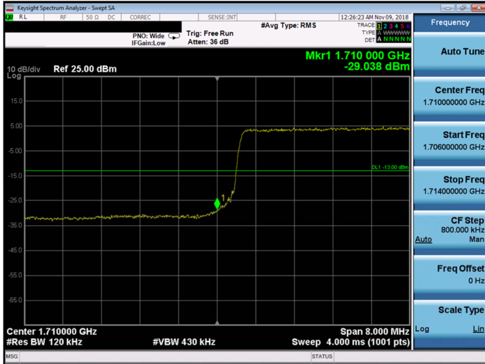
Plot 7-279. Lower Band Edge Plot (Band 66/4 - 10.0MHz QPSK - Full RB Configuration)
