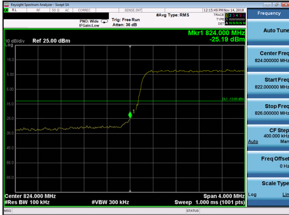
Plot 7-255. Lower Band Edge Plot (Band 26/5 - 5.0MHz QPSK - Full RB Configuration)
