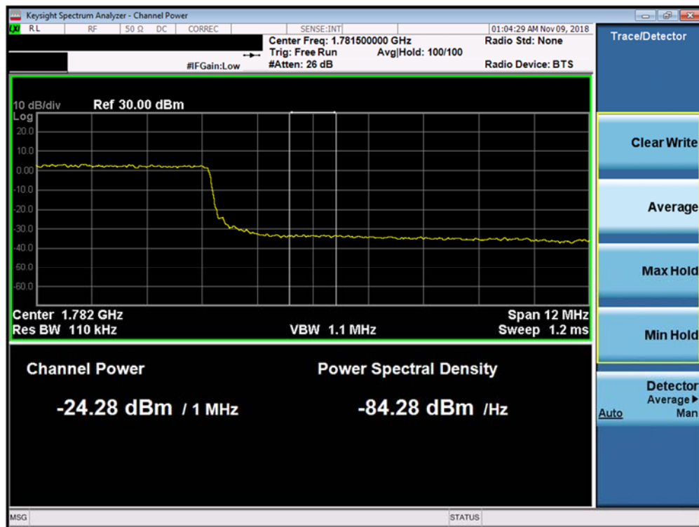
Plot 7-290. Upper Extended Band Edge Plot (Band 66 - 15.0MHz QPSK - Full RB Configuration)
