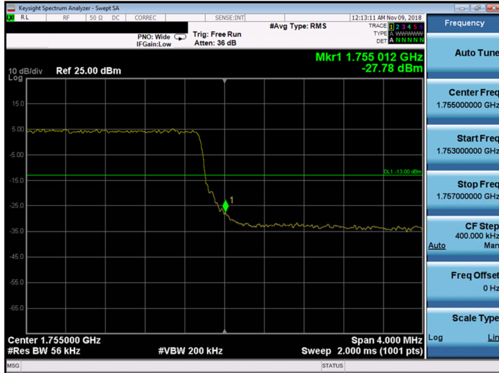
Plot 7-275. Upper Band Edge Plot (Band 4 - 5.0MHz QPSK - Full RB Configuration)
