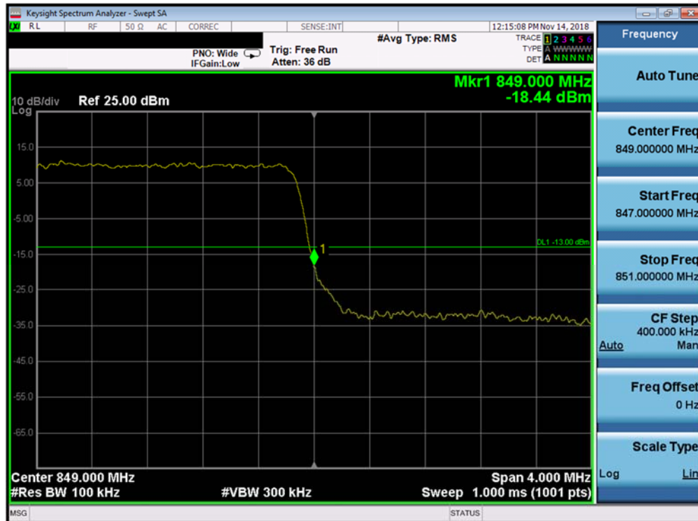
Plot 7-254. Upper Band Edge Plot (Band 26/5 - 3.0MHz QPSK - Full RB Configuration)
