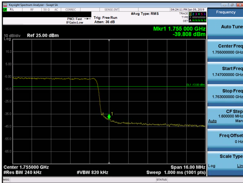
Plot 7-293. Upper Band Edge Plot (Band 4 - 20.0MHz QPSK - Full RB Configuration)
