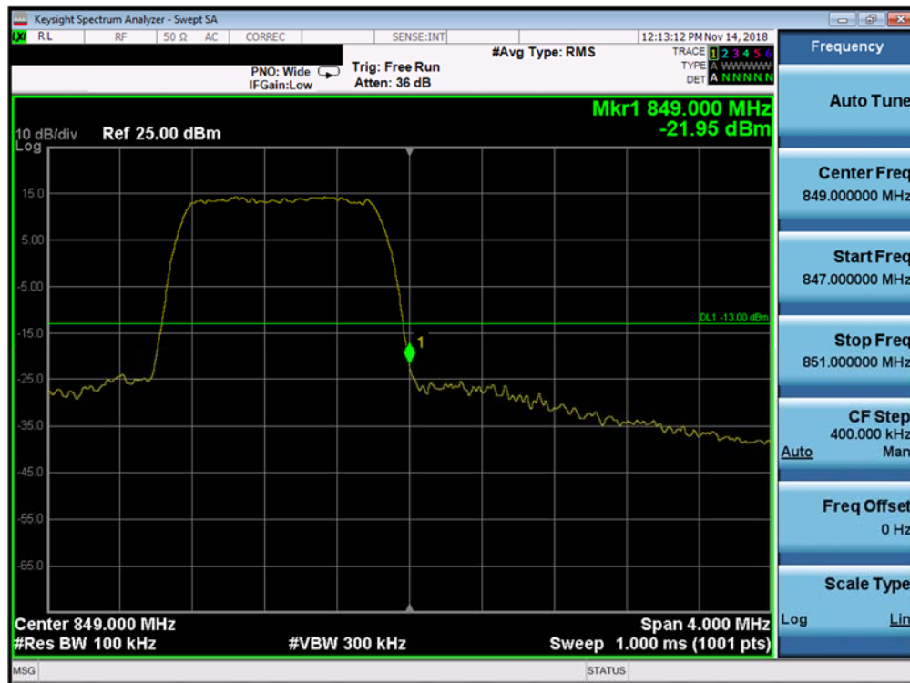
Plot 7-252. Upper Band Edge Plot (Band 26/5 - 1.4MHz QPSK - Full RB Configuration)
