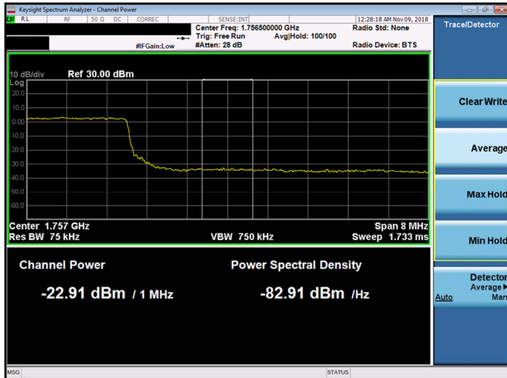
Plot 7-282. Upper Extended Band Edge Plot (Band 4 - 10.0MHz QPSK - Full RB Configuration)
