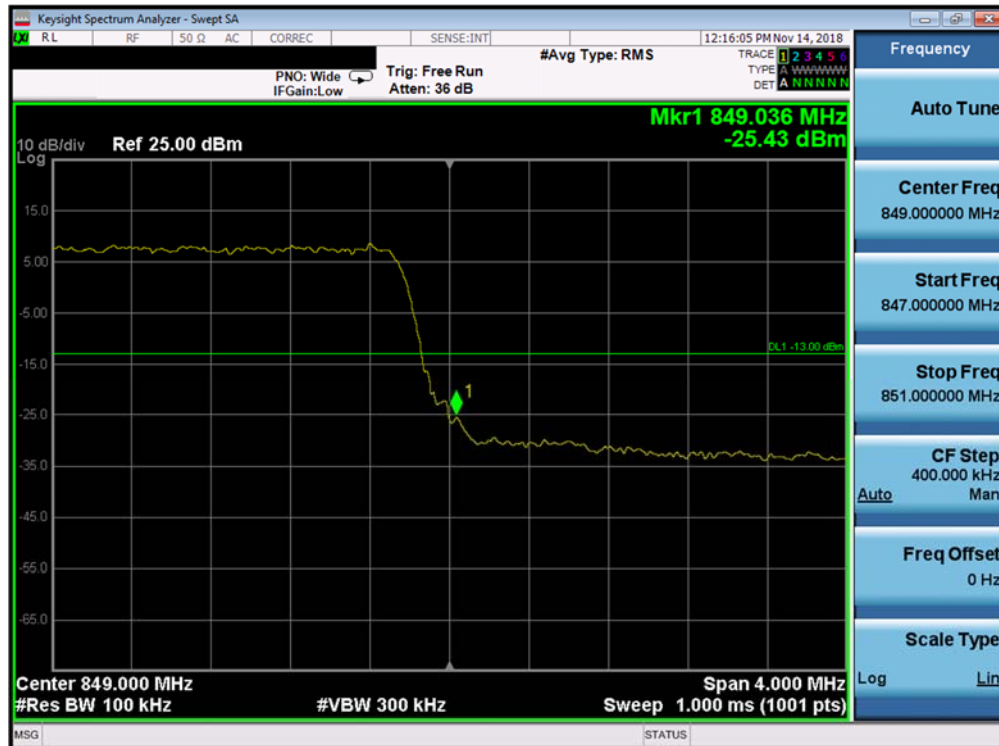
Plot 7-256. Upper Band Edge Plot (Band 26/5 - 5.0MHz QPSK - Full RB Configuration)
