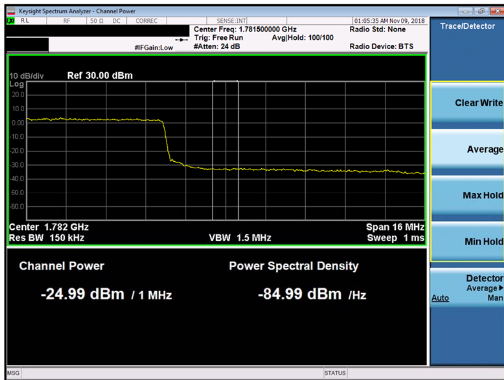
Plot 7-296. Upper Extended Band Edge Plot (Band 66 - 20.0MHz QPSK - Full RB Configuration)
