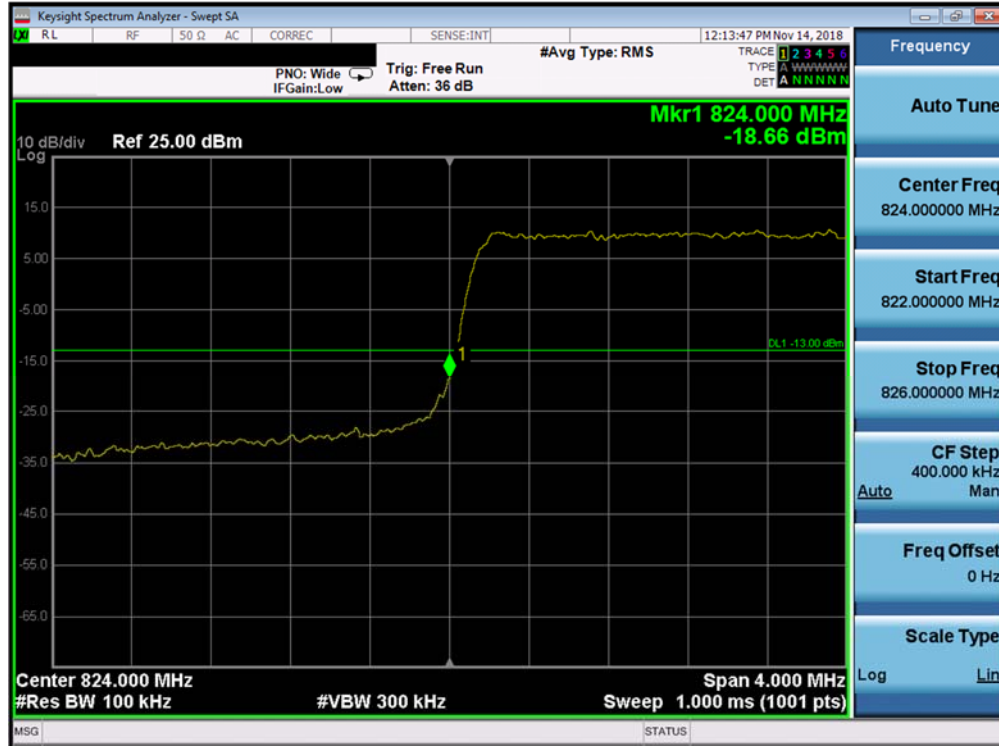
Plot 7-253. Lower Band Edge Plot (Band 26/5 - 3.0MHz QPSK - Full RB Configuration)
