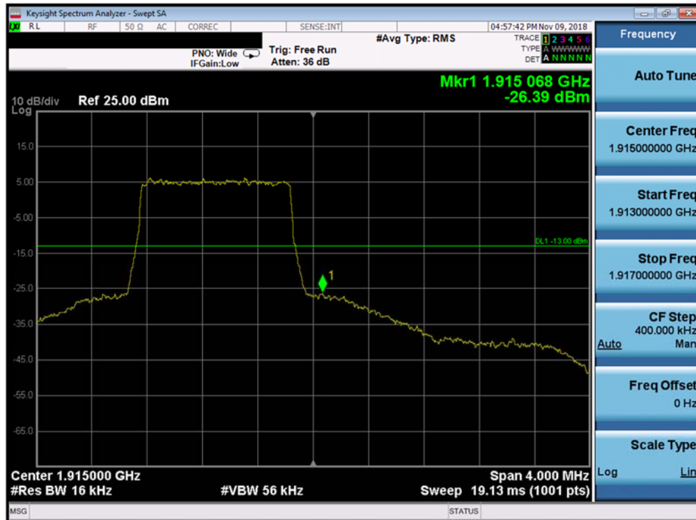
Plot 7-301. Upper Band Edge Plot (Band 25 - 1.4MHz QPSK - Full RB Configuration)
