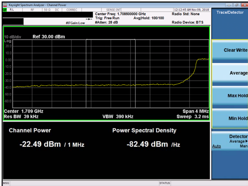
Plot 7-274. Lower Extended Band Edge Plot (Band 66/4 - 5.0MHz QPSK - Full RB Configuration)
