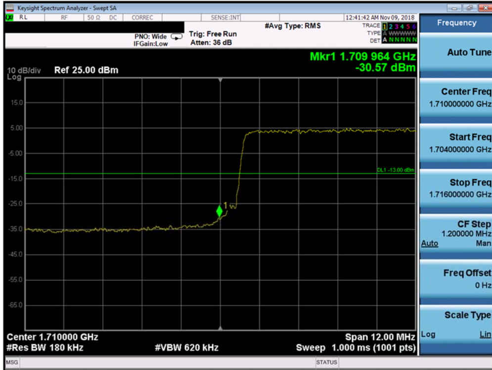
Plot 7-285. Lower Band Edge Plot (Band 66/4 - 15.0MHz QPSK - Full RB Configuration)
