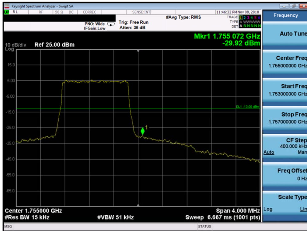
Plot 7-263. Upper Band Edge Plot (Band 4 - 1.4MHz QPSK - Full RB Configuration)
