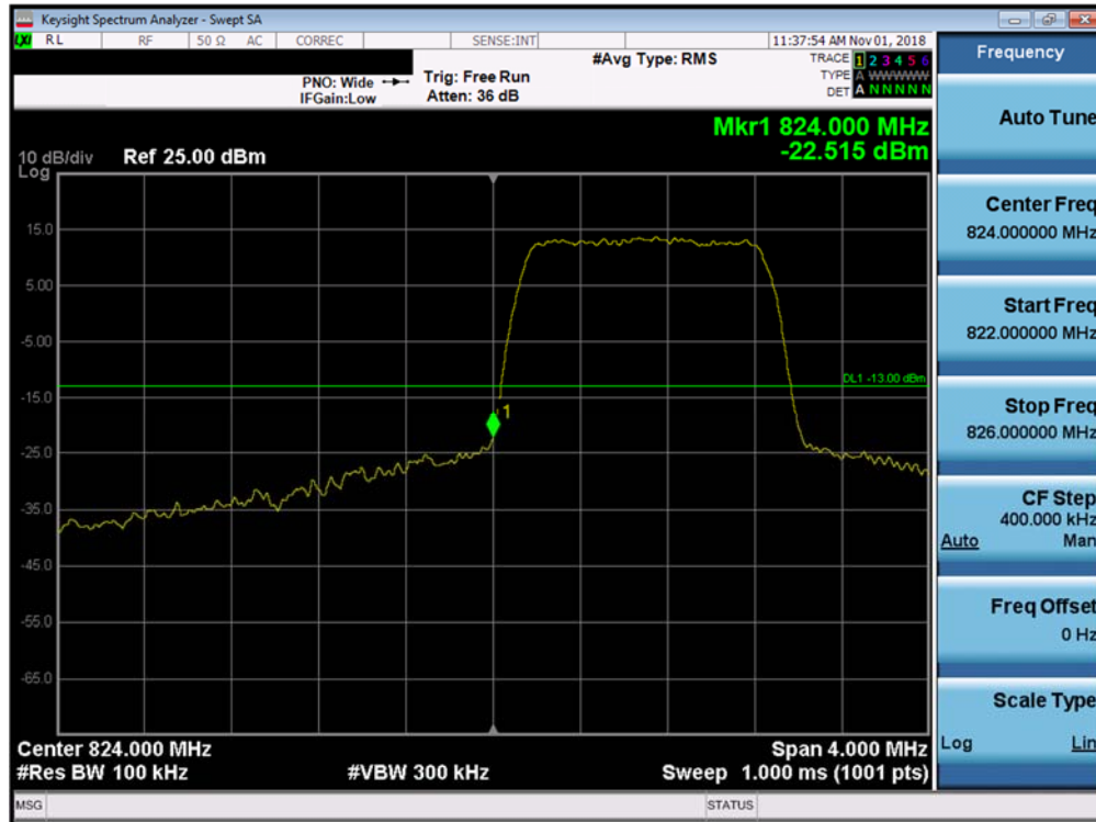
Plot 7-251. Lower Band Edge Plot (Band 26/5 - 1.4MHz QPSK - Full RB Configuration)
