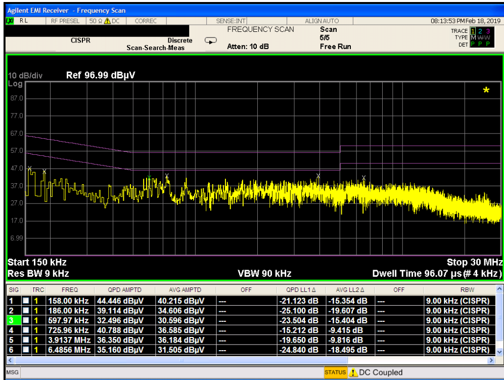
Plot 7-57. Line Conducted Plot with Bluetooth LE With WCP (L1)
