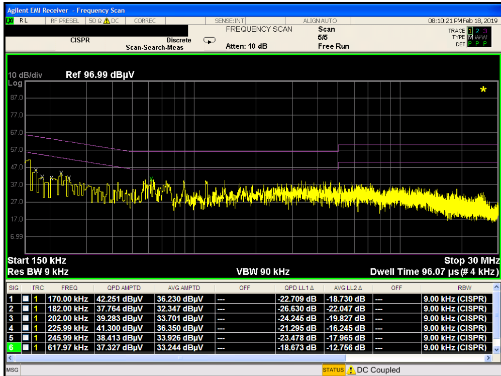
Plot 7-58. Line Conducted Plot with Bluetooth LE With WCP (N)
