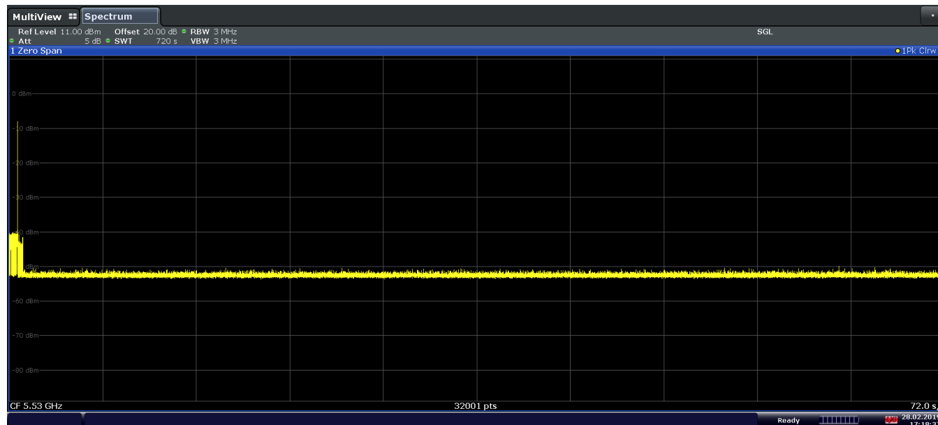
Figure 9-4. 5530MHz - Non-Occupancy Period (10 Minutes) - (40MHz)
