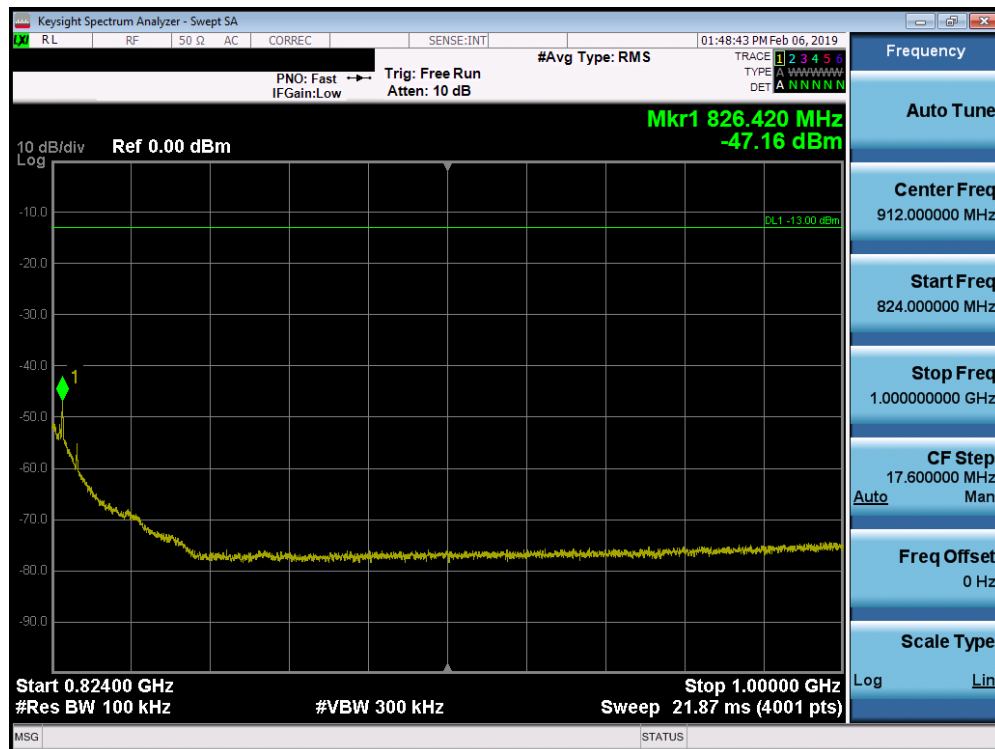
Plot 7-17. Conducted Spurious Plot (LTE Band 26, 10.0MHz QPSK – RB Size 1, RB Offset 0)
