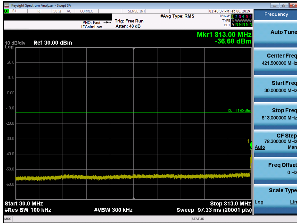
Plot 7-16. Conducted Spurious Plot (LTE Band 26, 10.0MHz QPSK – RB Size 1, RB Offset 0)
