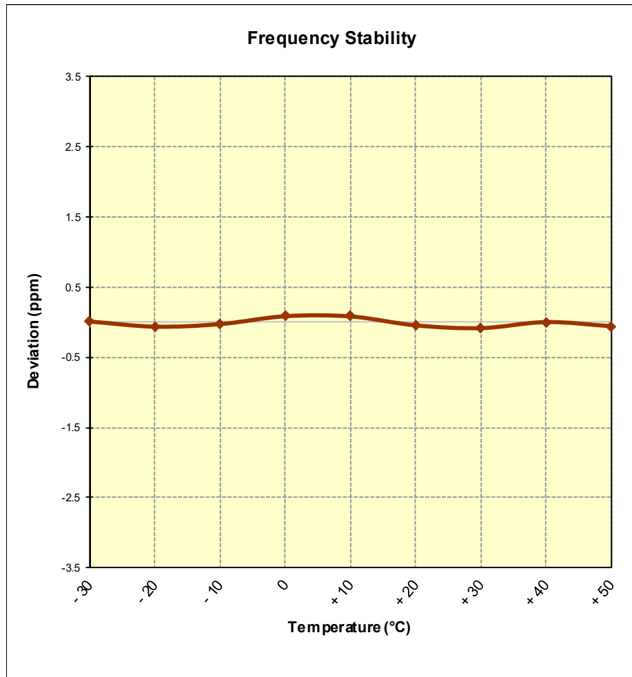
Figure 7-13. Frequency Stability Graph (PCS WCDMA Mode – Ch. 9400)
