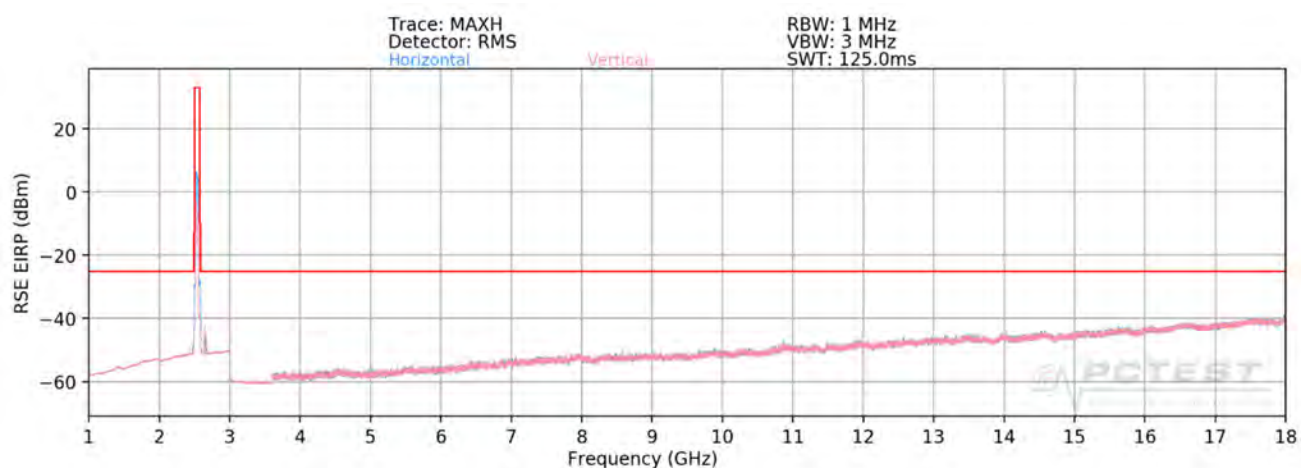
Plot 7-22. Radiated Spurious Plot (ULCA B7 PCC: RB 100 Offset 0, SCC: RB 100 Offset 0 – Mid Channel)
