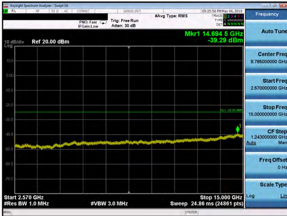
Plot 7-7. Conducted Spurious Plot (Band 7 – 20 MHz QPSK – PCC 100/0 SCC 100/0 – Mid Channel)
