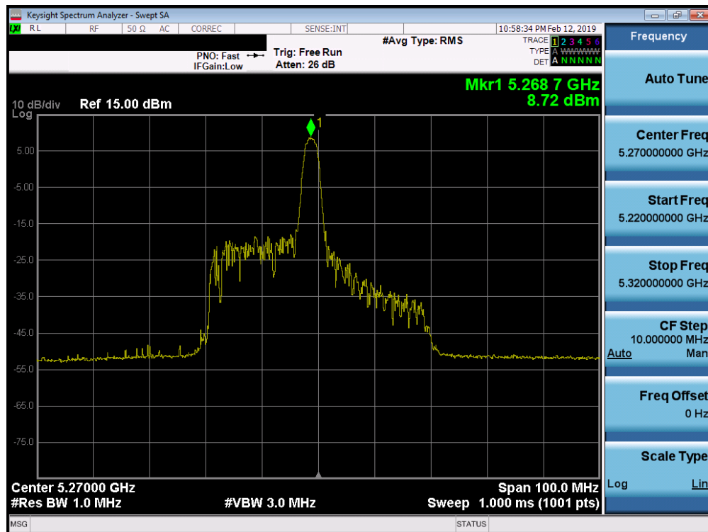
Plot 7-91. Power Spectral Density Plot SISO ANT2 (40MHz BW 802.11ax – 26 Tones (UNII Band 2A) – Ch. 54)
