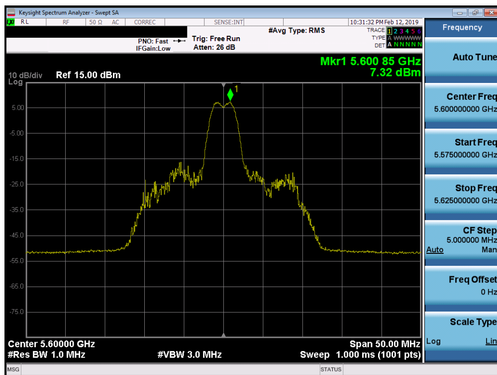
Plot 7-95. Power Spectral Density Plot SISO ANT2 (20MHz BW 802.11ax – 26 Tones (UNII Band 2C) – Ch. 120)
