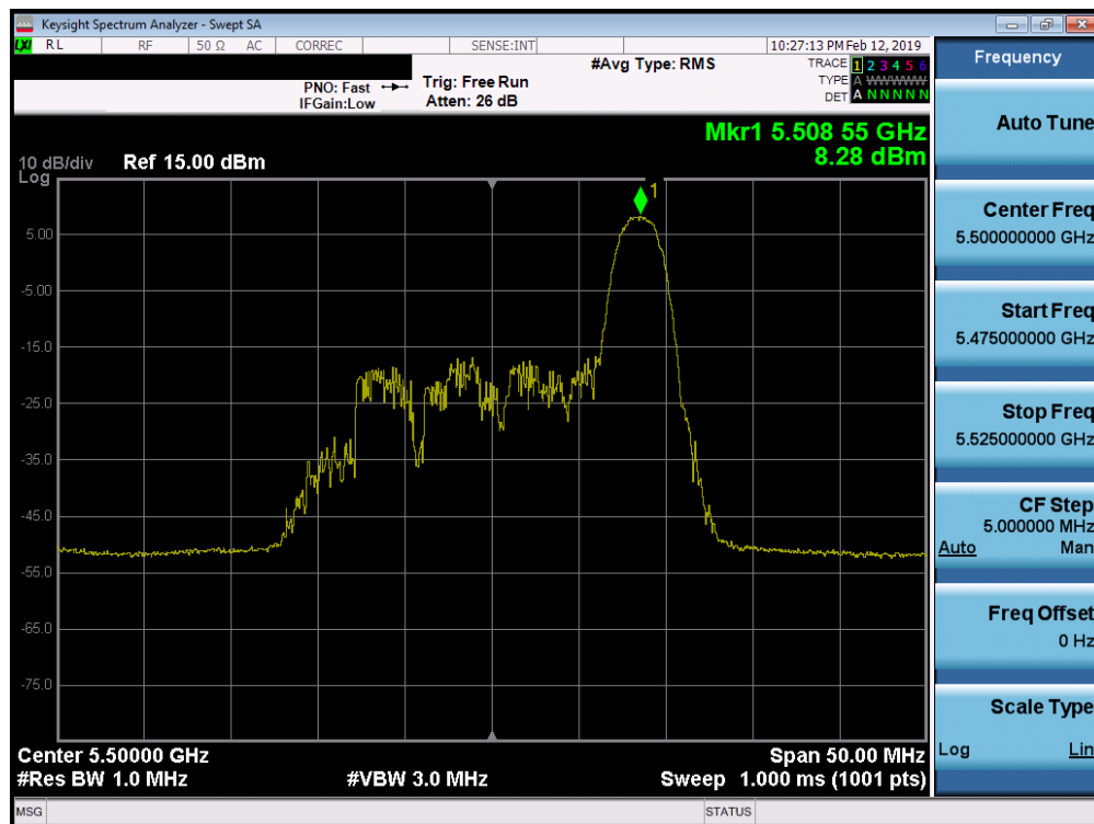
Plot 7-94. Power Spectral Density Plot SISO ANT2 (20MHz BW 802.11ax – 26 Tones (UNII Band 2C) – Ch. 100)
