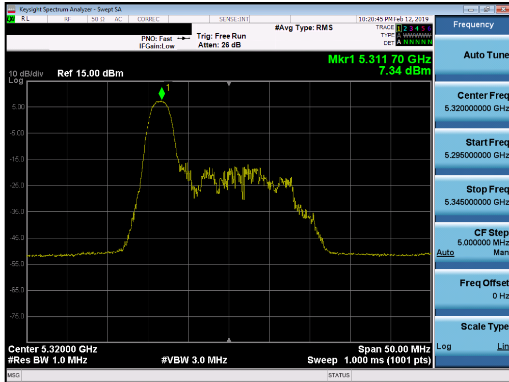
Plot 7-90. Power Spectral Density Plot SISO ANT2 (20MHz BW 802.11ax – 26 Tones (UNII Band 2A) – Ch. 64)
