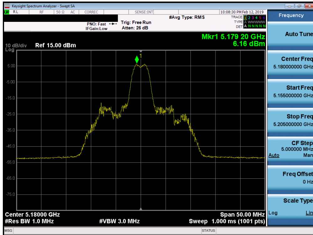
Plot 7-82. Power Spectral Density Plot SISO ANT2 (20MHz BW 802.11ax – 26 Tones (UNII Band 1) – Ch. 36)
