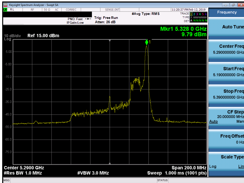
Plot 7-93. Power Spectral Density Plot SISO ANT2 (80MHz BW 802.11ax – 26 Tones (UNII Band 2A) – Ch. 58)
