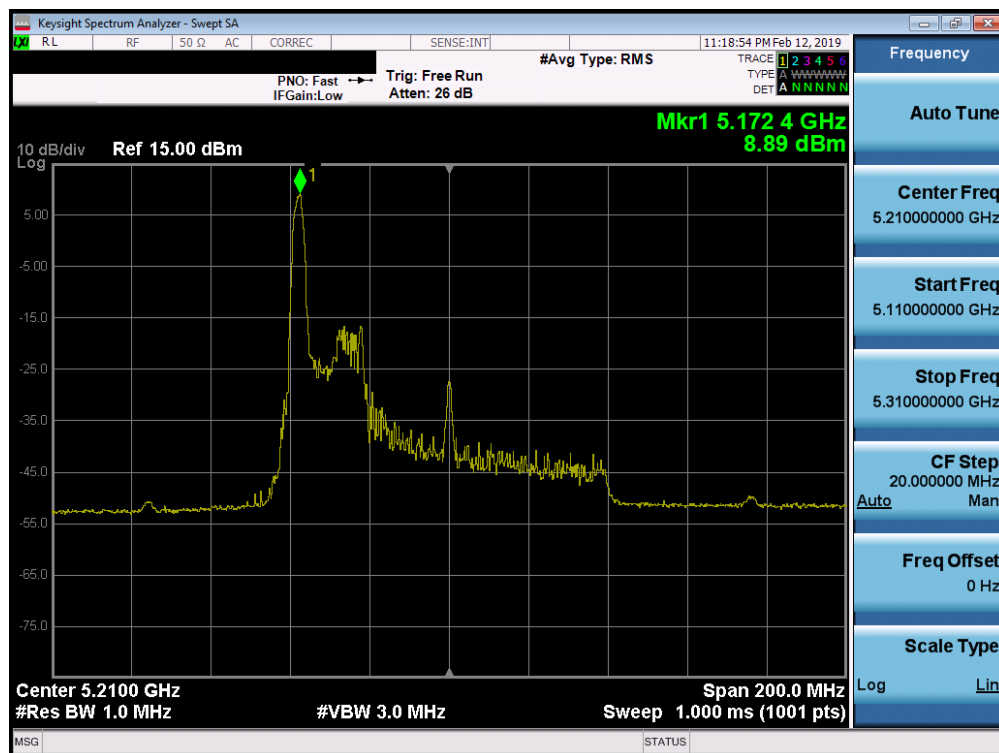
Plot 7-87. Power Spectral Density Plot SISO ANT2 (80MHz BW 802.11ax – 26 Tones (UNII Band 1) – Ch. 42)
