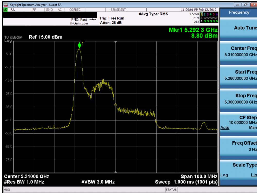
Plot 7-92. Power Spectral Density Plot SISO ANT2 (40MHz BW 802.11ax – 26 Tones (UNII Band 2A) – Ch. 62)
