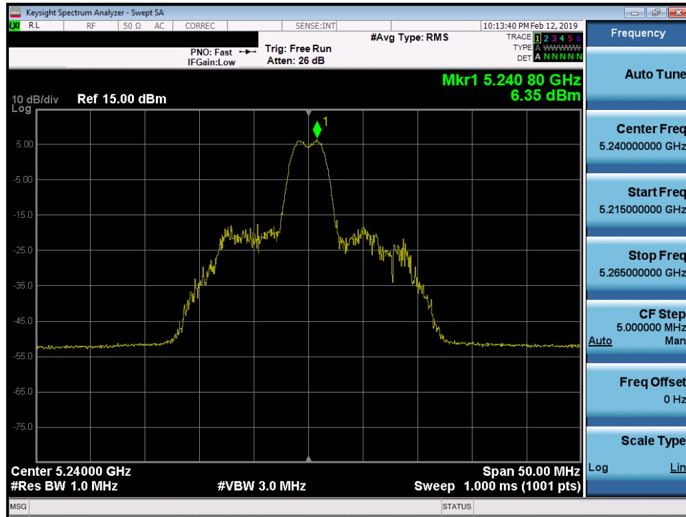
Plot 7-84. Power Spectral Density Plot SISO ANT2 (20MHz BW 802.11ax – 26 Tones (UNII Band 1) – Ch. 48)
