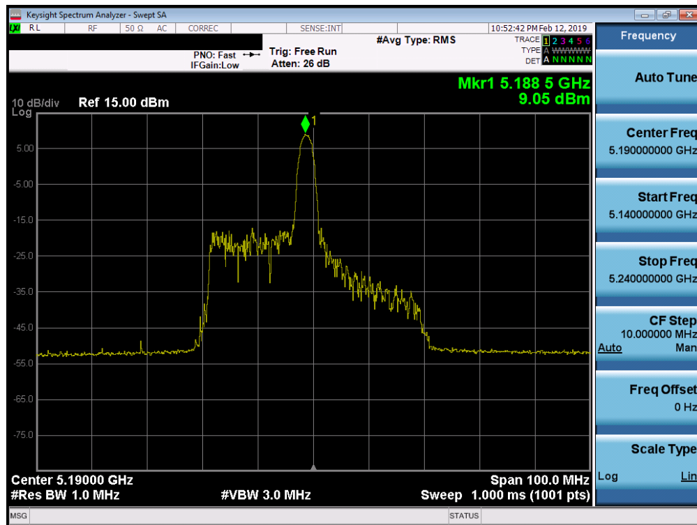
Plot 7-85. Power Spectral Density Plot SISO ANT2 (40MHz BW 802.11ax – 26 Tones (UNII Band 1) – Ch. 38)
