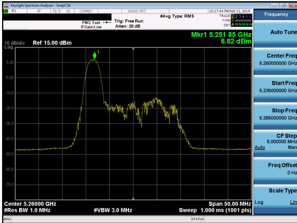
Plot 7-88. Power Spectral Density Plot SISO ANT2 (20MHz BW 802.11ax – 26 Tones (UNII Band 2A) – Ch. 52)
