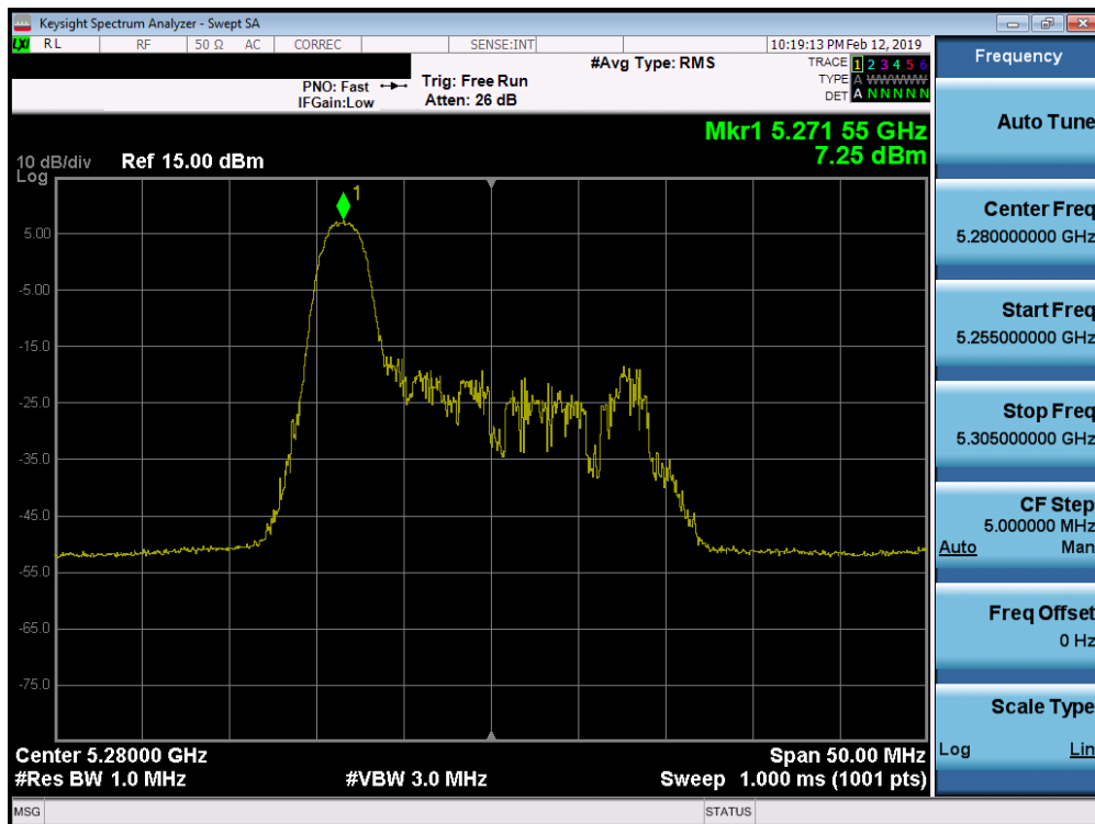
Plot 7-89. Power Spectral Density Plot SISO ANT2 (20MHz BW 802.11ax – 26 Tones (UNII Band 2A) – Ch. 56)
