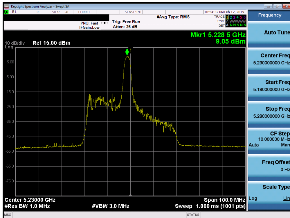
Plot 7-86. Power Spectral Density Plot SISO ANT2 (40MHz BW 802.11ax – 26 Tones (UNII Band 1) – Ch. 46)
