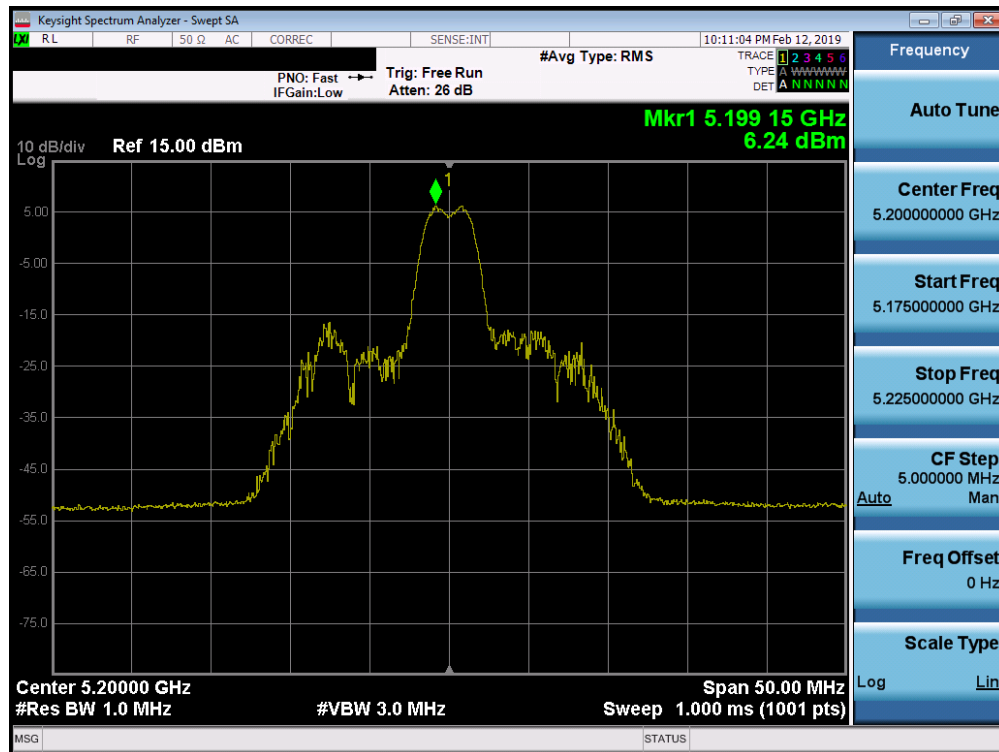
Plot 7-83. Power Spectral Density Plot SISO ANT2 (20MHz BW 802.11ax – 26 Tones (UNII Band 1) – Ch. 40)
