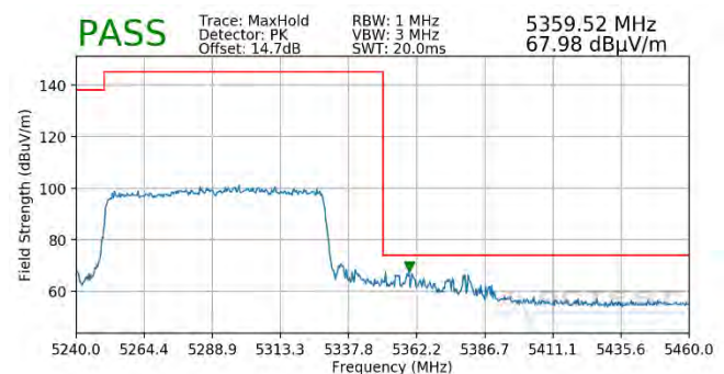
Plot 7-246. Radiated Upper Band Edge Plot MIMO (Peak – UNII Band 2A – 996 Tones)
