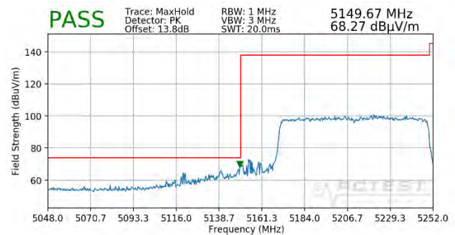
Plot 7-244. Radiated Lower Band Edge Plot MIMO (Peak – UNII Band 1 – 996 Tones)
