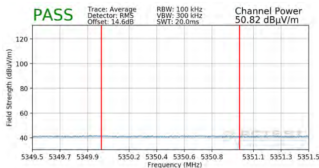
Plot 7-245. Radiated Upper Band Edge Plot MIMO (Average – UNII Band 2A – 996 Tones)
