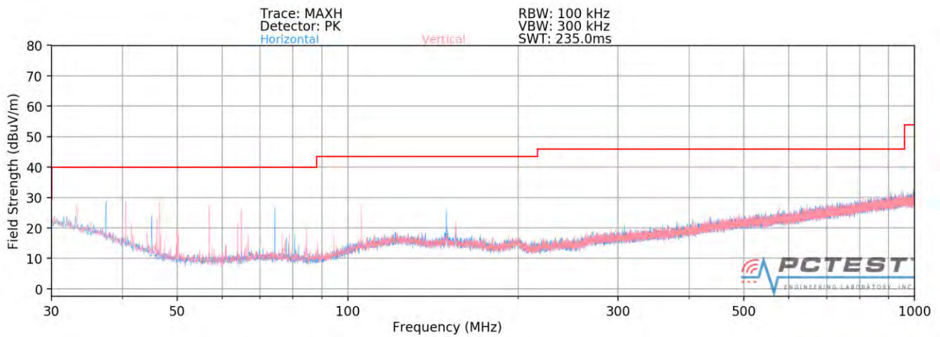
Plot 7-255. Radiated Spurious Plot below 1GHz MIMO (802.11ax – 242 Tones – U3 Ch. 157)
