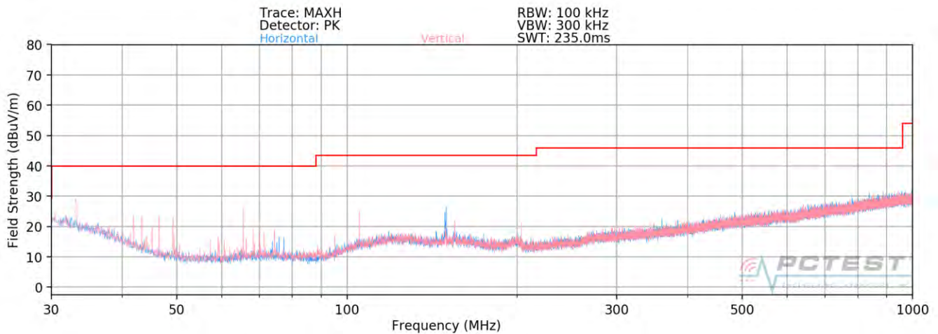
Plot 7-251. Radiated Spurious Plot below 1GHz SISO ANT1 (802.11ax – 242 Tones – U3 Ch. 157)
