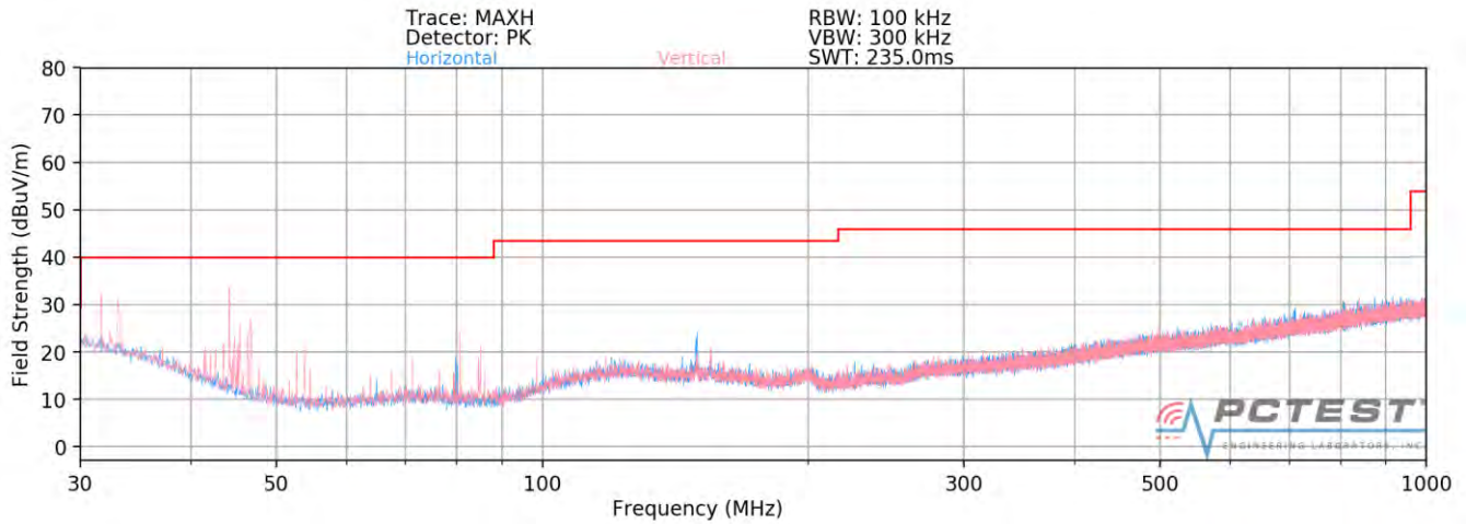
Plot 7-254. Radiated Spurious Plot below 1GHz MIMO (802.11ax – 26 Tones – U3 Ch. 157)
