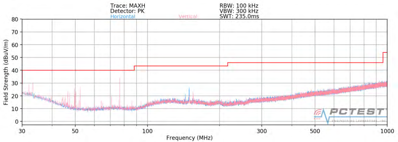
Plot 7-253. Radiated Spurious Plot below 1GHz SISO ANT2 (802.11ax – 242 Tones – U3 Ch. 157)
