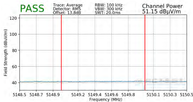
Plot 7-243. Radiated Lower Band Edge Plot MIMO (Average – UNII Band 1 – 996 Tones)
