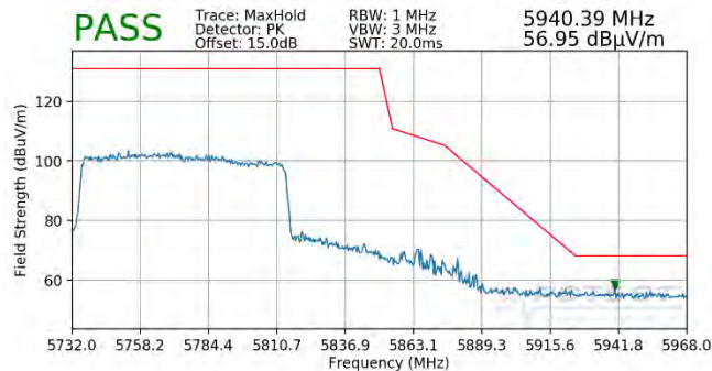
Plot 7-249. Radiated Upper Band Edge Plot MIMO (Peak – UNII Band 3 – 996 Tones)
