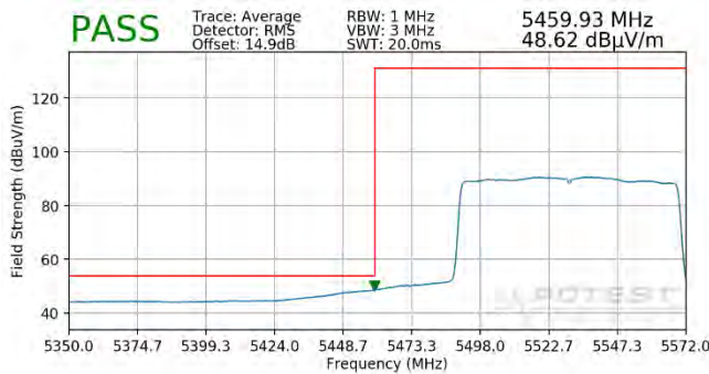
Plot 7-247. Radiated Lower Band Edge Plot MIMO (Average – UNII Band 2C – 996 Tones)
