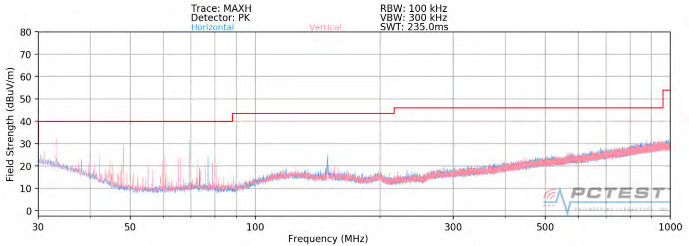
Plot 7-252. Radiated Spurious Plot below 1GHz SISO ANT2 (802.11ax – 26 Tones – U3 Ch. 157)
