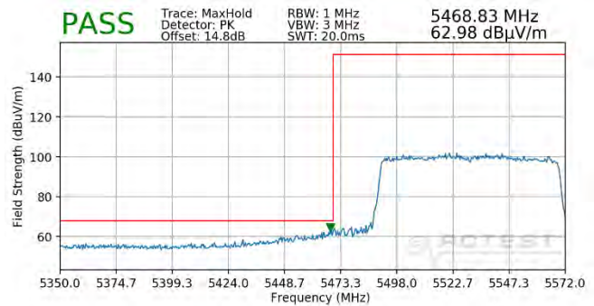
Plot 7-248. Radiated Lower Band Edge Plot MIMO (Peak – UNII Band 2C – 996 Tones)
