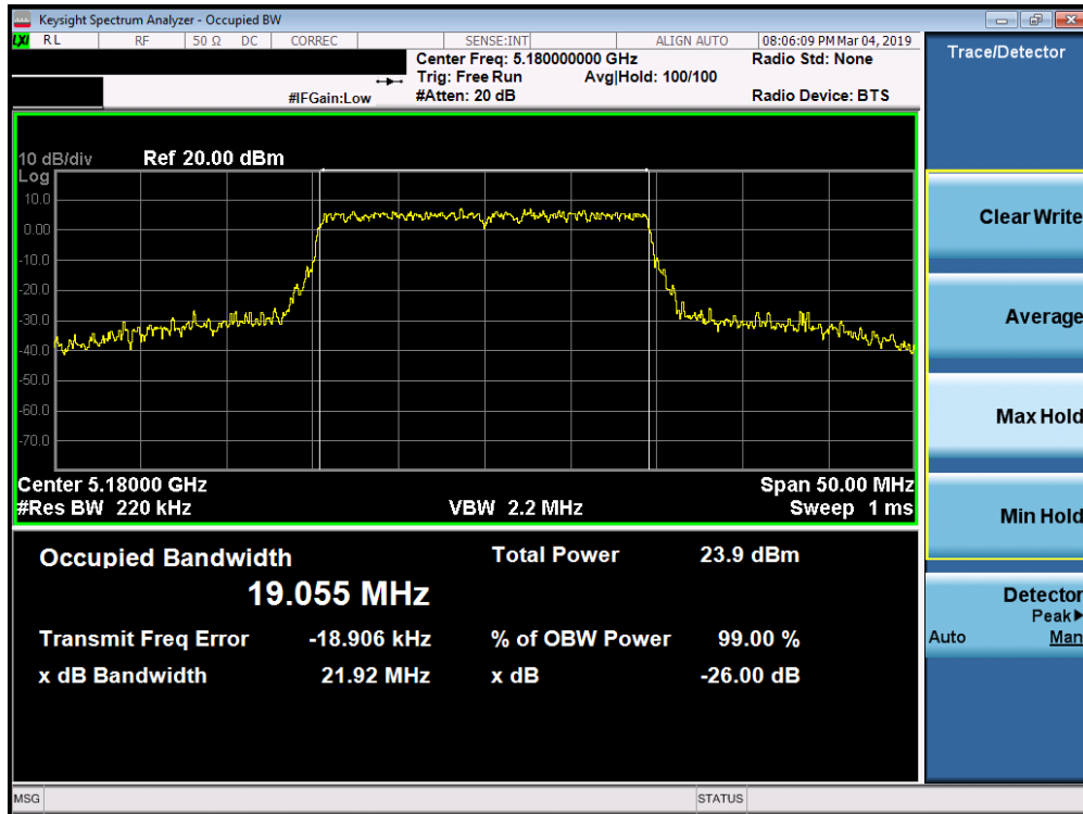
Plot 7-58. 26dB Bandwidth Plot SISO ANT2 (20MHz 802.11ax (UNII Band 1) – Ch. 36)
