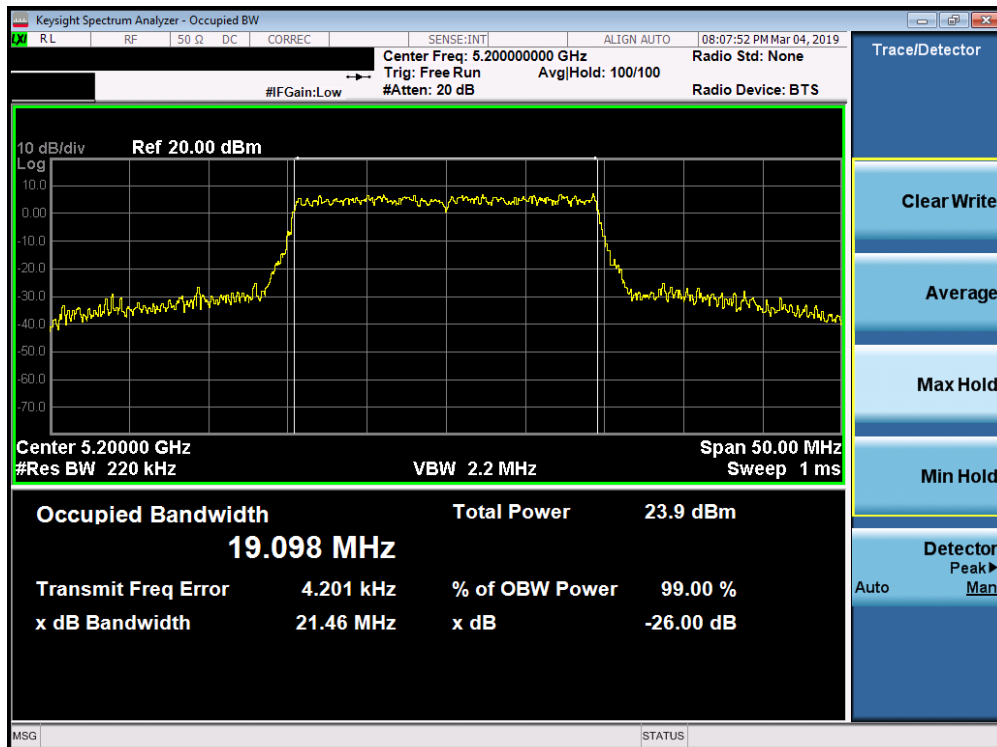
Plot 7-59. 26dB Bandwidth Plot SISO ANT2 (20MHz 802.11ax (UNII Band 1) – Ch. 40)
