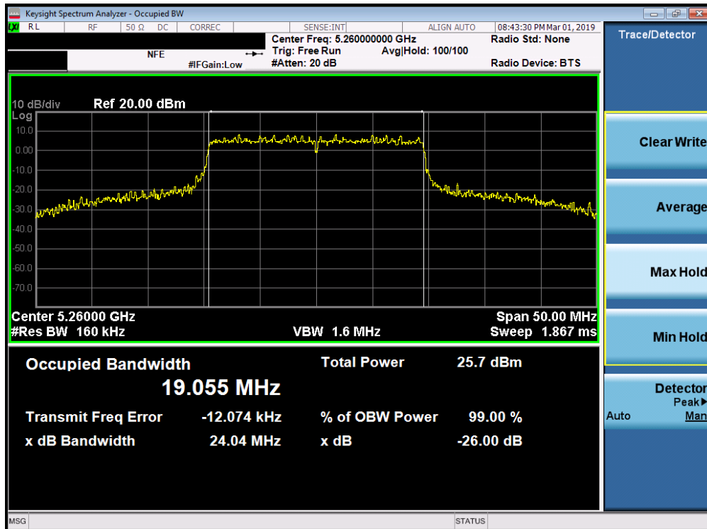
Plot 7-22. 26dB Bandwidth Plot SISO ANT1 (802.11ax (UNII Band 2A) – Ch. 52)
