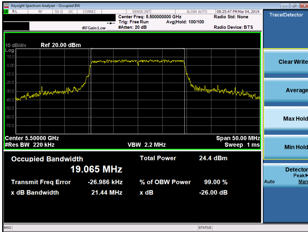
Plot 7-88. 26dB Bandwidth Plot SISO ANT2 (20MHz 802.11ax (UNII Band 2C) – Ch. 100)
