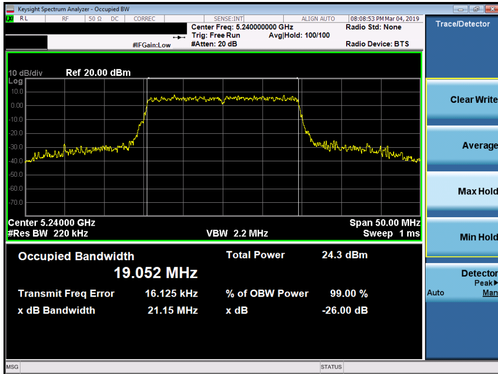
Plot 7-60. 26dB Bandwidth Plot SISO ANT2 (20MHz 802.11ax (UNII Band 1) – Ch. 48)
