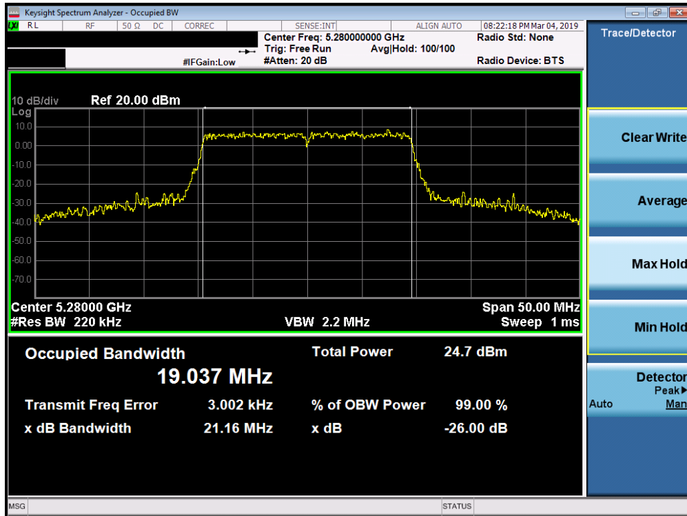
Plot 7-74. 26dB Bandwidth Plot SISO ANT2 (20MHz 802.11ax (UNII Band 2A) – Ch. 56)
