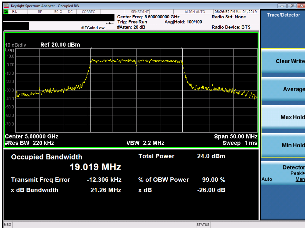
Plot 7-89. 26dB Bandwidth Plot SISO ANT2 (20MHz 802.11ax (UNII Band 2C) – Ch. 120)
