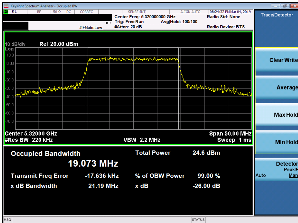
Plot 7-75. 26dB Bandwidth Plot SISO ANT2 (20MHz 802.11ax (UNII Band 2A) – Ch. 64)
