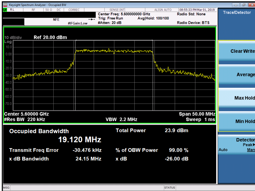
Plot 7-38. 26dB Bandwidth Plot SISO ANT1 (802.11ax (UNII Band 2C) – Ch. 120)
