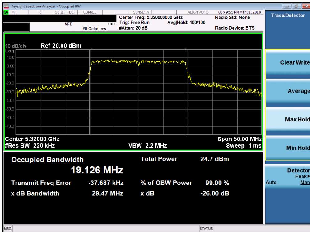
Plot 7-24. 26dB Bandwidth Plot SISO ANT1 (802.11ax (UNII Band 2A) – Ch. 64)
