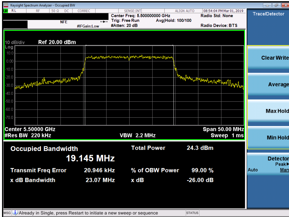
Plot 7-37. 26dB Bandwidth Plot SISO ANT1 (802.11ax (UNII Band 2C) – Ch. 100)
