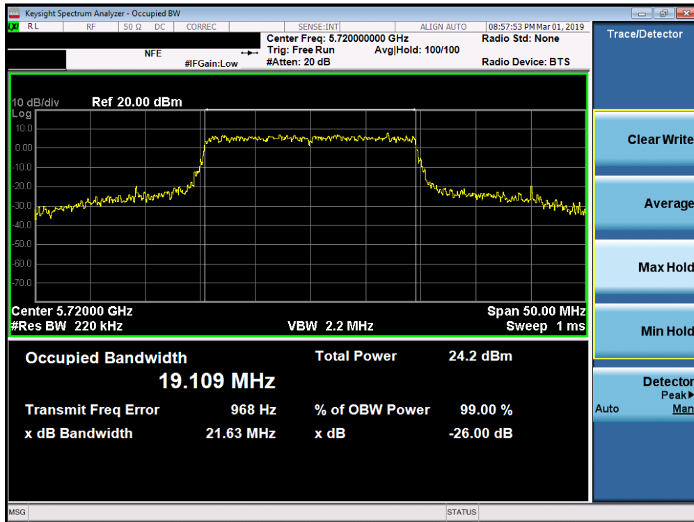
Plot 7-39. 26dB Bandwidth Plot SISO ANT1 (802.11ax (UNII Band 2C) – Ch. 144)
