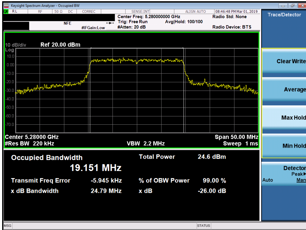
Plot 7-23. 26dB Bandwidth Plot SISO ANT1 (802.11ax (UNII Band 2A) – Ch. 56)
