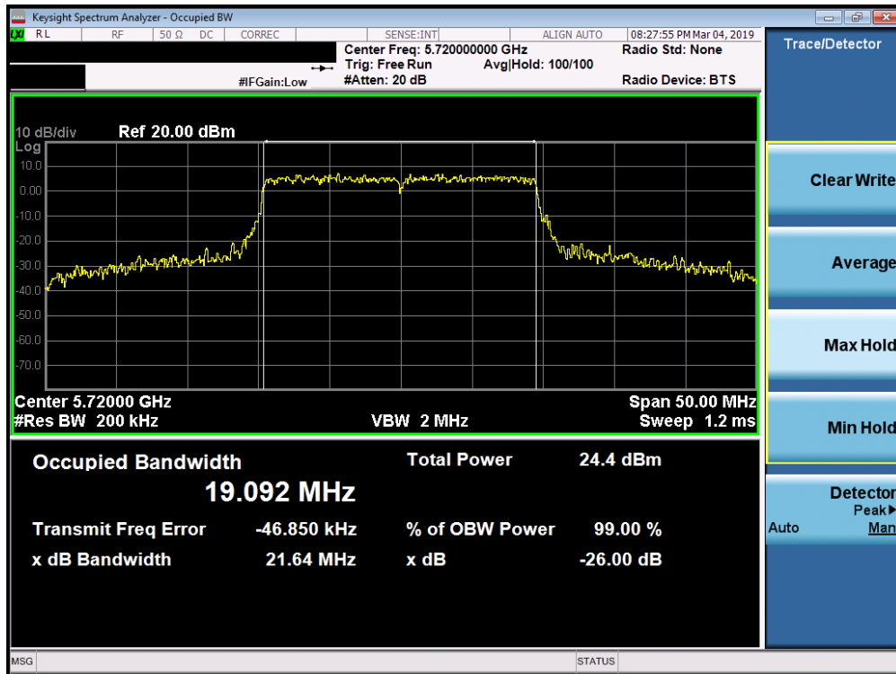
Plot 7-90. 26dB Bandwidth Plot SISO ANT2 (20MHz 802.11ax (UNII Band 2C) – Ch. 144)
