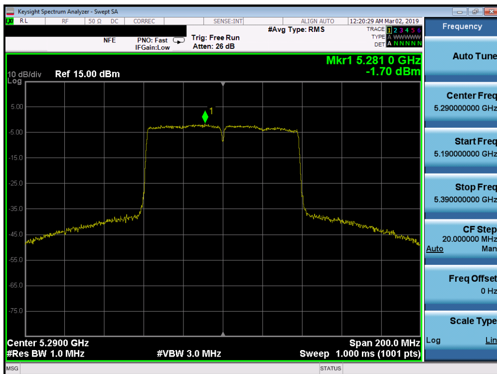
Plot 7-156. Power Spectral Density Plot SISO ANT1 (80MHz BW 802.11ac (UNII Band 2A) – Ch. 58)
