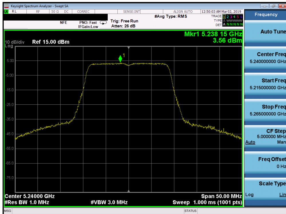
Plot 7-189. Power Spectral Density Plot SISO ANT2 (20MHz BW 802.11n (UNII Band 1) – Ch. 48)
