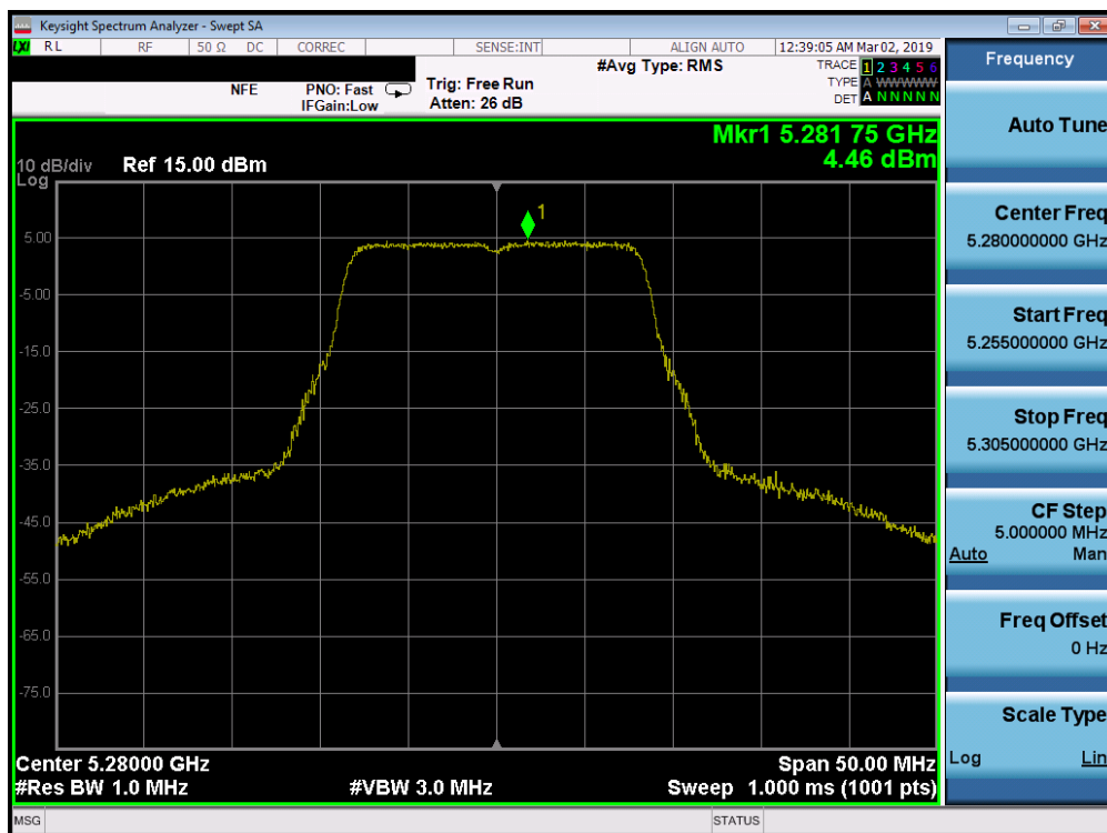
Plot 7-197. Power Spectral Density Plot SISO ANT2 (802.11a (UNII Band 2A) – Ch. 56)
