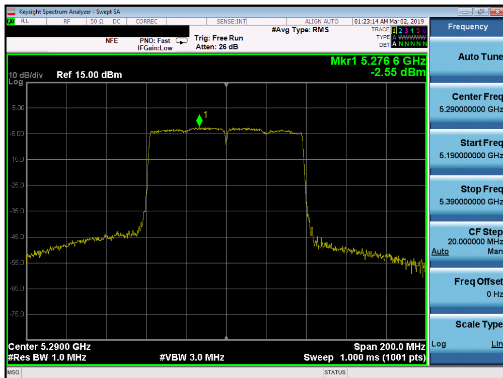
Plot 7-207. Power Spectral Density Plot SISO ANT2 (80MHz BW 802.11ac (UNII Band 2A) – Ch. 58)
