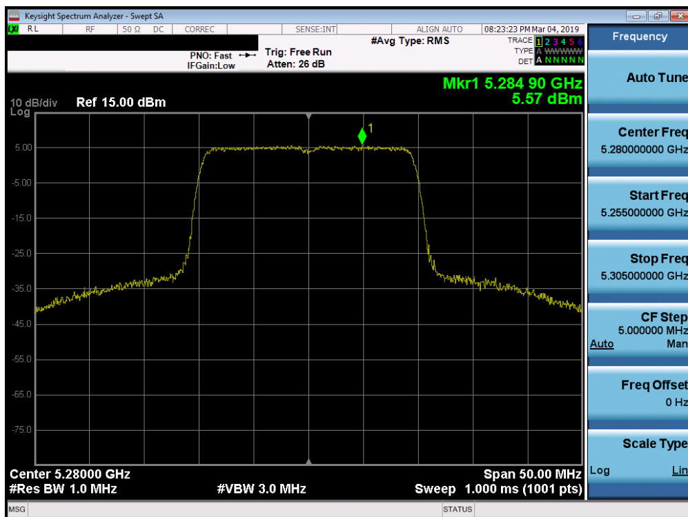
Plot 7-203. Power Spectral Density Plot SISO ANT2 (20MHz 802.11ax (UNII Band 2A) – Ch. 56)
