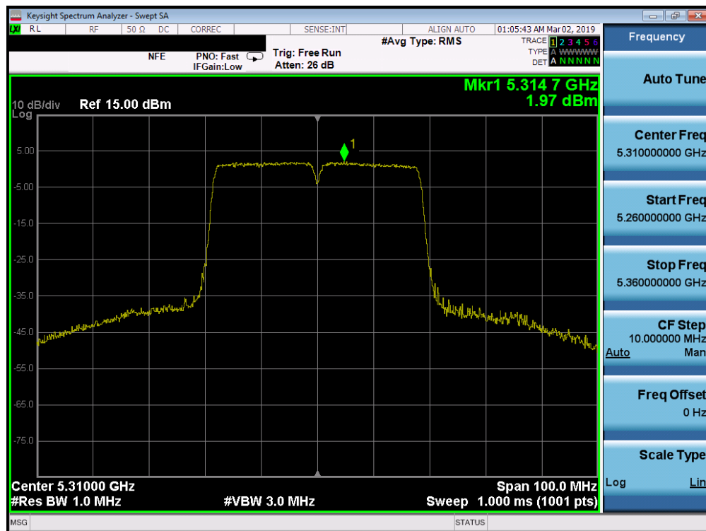
Plot 7-206. Power Spectral Density Plot SISO ANT2 (40MHz BW 802.11n (UNII Band 2A) – Ch. 62)
