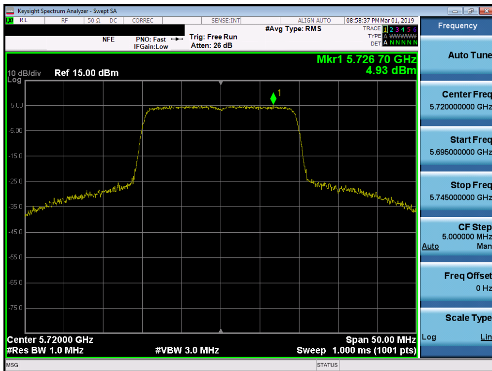
Plot 7-165. Power Spectral Density Plot SISO ANT1 (20MHz 802.11ax (UNII Band 2C) – Ch. 144)
