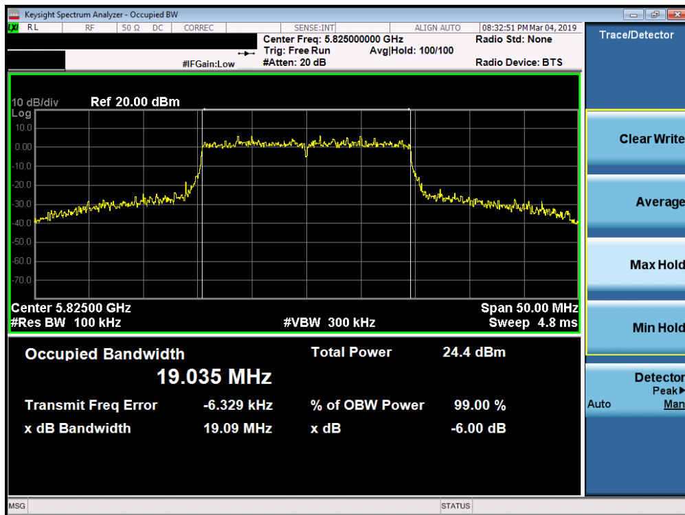
Plot 7-126. 6dB Bandwidth Plot SISO ANT2 (20MHz 802.11ax (UNII Band 3) – Ch. 165)
