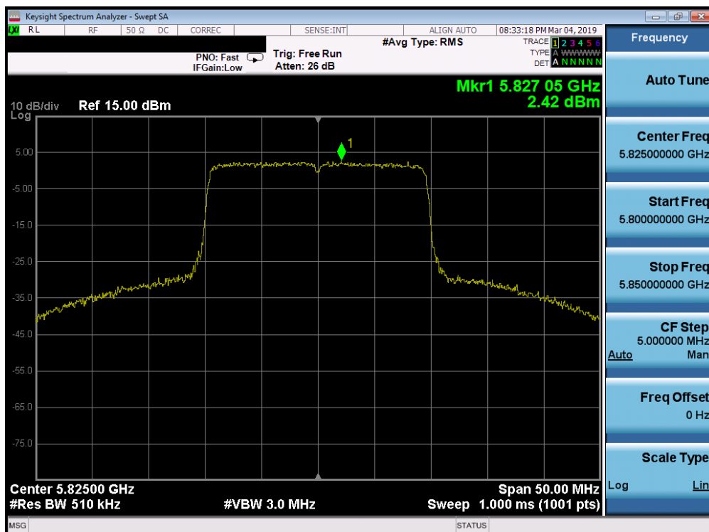
Plot 7-231. Power Spectral Density Plot SISO ANT2 (20MHz 802.11ax (UNII Band 3) – Ch. 165)
