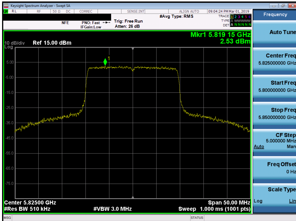
Plot 7-180. Power Spectral Density Plot SISO ANT1 (20MHz 802.11ax (UNII Band 3) – Ch. 165)
