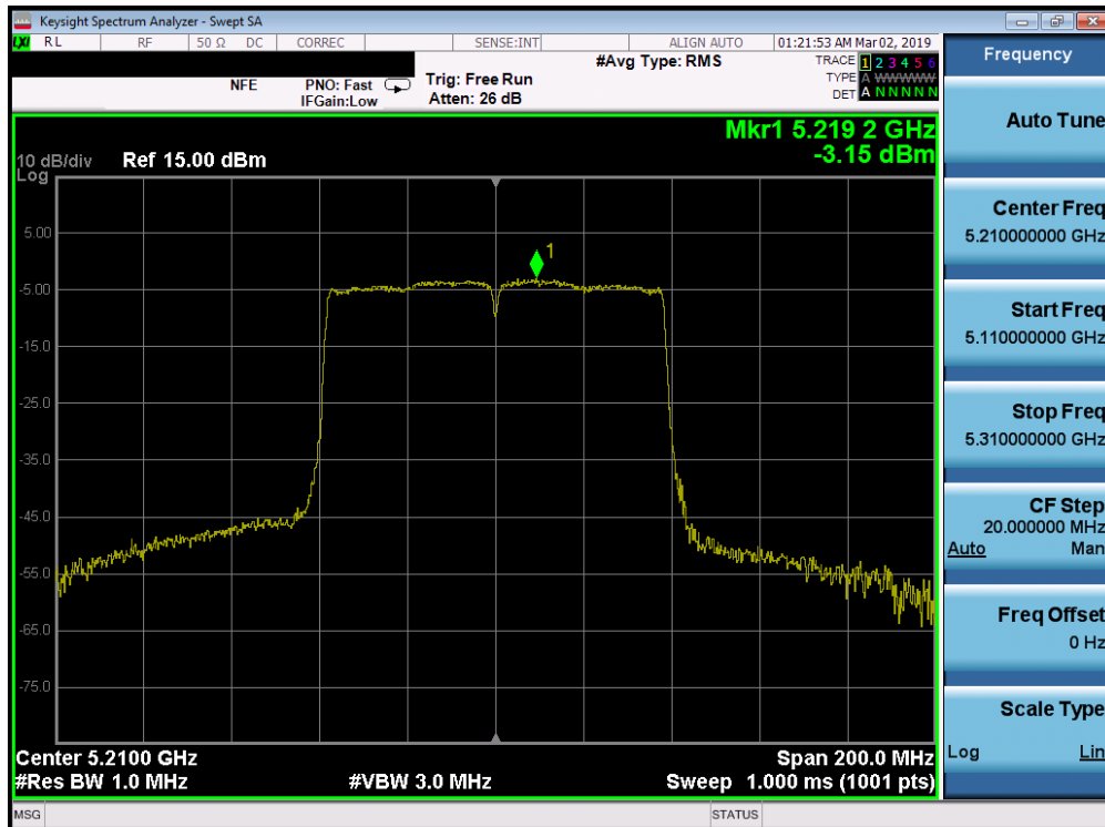
Plot 7-195. Power Spectral Density Plot SISO ANT2 (80MHz BW 802.11ac (UNII Band 1) – Ch. 42)
