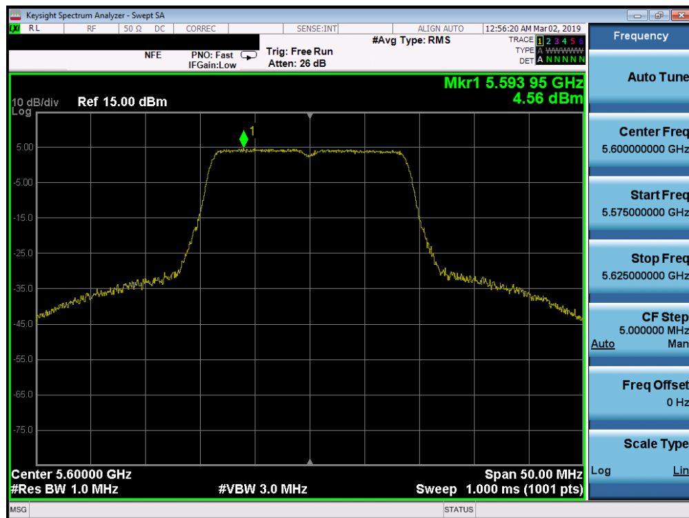
Plot 7-212. Power Spectral Density Plot SISO ANT2 (20MHz BW 802.11n (UNII Band 2C) – Ch. 120)
