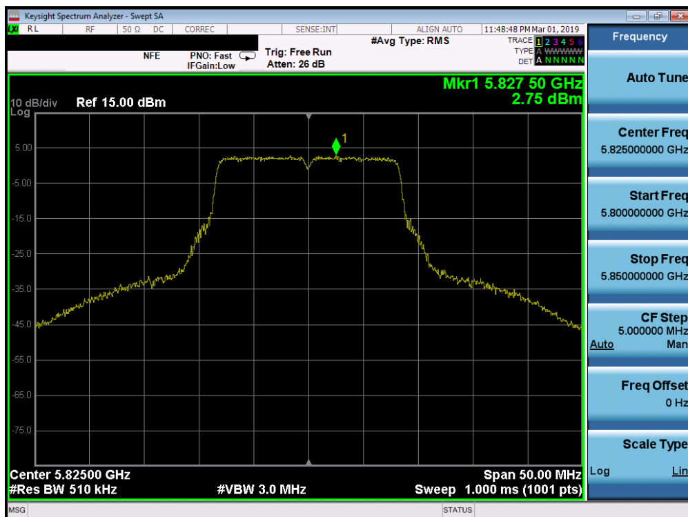
Plot 7-174. Power Spectral Density Plot SISO ANT1 (802.11a (UNII Band 3) – Ch. 165)
