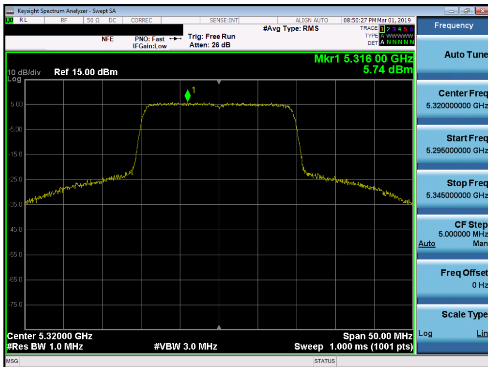
Plot 7-153. Power Spectral Density Plot SISO ANT1 (20MHz 802.11ax (UNII Band 2A) – Ch. 64)
