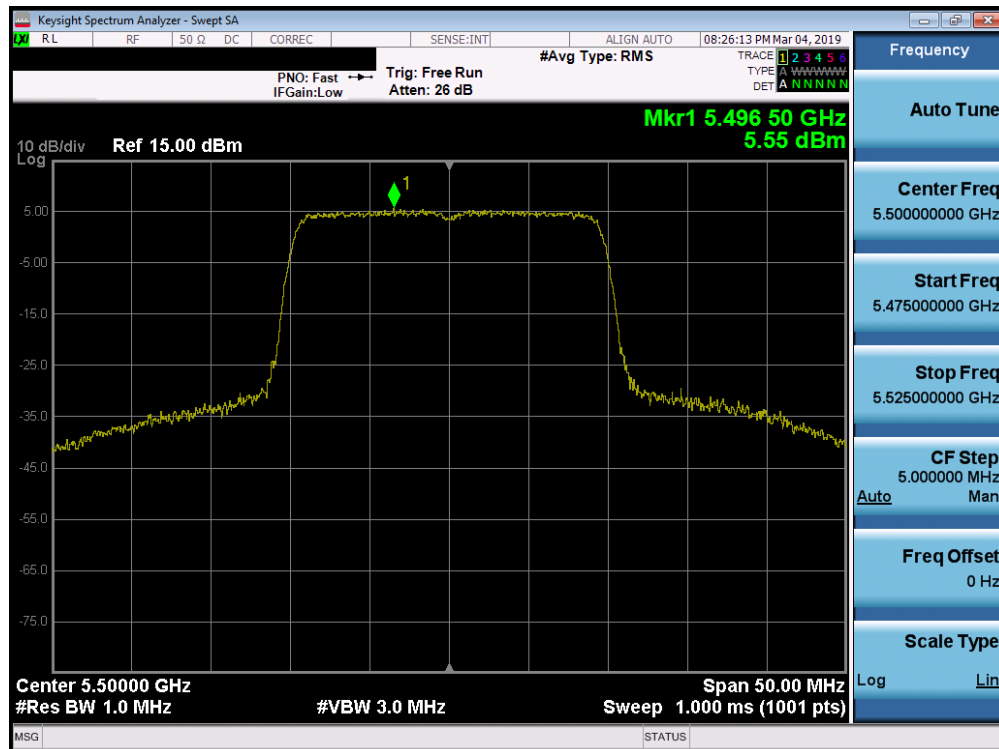
Plot 7-214. Power Spectral Density Plot SISO ANT2 (20MHz 802.11ax (UNII Band 2C) – Ch. 100)
