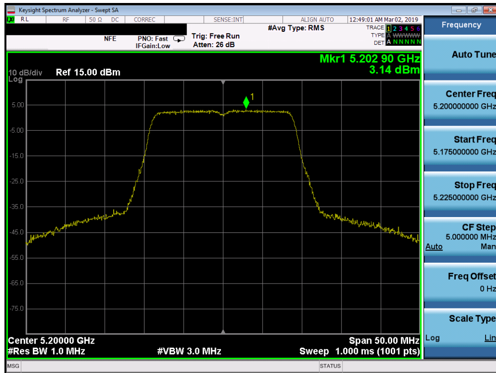
Plot 7-188. Power Spectral Density Plot SISO ANT2 (20MHz BW 802.11n (UNII Band 1) – Ch. 40)
