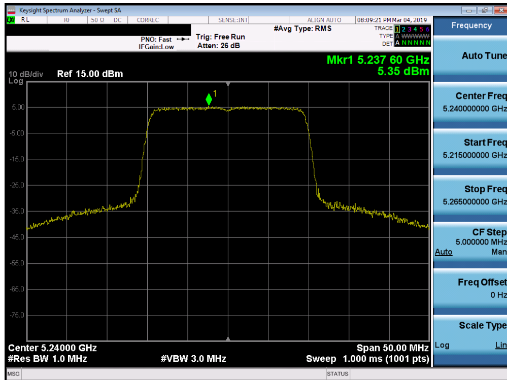
Plot 7-192. Power Spectral Density Plot SISO ANT2 (20MHz 802.11ax (UNII Band 1) – Ch. 48)
