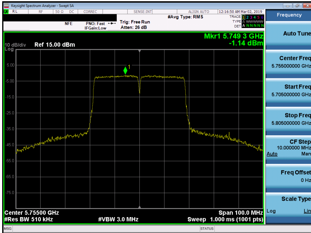
Plot 7-181. Power Spectral Density Plot SISO ANT1 (40MHz BW 802.11n (UNII Band 3) – Ch. 151)
