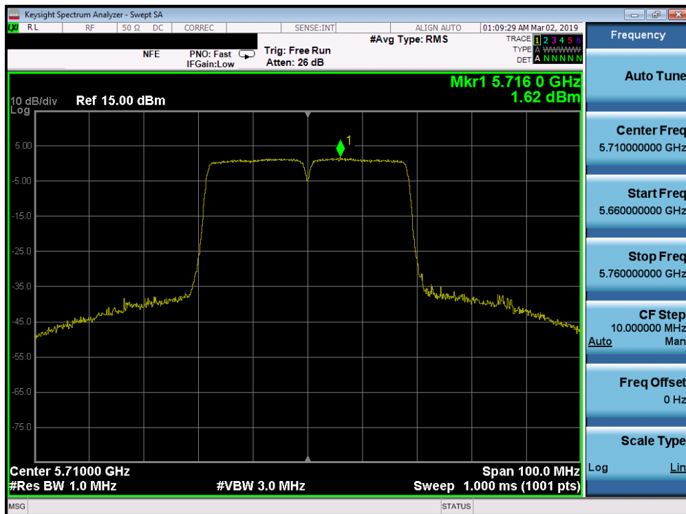
Plot 7-219. Power Spectral Density Plot SISO ANT2 (40MHz BW 802.11n (UNII Band 2C) – Ch. 142)
