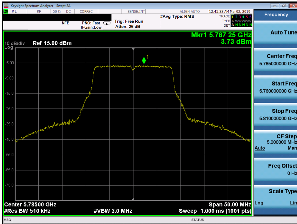
Plot 7-224. Power Spectral Density Plot SISO ANT2 (802.11a (UNII Band 3) – Ch. 157)
