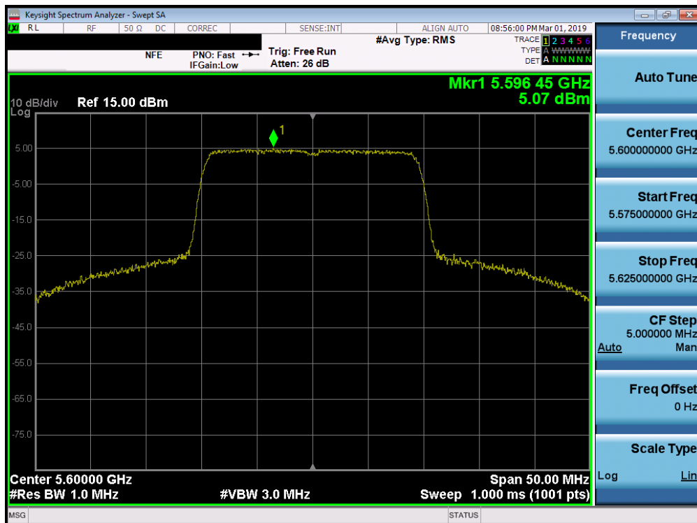
Plot 7-164. Power Spectral Density Plot SISO ANT1 (20MHz 802.11ax (UNII Band 2C) – Ch. 120)
