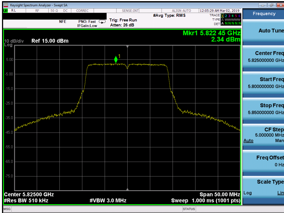
Plot 7-177. Power Spectral Density Plot SISO ANT1 (20MHz BW 802.11n (UNII Band 3) – Ch. 165)
