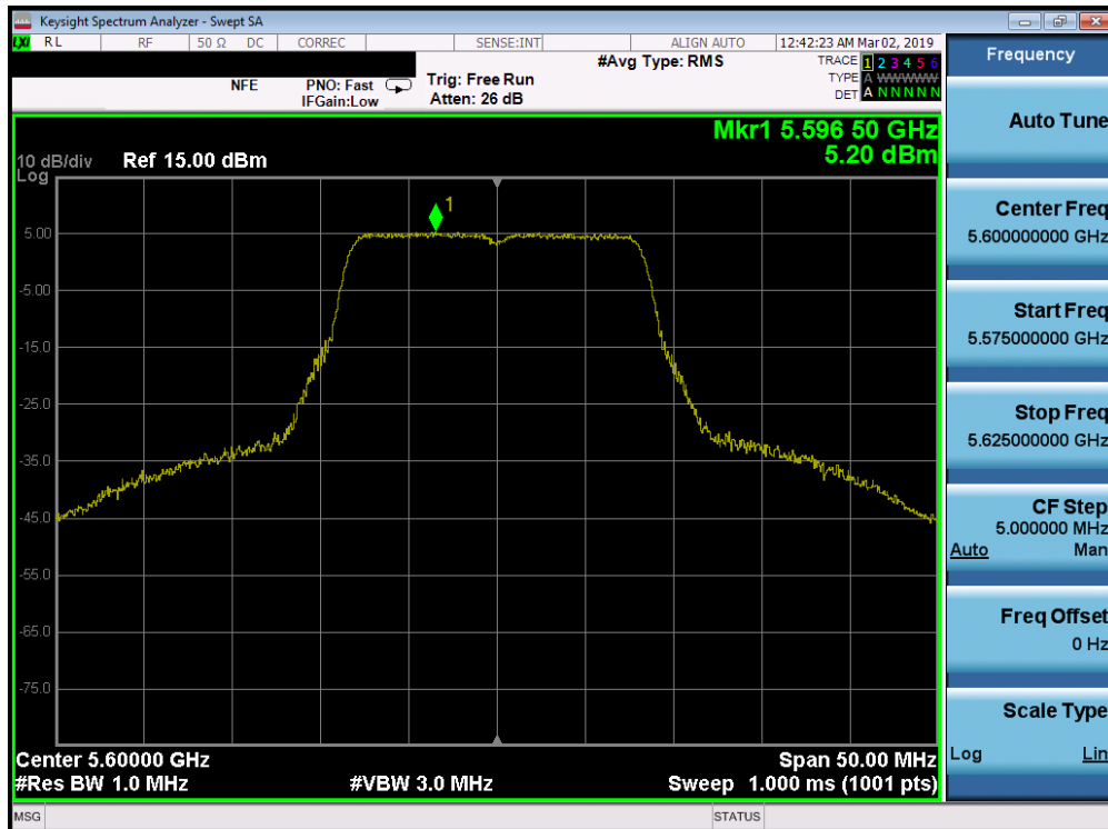
Plot 7-209. Power Spectral Density Plot SISO ANT2 (802.11a (UNII Band 2C) – Ch. 120)
