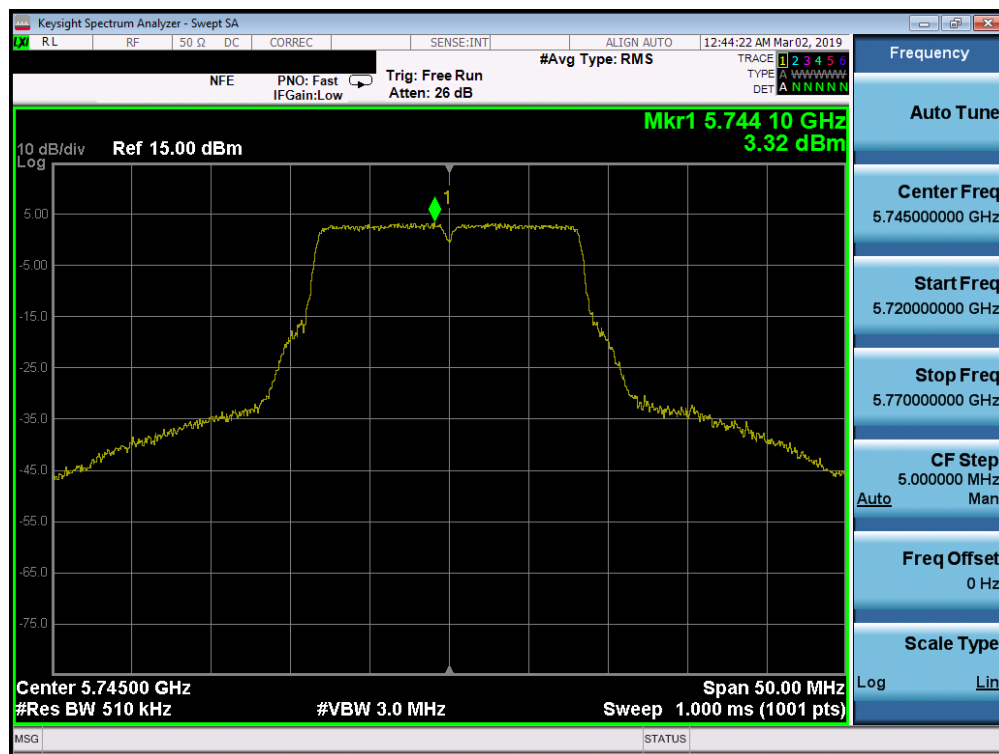
Plot 7-223. Power Spectral Density Plot SISO ANT2 (802.11a (UNII Band 3) – Ch. 149)
