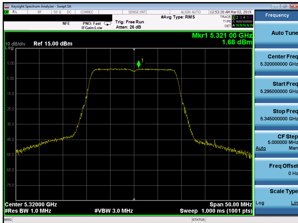
Plot 7-201. Power Spectral Density Plot SISO ANT2 (20MHz BW 802.11n (UNII Band 2A) – Ch. 64)
