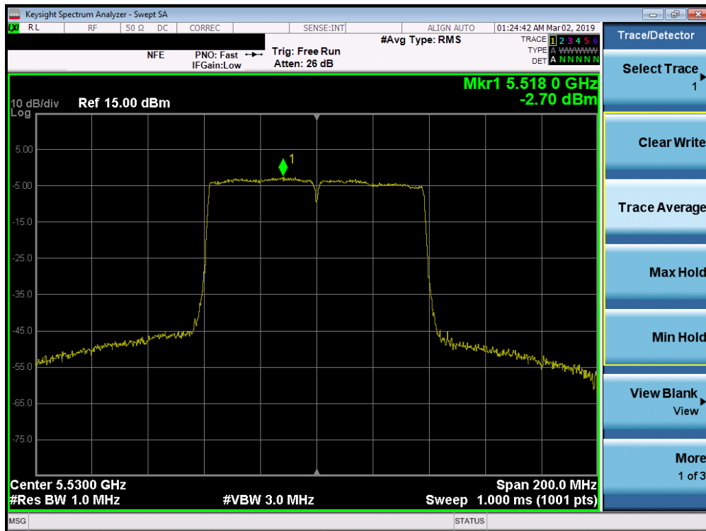
Plot 7-220. Power Spectral Density Plot SISO ANT2 (80MHz BW 802.11ac (UNII Band 2C) – Ch. 106)
