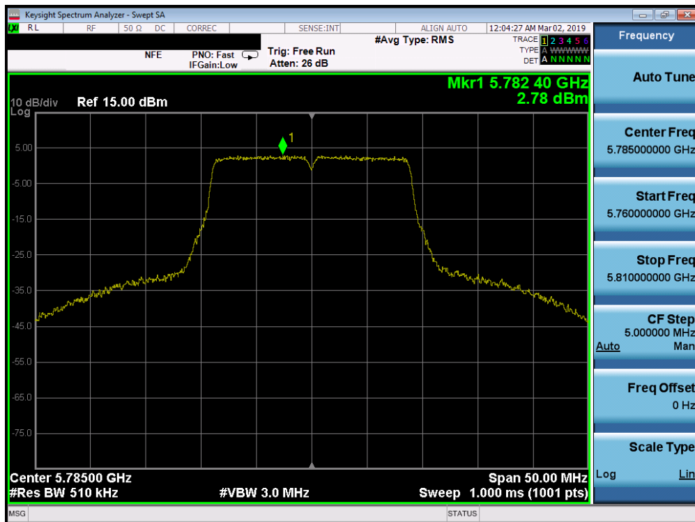
Plot 7-176. Power Spectral Density Plot SISO ANT1 (20MHz BW 802.11n (UNII Band 3) – Ch. 157)
