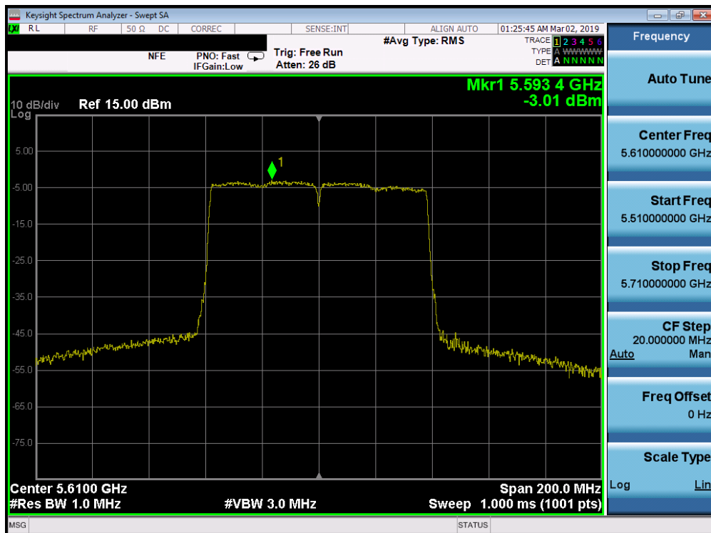
Plot 7-221. Power Spectral Density Plot SISO ANT2 (80MHz BW 802.11ac (UNII Band 2C) – Ch. 122)
