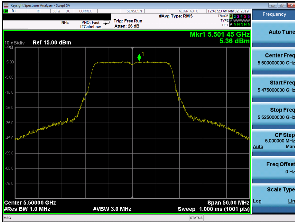
Plot 7-208. Power Spectral Density Plot SISO ANT2 (802.11a (UNII Band 2C) – Ch. 100)
