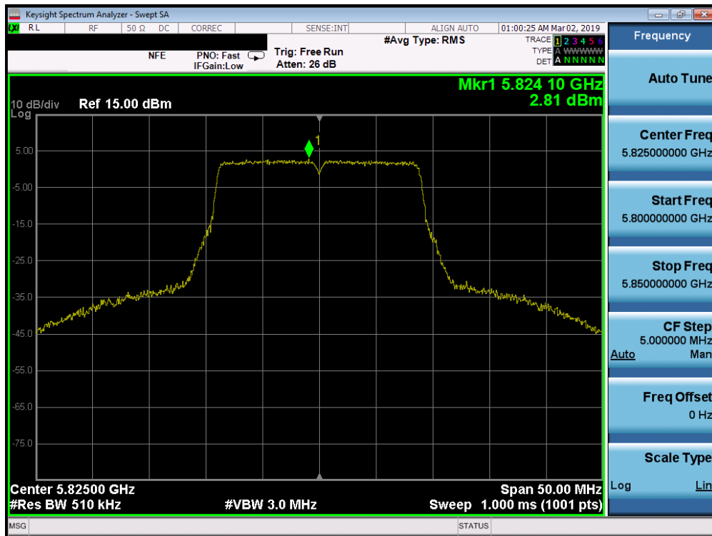
Plot 7-228. Power Spectral Density Plot SISO ANT2 (20MHz BW 802.11n (UNII Band 3) – Ch. 165)
