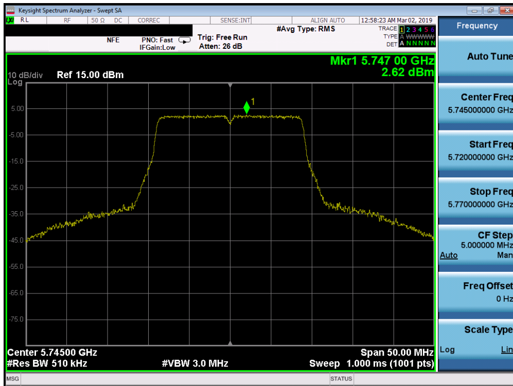
Plot 7-226. Power Spectral Density Plot SISO ANT2 (20MHz BW 802.11n (UNII Band 3) – Ch. 149)
