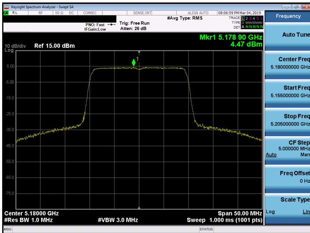
Plot 7-190. Power Spectral Density Plot SISO ANT2 (20MHz 802.11ax (UNII Band 1) – Ch. 36)
