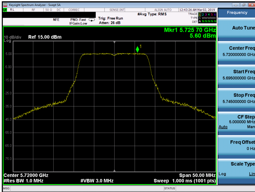
Plot 7-210. Power Spectral Density Plot SISO ANT2 (802.11a (UNII Band 2C) – Ch. 144)
