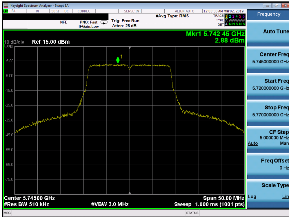
Plot 7-175. Power Spectral Density Plot SISO ANT1 (20MHz BW 802.11n (UNII Band 3) – Ch. 149)
