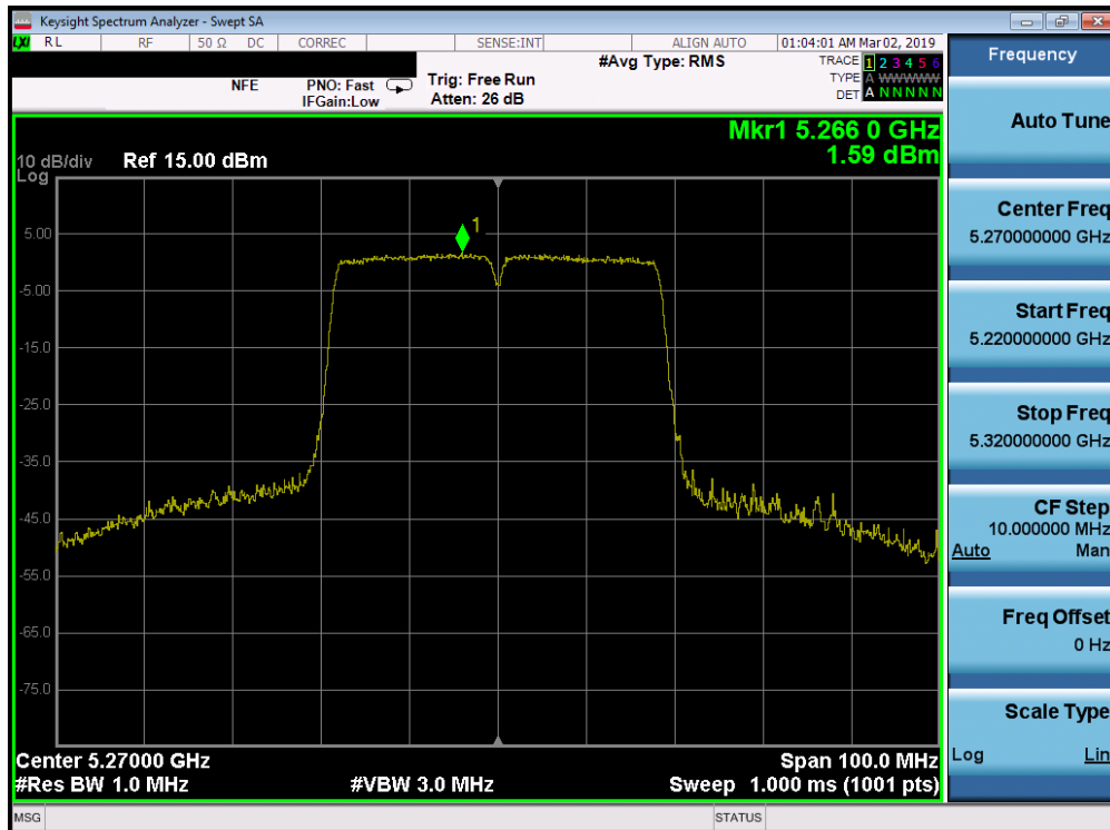
Plot 7-205. Power Spectral Density Plot SISO ANT2 (40MHz BW 802.11n (UNII Band 2A) – Ch. 54)
