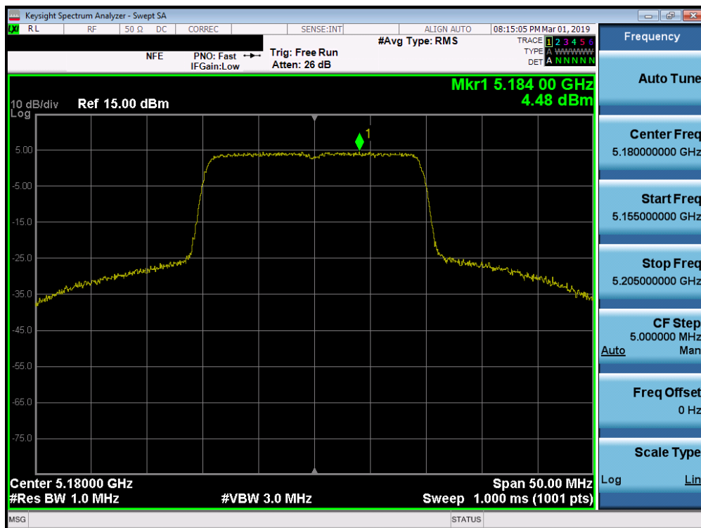
Plot 7-139. Power Spectral Density Plot SISO ANT1 (20MHz 802.11ax (UNII Band 1) – Ch. 36)
