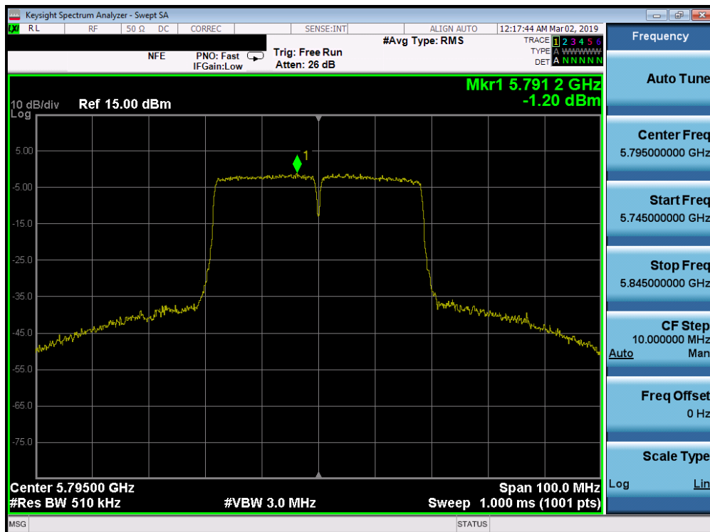
Plot 7-182. Power Spectral Density Plot SISO ANT1 (40MHz BW 802.11n (UNII Band 3) – Ch. 159)
