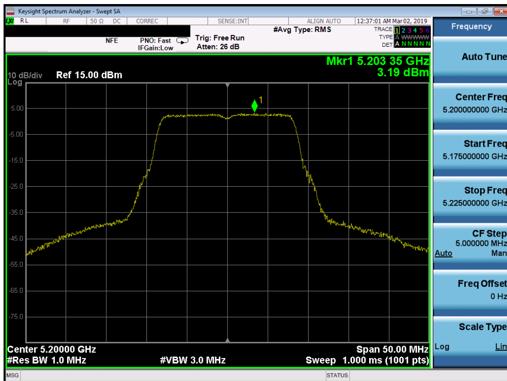
Plot 7-185. Power Spectral Density Plot SISO ANT2 (802.11a (UNII Band 1) – Ch. 40)
