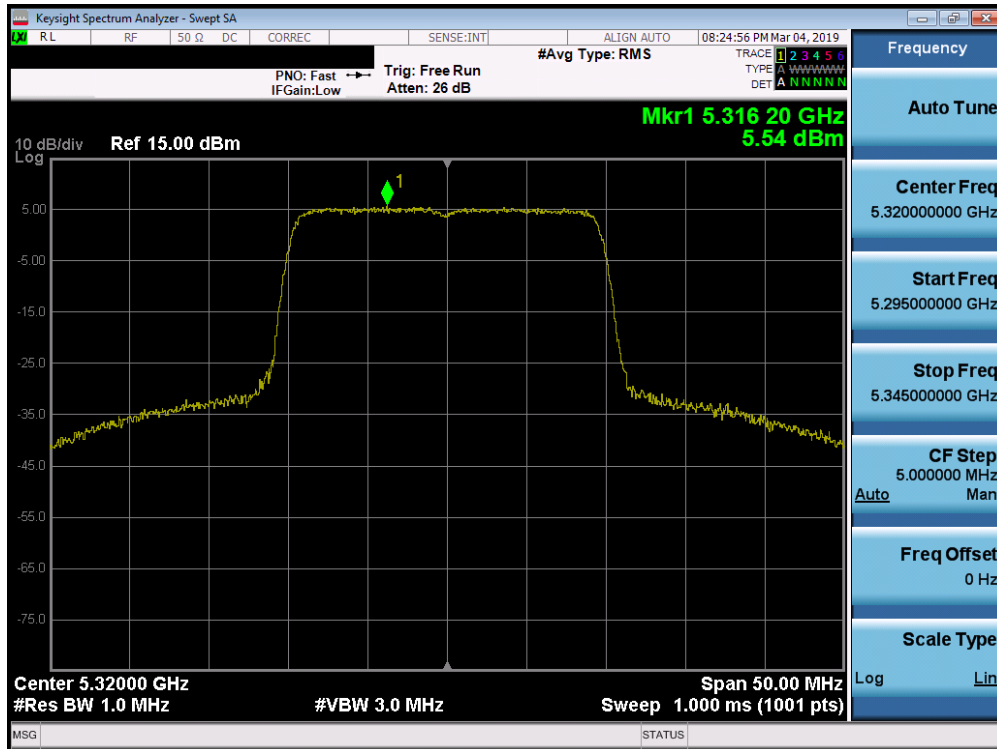
Plot 7-204. Power Spectral Density Plot SISO ANT2 (20MHz 802.11ax (UNII Band 2A) – Ch. 64)
