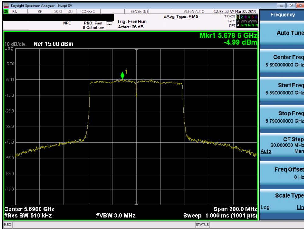
Plot 7-171. Power Spectral Density Plot SISO ANT1 (80MHz BW 802.11ac (UNII Band 2C) – Ch. 138)
