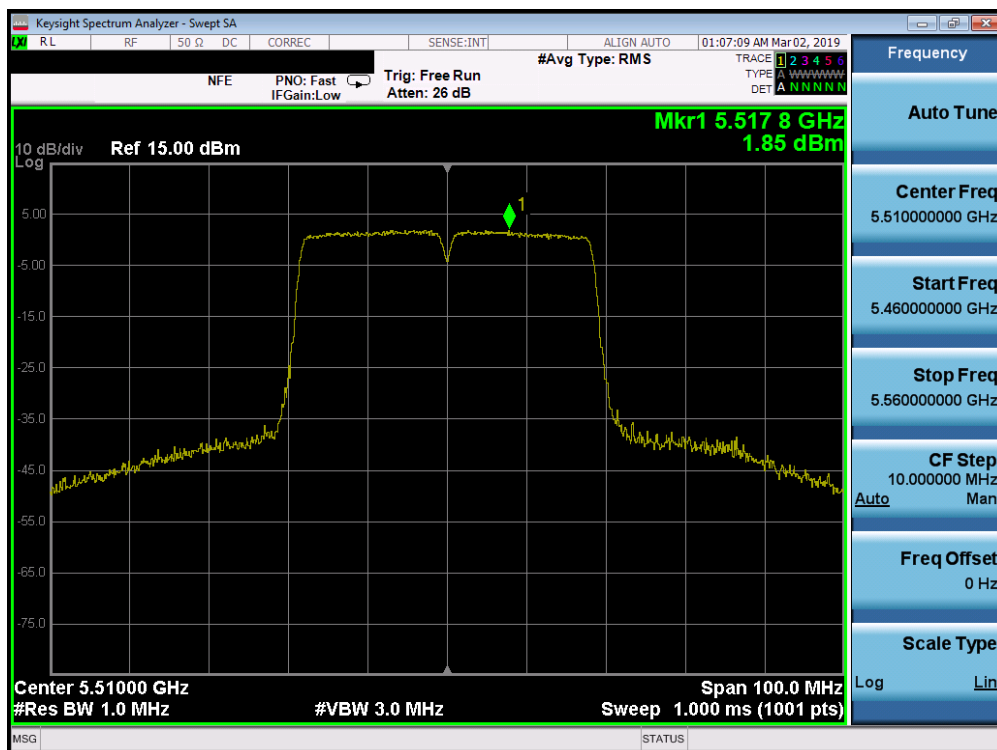
Plot 7-217. Power Spectral Density Plot SISO ANT2 (40MHz BW 802.11n (UNII Band 2C) – Ch. 102)
