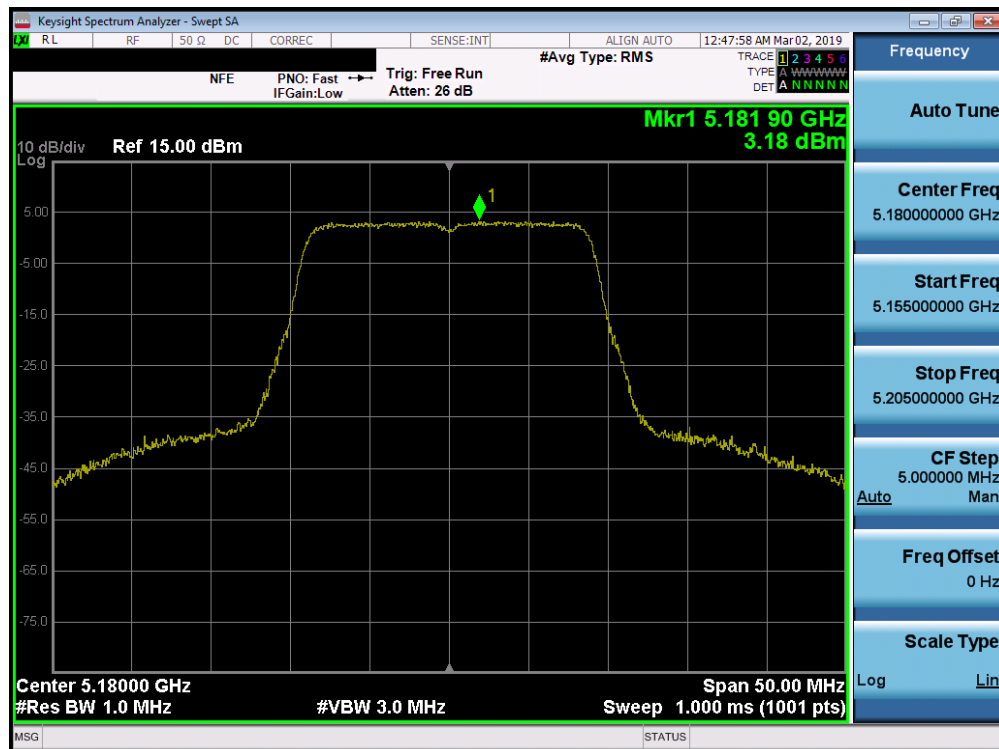
Plot 7-187. Power Spectral Density Plot SISO ANT2 (20MHz BW 802.11n (UNII Band 1) – Ch. 36)
