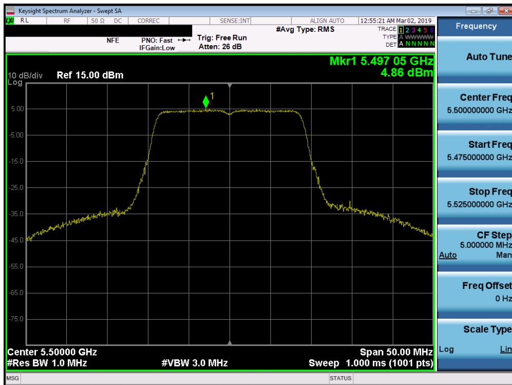
Plot 7-211. Power Spectral Density Plot SISO ANT2 (20MHz BW 802.11n (UNII Band 2C) – Ch. 100)
