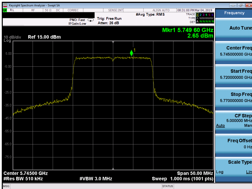
Plot 7-229. Power Spectral Density Plot SISO ANT2 (20MHz BW 802.11ax (UNII Band 3) – Ch. 149)
