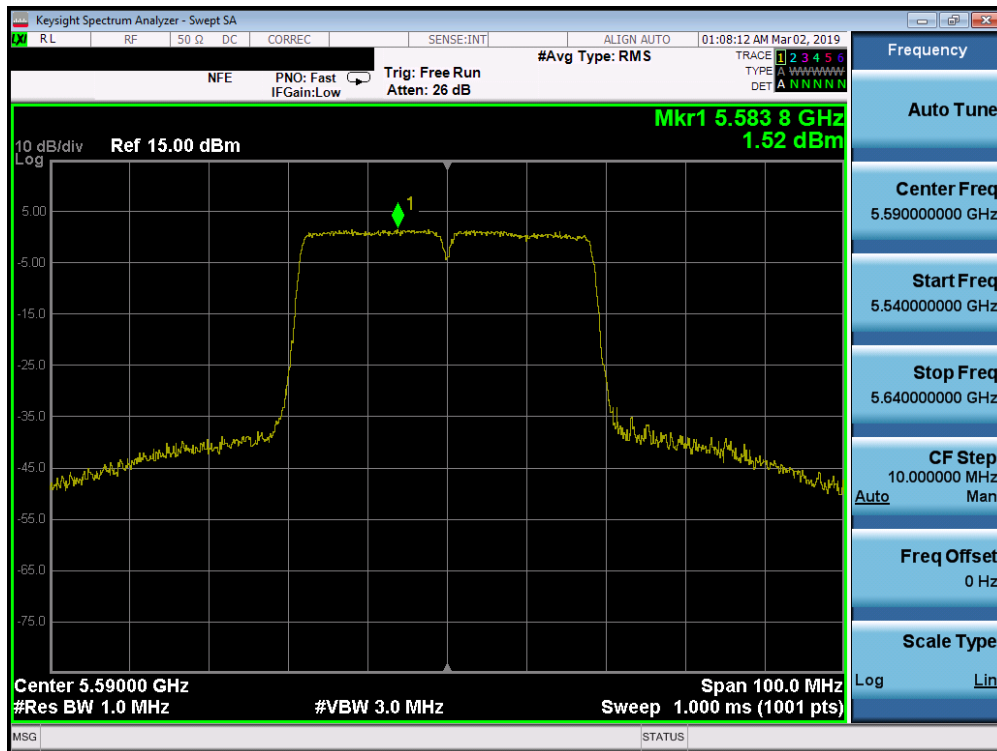
Plot 7-218. Power Spectral Density Plot SISO ANT2 (40MHz BW 802.11n (UNII Band 2C) – Ch. 118)
