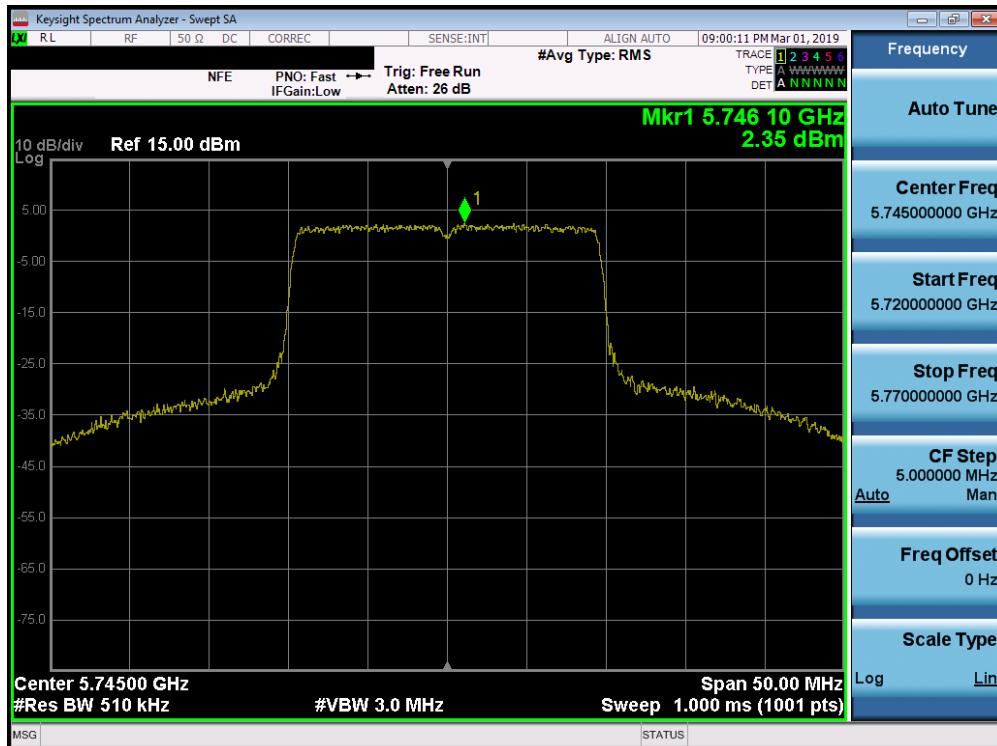
Plot 7-178. Power Spectral Density Plot SISO ANT1 (20MHz BW 802.11ax (UNII Band 3) – Ch. 149)
