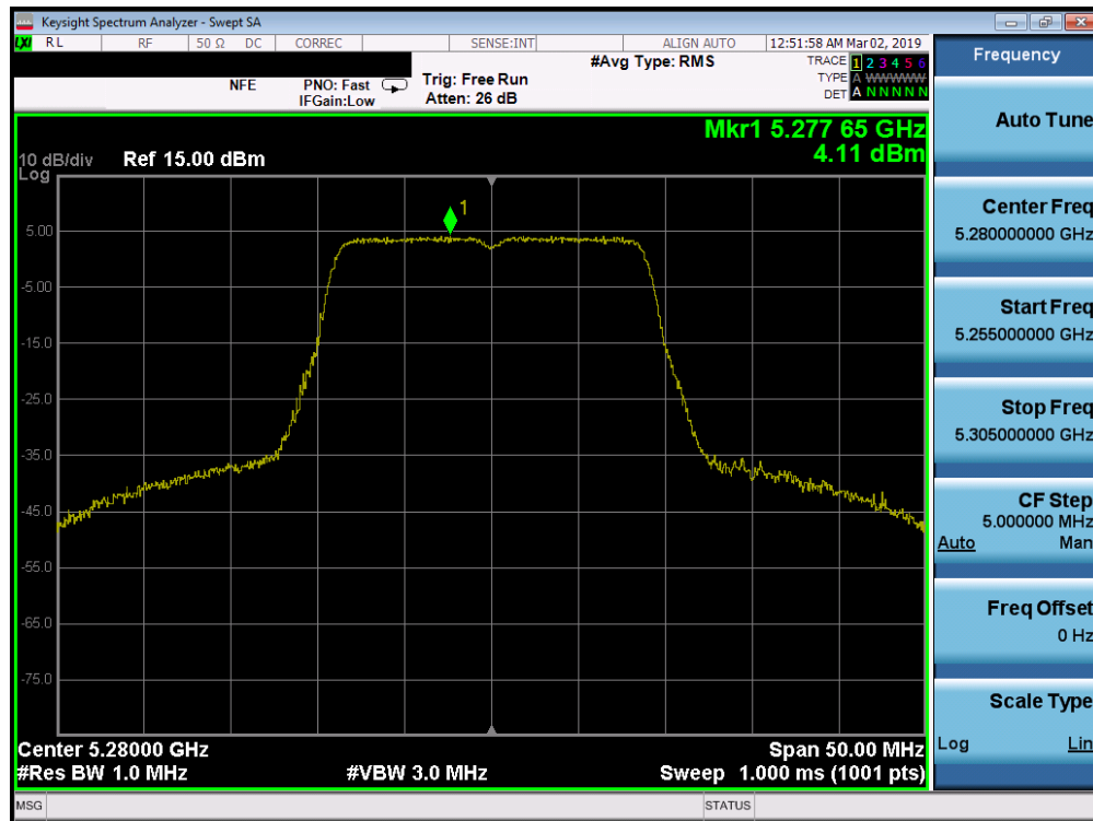
Plot 7-200. Power Spectral Density Plot SISO ANT2 (20MHz BW 802.11n (UNII Band 2A) – Ch. 56)
