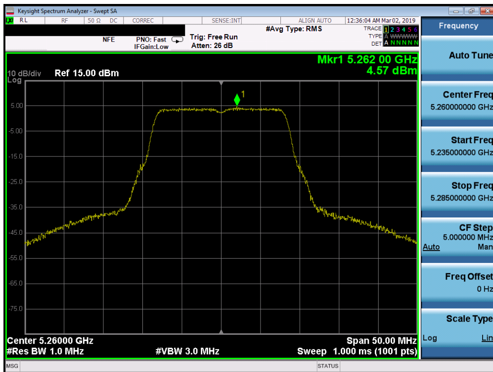
Plot 7-196. Power Spectral Density Plot SISO ANT2 (802.11a (UNII Band 2A) – Ch. 52)
