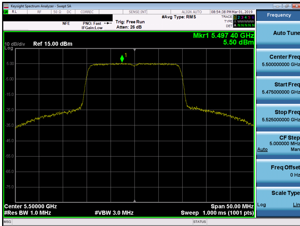
Plot 7-163. Power Spectral Density Plot SISO ANT1 (20MHz 802.11ax (UNII Band 2C) – Ch. 100)
