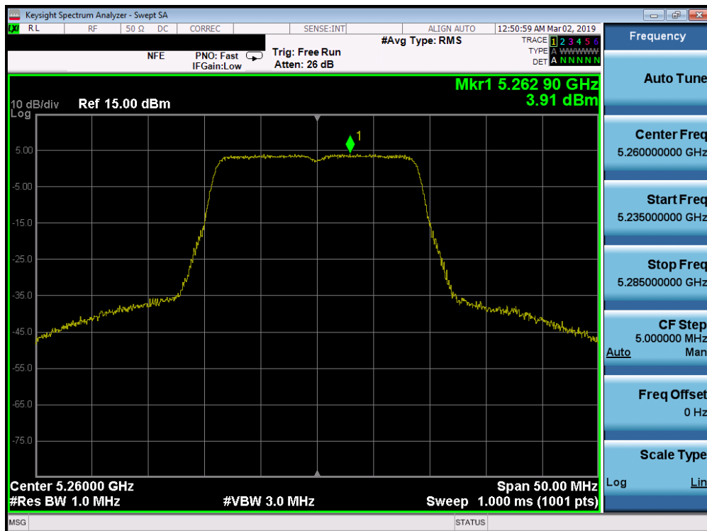
Plot 7-199. Power Spectral Density Plot SISO ANT2 (20MHz BW 802.11n (UNII Band 2A) – Ch. 52)
