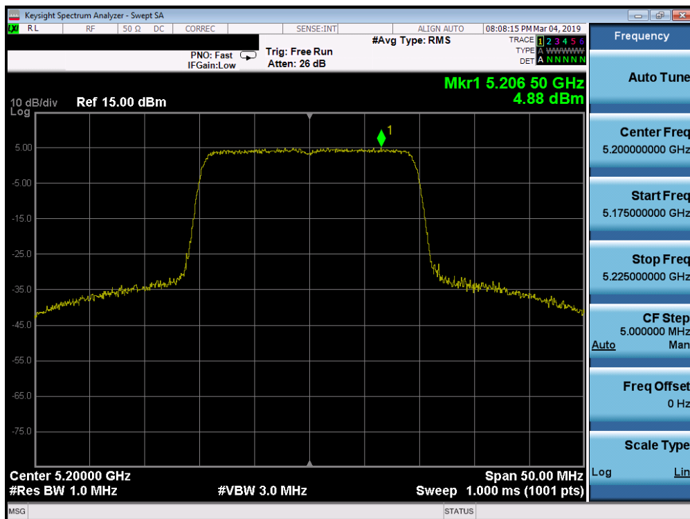
Plot 7-191. Power Spectral Density Plot SISO ANT2 (20MHz 802.11ax (UNII Band 1) – Ch. 40)
