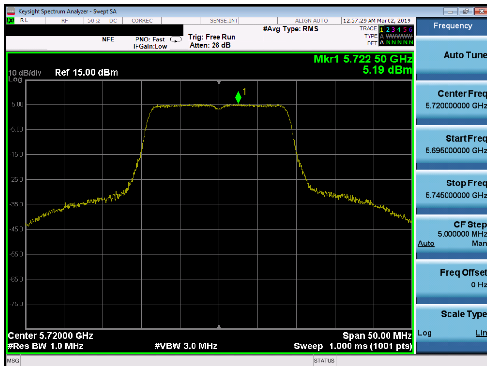
Plot 7-213. Power Spectral Density Plot SISO ANT2 (20MHz BW 802.11n (UNII Band 2C) – Ch. 144)
