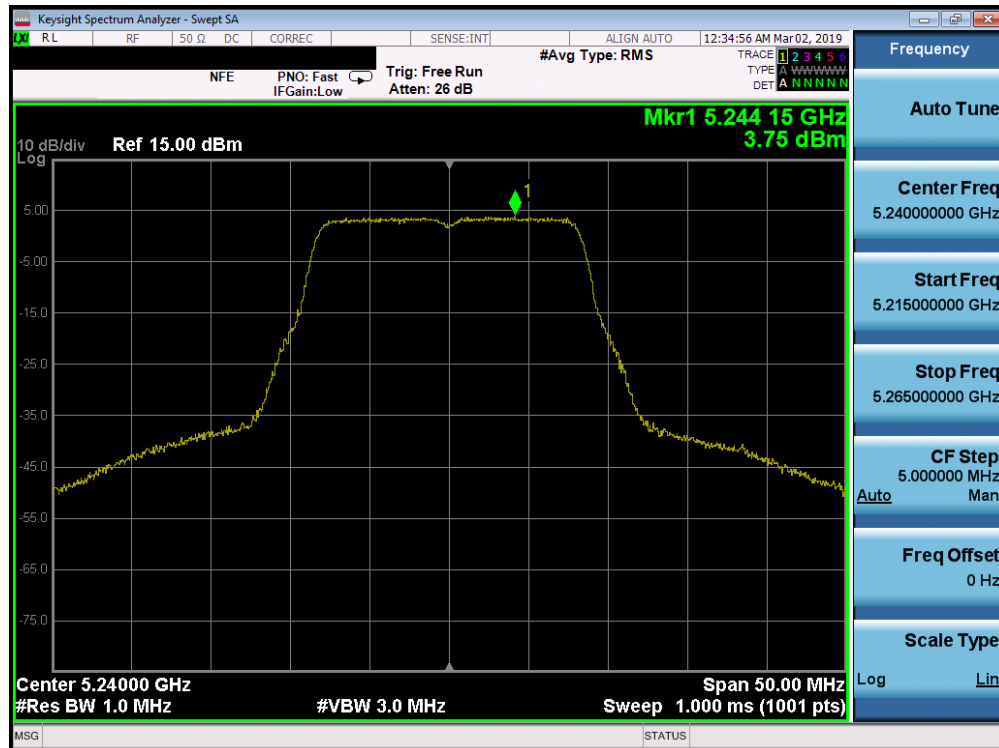
Plot 7-186. Power Spectral Density Plot SISO ANT2 (802.11a (UNII Band 1) – Ch. 48)
