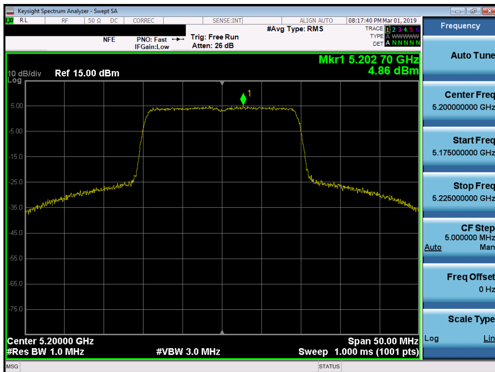
Plot 7-140. Power Spectral Density Plot SISO ANT1 (20MHz 802.11ax (UNII Band 1) – Ch. 40)
