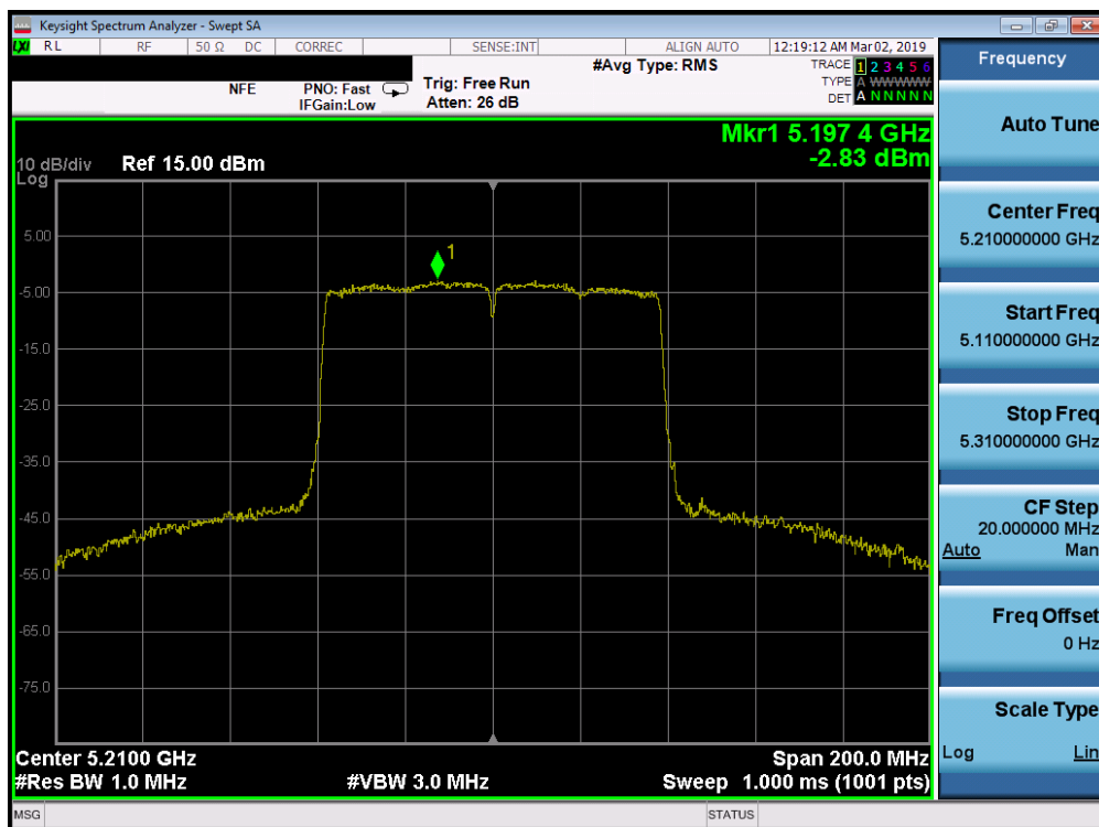
Plot 7-144. Power Spectral Density Plot SISO ANT1 (80MHz BW 802.11ac (UNII Band 1) – Ch. 42)
