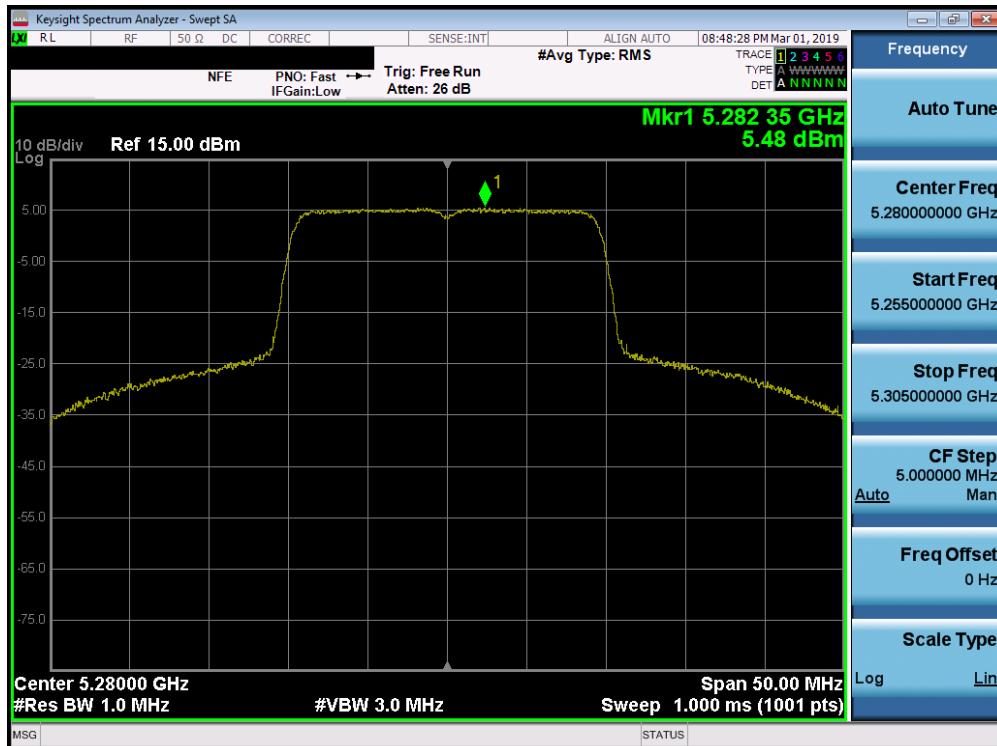
Plot 7-152. Power Spectral Density Plot SISO ANT1 (20MHz 802.11ax (UNII Band 2A) – Ch. 56)
