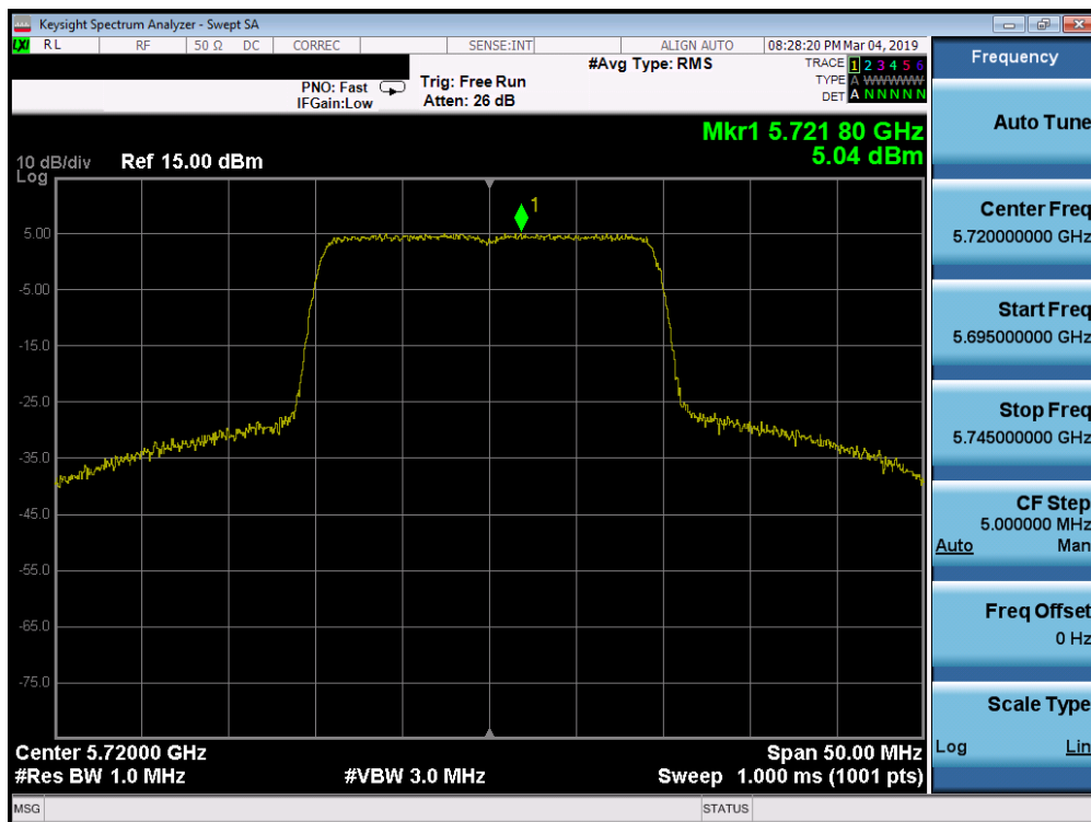
Plot 7-216. Power Spectral Density Plot SISO ANT2 (20MHz 802.11ax (UNII Band 2C) – Ch. 144)
