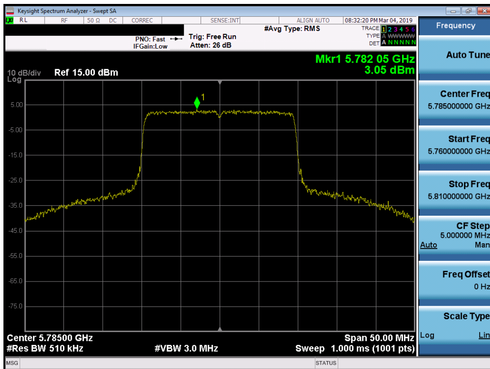
Plot 7-230. Power Spectral Density Plot SISO ANT2 (20MHz 802.11ax (UNII Band 3) – Ch. 157)
