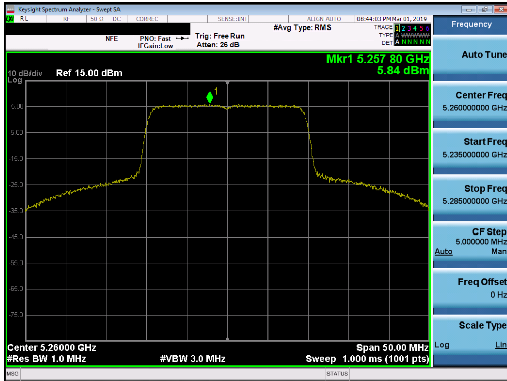
Plot 7-151. Power Spectral Density Plot SISO ANT1 (20MHz 802.11ax (UNII Band 2A) – Ch. 52)
