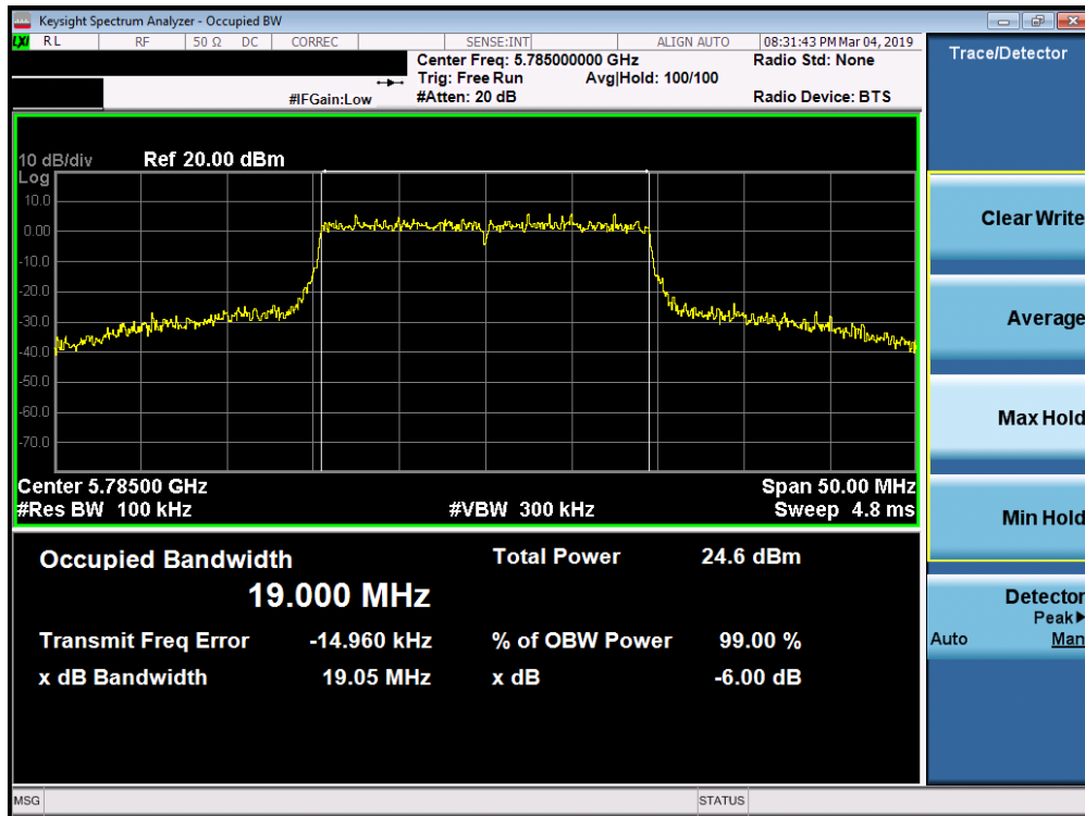
Plot 7-125. 6dB Bandwidth Plot SISO ANT2 (20MHz 802.11ax (UNII Band 3) – Ch. 157)
