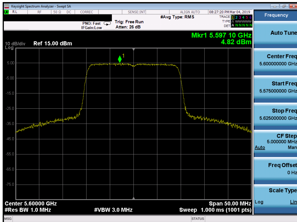
Plot 7-215. Power Spectral Density Plot SISO ANT2 (20MHz 802.11ax (UNII Band 2C) – Ch. 120)
