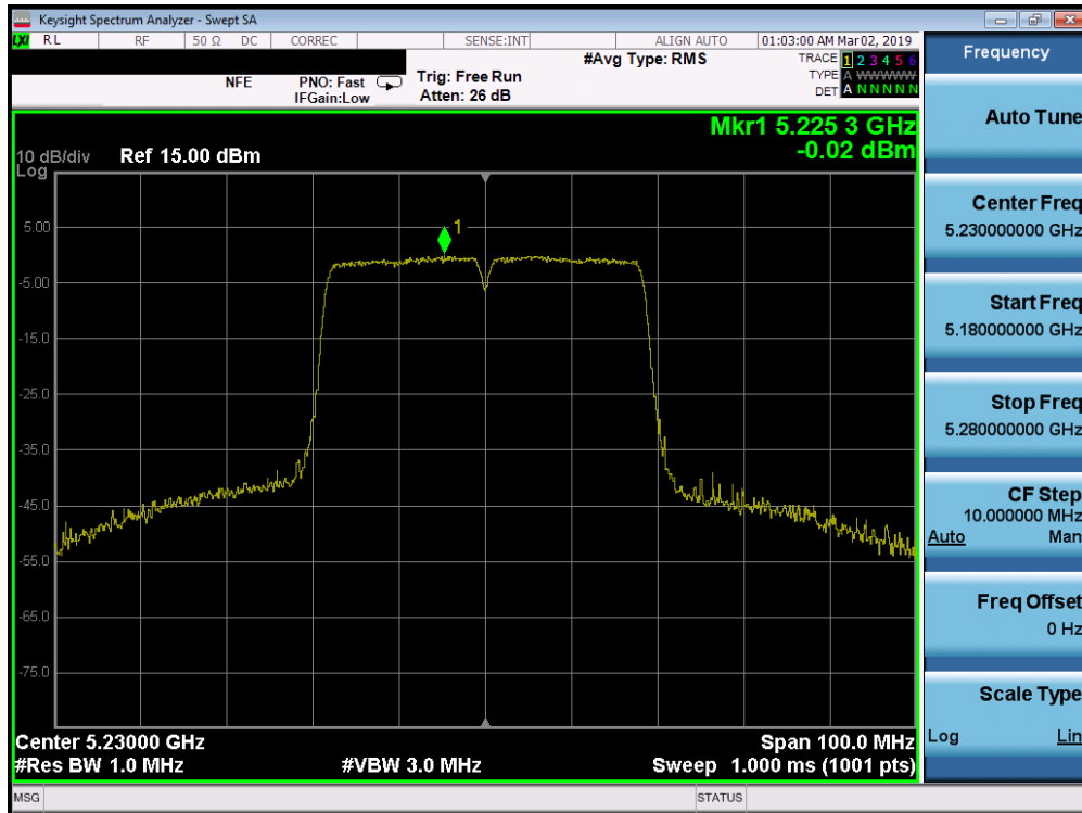
Plot 7-194. Power Spectral Density Plot SISO ANT2 (40MHz BW 802.11n (UNII Band 1) – Ch. 46)
