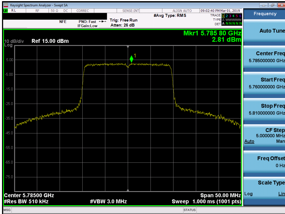
Plot 7-179. Power Spectral Density Plot SISO ANT1 (20MHz 802.11ax (UNII Band 3) – Ch. 157)
