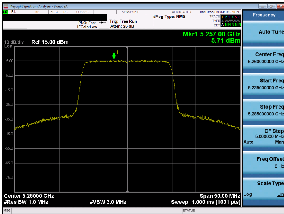
Plot 7-202. Power Spectral Density Plot SISO ANT2 (20MHz 802.11ax (UNII Band 2A) – Ch. 52)
