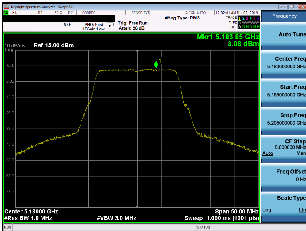
Plot 7-184. Power Spectral Density Plot SISO ANT2 (802.11a (UNII Band 1) – Ch. 36)
