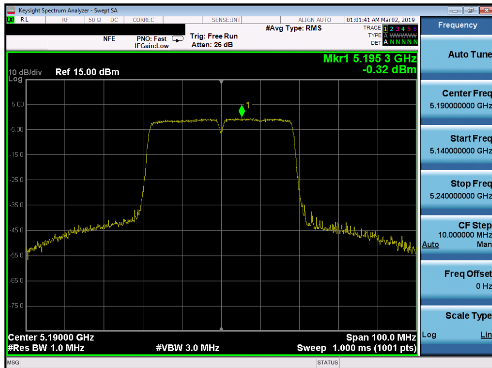
Plot 7-193. Power Spectral Density Plot SISO ANT2 (40MHz BW 802.11n (UNII Band 1) – Ch. 38)
