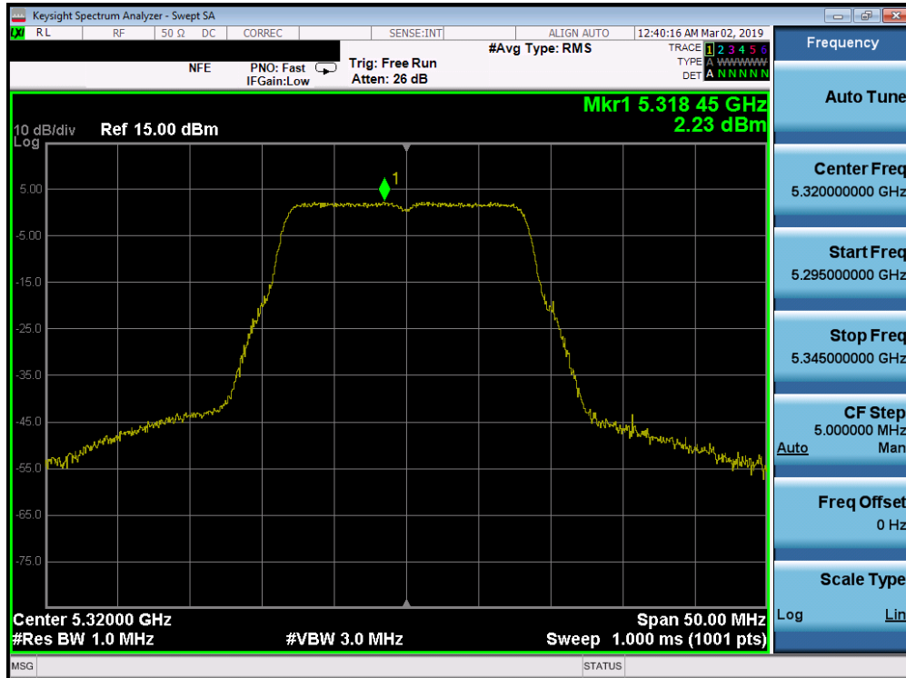
Plot 7-198. Power Spectral Density Plot SISO ANT2 (802.11a (UNII Band 2A) – Ch. 64)
