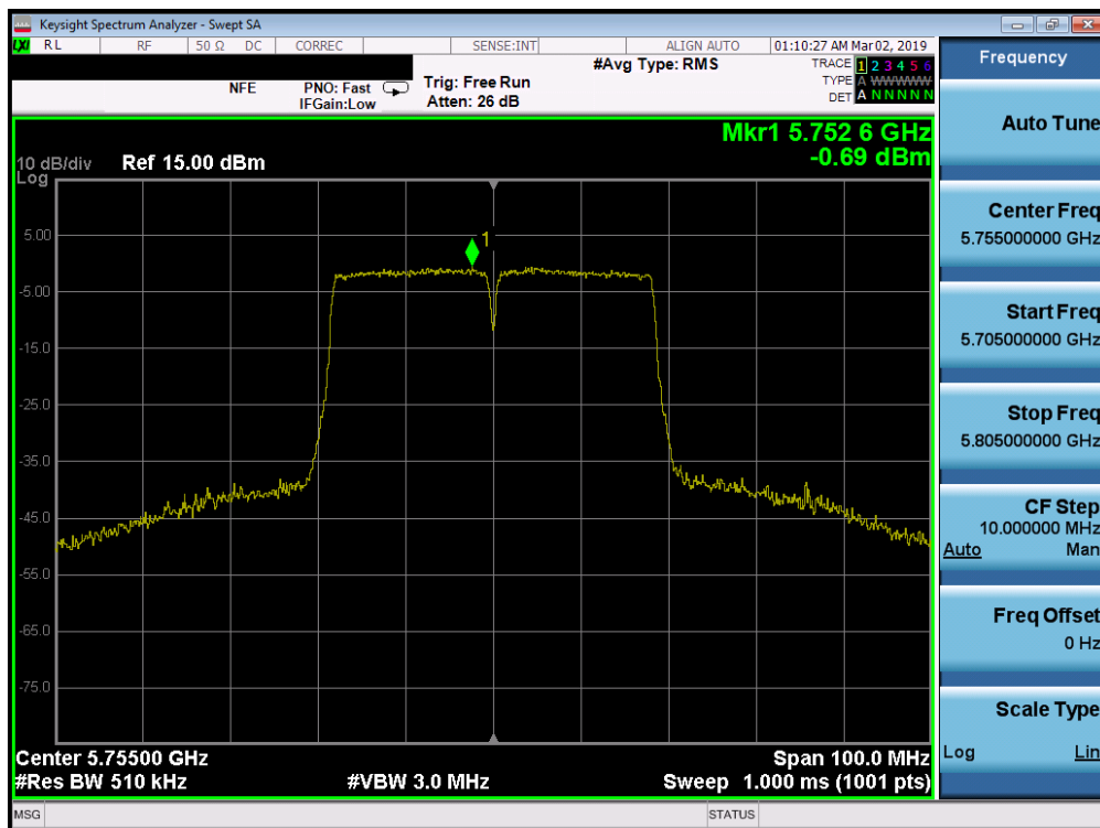
Plot 7-232. Power Spectral Density Plot SISO ANT2 (40MHz BW 802.11n (UNII Band 3) – Ch. 151)
