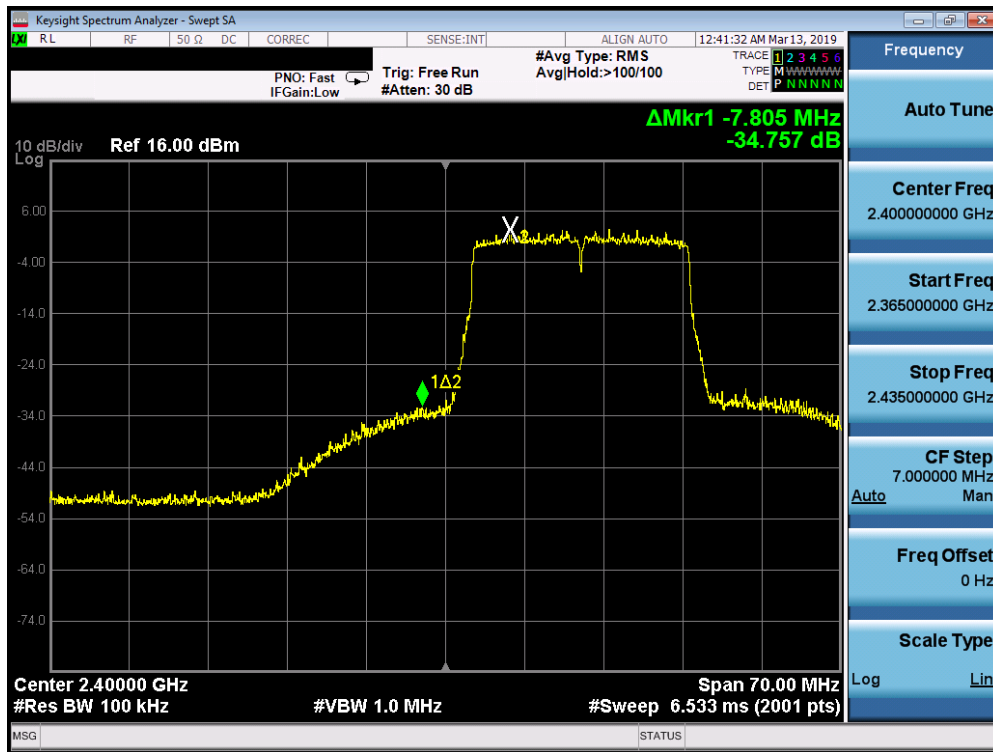
Plot 7-23. Band Edge Plot SISO ANT2 (802.11ax OFDMA - 242 Tones - Ch. 1)
