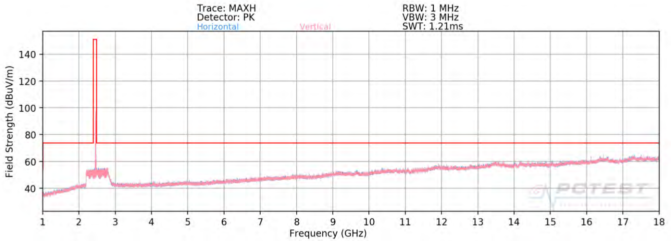
Plot 7-52. Radiated Spurious Plot above 1GHz SISO ANT2 (802.11ax OFDMA – 242 Tones – Ch. 11)
