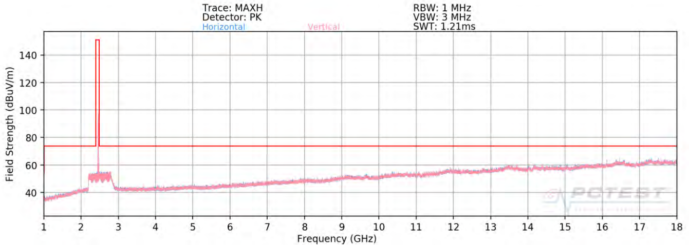
Plot 7-49. Radiated Spurious Plot above 1GHz SISO ANT2 (802.11ax OFDMA – 26 Tones – Ch. 11)
