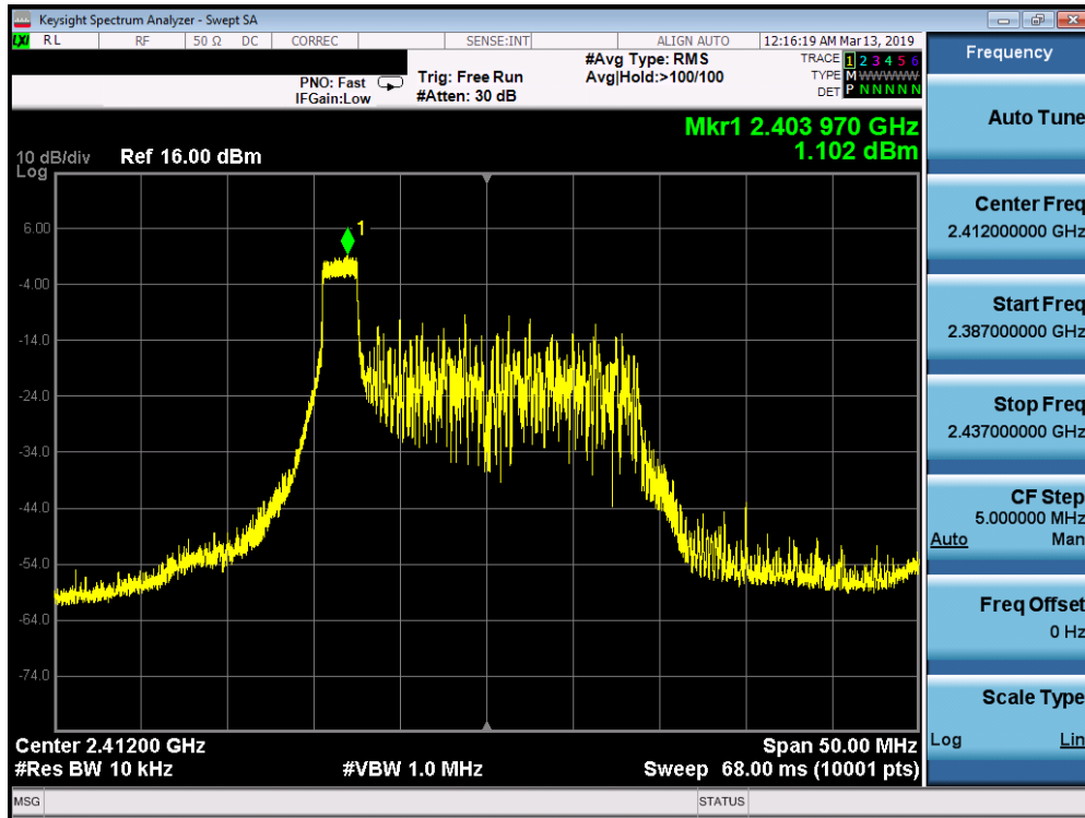
Plot 7-13. Power Spectral Density Plot ANT1 MIMO (802.11ax OFDMA – 26 Tones – Ch. 1)
