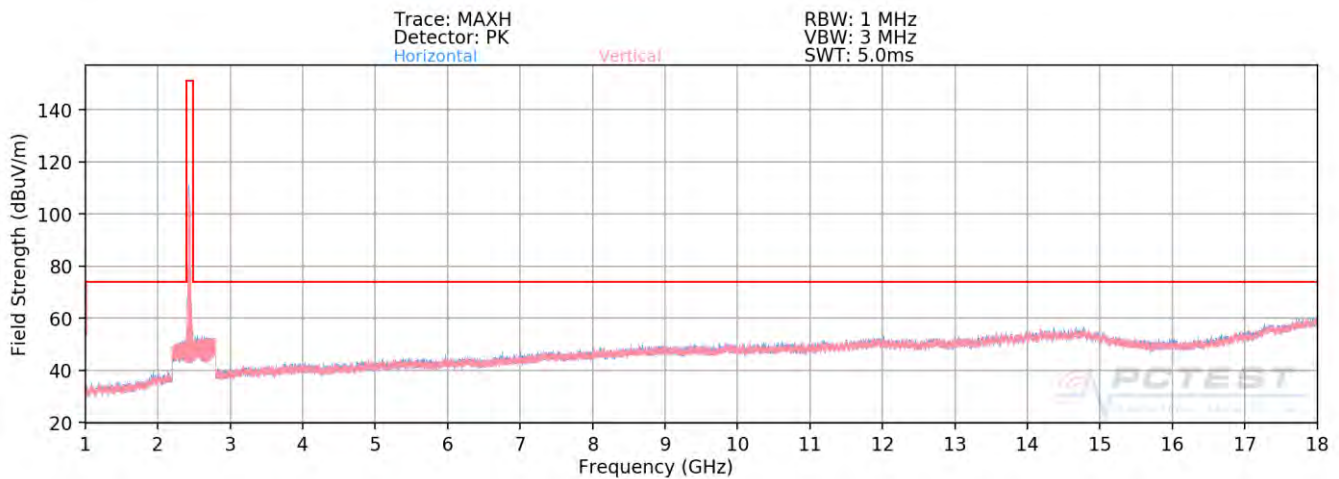
Plot 7-59. Radiated Spurious Plot above 1GHz MIMO (802.11ax OFDMA – 242 Tones – Ch. 6)
