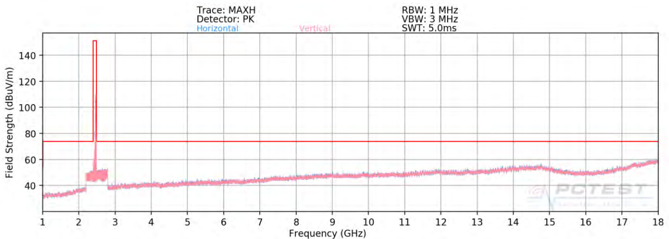
Plot 7-60. Radiated Spurious Plot above 1GHz MIMO (802.11ax OFDMA – 242 Tones – Ch. 11)
