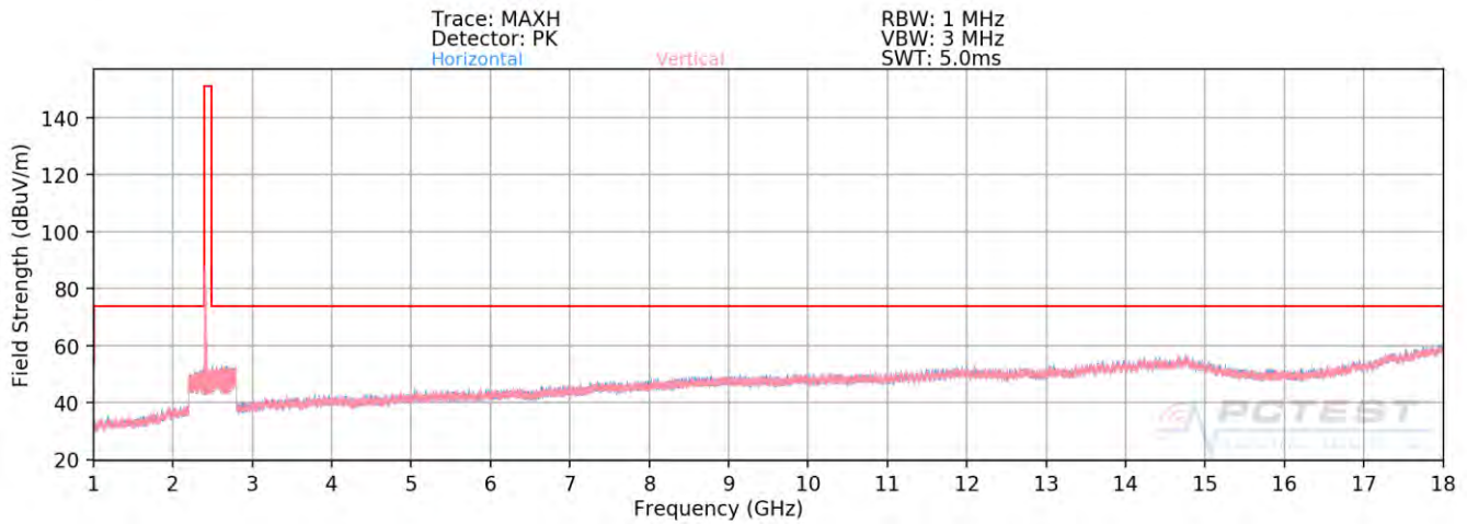
Plot 7-55. Radiated Spurious Plot above 1GHz MIMO (802.11ax OFDMA – 26 Tones – Ch. 1)
