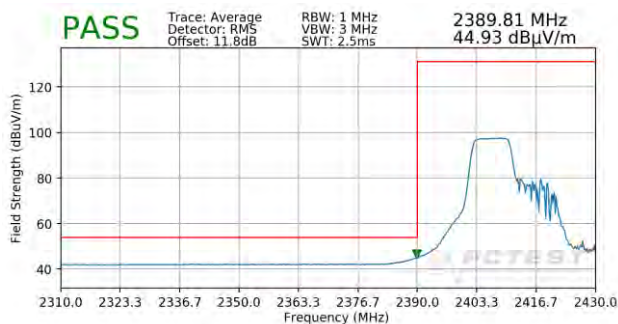
Plot 7-87. Radiated Restricted Lower Band Edge Measurement SISO ANT2 (Average – 106 Tones)
