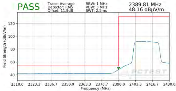
Plot 7-99. Radiated Restricted Lower Band Edge Measurement SISO ANT2 (Average – 242 Tones)
