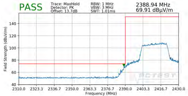
Plot 7-76. Radiated Restricted Lower Band Edge Measurement SISO ANT1 (Peak – 242 Tones)
