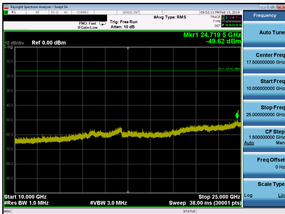
Plot 7-32. Conducted Spurious Plot SISO ANT1 (802.11ax OFDMA- 242 Tones – Ch. 11)
