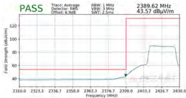
Plot 7-101. Radiated Restricted Lower Band Edge Measurement SISO ANT2 (Average – 242 Tones)
