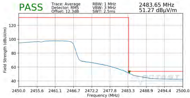
Plot 7-79. Radiated Restricted Upper Band Edge Measurement SISO ANT1 (Average – 242 Tones)
