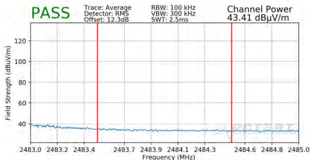
Plot 7-97. Radiated Restricted Upper Band Edge Measurement SISO ANT2 (Average – 106 Tones)
