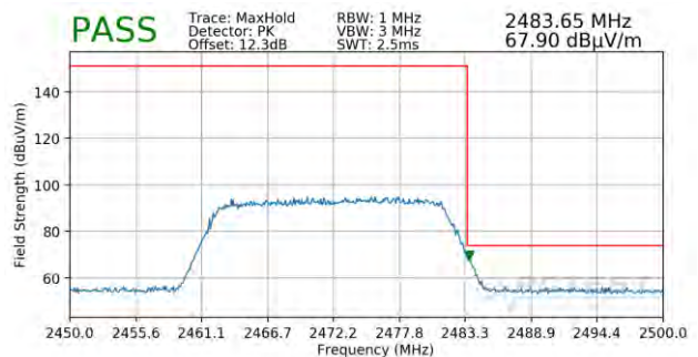
Plot 7-110. Radiated Restricted Upper Band Edge Measurement SISO ANT2 (Peak – 242 Tones)
