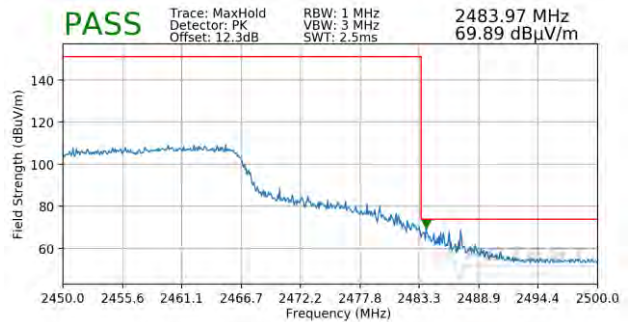
Plot 7-80. Radiated Restricted Upper Band Edge Measurement SISO ANT1 (Peak – 242 Tones)
