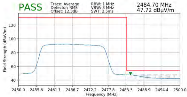
Plot 7-131. Radiated Restricted Upper Band Edge Measurement MIMO (Average – 242 Tones)
