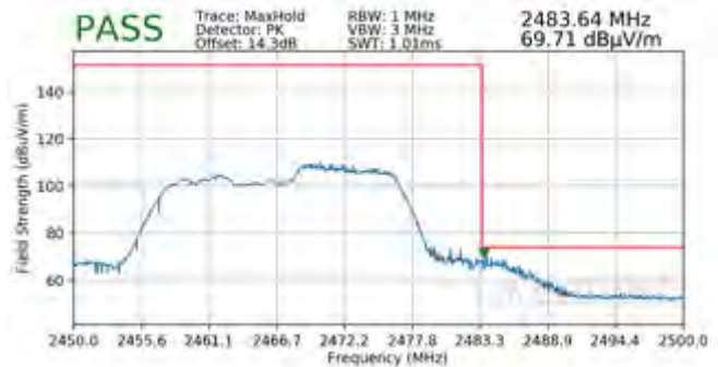
Plot 7-72. Radiated Restricted Upper Band Edge Measurement SISO ANT1 (Peak – 106 Tones)
