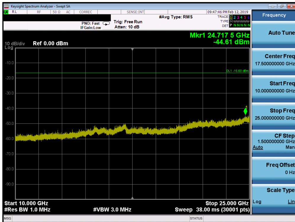
Plot 7-36. Conducted Spurious Plot SISO ANT2 (802.11ax OFDMA- 242 Tones – Ch. 6)
