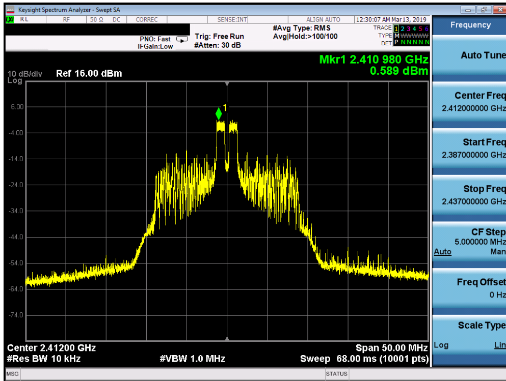
Plot 7-16. Power Spectral Density Plot ANT2 MIMO (802.11ax OFDMA – 26 Tones – Ch. 1)
