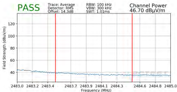
Plot 7-73. Radiated Restricted Upper Band Edge Measurement SISO ANT1 (Average – 106 Tones)
