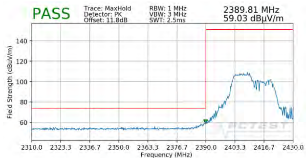
Plot 7-88. Radiated Restricted Lower Band Edge Measurement SISO ANT2 (Peak – 106 Tones)
