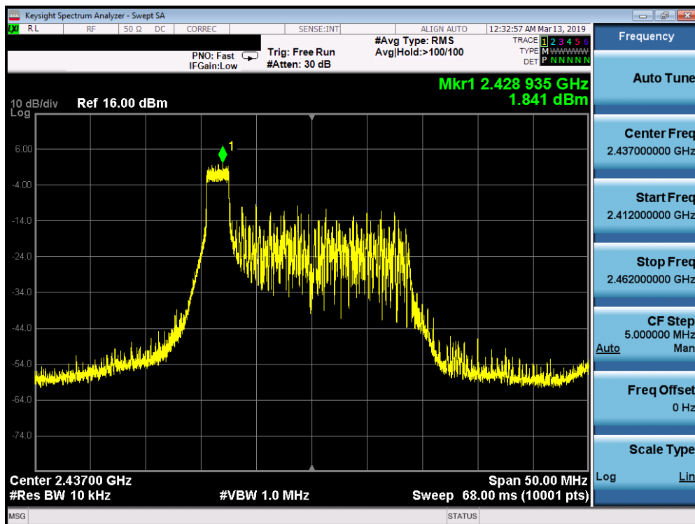
Plot 7-17. Power Spectral Density Plot ANT2 MIMO (802.11ax OFDMA – 26 Tones – Ch. 6)
