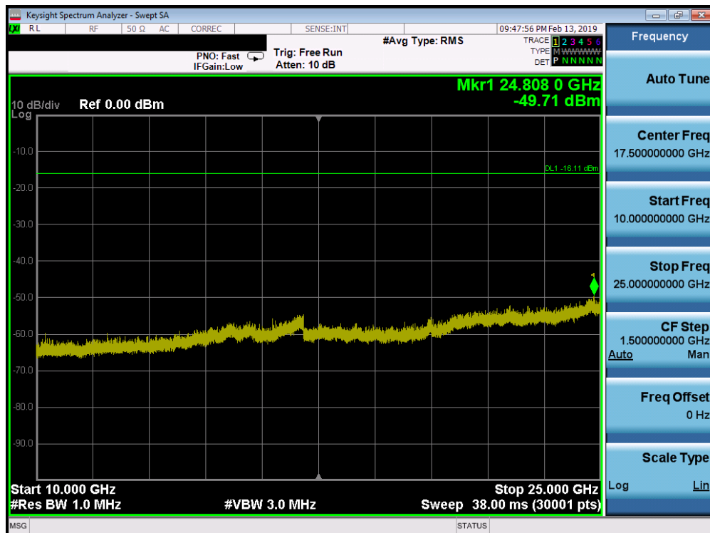
Plot 7-28. Conducted Spurious Plot SISO ANT1 (802.11ax OFDMA– 242 Tones – Ch. 1)
