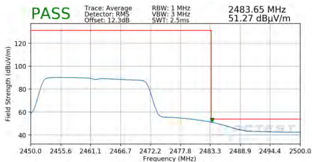
Plot 7-105. Radiated Restricted Upper Band Edge Measurement SISO ANT2 (Average – 242 Tones)
