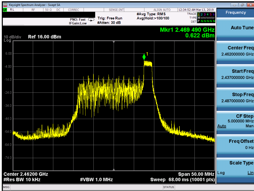
Plot 7-18. Power Spectral Density Plot ANT2 MIMO (802.11ax OFDMA – 26 Tones – Ch. 11)
