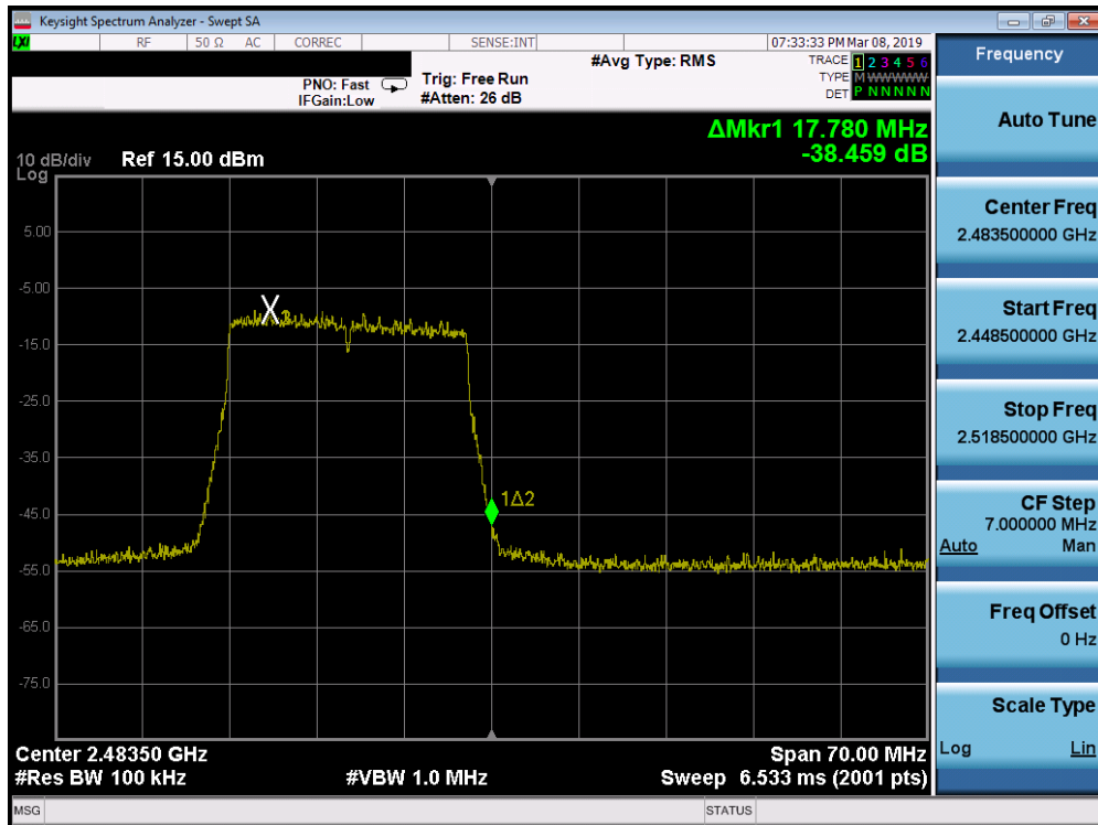
Plot 7-22. Band Edge Plot SISO ANT1 (802.11ax OFDMA - 242 Tones - Ch. 13)
