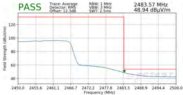
Plot 7-127. Radiated Restricted Upper Band Edge Measurement MIMO (Average – 242 Tones)
