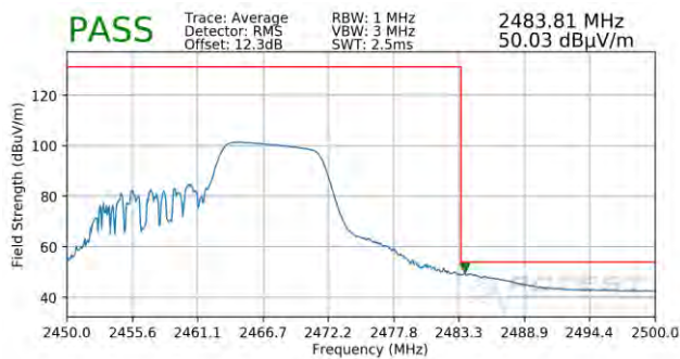
Plot 7-69. Radiated Restricted Upper Band Edge Measurement SISO ANT1 (Average – 106 Tones)
