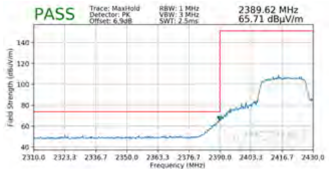
Plot 7-126. Radiated Restricted Lower Band Edge Measurement MIMO (Peak - 242 Tones)
