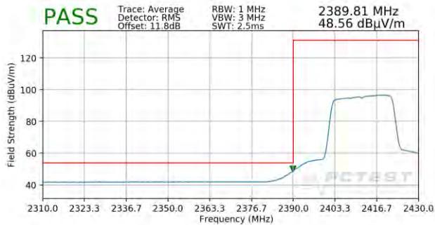
Plot 7-123. Radiated Restricted Lower Band Edge Measurement MIMO (Average - 242 Tones)
