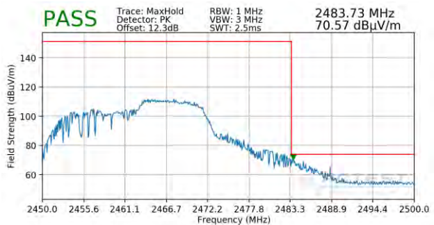
Plot 7-70. Radiated Restricted Upper Band Edge Measurement SISO ANT1 (Peak – 106 Tones)
