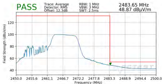
Plot 7-117. Radiated Restricted Upper Band Edge Measurement MIMO (Average – 106 Tones)
