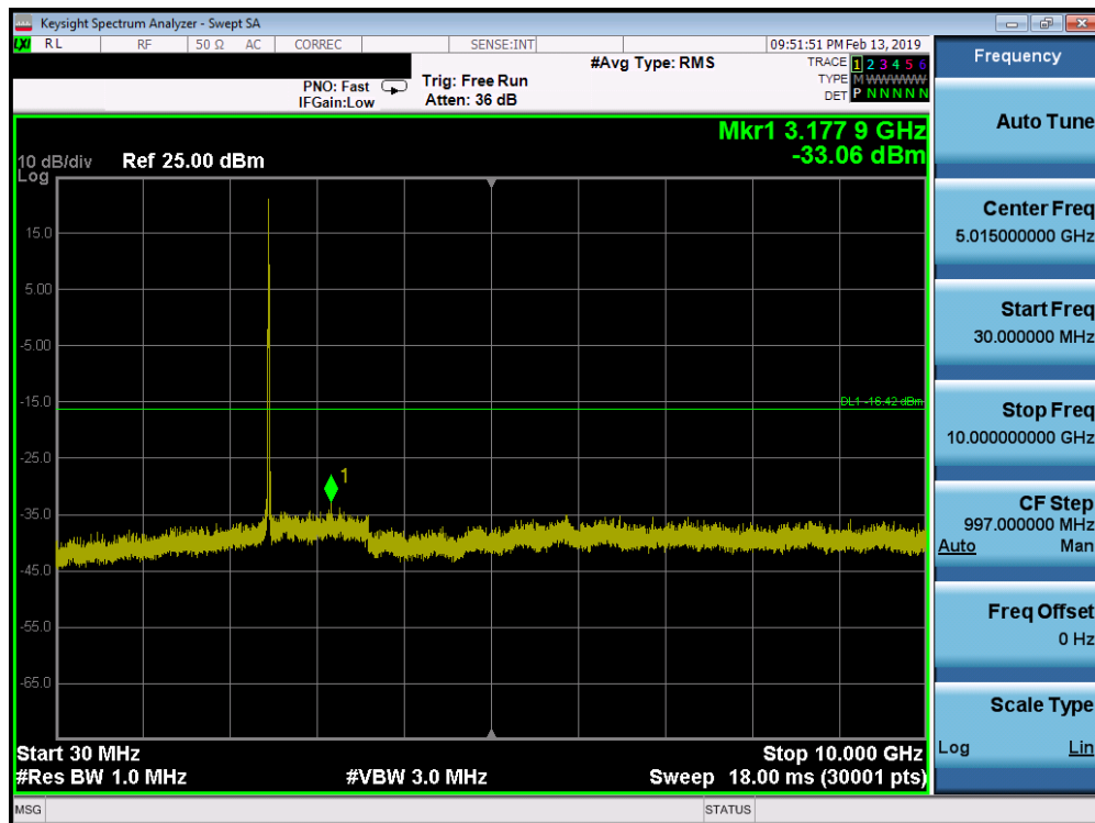
Plot 7-31. Conducted Spurious Plot SISO ANT1 (802.11ax OFDMA- 242 Tones – Ch. 11)
