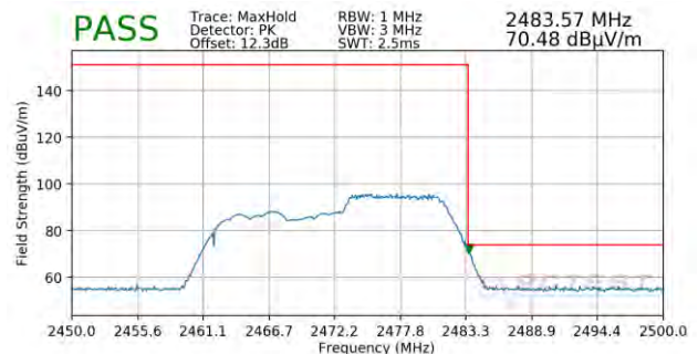
Plot 7-98. Radiated Restricted Upper Band Edge Measurement SISO ANT2 (Peak – 106 Tones)
