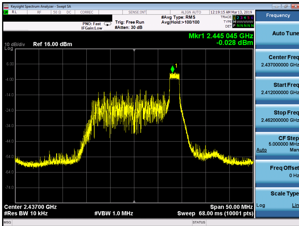
Plot 7-14. Power Spectral Density Plot ANT1 MIMO (802.11ax OFDMA – 26 Tones – Ch. 6)
