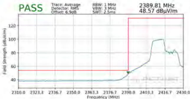
Plot 7-113. Radiated Restricted Lower Band Edge Measurement MIMO (Average – 106 Tones)
