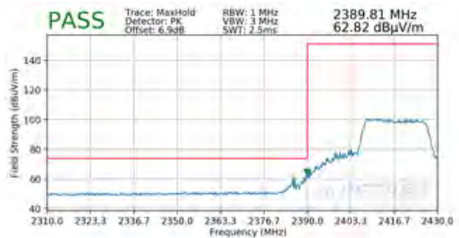
Plot 7-102. Radiated Restricted Lower Band Edge Measurement SISO ANT2 (Peak – 242 Tones)
