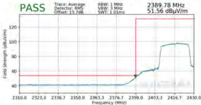
Plot 7-77. Radiated Restricted Lower Band Edge Measurement SISO ANT1 (Average – 242 Tones)
