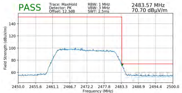
Plot 7-134. Radiated Restricted Upper Band Edge Measurement MIMO (Peak – 242 Tones)
