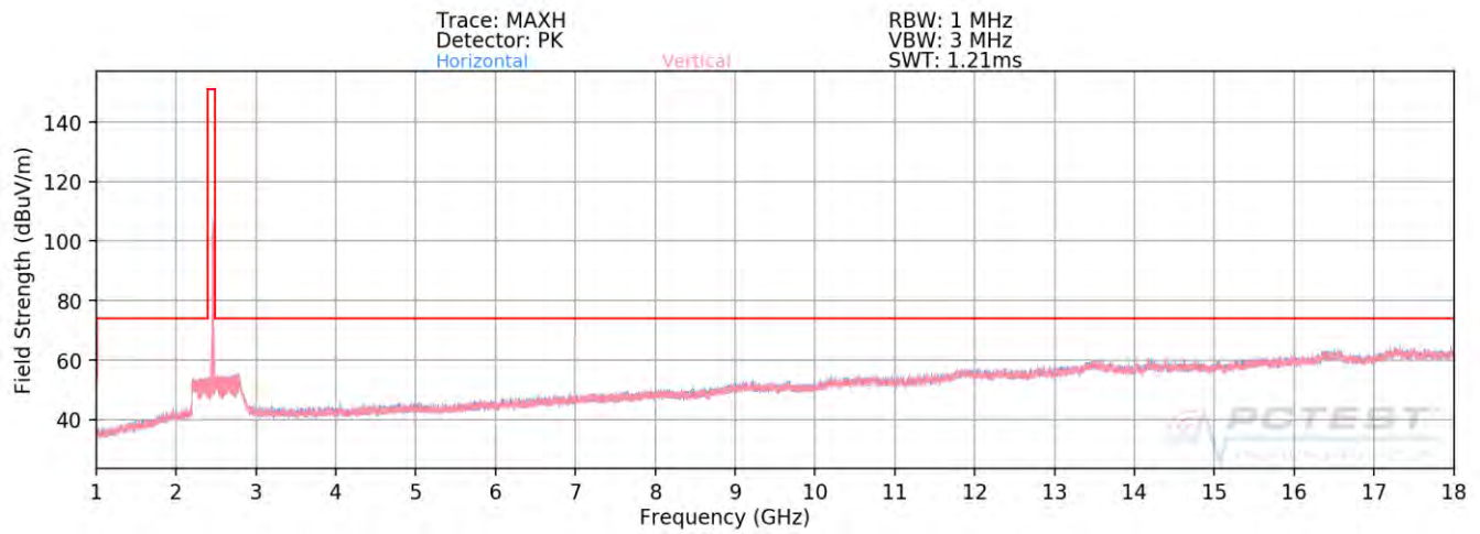
Plot 7-44. Radiated Spurious Plot above 1GHz SISO ANT1 (802.11ax OFDMA – 242 Tones – Ch. 11)
