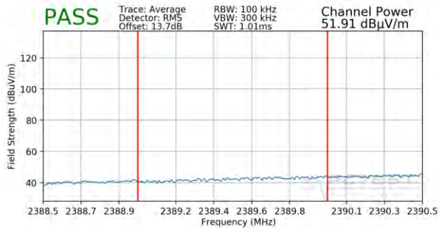
Plot 7-75. Radiated Restricted Lower Band Edge Measurement SISO ANT1 (Average – 242 Tones)
