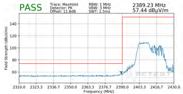
Plot 7-112. Radiated Restricted Lower Band Edge Measurement MIMO (Peak – 106 Tones)
