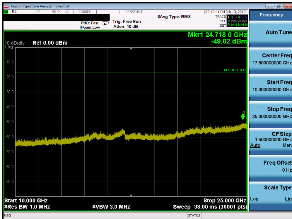
Plot 7-30. Conducted Spurious Plot SISO ANT1 (802.11ax OFDMA- 242 Tones – Ch. 6)
