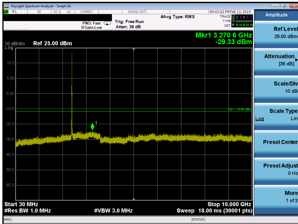
Plot 7-33. Conducted Spurious Plot SISO ANT2 (802.11ax OFDMA – 242 Tones – Ch. 1)
