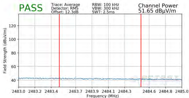
Plot 7-129. Radiated Restricted Upper Band Edge Measurement MIMO (Average – 242 Tones)
