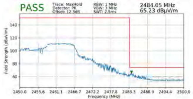
Plot 7-68. Radiated Restricted Upper Band Edge Measurement SISO ANT1 (Peak – 106 Tones)
