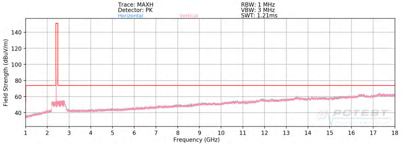
Plot 7-47. Radiated Spurious Plot above 1GHz SISO ANT2 (802.11ax OFDMA – 26 Tones – Ch. 1)
