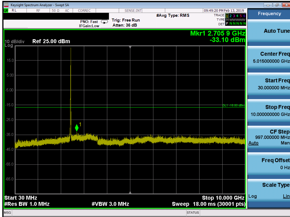
Plot 7-29. Conducted Spurious Plot SISO ANT1 (802.11ax OFDMA- 242 Tones – Ch. 6)
