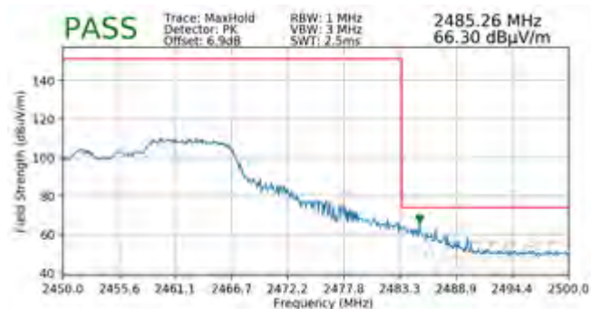
Plot 7-116. Radiated Restricted Upper Band Edge Measurement MIMO (Peak – 106 Tones)
