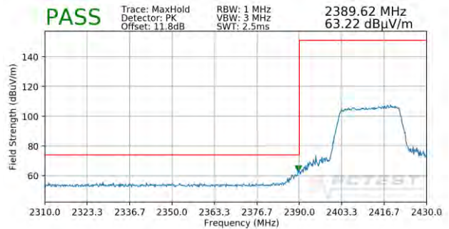
Plot 7-124. Radiated Restricted Lower Band Edge Measurement MIMO (Peak - 242 Tones)
