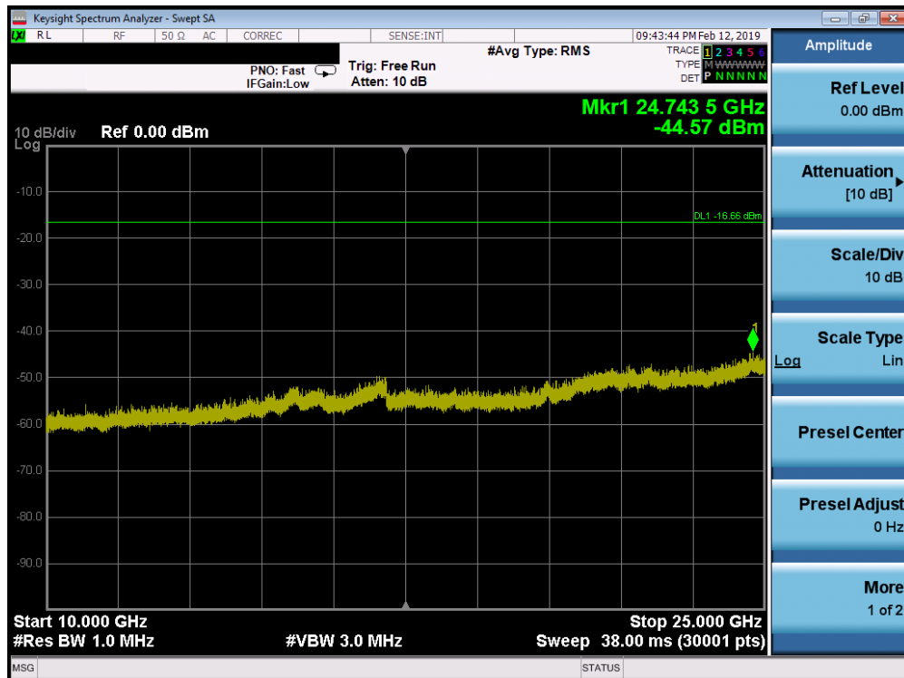
Plot 7-34. Conducted Spurious Plot SISO ANT2 (802.11ax OFDMA– 242 Tones – Ch. 1)
