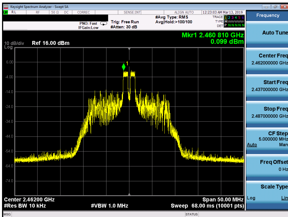
Plot 7-15. Power Spectral Density Plot ANT1 MIMO (802.11ax OFDMA – 26 Tones – Ch. 11)
