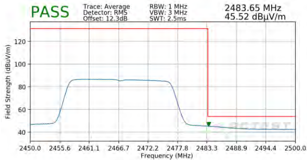
Plot 7-107. Radiated Restricted Band Edge Measurement SISO ANT2 with WCP (Average – 242 Tones)
