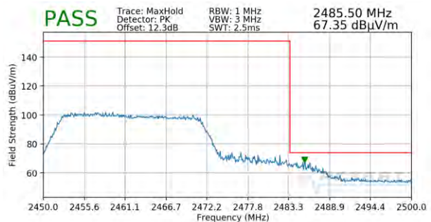
Plot 7-106. Radiated Restricted Upper Band Edge Measurement SISO ANT2 (Peak – 242 Tones)
