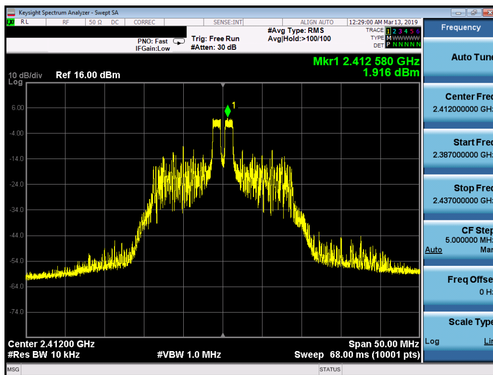
Plot 7-10. Power Spectral Density Plot SISO ANT2 (802.11ax OFDMA – 26 Tones – Ch. 1)
