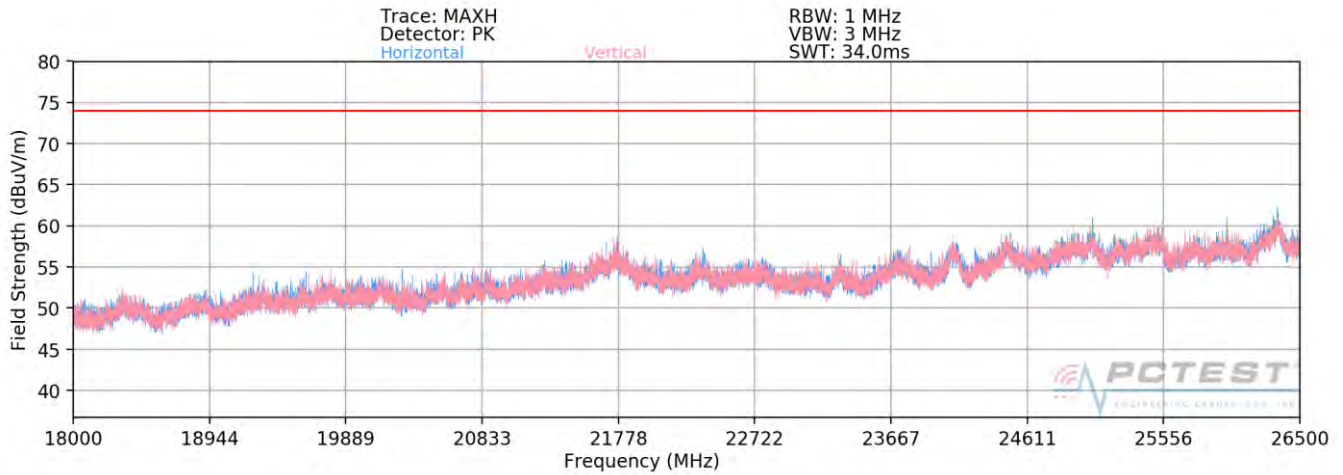
Plot 7-53. Radiated Spurious Plot above 18GHz SISO ANT2 (802.11ax OFDMA – 26 Tones)
