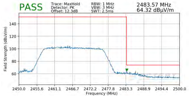
Plot 7-132. Radiated Restricted Upper Band Edge Measurement MIMO (Peak – 242 Tones)
