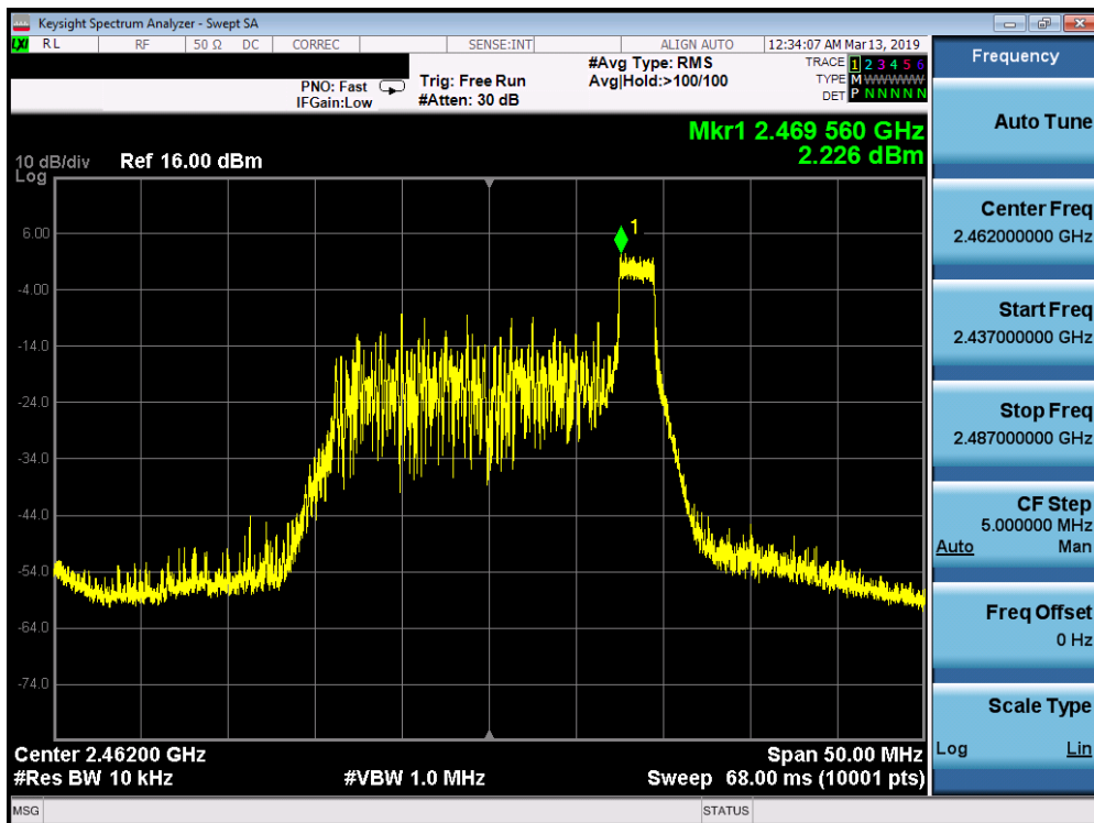
Plot 7-12. Power Spectral Density Plot SISO ANT2 (802.11ax OFDMA – 26 Tones – Ch. 11)
