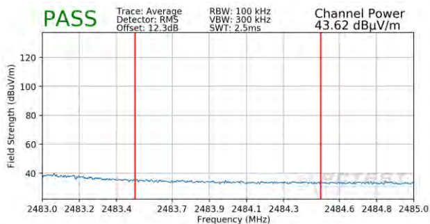
Plot 7-109. Radiated Restricted Upper Band Edge Measurement SISO ANT2 (Average – 242 Tones)
