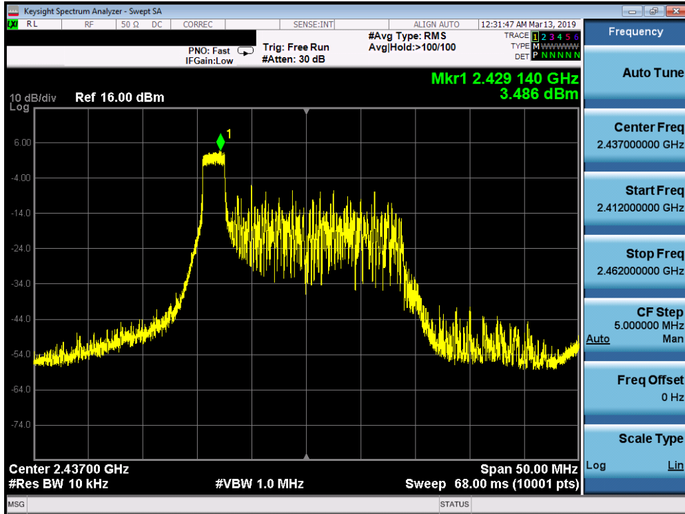
Plot 7-11. Power Spectral Density Plot SISO ANT2 (802.11ax OFDMA – 26 Tones – Ch. 6)
