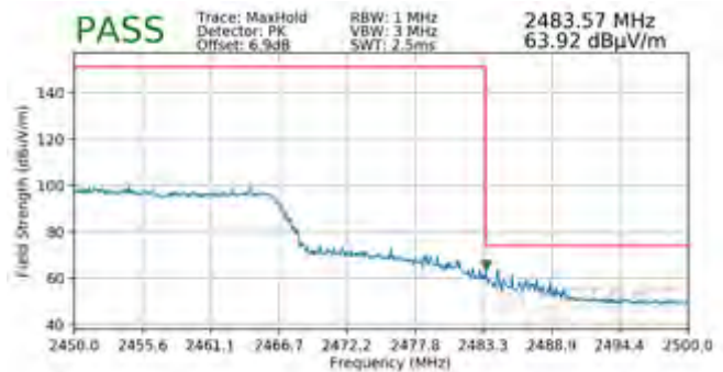
Plot 7-104. Radiated Restricted Upper Band Edge Measurement SISO ANT2 (Peak – 242 Tones)
