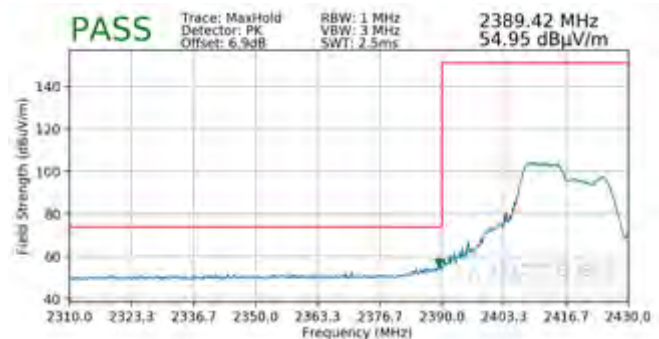
Plot 7-90. Radiated Restricted Lower Band Edge Measurement SISO ANT2 (Peak – 106 Tones)
