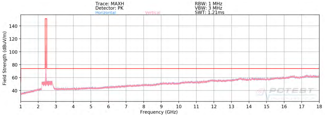
Plot 7-40. Radiated Spurious Plot above 1GHz SISO ANT1 (802.11ax OFDMA – 26 Tones – Ch. 6)
