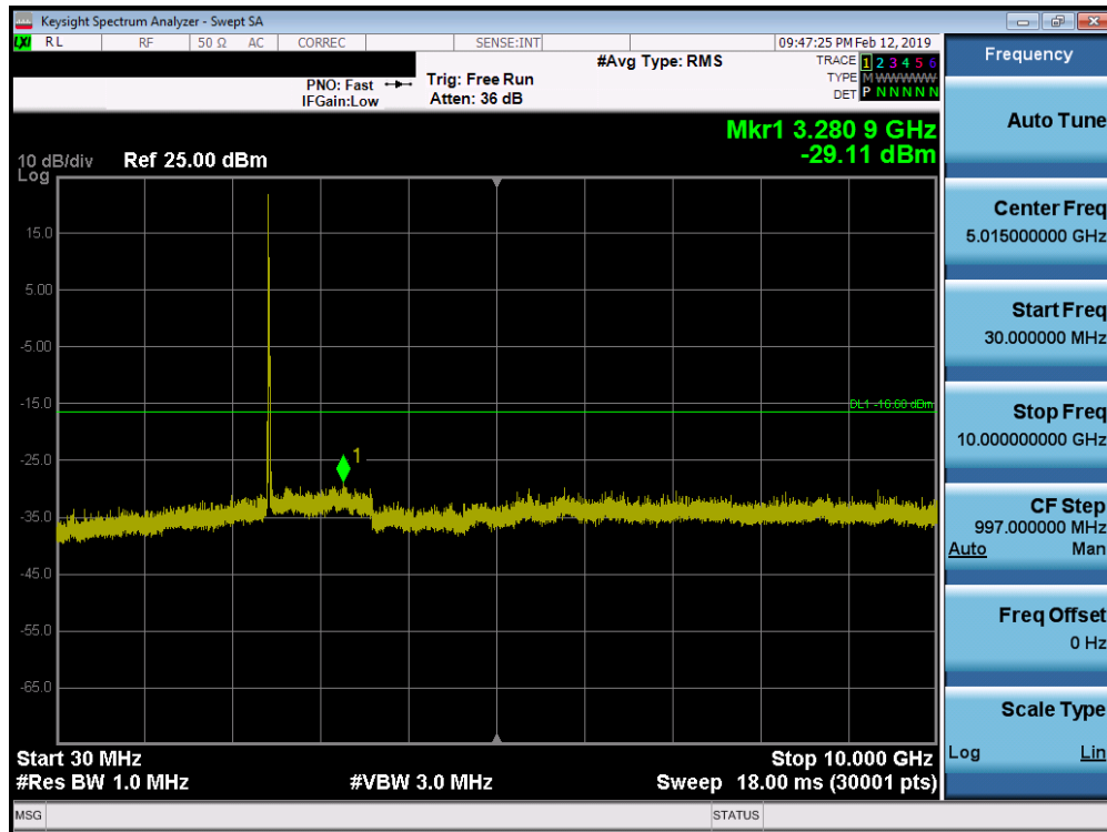
Plot 7-35. Conducted Spurious Plot SISO ANT2 (802.11ax OFDMA- 242 Tones – Ch. 6)
