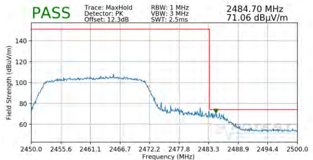
Plot 7-82. Radiated Restricted Upper Band Edge Measurement SISO ANT1 (Peak – 242 Tones)
