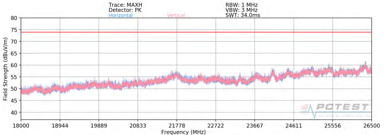
Plot 7-46. Radiated Spurious Plot above 18GHz SISO ANT1 (802.11ax OFDMA – 242 Tones)
