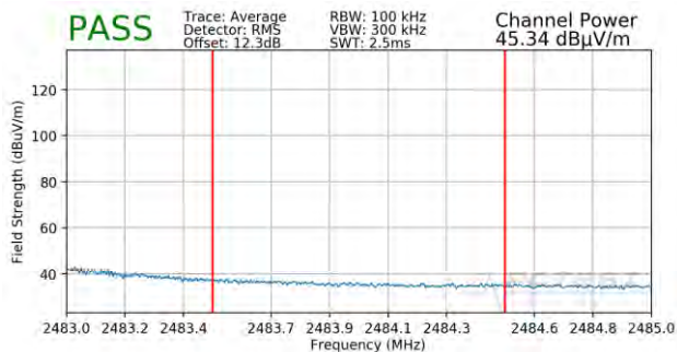
Plot 7-133. Radiated Restricted Upper Band Edge Measurement MIMO (Average – 242 Tones)
