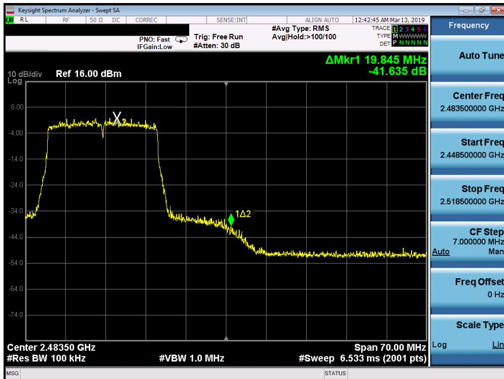
Plot 7-24. Band Edge Plot SISO ANT2 (802.11ax OFDMA - 242 Tones - Ch. 11)
