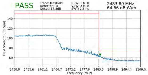
Plot 7-128. Radiated Restricted Upper Band Edge Measurement MIMO (Peak – 242 Tones)
