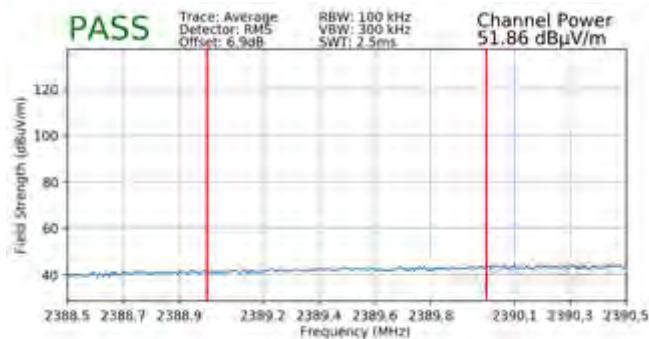
Plot 7-125. Radiated Restricted Lower Band Edge Measurement MIMO (Average - 242 Tones)
