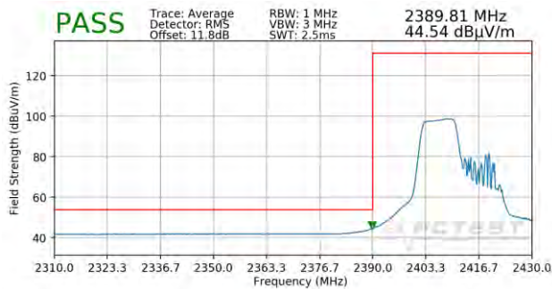
Plot 7-111. Radiated Restricted Lower Band Edge Measurement MIMO (Average – 106 Tones)
