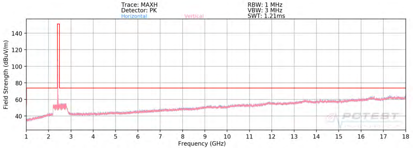
Plot 7-39. Radiated Spurious Plot above 1GHz SISO ANT1 (802.11ax OFDMA – 26 Tones – Ch. 1)
