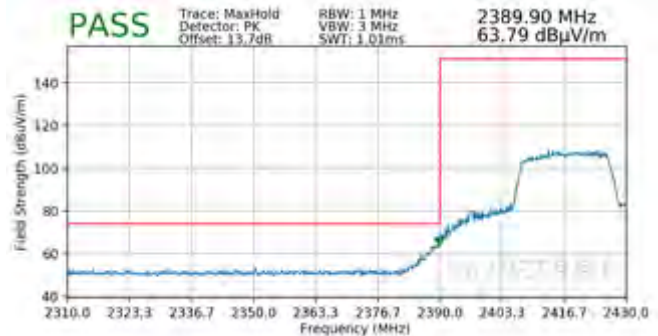
Plot 7-78. Radiated Restricted Lower Band Edge Measurement SISO ANT1 (Peak – 242 Tones)
