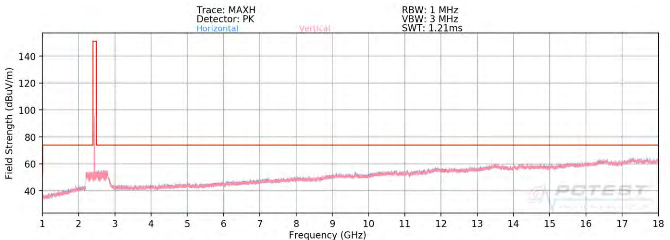
Plot 7-51. Radiated Spurious Plot above 1GHz SISO ANT2 (802.11ax OFDMA – 242 Tones – Ch. 6)
