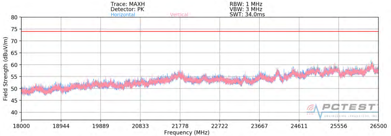
Plot 7-45. Radiated Spurious Plot above 18GHz SISO ANT1 (802.11ax OFDMA – 26 Tones)
