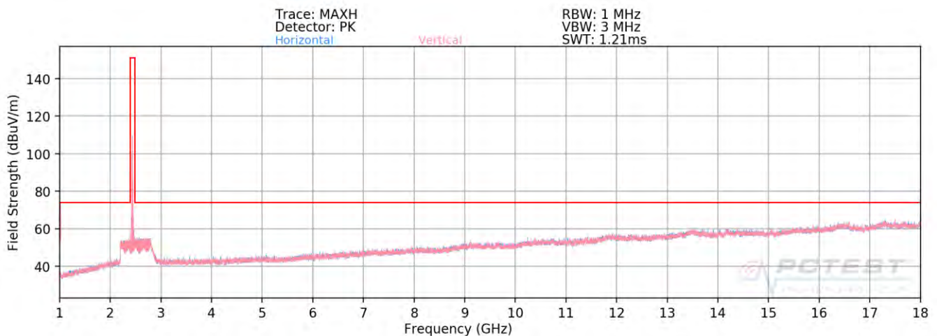
Plot 7-43. Radiated Spurious Plot above 1GHz SISO ANT1 (802.11ax OFDMA – 242 Tones – Ch. 6)
