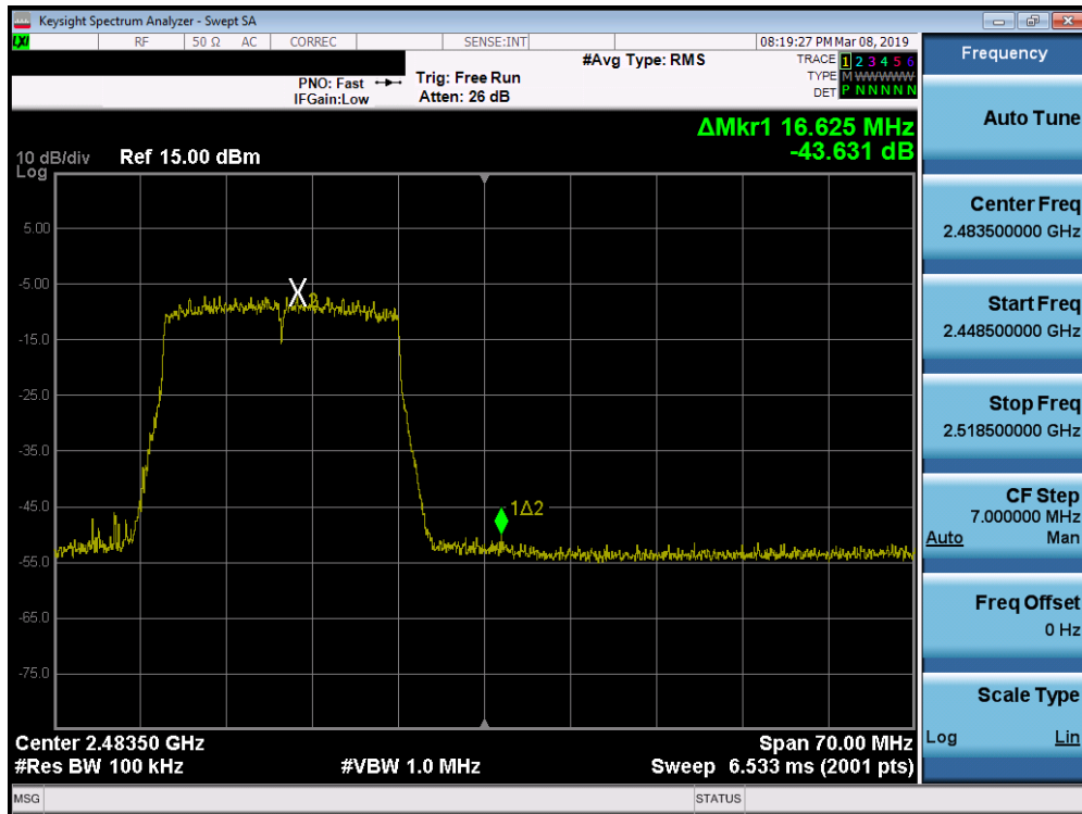
Plot 7-21. Band Edge Plot SISO ANT1 (802.11ax OFDMA - 242 Tones - Ch. 12)
