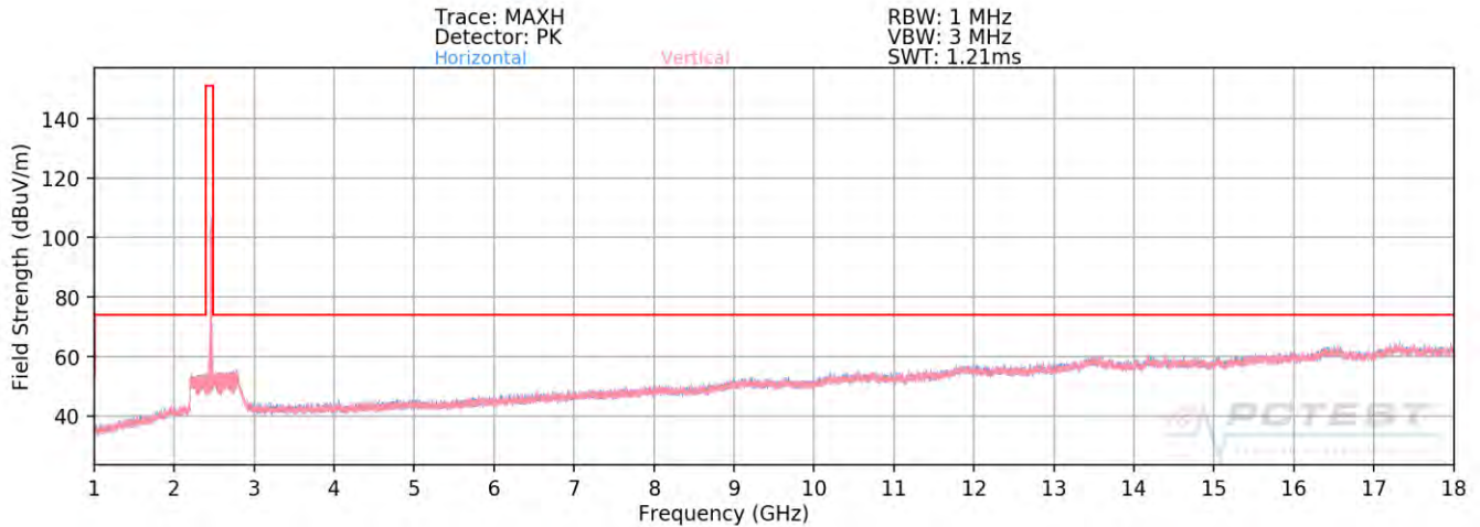
Plot 7-41. Radiated Spurious Plot above 1GHz SISO ANT1 (802.11ax OFDMA – 26 Tones – Ch. 11)
