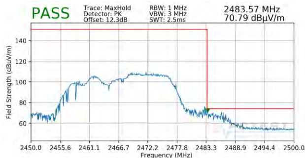
Plot 7-118. Radiated Restricted Upper Band Edge Measurement MIMO (Peak – 106 Tones)
