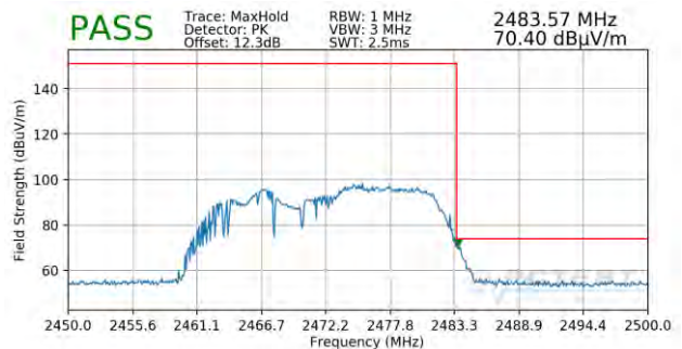
Plot 7-122. Radiated Restricted Upper Band Edge Measurement MIMO (Peak – 106 Tones)
