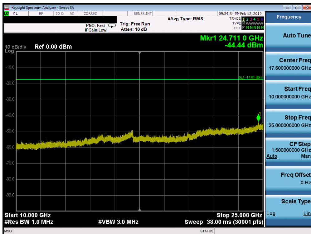
Plot 7-38. Conducted Spurious Plot SISO ANT2 (802.11ax OFDMA– 242 Tones – Ch. 11)
