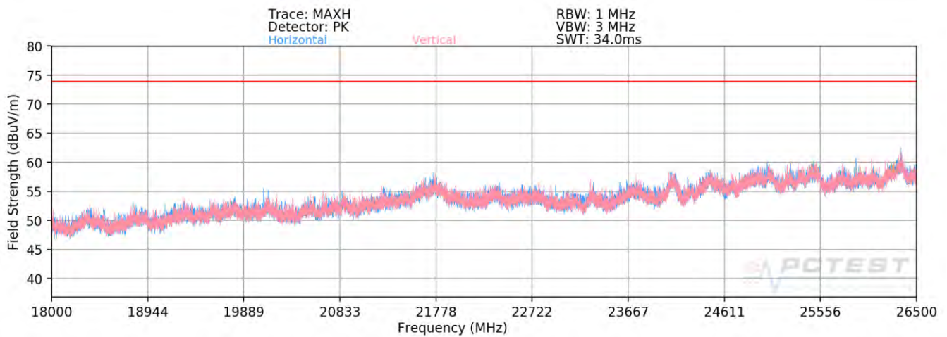
Plot 7-62. Radiated Spurious Plot above 18GHz MIMO (802.11ax OFDMA – 242 Tones)
