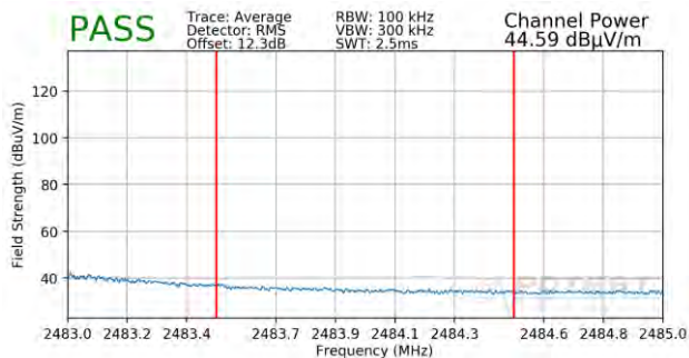
Plot 7-121. Radiated Restricted Upper Band Edge Measurement MIMO (Average – 106 Tones)
