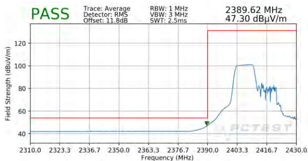
Plot 7-63. Radiated Restricted Lower Band Edge Measurement SISO ANT1 (Average – 106 Tones)
