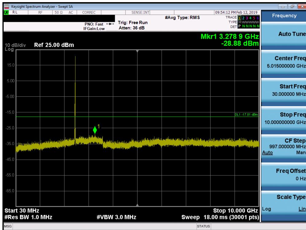
Plot 7-37. Conducted Spurious Plot SISO ANT2 (802.11ax OFDMA– 242 Tones – Ch. 11)
