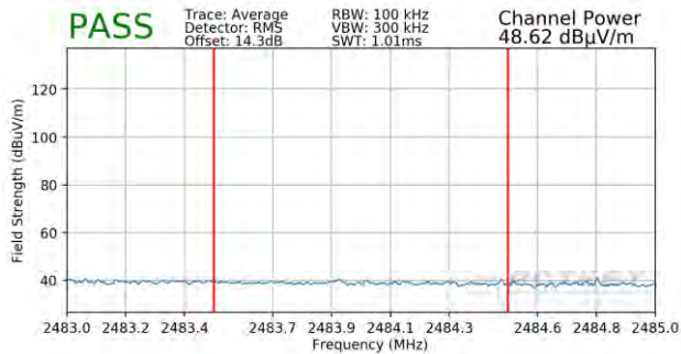
Plot 7-71. Radiated Restricted Upper Band Edge Measurement SISO ANT1 (Average – 106 Tones)
