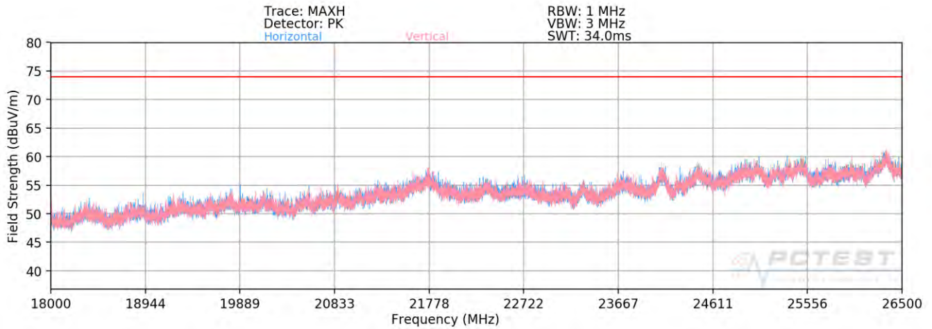
Plot 7-61. Radiated Spurious Plot above 18GHz MIMO (802.11ax OFDMA – 26 Tones)
