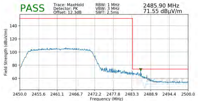
Plot 7-130. Radiated Restricted Upper Band Edge Measurement MIMO (Peak – 242 Tones)
