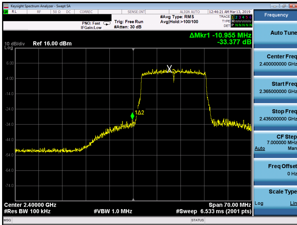
Plot 7-19. Band Edge Plot SISO ANT1 (802.11ax OFDMA – 242 Tones – Ch. 1)
