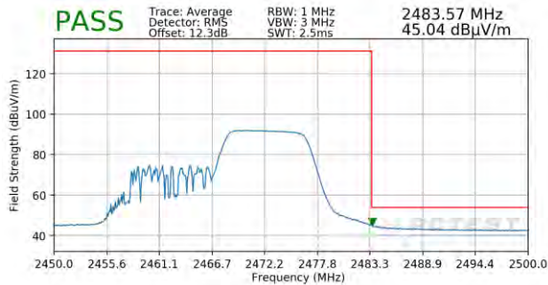
Plot 7-95. Radiated Restricted Upper Band Edge Measurement SISO ANT2 (Average – 106 Tones)
