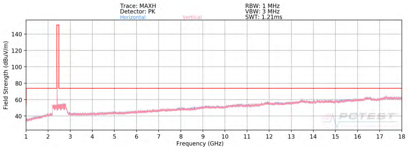
Plot 7-50. Radiated Spurious Plot above 1GHz SISO ANT2 (802.11ax OFDMA – 242 Tones – Ch. 1)
