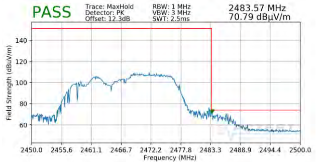
Plot 7-120. Radiated Restricted Upper Band Edge Measurement MIMO (Peak – 106 Tones)
