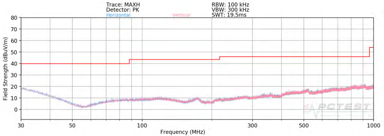
Plot 7-135. Radiated Spurious Plot below 1GHz MIMO (26 Tones)
