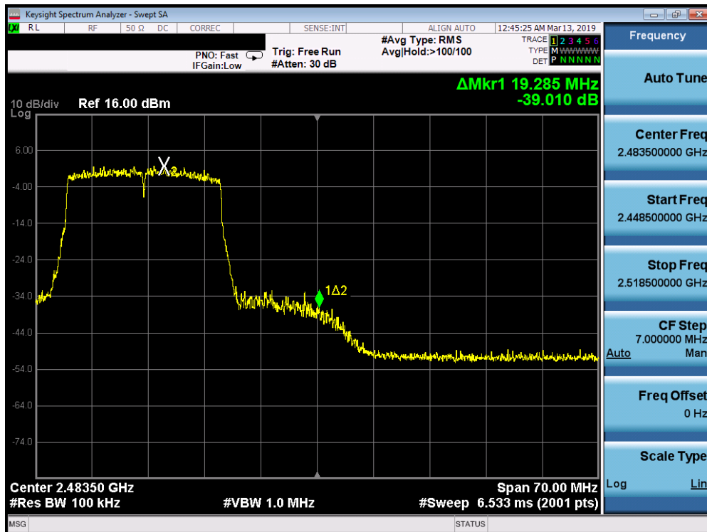
Plot 7-20. Band Edge Plot SISO ANT1 (802.11ax OFDMA – 242 Tones – Ch. 11)
