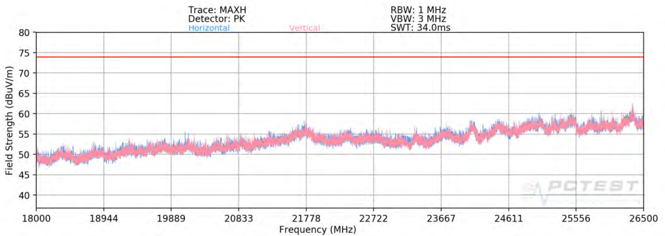
Plot 7-54. Radiated Spurious Plot above 18GHz SISO ANT2 (802.11ax OFDMA – 242 Tones)
