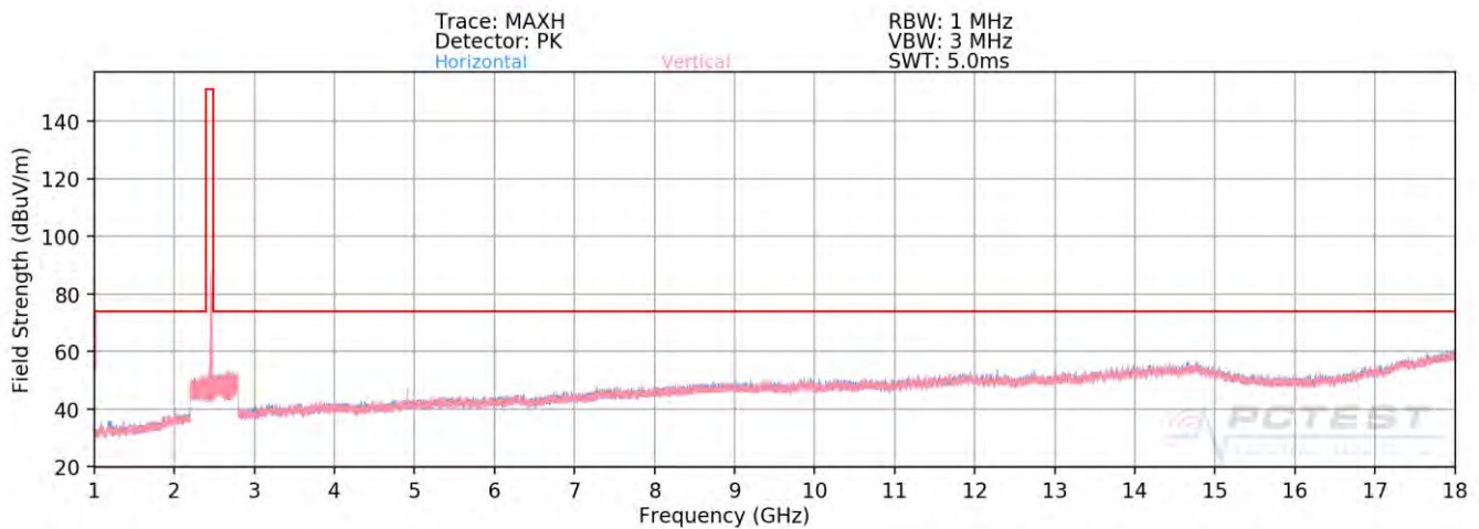
Plot 7-57. Radiated Spurious Plot above 1GHz MIMO (802.11ax OFDMA – 26 Tones – Ch. 11)
