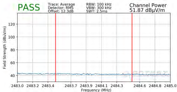
Plot 7-81. Radiated Restricted Upper Band Edge Measurement SISO ANT1 (Average – 242 Tones)
