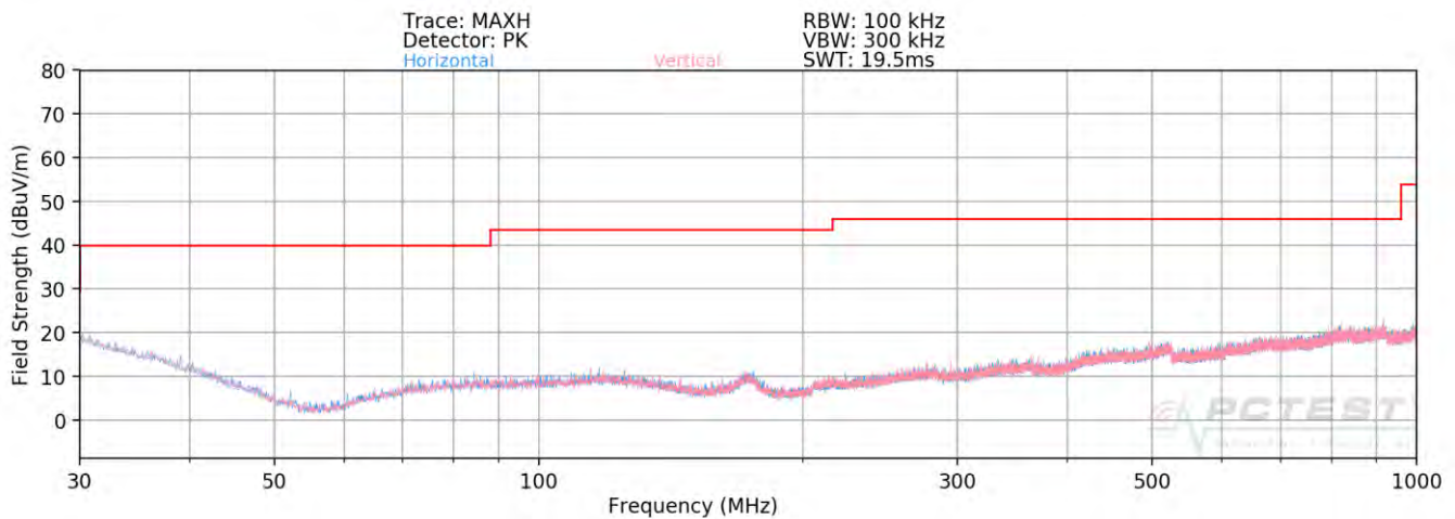
Plot 7-136. Radiated Spurious Plot below 1GHz MIMO (242 Tones)
