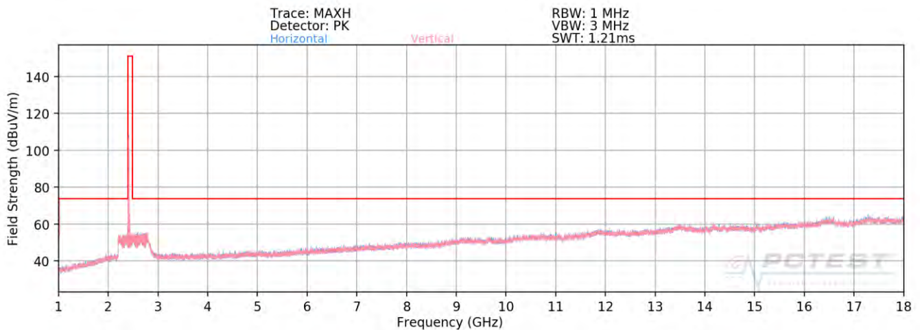
Plot 7-42. Radiated Spurious Plot above 1GHz SISO ANT1 (802.11ax OFDMA – 242 Tones – Ch. 1)
