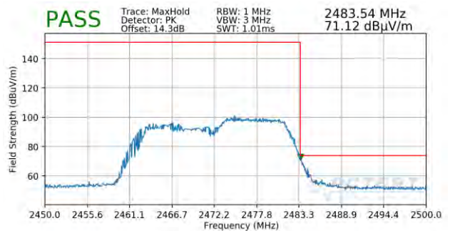
Plot 7-74. Radiated Restricted Upper Band Edge Measurement SISO ANT1 (Peak – 106 Tones)
