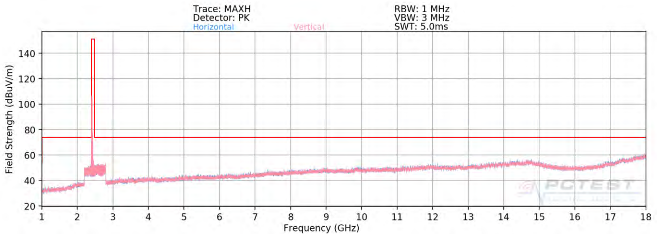
Plot 7-58. Radiated Spurious Plot above 1GHz MIMO (802.11ax OFDMA – 242 Tones – Ch. 1)
