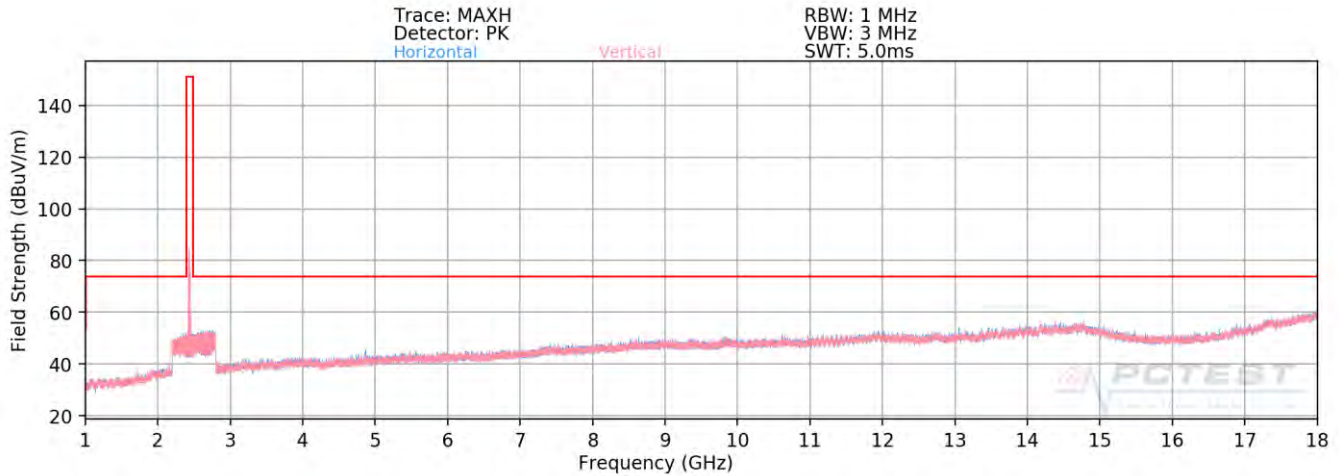
Plot 7-56. Radiated Spurious Plot above 1GHz MIMO (802.11ax OFDMA – 26 Tones – Ch. 6)
