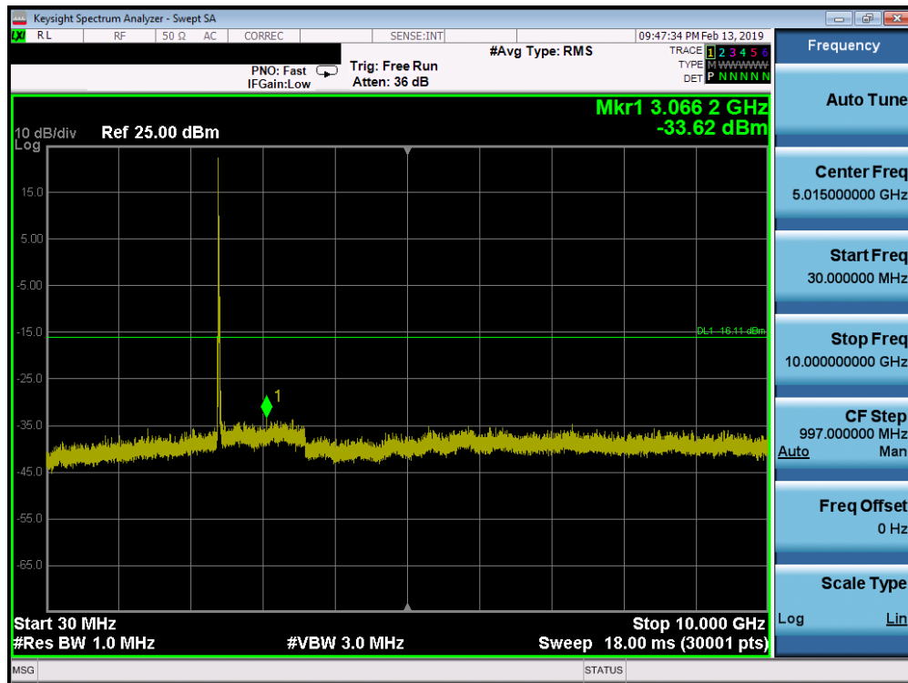
Plot 7-27. Conducted Spurious Plot SISO ANT1 (802.11ax OFDMA – 242 Tones – Ch. 1)
