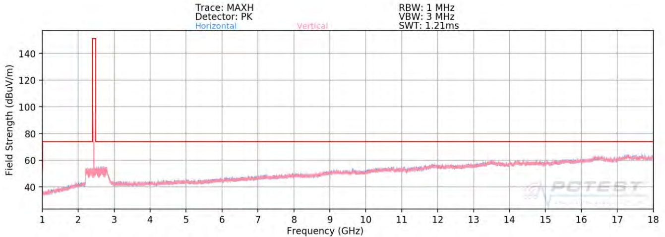
Plot 7-48. Radiated Spurious Plot above 1GHz SISO ANT2 (802.11ax OFDMA – 26 Tones – Ch. 6)
