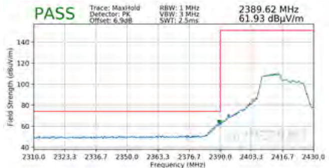
Plot 7-114. Radiated Restricted Lower Band Edge Measurement MIMO (Peak – 106 Tones)
