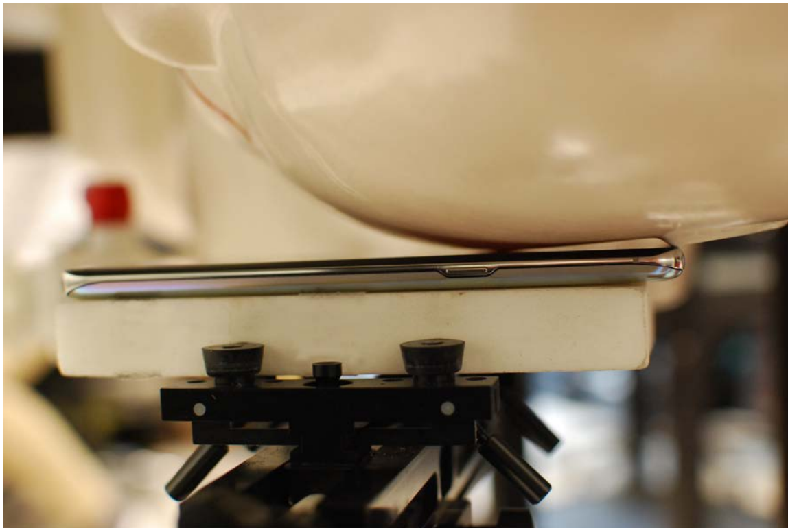
SAR Test Setup Photo 2 – Left Cheek
