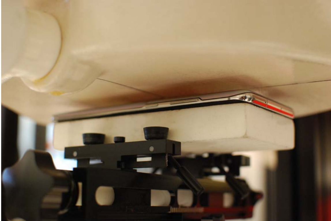
SAR Test Setup Photo 7 – Back Side at 0.7 cm
