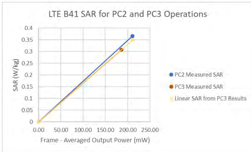
Figure 14-4 LTE Band 41 UCLA Body-Worn Linearity
