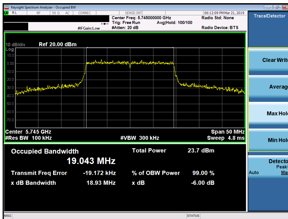
Plot 7-103. 6dB Bandwidth Plot SISO ANT2 (20MHz BW 802.11ax – Full Tones (UNII Band 3) – Ch. 149)
