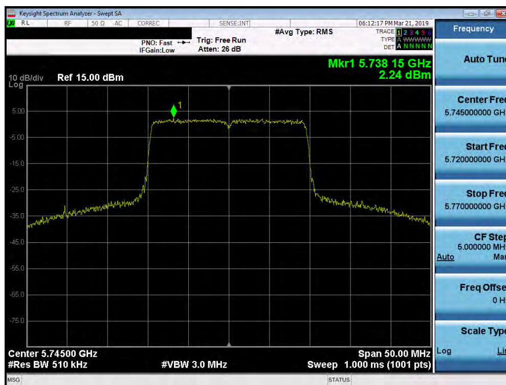
Plot 7-211. Power Spectral Density Plot SISO ANT2 (20MHz BW 802.11ax – Full Tones (UNII Band 3) – Ch. 149)
