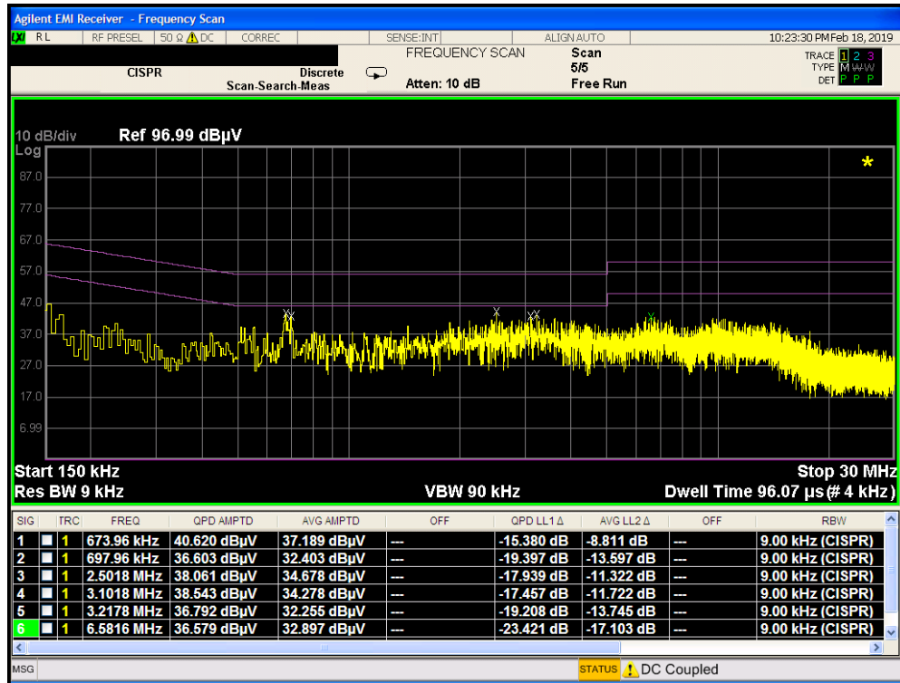
Plot 7-55. Line Conducted Plot with Bluetooth LE (L1) with Travel Adapter
