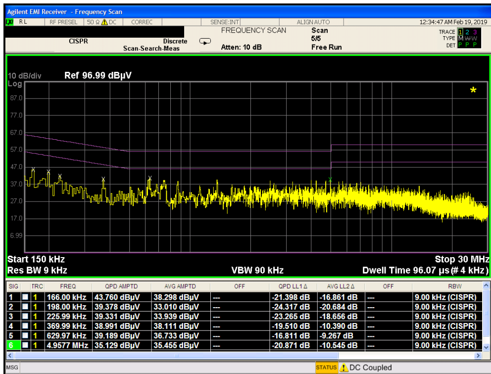
Plot 7-58. Line Conducted Plot with Bluetooth LE (N) with Wireless Charging Pad
