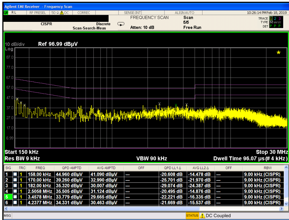
Plot 7-56. Line Conducted Plot with Bluetooth LE (N) with Travel Adapter
